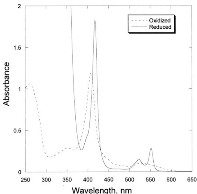
Fig. 8.3. Reduced (solid line) and oxidized (dashed line) spectra of the periplasmic fraction of E. coli cells expressing tri-heme cytochrome PpcA from Geobacter sulfurreducens . Note a large peak below \sim 360 nm in the reduced spectrum (products of dithionite oxidation).
