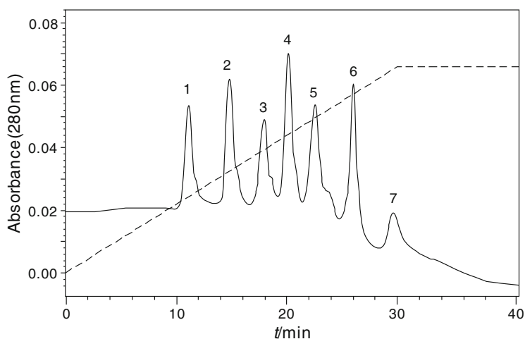
Fig. 5.5. Chromatogram of standard proteins by chromatographic cake (10 \times 50 mm). Stationary phase: PEG-600; linear gradient elution (dash line): 100% solution C to 100% solution D for 30 min with a 10-min delay; flow rate, 8.0 mL/min; peak: 1, cytochrome-C; 2, myoglobin; 3, RNase A; 4, lysozyme; 5, \alpha -chymotrypsin; 6, \alpha -amylase; 7, insulin. Total mass of proteins, 2.1 mg.
