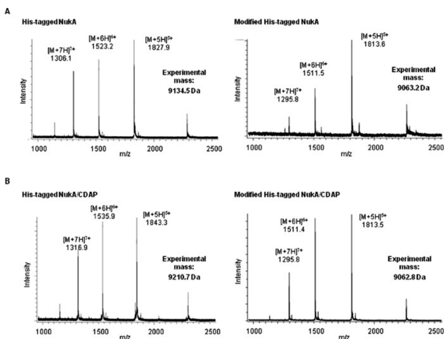
Fig. 13.1. ESI-MS spectra of the purified His-tagged NukaA and the modified His-tagged NukaA (a), and their masses cyanylated with CDAP (b). (a) From the recorded multiply charged ions, experimental masses of 9134.5 Da and 9063.2 Da could be calculated for His-tagged NukaA and the modified His-tagged NukaA, respectively. These results indicate that His-tagged NukaA (9134.5 Da) co-expressed with NukM for 20 h at 20°C is converted into the peptide (the modified His-tagged NukaA, 9063.2 Da) with decrease in mass of 71.3 Da. This mass reduction is in good agreement with the formation of unusual amino acids at the expected positions ( see Fig. 13.2). (b) His-tagged NukaA containing three Cys residues is used as a control. A total mass shift with +76.2 Da is observed by CDAP treatment, indicating complete CDAP addition to three free cysteine residues. In contrast, the modified His-tagged NukaA shows no mass change by CDAP treatment. These results suggest the presence of three thioether bridges in the modified His-tagged NukaA.
