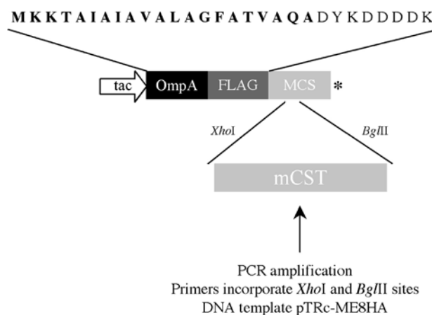
Fig. 14.1. pFLAG-mCST was constructed as described in (8). The coding sequence of the full-length mCST was amplified by PCR using pTRc-ME8HA (7) as the template and a forward primer that introduced an XhoI site and a reverse primer that introduced a BglII site. The resultant PCR product was digested with XhoI and BglII and ligated into the corresponding sites of pFLAG-ATS to generate pFLAG-mCST. Using this plasmid the mCST can be expressed in E. coli BL21 fused to an N-terminal OmpA signal sequence, shown in bold, and the eight amino acid residue FLAG-tag under the control of the IPTG inducible tac promoter (a hybrid of the E. coli trp and lac promoters).
