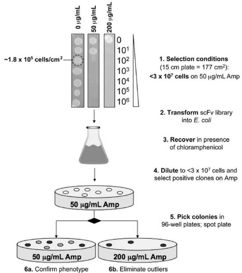
Fig. 4.3. Detailed strategy for the isolation of folded proteins (e.g., scFv antibodies) from recombinant libraries using the Tat folding reporter. Cells were serially diluted 10-fold (indicated by white triangle ) from an overnight culture such that the most dilute cells ( bottom spots in each image) are a 10^6 dilution of overnight culture.
