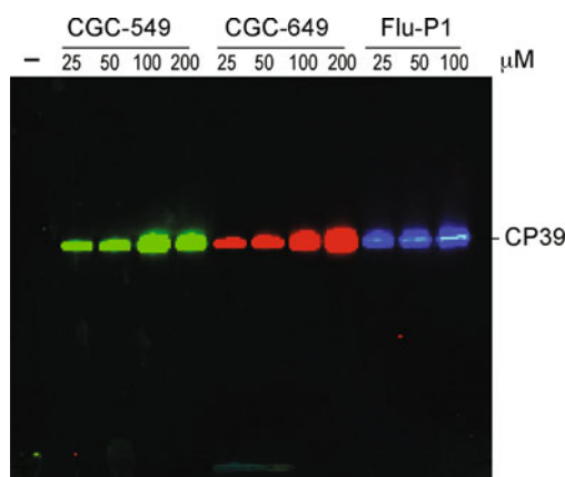
Fig. 6.3. The C-terminal thioester-tagged CP39 was incubated with 0, 25, 50, 100, or 200 \mu M CGC-549, CGC-649, or Flu-P1 peptide overnight at 4°C. The samples were electrophoresed on a 12% SDS polyacrylamide gel and electroblotted to a nitrocellulose membrane. The membrane was scanned using the Typhoon fluorescent imager with the 532/580 nm excitation/emission filter set for CGC 549 ( green ), 633/670 nm excitation/emission filter set for CGC 649 ( red ), and 488/520 nm for Flu-P1 ( blue ). The merged image for the three channels is shown.
