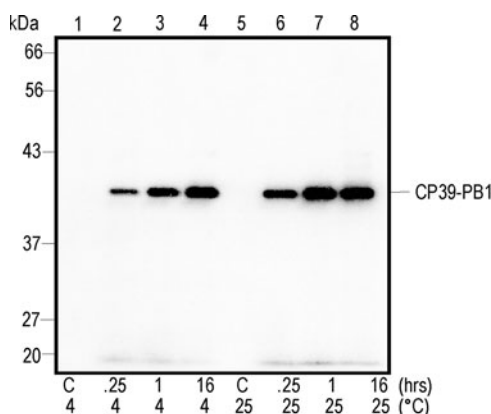
Fig. 6.4. Western blot analysis of the peptide PB1 ligated to the carrier protein (CP39) using anti-PB1 antiserum. PB1 was synthesized with an N-terminal cysteine (CTRSRHSSYPNEYEEDEEMEEEL; MW 2862 Da) and ligated to the C-terminal thioester-tagged carrier protein 39. The reaction times and temperatures are indicated. The samples were electrophoresed on a 12% SDS polyacrylamide gel and transferred to nitrocellulose. Anti-PB1 peptide antibody was used as the primary antibody. Lanes 1 and 5 are controls (C) that contain only carrier protein 39.
