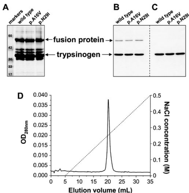
Fig. 10.2. Expression and purification of the intein–trypsinogen fusions. In the experiment shown here, wild-type cationic trypsinogen and pancreatitis-associated mutants p.A16V and p.N29I were expressed and purified. SDS-PAGE analysis of (a) inclusion bodies from LG-3 cells expressing the intein–trypsinogen fusions; (b) trypsinogens eluted from the ecotin affinity column; (c) trypsinogen fractions after Mono S chromatography. Inclusion body fraction prepared from 1.8 mL LG-3 culture ( OD_{600} = 1.6 ) or \sim 5 \mu\text{g} purified protein was loaded per lane. (d) Mono S chromatography of cationic trypsinogen eluted from the ecotin affinity column. The column was developed with a 0–0.5 M gradient of NaCl at a flow rate of 1 mL/min. Under these conditions only pure trypsinogen is eluted, while unprocessed fusion proteins are not recovered. Reproduced from (9) with permission from Elsevier Science.
