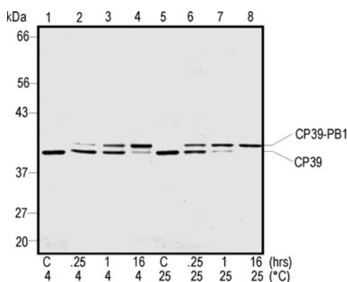
Fig. 6.2. Analysis of intein-mediated protein ligation (IPL) by Coomassie blue-stained SDS-PAGE. PB1 was synthesized with an N-terminal cysteine (CTSRHSSYPNEY-EEDEEMEEEL; MW 2862 Da) and ligated to the C-terminal thioester-tagged carrier protein 39. The reaction times and temperatures are indicated. The samples were electrophoresed on a 12% SDS polyacrylamide gel and examined by Coomassie blue staining. Lanes 1 and 5 are controls (C) that contain only carrier protein 39.
