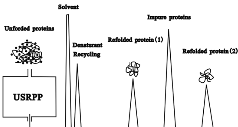
Fig. 5.1. Scheme of an ideal protein folding liquid chromatography having four functions simultaneously (3, 5, 6). Four functions: removal of denaturants, refolding of target proteins, separation from contaminant proteins including misfolded intermediates of the target protein, and easy recovery of denaturants.
