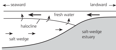
Salt wedge
