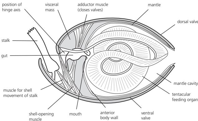
Brachiopoda
