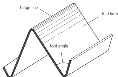
Fold
