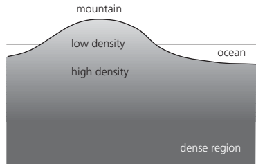
Pratt model
