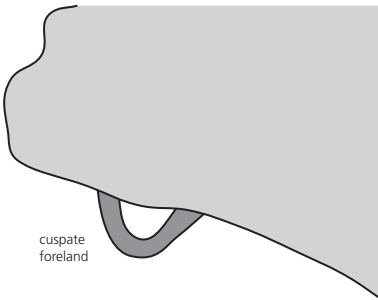
Cusped foreland
