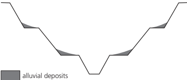
river terrace
