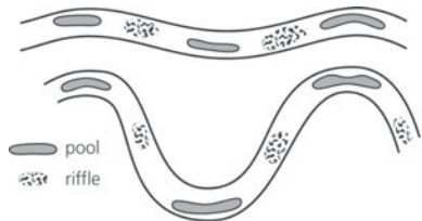
Pool-and-riffle
