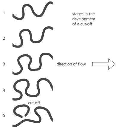
Cut-off
