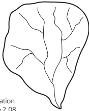
bifurcation ratio = 2.08
