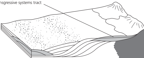
Transgressive systems tract
