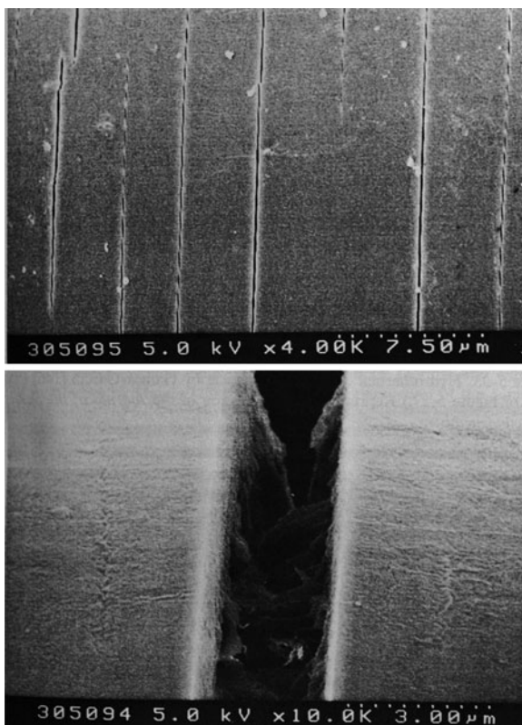
Fig. 6.33 Transverse cracks in the cuticle (Type 2 crack) from long term uv-exposure at high RH and extension (SEM kindly provided by Sigrid Ruetsch of Textile Research Institute)
