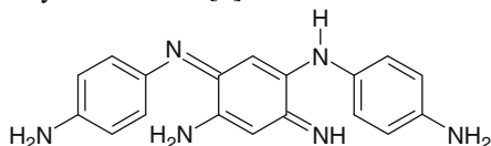
Trimer of p -phenylenediamine and m -phenylenediamine (XXXI)
