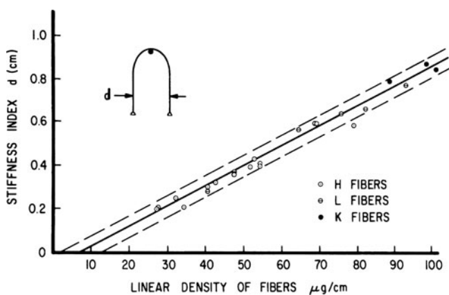
Fig. 9.16 Hair fiber stiffness index and linear density [49] (reprinted with permission of the Journal of the Society of Cosmetic Chemists)
