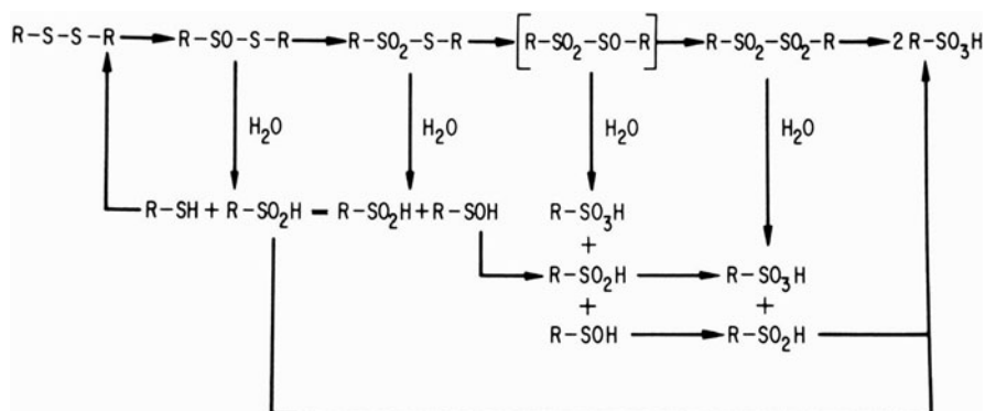
Fig. 5.5 S-S fission of disulfides in an aqueous alkaline oxidizing medium [24] (Reprinted with permission of the Journal of the Society of Cosmetic Chemists)
