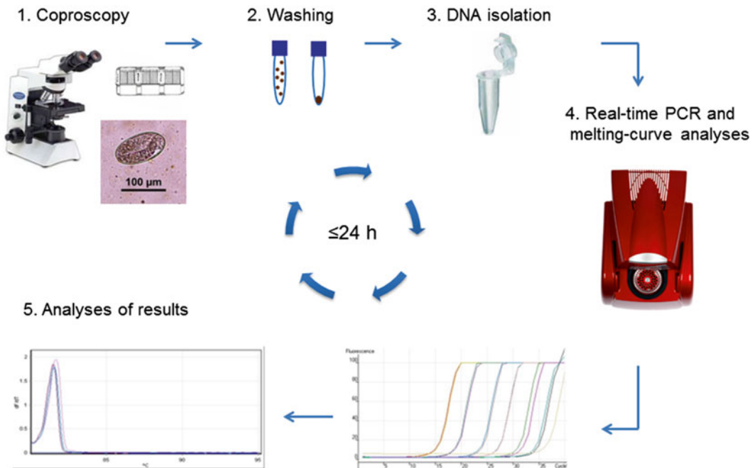
Fig. 1 Step-by-step protocol for the molecular diagnosis of strongylid nematode infections from small ruminant fecal samples. Following coproscopy (1), the fecal suspension is washed and nematode parasite eggs are recovered (2). Genomic DNA is isolated from eggs (3), and regions within the second internal transcribed spacer of nuclear ribosomal DNA specifically amplified by real-time PCR (4). After completion of PCR and melting-curve analysis (5), an estimate of the contribution of individual nematode species or genera to the egg count is estimated
