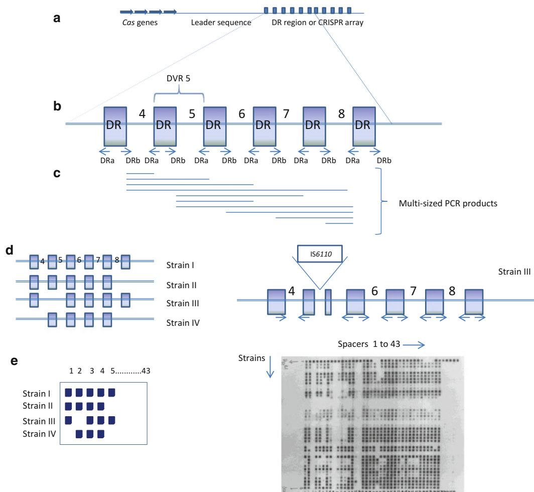
Fig. 1 Schematic structure of a CRISPR/Cas region in MTBC strains and application of the CRISPR array, to the development of the spoligotyping method, using 43 selected spacer sequences. (a) General structure of a CRISPR/Cas region; (b) structure of DR region: 0–56 copies of 36 bp direct repeats, separated by variable spacer sequences of 36–51 bp, whose order is well conserved in the genome of MTBC. Spacers, here numbered from 4 to 8. The DRs together with the adjacent spacers form the direct variant repeats (DVRs); (c) PCR amplification of the DR flanking spacers, using primers DRa and DRb, one of them biotin labeled, complementary to the conserved direct repeats; (d) five pretend patterns in the DR region and possible formation of strain III pattern by insertion of IS6110 sequence in DVR 5, hampering the amplification of spacer 5 by loss of primer DVRb hybridization site. (e) Simplified spoligotyping membrane results obtained for the five strains and example of a real spoligotyping membrane. Note that the genome spacer order/number does not correspond to the membrane spacer order/number
