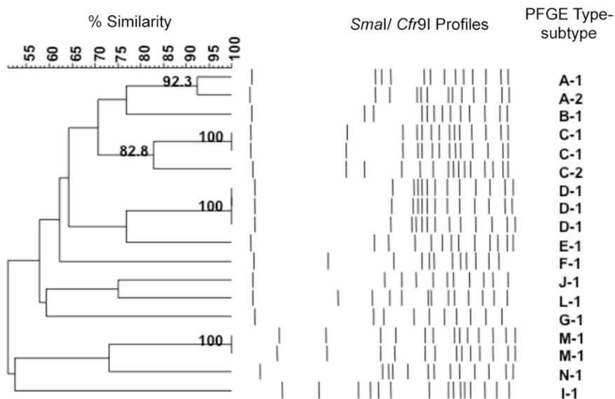
Fig. 3 Representative image of a dendrogram of PFGE patterns of bovine streptococci ( S. dysgalactiae subsp. dysgalactiae ) (adapted from Rato et al. ( http://wwwnc.cdc.gov/eid/article/16/1/09-0632-f1 )) [7]. The dendrogram was produced by using Dice coefficients and an unweighted pair group method using arithmetic averages (UPGMA). Default clustering settings of 0 % optimization (i.e., the relative distance an entire lane is allowed to shift in matching attempts) and 1.5 % band position tolerance were used
