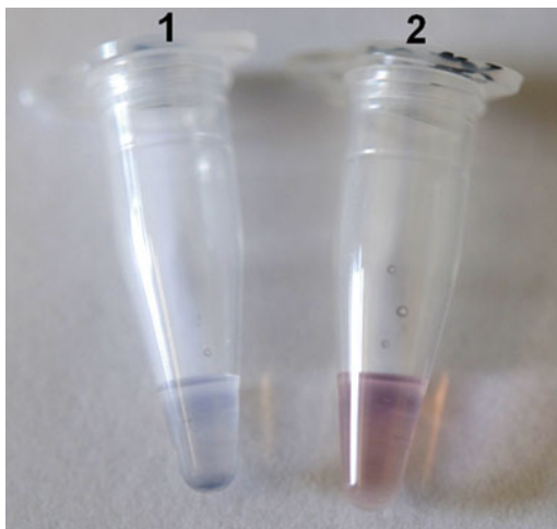
Fig. 2 Colorimetric assay using unmodified AuNPs. Each tube contains 5 \mu L of sample (SVCV RNA), 1.8 \mu M of oligonucleotide probe, and 0.1 M of NaCl. The samples were denatured at 95 °C for 30 s and annealed at 58 °C for 30 s and then cooled at room temperature for 10 min. 10 \mu L of AuNPs solution was added and results were observed within 1 min. Tube 1 contains a positive sample and tube 2 contains a negative sample. In the positive sample, the color changes from red to blue
