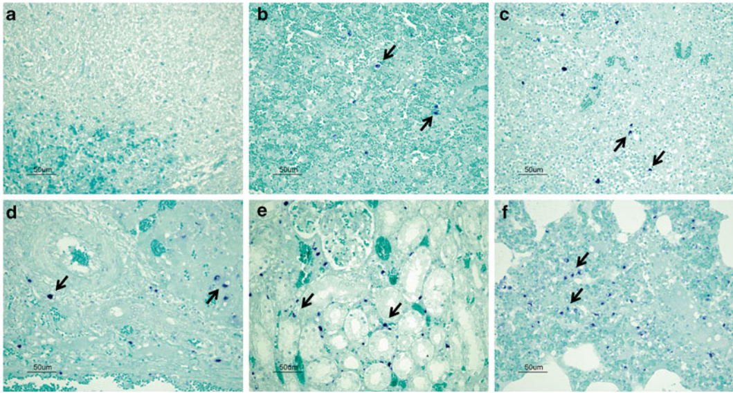
Fig. 2 ASFV-DNA detection using DIG-labeled probes in formalin-fixed paraffin-embedded tissues. (a) Negative lymph node. (b–f) Positive tissues, where dark-blue dots in the preparation correspond to the presence of viral nucleic acids (examples of positive labeling are indicated with arrows ). (b) Spleen. Intense positive detection in red pulp macrophages and trabecular medullary areas. (c) Lymph node. Moderate positive detection in perifollicular macrophages (marginal zone). (d) Liver. Moderate to intense positive detection in sinusoidal and alveolar macrophages and Kupffer cells. (e) Kidney. Intense positive detection in circulating macrophages and renal endothelium. (f) Lung. Intense positive detection in pulmonary alveolar, vascular, and parenchymal macrophages
