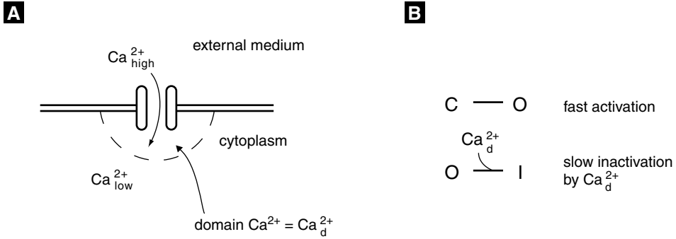
Figure 4.2 (A) Cartoon of domain calcium. (B) State diagram for \text{Ca}^{2+} channel.
