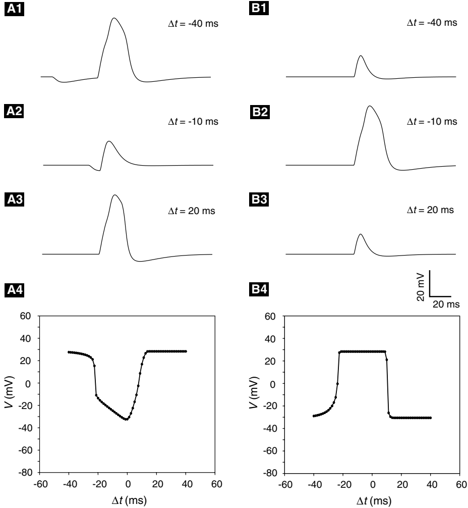
Figure 6.10 (A1–A4) Implementing subtraction with excitation and inhibition. (A1–A3) membrane potential time courses V of target neuron for excitatory input from receptor cell R_2 and inhibitory input from R_1 , offset in time by \Delta t (see schematic in Figure 6.8B). Results for different values of \Delta t , -40 , -10 , 20 ms, are shown in (A1–A3), respectively. (A4) Response plot of peak of V_1 (associated with input from R_1 ) versus \Delta t . Parameter values for excitatory inputs as in Figure 6.9; for inhibitory input kinetics: \alpha_1 = 0.5/\text{ms} , \beta_1 = 0.1/\text{ms} , V_{\text{syn},1} = -84 mV, \theta_{\text{syn}} = 20 mV, k_{\text{syn}} = 2 mV, g_1 = 2.5 mS/cm ^2 , g_2 = 2.0 mS/cm ^2 . (B1–B4) Directionally selective, motion-detecting neuron. (B1–B3) Membrane potential time courses V_2 of second layer neuron N_2 (Figure 6.8C) that receives excitatory input from receptor cell R_2 and inhibitory input from N_1 (A1–A4). Results for different values of \Delta t , -40 , -10 , 20 ms, are shown in panels (B1–B3), respectively. (B4) Response plot of peak of V_2 versus \Delta t . Parameter values for N_1 and the inputs to N_1 are same as in the left panels; for N_2 and inputs, the parameters are identical as onto N_1 (with g_{N2,N1} = 2.5 mS/cm ^2 , g_{N2,R2} = 2.0 mS/cm ^2 ). Input from R_2 to N_2 is delayed in each case by 10 ms. At t = 0 neurons are at rest, V = -60.9 mV, w = 0.0149 and synaptic gating variables are zero.
