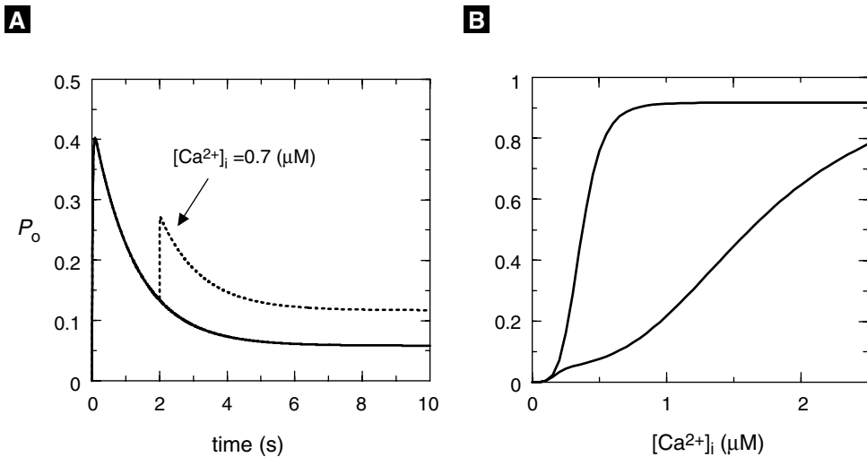
Figure 5.6 Keizer-Levine model: (A) Time course of response of P_O to a step increase in [\text{Ca}^{2+}]_i from 0.1 to 0.35 \mu\text{M} (solid). Dotted curve shows "adaptation" when a second step to 0.7 \mu\text{M} is applied at t = 2 s. (B) Peak and steady-state levels of P_O for different values of [\text{Ca}^{2+}]_i . (see Keizer and Levine (1996), Figure 5.3, and Figure 5.4, this chapter.) Parameters: k_a^+ = 1500 / (\mu\text{M}^4 \text{ s}) , k_a^- = 28.8 / \text{s} , k_b^+ = 1500 / (\mu\text{M}^3 \text{ s}) , k_b^- = 385.9 / \text{s} , k_c^+ = 1.75 / \text{s} , k_c^- = 0.1 / \text{s} .
