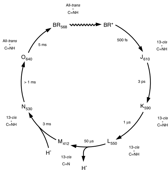
Figure 3.16 An irreversible diagram for the light-driven proton pump, bacteriorhodopsin, a 27 kD protein from the salt tolerant bacterium, Halobacterium halobium . Light absorbed in the step \text{BR}_{568} \rightarrow \text{BR}^* drives the trans to cis conformational change in retinal, leading to the release of a proton. Redrawn from Lauser (1991).
