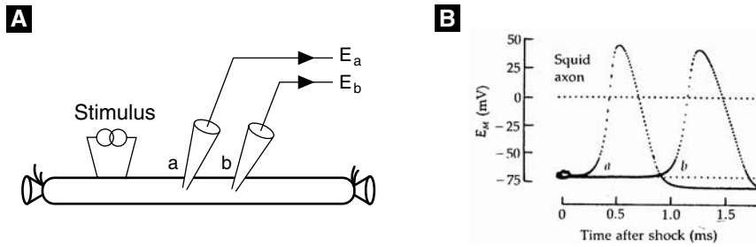
Figure 1.1 (A) Schematic diagram of the recording electrodes (a and b) used to detect action potentials following a stimulus shock in an isolated giant axon from squid. Adapted from Hille (2001). (B) The membrane potential recorded at electrodes a and b in the upper panel following a depolarizing shock. Reprinted from delCastillo and Moore (1959).
