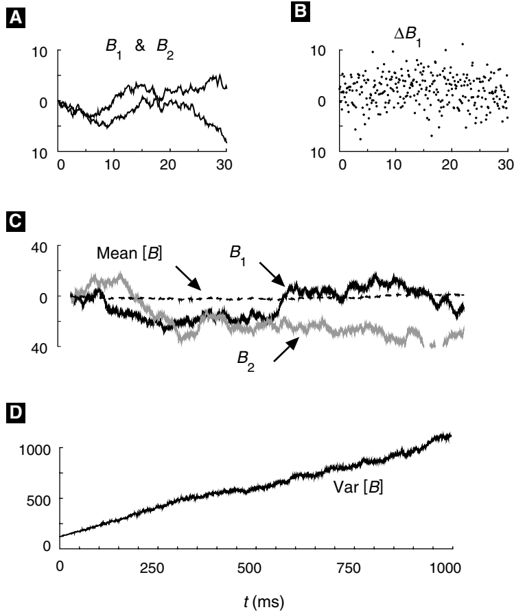
Figure 11.9 Two instantiations of a Wiener process, B_1 and B_2 , have trajectories similar to the random walks shown in Figure 12.4. The mean of 100 trials is near zero, while the variance of 100 trials increases linearly with time. In these simulations the increments ( \Delta B ) are normally distributed with mean zero and variance 1/\Delta t , where \Delta t is the integration time step.
