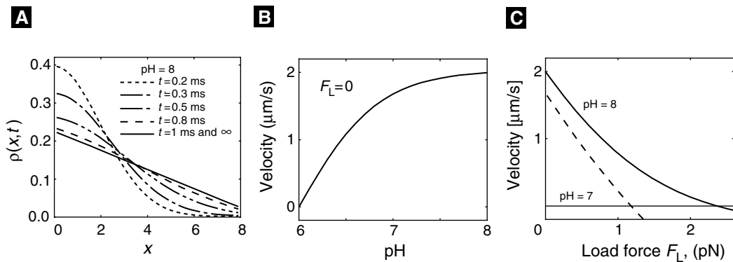
Figure 13.8 Numerical results of the simplified F_0 motor. Here pH is the pH value of the right compartment. The external load force is F_L . In all the figures the number of grid points used in the simulations was M = 32 . (A) Relaxation of the marginal density \rho = \rho_{\text{rmon}} + \rho_{\text{off}} to steady state for pH = 8 and no external load. (B) Motor velocity as a function of pH with no external load. (C) Motor velocity as a function of the load force for pH = 7 and pH = 8.
