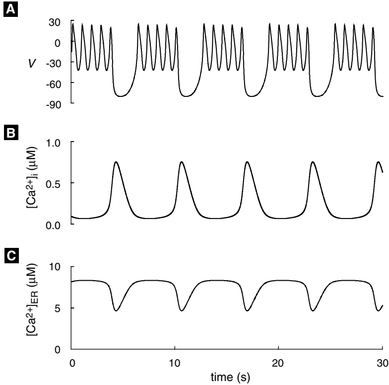
Figure 5.16 Full gonadotroph model (Equations (5.55)–(5.59) in dimensional form ): bursting as a result of interaction between the plasma membrane oscillator and the ER oscillator. Plasma membrane voltage V (A), cytosolic calcium level [Ca^{2+}]_i (B), and the store calcium content [Ca^{2+}]_{ER} (C) are shown. Each spike in [Ca^{2+}]_i hyperpolarizes the plasma membrane by activating calcium-sensitive potassium channels. ER parameters as in Figure 5.14 except: L = 1.48 pL/s, P = 2960 pL/s, K_i = 0 \mu M, A = 2 /s, V_{SERCA} = 480 aMol/s, V_p = 400 aMol/s. Plasma membrane (Morris–Lecar) parameters: V_K = -85 mV, V_{Ca} = 120 mV, K_{K(Ca)} = 0.5 \mu M, C_m = 1 \mu F/cm 2 , g_K = 20 \mu S/cm 2 , g_{Ca} = 20 \mu S/cm 2 , g_{K(Ca)} = 8 \mu S/cm 2 , \phi = 12 /s, v_1 = -3 mV, v_2 = 30 mV, v_3 = -20 mV, v_4 = 30 mV, \alpha = 0.2 (aMol·cm 2 )/nC.
