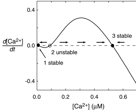
Figure 8.3 Using parameters as in Exercise 4, the cubic rate function dc/dt = f(c) of the fertilization \text{Ca}^{2+} wave model, (8.15), leads to a bistable phase portrait (x-axis). Equilibrium point 1 represents a stable resting state at basal [\text{Ca}^{2+}]_i (ER replete) while equilibrium 3 is a stable resting point at high [\text{Ca}^{2+}]_i (ER empty). Equilibrium 2 lies between points 1 and 3, is unstable, and corresponds to a threshold for \text{Ca}^{2+} -induced \text{Ca}^{2+} release.
