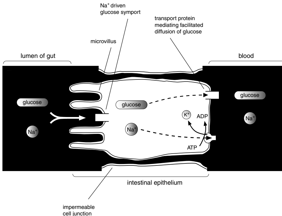
Figure 3.9 A cartoon representing the cotransport of glucose and \text{Na}^+ into intestinal epithelium, followed by the passive transport of glucose into the blood. Energy stored in the gradient of \text{Na}^+ (higher in the lumen of the gut) is utilized to transport glucose from a high concentration to a low concentration. \text{Na}^+ that accumulates in the epithelial cells is removed by active transport into the blood by the \text{Na}^+/\text{K}^+ ATPase. Adapted from Alberts et al. (1994).
