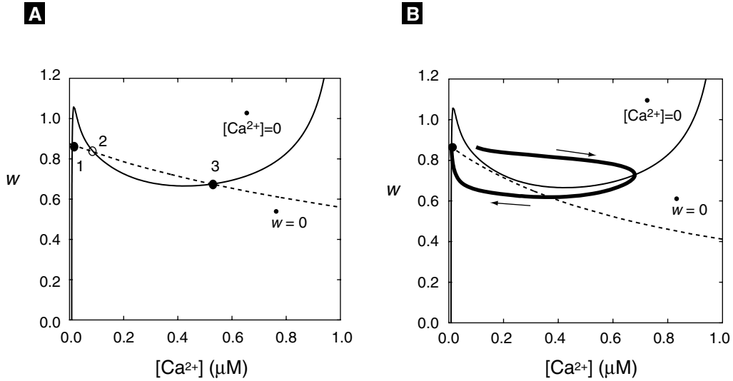
Figure 8.6 The (w, [Ca^{2+}]_i) phase plane for the reaction terms of the fertilization Ca^{2+} wave model (8.6)–(8.7) can exhibit bistability (A) or excitability (B) with a change of IP_3R parameters. Parameters as in Exercise 4 except d_2 = 2 \mu M in the bistable case, while d_2 = 1 \mu M in the excitable case. In the Li–Rinzel reduction of the DeYoung–Keizer IP_3R model, this change in d_2 increases equilibrium IP_3R inactivation (note the downward/leftward shift in w nullcline) and eliminates the high [Ca^{2+}]_i equilibrium present in (A).
