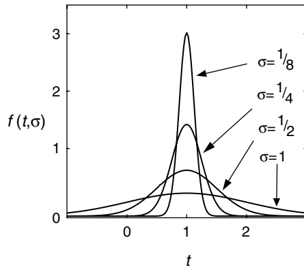
Figure 12.10 The Dirac delta function can be viewed as the limit of a sequence of normal probability density functions as the standard deviation goes to zero.
