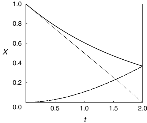
Figure 1.9 The forward Euler method of numerical integration relies upon a series of short linear approximations using the derivative at the old time point. The solution to (1.6) with \tau = 2 is shown in solid, the linear approximation using the derivative at t = 0 ( -0.5 ) is shown in dots, and the difference between these two curves is shown in dashes. Note that by t = 2 , the magnitude of error between the actual and approximate functions is equal to the value of the actual function.
