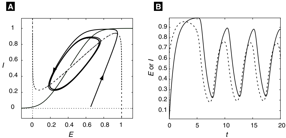
Figure 6.13 Network oscillations. (A) Phase plane and (B) time courses for the firing rate model, with increased input to the excitatory population: P_E = -1 . Other parameters are as in Figure 6.12. Dashed line is for E -nullcline in (A) and E vs. t in (B); solid line is for I -nullcline in (A) and for I vs. t in (B). Darker solid curve in (A) is the phase plot.
