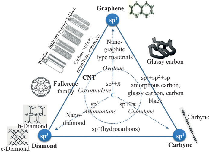
Figure 2.2. Simplified classification of carbon materials based on the hybridization of carbon atoms.
