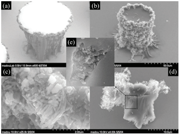
Figure 1.4. Typical SEM images of (a) a photoresist post obtained from modified SU-8 before pyrolysis, (b) a carbon post after pyrolysis, (c) a carbon post surface under high magnification, (d) a broken piece of a carbon post with embedded carbon fibers, and (e) an embedded cavity under high magnification [24, 25].
