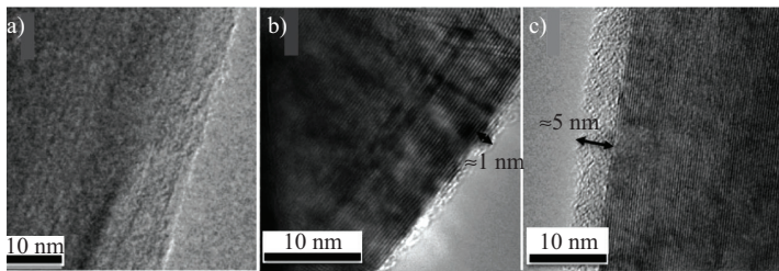
Plasma polymerization of an acrylic monomer on carbon nanotubes (CNTs) surfaces: (a) bare CNT, (b) 5-minute polymerization, (c) 15-minute polymerization [1].
