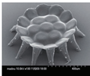
Microtable made with carbon MEMS at UCL. See also Figure 1.3 (Courtesy of Dr. Marc Madou, UC Irvine, CA, USA).
