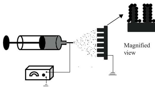
Figure 6.14. Schematic for fabricating hierarchical C-MEMS structures by combining electrospaying with lithographically fabricated master stamp.
