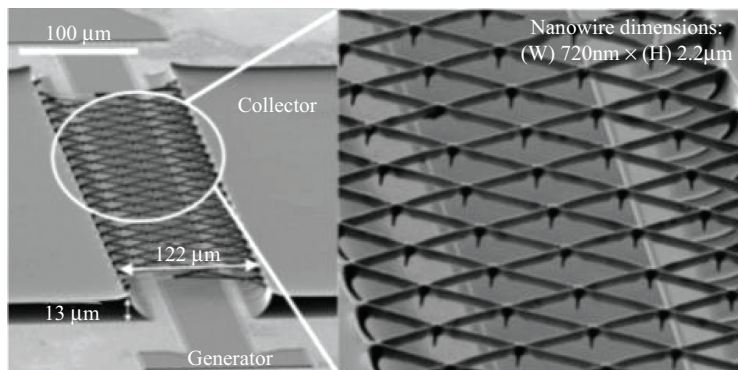
Figure 4.29. SEM images of nanoelectrode set [26].
