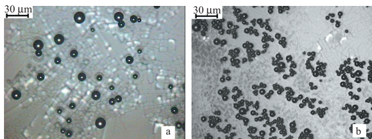
Figure 6.6. Optical micrographs showing the effect of surfactant concentration on particle size at R/C = 25 , stirring time of 5 h in low surfactant concentration region (a) 1% (v/v) span-80; (b) 4% (v/v) span-80.
