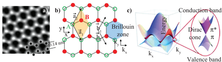
Figure 2.10. (a) Atomic-resolution image of a graphene sheet, with an indication of the carbon–carbon bond length of about 0.142 nm. (b) Honeycomb lattice structure of graphene exhibiting a basis with two carbon atoms, A and B, per unit cell [43]. (c) Idealized Brillouin zone (graphene \pi -band) with a zoom to the K-point, where the bands cross at the Fermi level forming a Dirac cone.
