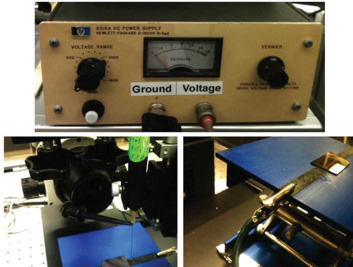
Figure 5.10. Photographs of voltage supply, syringe, and grounded substrate of EMS setup [8].
