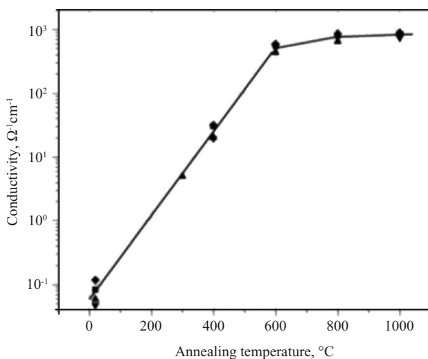
Figure 4.5. The conductivity versus annealing temperature graph [13].
