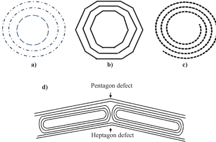
Figure 2.7. Top views of MWCNTs: (a) cylindrically curved Russian inset doll model, (b) coaxial polygon, and (c) graphene sheets scroll (according to Amelinckx et al. [34]). The figure (d) reports instead a scheme representing the structure of an encapsulate kink in an MWCNT.
