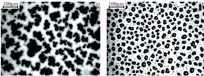
Figure 6.3. Optical micrographs showing the transition to nonspherical shapes of RF-derived carbon xerogel microparticles with a change in dilution ratio: (a) R/W = 0.037; (b) R/W = 0.0037. Other conditions for both cases are R/C = 25, surfactant concentration = 1% (v/v), and stirring time = 5 h.
