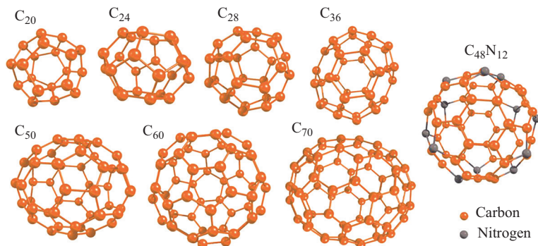
Figure 2.8. Family of fullerene carbon materials.
