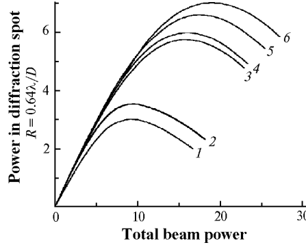
Figure 4.1.1. Dependence of the power in the diffraction spot on the total power of the beam (power optimization curves). Types of beams: (1) truncated Gaussian beam, (2) unlimited Gaussian beam, (3) hyper-Gaussian beam directed at an angle to the wind, (4) wide Gaussian beam, (5) super-Gaussian beam, and (6) hyper-Gaussian beam directed with a side to the wind.
