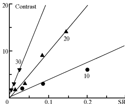
Figure 3.2.3. Dependence of PSF contrast on the Strehl ratio at modal correction for the aperture diameter D/r_0 = 10, 20 , and 30 . The straight-line slope coefficients obtained from fitting by linear regression are equal to 37, 99 , and 206 , respectively. The contrast is defined as the ratio of the PSF intensity on the optical axis ( \alpha = 0 ) to the intensity at the level of the first light fringe ( \alpha \cong 2\lambda/D ).
