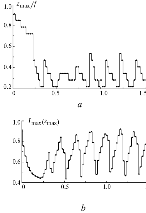
Figure 4.3.1. Dynamics of (a) the waist position and (b) the peak intensity in the waist cross section at l_0=24 . The intensity is normalized to the diffraction-limited value of the intensity at the beam focus. The time t is normalized to the convective time 2a_0/V .
