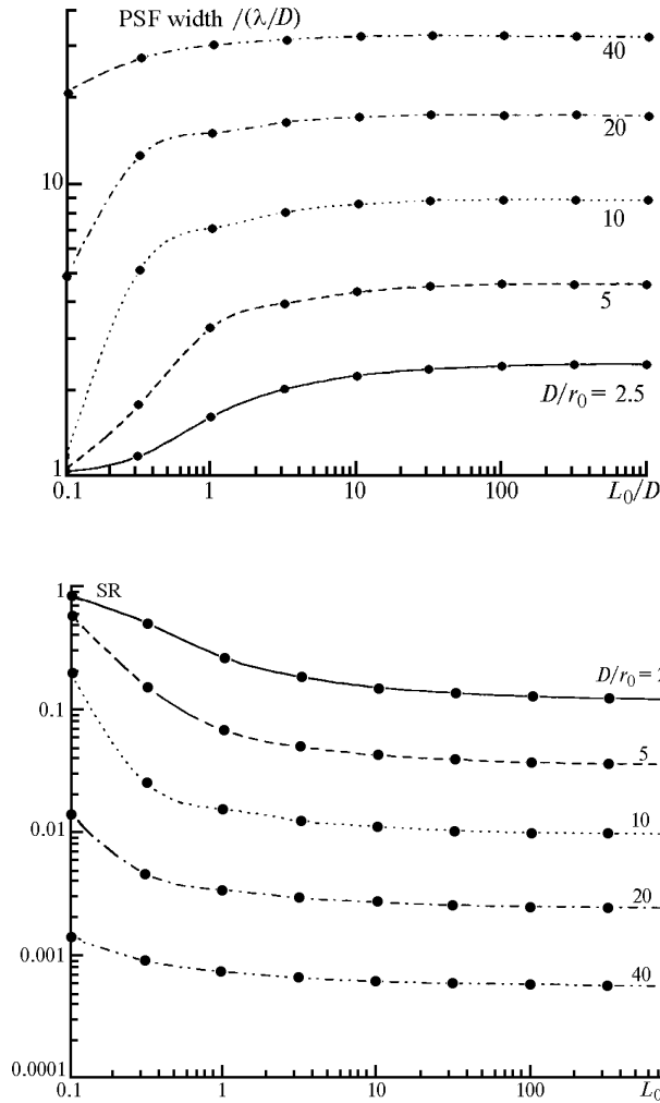
Figure 3.1.3. Dependence of PSF width and SR on L_0/D at different values of D/r_0 .
