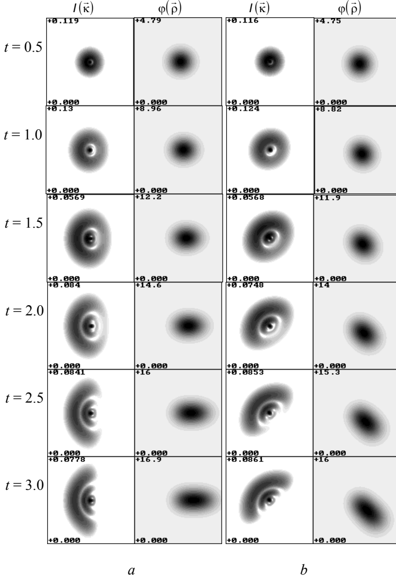
Figure 1.1.1. Dynamics of thermal blooming under conditions of forced convection (isobaric approximation): (a) wind is directed along the 0x-axis and (b) at an angle of 45 deg to the 0x-axis; I(\vec{k}) is the intensity distribution in the far zone; \varphi(\vec{\rho}) is the phase screen.
