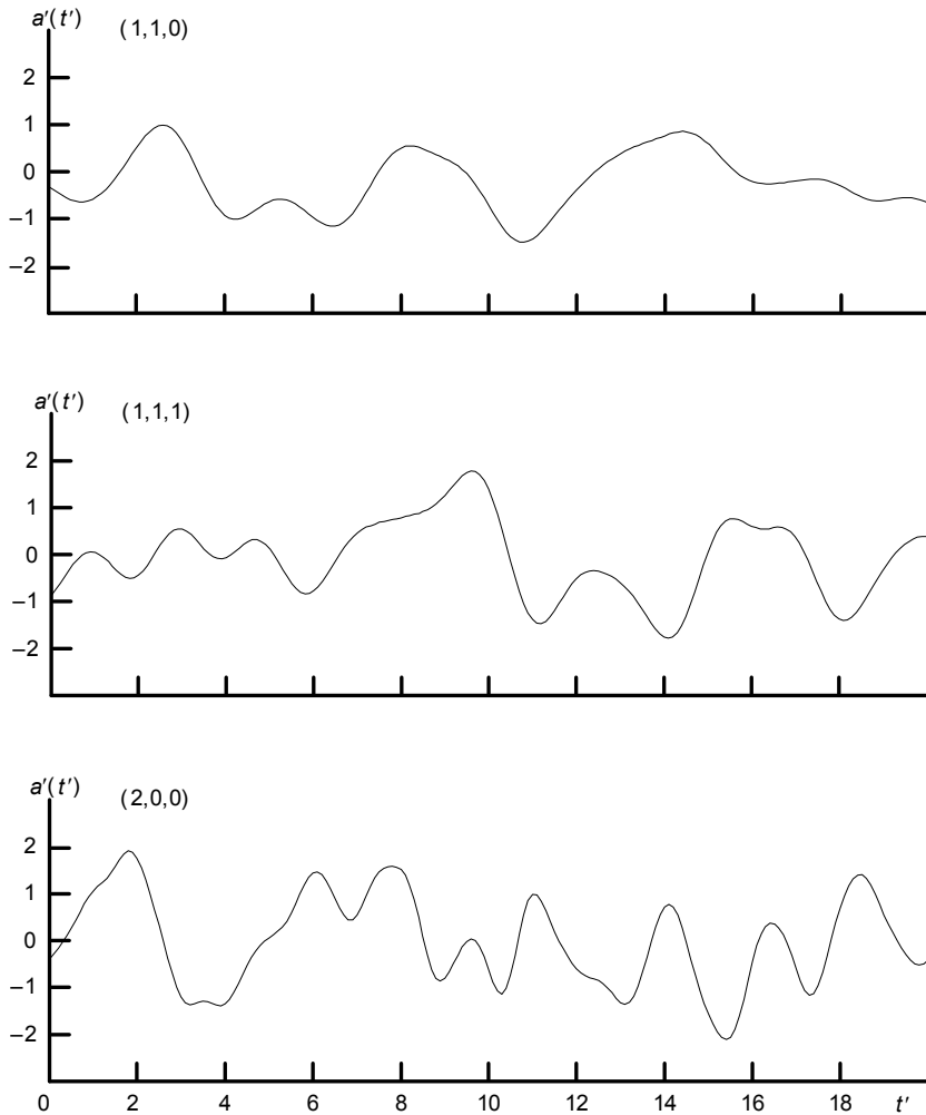
Figure 1.3.2. Random temporal samples of tilt and defocusing coefficients: a'_n = a_n / \sigma_n , t' = t \times V / R ; \sigma_n is the standard deviation; L_0/D = 10 . The numbers in parentheses above the curves correspond to radial order, azimuth frequency, and parity parameter.
