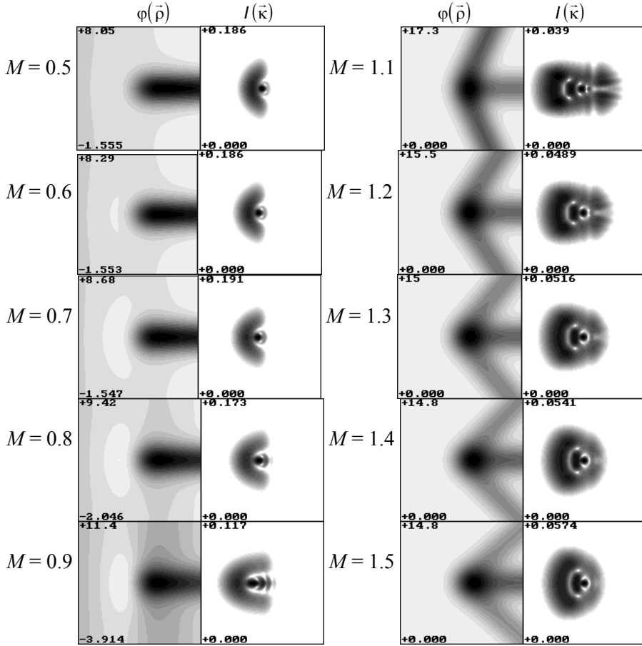
Figure 1.1.2. Thermal blooming behind the phase screen under conditions of forced convection (stationary solution of the linearized equations of hydrodynamics); I(\bar{\kappa}) is the intensity distribution in the far zone, \phi(\bar{\rho}) is the phase screen.
