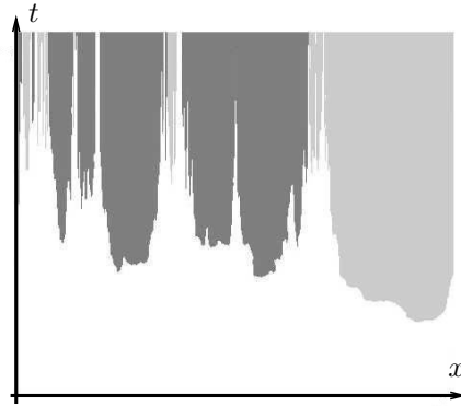
Fig. 7.1 A 1+1-dimensional slice of the spacetime in an eternally inflating universe (numerical simulation in [Vanchurin et al. (2000)], see also Fig. 6.2). Shades of different color represent different regions where reheating took place. The reheating surface is the line separating the white (inflating) domain and the shaded domains.
