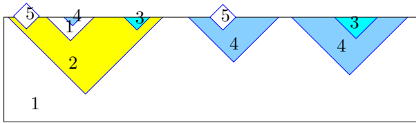
Fig. 5.2 A conformal diagram of the spacetime where self-reproduction occurs via bubble nucleation. Regions labeled “5” are asymptotically flat ( \Lambda = 0 ).
