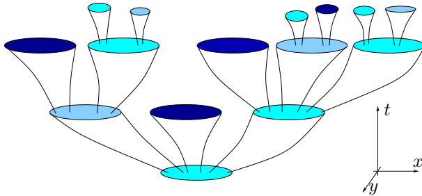
Fig. 3.1 A qualitative diagram of self-reproduction during inflation. Shaded spacelike domains represent Hubble-size regions with different values of the inflaton field \phi . The time step is of order H^{-1} . Dark-colored shades are regions undergoing reheating ( \phi = \phi_* ); lighter-colored shades are regions where inflation continues. On average, the number of inflating regions grows with time.
