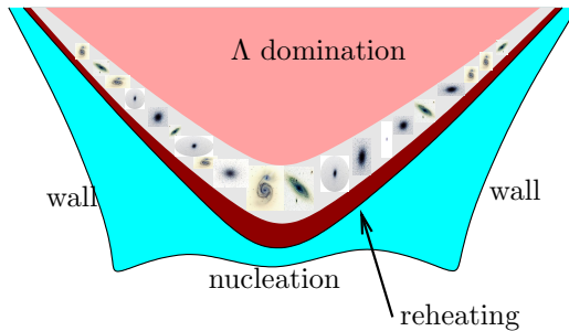
Fig. 3.2 A spacetime diagram of a bubble interior. The infinite, spacelike reheating surface is shown in darker shade. Galaxy formation is possible within the spacetime region indicated.
