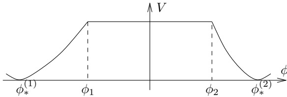
Fig. 6.1 Illustrative inflationary potential with a flat self-reproduction regime \phi_1 < \phi < \phi_2 and deterministic regimes \phi_*^{(1)} < \phi < \phi_1 and \phi_2 < \phi < \phi_*^{(2)} .
