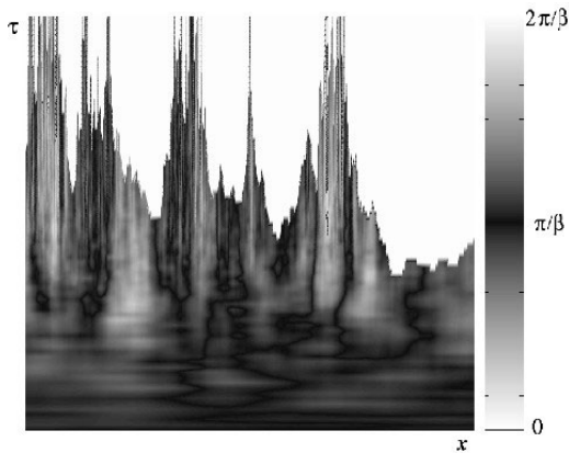
Fig. 6.2 A 1+1-dimensional slice of spacetime in a two-field inflationary model (numerical simulation in [Vanchurin et al. (2000)]). Shades denote different values of the field \chi , which takes values in the periodically identified interval [0, 2\pi/\beta] . The white region represents the thermalized domain. The boundary of the thermalized domain is the reheating surface in spacetime, which contains regions with all possible values of the field \chi .
