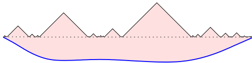
Fig. 5.3 A conformal diagram of the future part of a landscape-driven spacetime (figure from [Winitzki (2005b)]).
