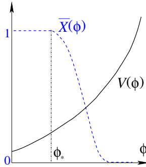
Fig. 4.4 Probability \bar{X}(\phi) of having no eternal points is very small in the inflating regime but almost equal to 1 near reheating, \phi \approx \phi_* .
