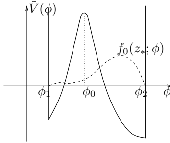
Fig. 8.2 Sketch of the eigenfunction f_0(z_*; \phi) (dashed line) interpreted as the wavefunction of a stationary state with zero energy in the potential \tilde{V}(\phi) (solid line). Due to exponential suppression by the potential barrier, the amplitude of f_0 in the right region is exponentially larger than that in the left region.
