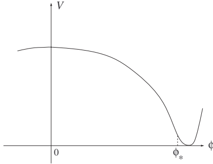
Fig. 2.1 The inflaton potential for the “new” inflationary scenario at T = 0 . The neighborhood of the maximum of the potential at \phi = 0 is very flat, so that the field \phi changes very slowly. Thermalization occurs after the field \phi finally rolls down to the “thermalization point” \phi = \phi_* .
