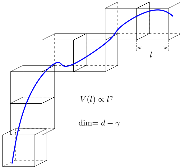
Fig. 4.1 Definition of “box” fractal dimension. The given set (curved line) is approximated by cubes of size l ; the total volume scales as V(l) \propto l^\gamma for l \rightarrow 0 , and the fractal dimension is then d - \gamma where d is the dimension of space.
