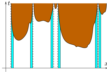
Fig. 7.2 A schematic representation of the ensemble E_V in comoving coordinates (t, x) . Lightly shaded vertical strips represent the comoving future of various initial H -regions from E_V ; dark shades represent reheated domains; the boundary of the dark-shaded domains is the reheating surface. Vertical dashed lines are the eternally inflating comoving worldlines that never cross the reheating surface. The 3-volumes of the reheating surfaces in the comoving future of the pictured H -regions are large but finite because these H -regions are located near eternal worldlines but do not contain any such worldlines.
