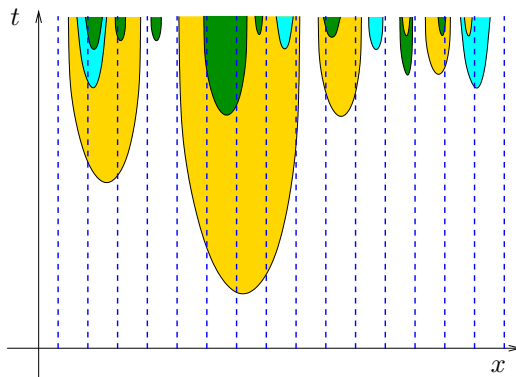
Fig. 6.4 Weighting prescriptions for models of tunneling type. Shaded regions are bubbles of different types. Dashed vertical lines represent randomly chosen comoving geodesics used to define a finite subset of bubbles.
