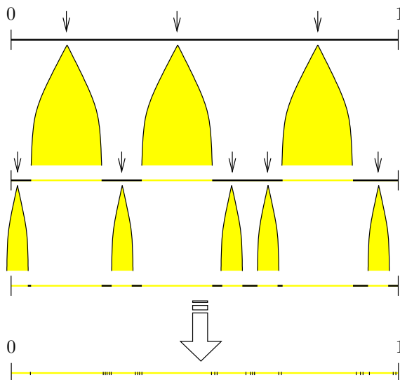
Fig. 4.2 Construction of a random Cantor set. Portions of the comoving segment [0, 1] are removed due to the appearance of reheated regions (yellow cones). At later times, the comoving size of removed regions shrinks. The set of points that remain after infinite time has measure zero and a fractal structure.
