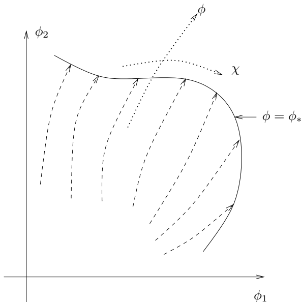
Fig. 2.2 Reheating boundary in field space (solid line) in a fiducial model with two fields \phi_1, \phi_2 . The slow-roll trajectories (dashed lines) approach the reheating boundary, which is a one-dimensional manifold in field space. In the coordinates (\phi, \chi) the reheating boundary is \phi = \text{const} , and different reheating possibilities have different values of \chi .
