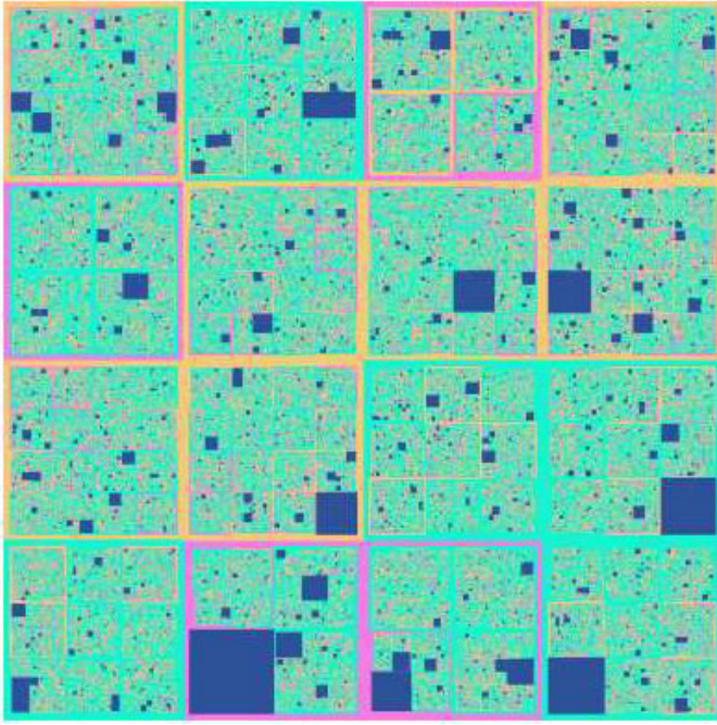
Fig. 9.1 An example simulation of “eternal inflation in a box” in two spatial dimensions. Bubbles ( H -regions) are represented in comoving coordinates by squares. Dark shades indicate bubbles of terminal types. Other shades correspond to nested bubbles of various nonterminal (“recyclable”) types. For the purposes of visual illustration, nucleation rates were chosen of order one, and colored lines were drawn at bubble boundaries.
