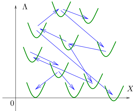
Fig. 5.1 A schematic representation of the “landscape of string theory,” consisting of a large number of local minima of an effective potential. The variable X collectively denotes various fields and \Lambda is the effective cosmological constant. Arrows show possible tunneling transitions between vacua.
