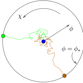
Fig. 6.3 A random walk in field space for a two-field inflationary model considered in [Vanchurin et al. (2000)]. The center of the field space is a diffusion-dominated regime. The reheating condition, \phi = \phi_* , selects a compact and connected region (a circle) in field space, which is the exit boundary for the random walk. The problem is to determine the volume-weighted probability distribution for the values of \chi at reheating.
