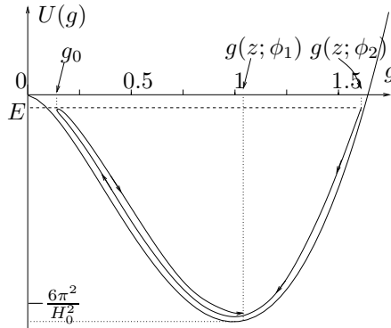
Fig. 8.1 Potential U(g) given by Eq. (8.112) can be used to interpret solutions g(z; \phi) as mechanical motion in “time” \phi at constant total energy E . The potential vanishes at g = 0 and g = e^{1/2} and has a minimum at g = 1 . The value g_0 is the turning point where U(g_0) = E . A trajectory corresponding to z < 0 will begin and end with g > 1 , i.e. to the right of the minimum of the potential. Solutions cease to exist when z < z_* ; the solution g(z_*; \phi) , shown by the thin line with arrows, corresponds to a trajectory that starts at rest (as demonstrated in the text). The energy of this trajectory is E \approx 0 , and so the value g(z_*; \phi_2) is close to e^{1/2} while g(z_*; \phi_1) is close to 1.
