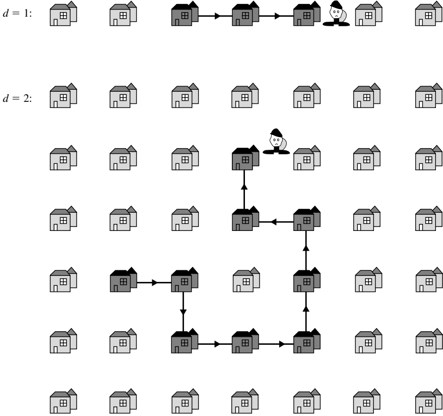
Fig. 7.10 A burglar's self-avoiding walk in one and two dimensions.
