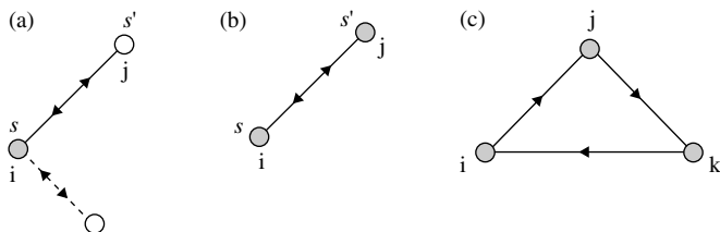
Fig. 6.5 Master equation: (a) summation over all final and initial (b) detailed balance, and (c) steady state.
