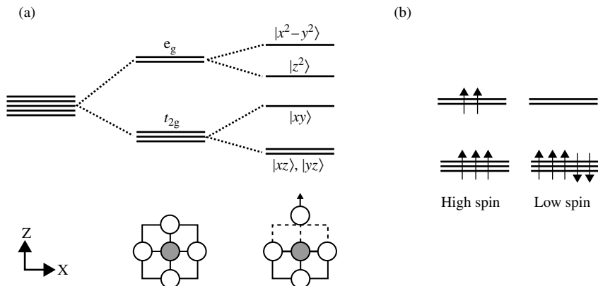
Fig. 3.7 Crystal-field splitting: (a) e_g - t_{2g} splitting in an octahedral environment (center) and splitting in a tetragonal field (right) and (b) high-spin low-spin transition for \text{Mn}^{2+} in an octahedral field.
