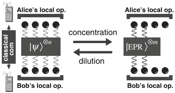
Fig. 7.4 Entanglement concentration and dilution
