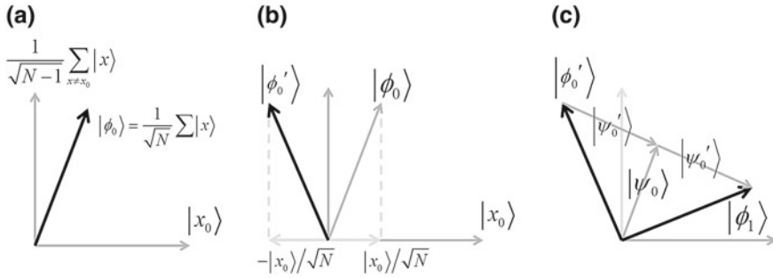
Fig. 4.1 a Step (i). b Step (iii). c Step (iv)
