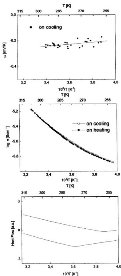
Figure 8. Electrical and thermal properties of manganese spinel (series A) as a function of temperature: a) thermoelectric power, b) electrical conductivity, c) DSC
