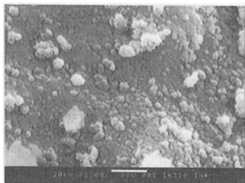
Figure 12: SEM micrograph of 7 mole% Li-doped BPO 4 . Bar indicates 1 \mu m.
