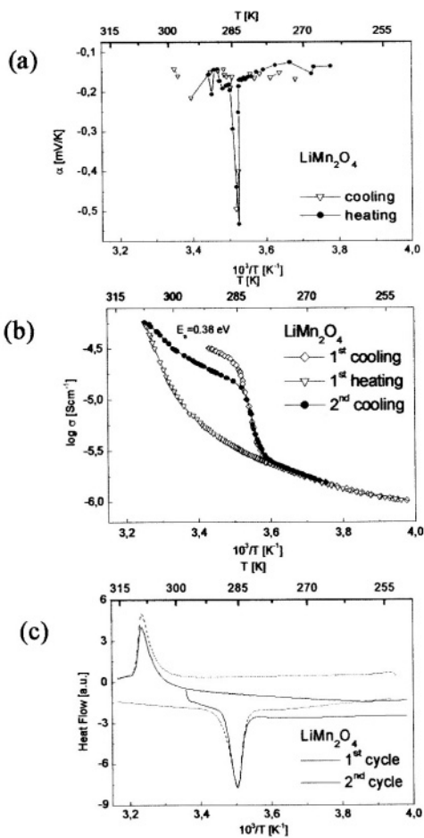
Figure 9. Electrical and thermal properties of LiMn 2 O 4 (B series) as a function of temperature: a) thermoelectric power, b) electrical conductivity, c) DSC
