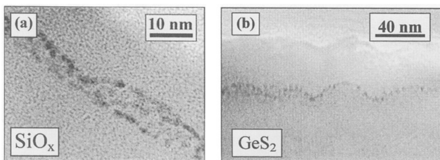
Figure 2. Cross-section view of as-deposited three-layer structures at low magnification: (a)-SiO x (40 nm)/CdSe(2 nm)/SiO x (20 nm) and (b)-GeS 2 (40 nm)/CdSe(2 nm)/GeS 2 (20 nm). CdSe particles, which are not disposed in a plane are revealed in both systems. Their spatial distribution follows the surface morphology of the SiO x and GeS 2 films, respectively.
