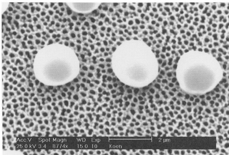
Figure 6. \text{SnO}_2 particles made via the EHDA route.
