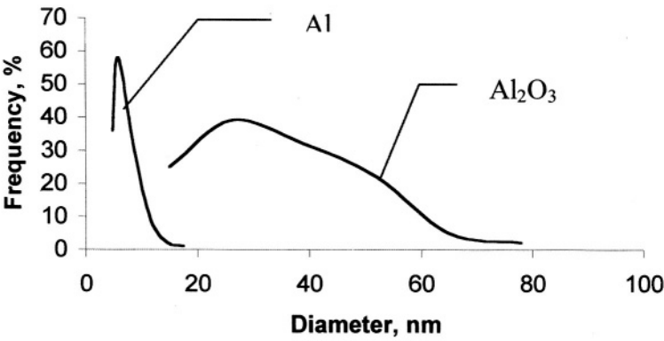
Figure 11. Morphology of Al(Al 2 O 3 )/Polymer nanocomposite (Sample 6, Table 2): a) TEM (light field) of Al and Al 2 O 3 nanoparticles; b) Al and Al 2 O 3 particle size distribution.
