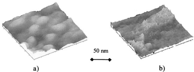
Figure 9. AFM image of a Sn-Polymer composite (Sample 4, 16Vol.%Sn). Scan size 140*140nm: a) surface morphology; b) the same area in phase contrast regime. Spreading of connected nanoparticle chains.
