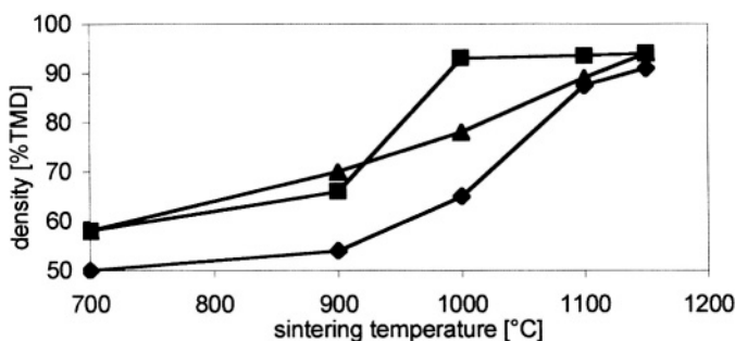
Figure 17: Sintering of green compacts of zirconia-hematite nano-nano composites compacted with different techniques. ◆=CIP at 400 MPa, ▲=CUP at 1000 MPa, ■=MPC at 1500 MPa [33].
