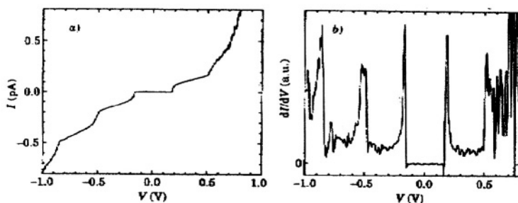
Figure 7: I(V) characteristics of a symmetric Au/Polymer/PcPd/Polymer/Au heterojunction measured at 4.2 K. (a) and the corresponding derivative (b)); PcPd is an octasubstituted metal-lophtalocyanine (from ref. [41]).
