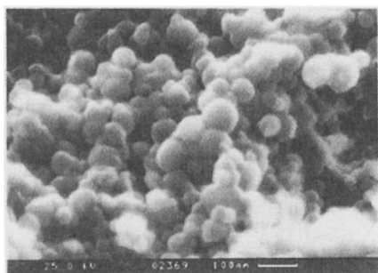
Figure 7: SEM micrograph of MPC n\text{-Al}_2\text{O}_3 [22] Bar=100 nm.
