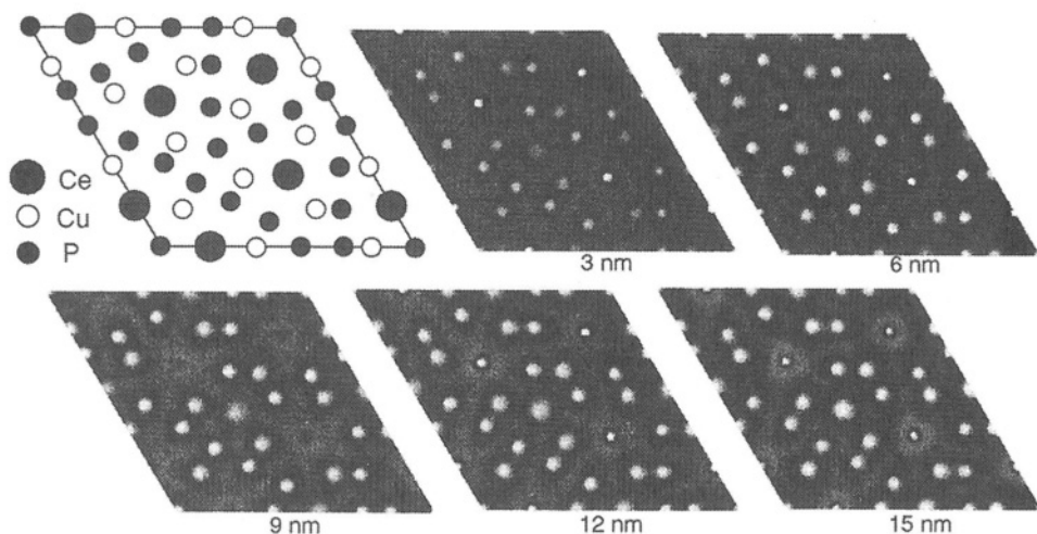
Figure 5. A structure model of \text{Ce}_5\text{Cu}_{12}\text{P}_9 , and 5 calculated exit waves (amplitude) for 5 different thicknesses and indicated below the images. The images are one unit cell large and correspond to the structure mode. Note that the Ce atoms (the strongest scattering atoms) are most dominant in the very thin exit wave but for instance almost absent in the exit wave of 9 nm thickness.
