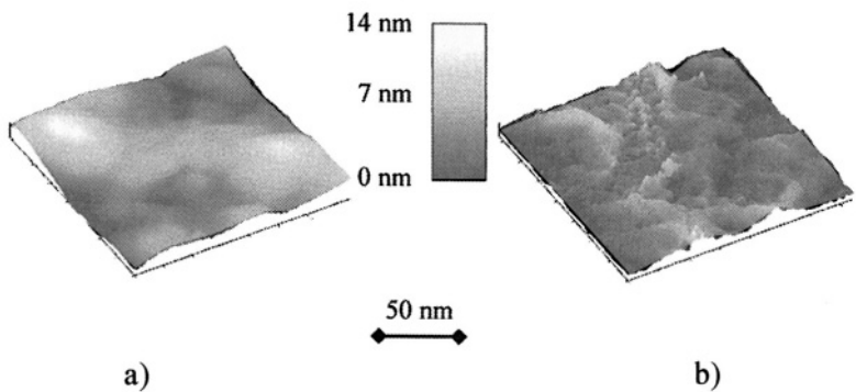
Figure 8. AFM image of a Sn-Polymer composite (Sample 3, 12Vol.%Sn). Scan size 140*140nm: a) surface morphology; b) the same area in phase contrast. Nanoparticles aggregate connecting into continuous chains.
