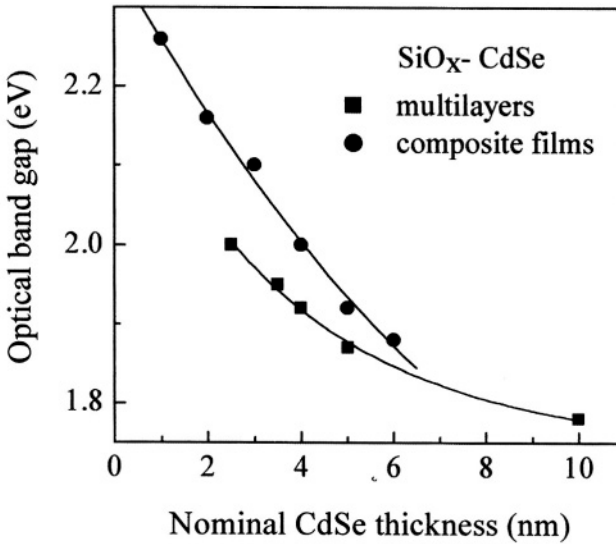
Figure 3. Thickness dependencies of the optical absorption gap E_g^o of CdSe nanocrystalline layers in \text{SiO}_x -CdSe multilayer structures. The lines are guides to the eye. The E_g^o values of the composite films correspond to quasi three-dimensional carrier confinement, while the E_g^o values of the multilayers correspond to one-dimensional confinement.
