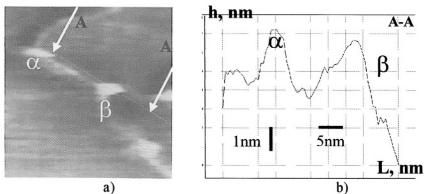
Figure 5 . a) Phase-contrast AFM image of the composite. Dark regions are polymer spherulites and light spots are Pd nano-particles situated on the boundary between polymer spherulites. b) Cross-section A-A. Profile maximums correspond to Pd particles embedded into the boundary surface between the polymer spherulites.
