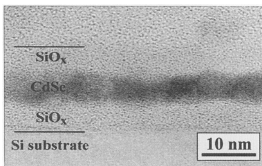
Figure 1. Cross-section view of a SiO x (5.8 nm)/CdSe(4.5 nm)/SiO x (5.8 nm) structure. The micrograph shows a continuous nanocrystalline CdSe layer sandwiched between two amorphous SiO x layers. The CdSe nanocrystallite size along the ML axes is equal to the CdSe layer thickness.
