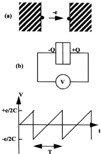
Figure 3: a) Metal - Insulator - Metal tunneling junction; b) Its equivalent diagram and c) the potential for a constant current I ( =e/T ) as a function of time.
