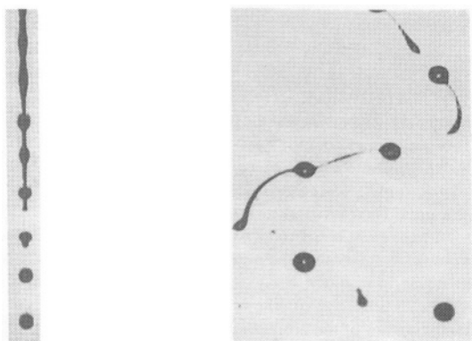
Figure 4. Break up of the jet at low (left) and high (right) stress ratios.
