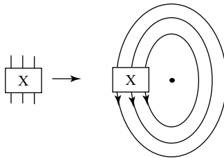
Fig. 3. The operation of closing a braid X to form a closed braid.
