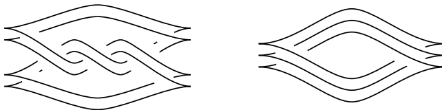
Fig. 49. A 2-copy of the right handed trefoil (left) and a 3-copy of the unknot (right).
