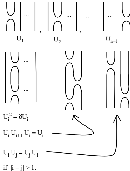
Fig. 48. Relations in the Temperley–Lieb monoid.
