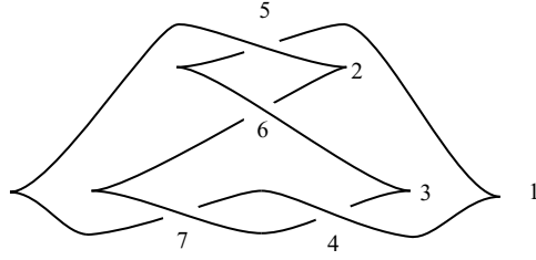
Fig. 37. The front projection of the Legendrian figure eight knot with tb = -3 .
