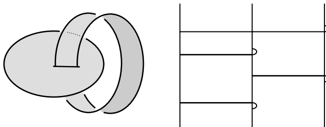
Fig. 24. A quasipositive fibered link which is not strongly quasipositive.
