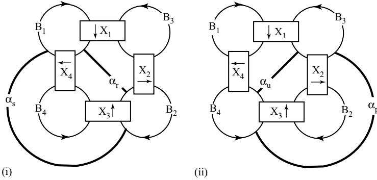
Fig. 11. (i) The diagram corresponding to the irreducible peak \{Y(r), \hat{Y}, Y(s)\} . (ii) Two additional reducing arcs used to eliminate irreducible peaks. Each pair \alpha_r, \alpha_s and \alpha_p, \alpha_u is a possible non-commuting pair associated to the peak. The blocks X_1, X_2, X_3, X_4 indicate (possibly empty) collections of signed arcs.
