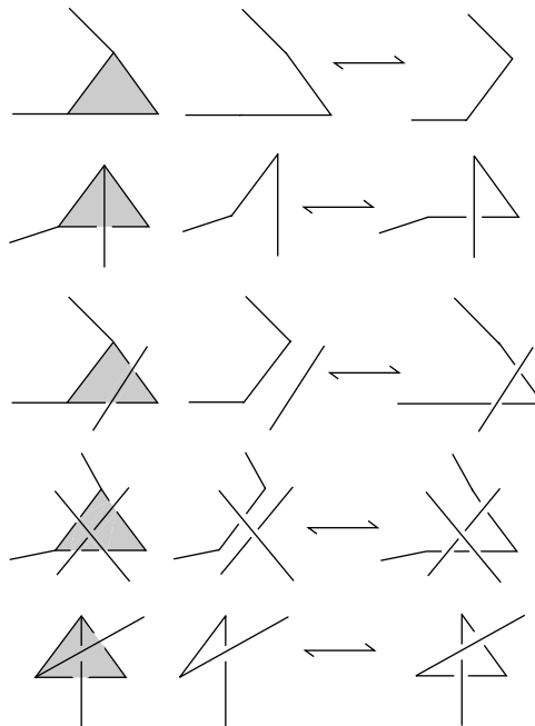
Fig. 9. Projections of triangle moves.
