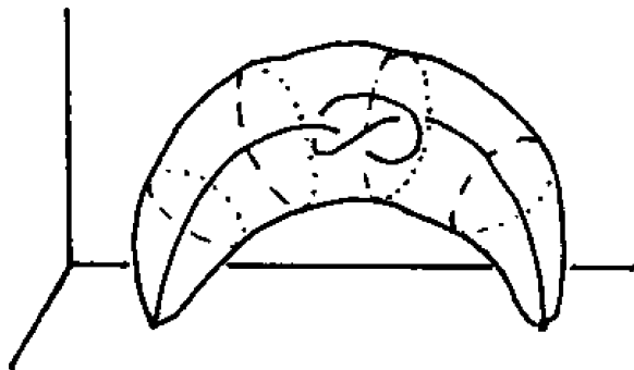
Fig. 10. We rotate a ball around the knotted arc.
