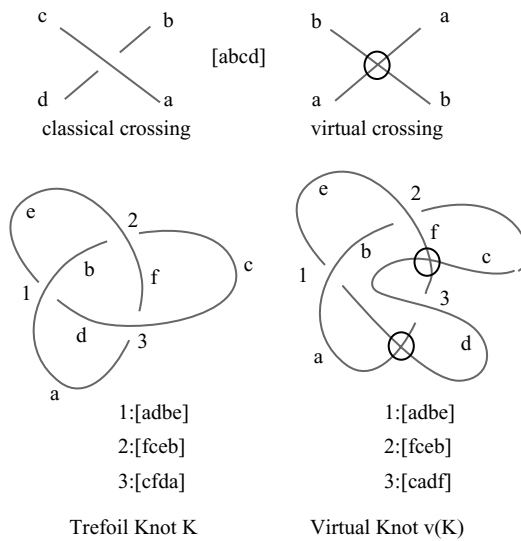
Fig. 63. Coding a link diagram.
