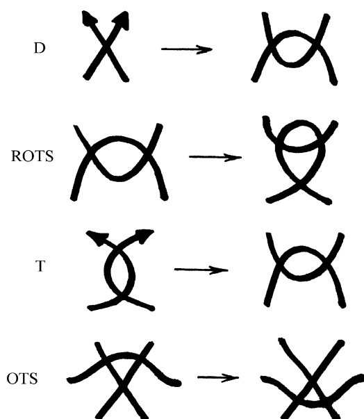
Fig. 8. The D, ROTS, T, and OTS operators.
