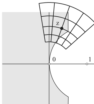
Fig. 18. Do not let \text{Re}(\log z) or \text{Im}(\log z) change by more than 1/2 during a single iteration of Newton's method. Our choice of coordinates (in Region A, B or C) guarantees that the parameter z lies in the shaded region relative to the chosen coordinates, away from the singularity at z = 1 or \log z = 0 . More precisely, all points in the shaded region satisfy |\text{Im}(\log z)| \geq \pi/3 > 1 , so the restriction |\Delta \text{Im}(\log z)| \leq 1/2 keeps z safely away from the singularity at z = 1 . Similarly the restriction |\Delta \text{Re}(\log z)| \leq 1/2 keeps the solution from approaching the singularities at z = 0 or z = \infty too quickly.
