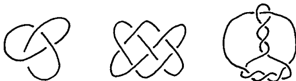
Fig. 1. Some smooth knots S^1 \subset \mathbb{R}^3 . A smooth knot can always be given a PL structure by employing a suitable triangulation of \mathbb{R}^3 that contains the knot as a subcomplex.
