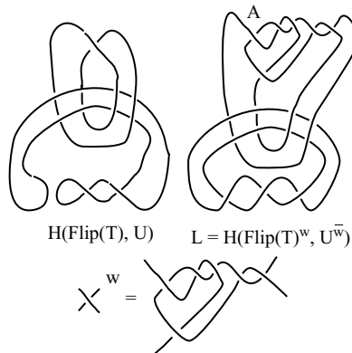
Fig. 68. Applying omega operations to an unlink with flipped crossing.
