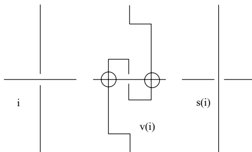
Fig. 55. Switching and virtualizing a crossing.
