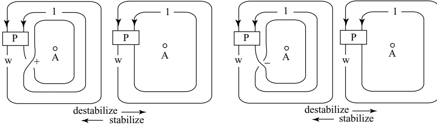
Fig. 7. The destabilization and stabilization moves.
