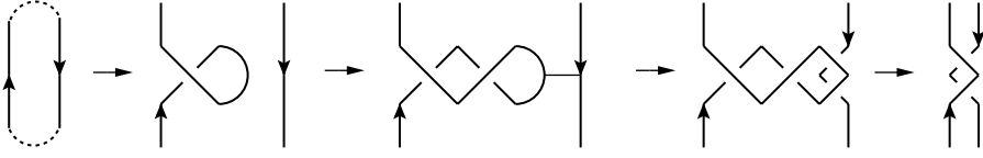
Fig. 9. Replacing moves of type \text{II}^{\text{nb}} .
