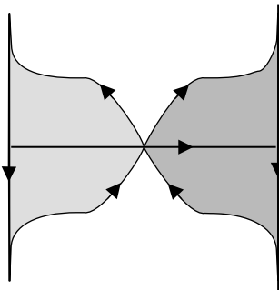
Fig. 2. The standard bowtie and associated arcs.
