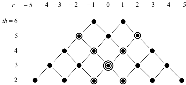
Fig. 47. Classification of Legendrian (2,3) -cables of (2,3) -torus knots. Concentric circles indicate multiplicities, i.e., the number of distinct isotopy classes with a given r and tb .
