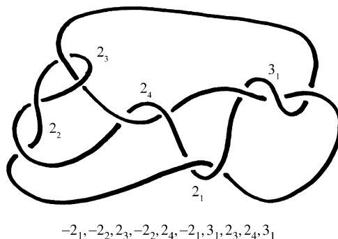
Fig. 9. A diagram with k -group encoding.
