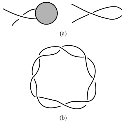
Fig. 1. Unreduced diagrams and a 2-braid.
