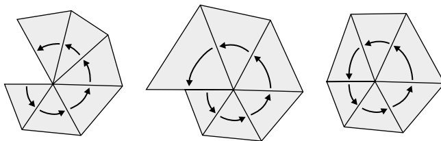
Fig. 16. Look at a cusp cross section to see how the dihedral angles meet near an edge. In a failed attempt at a hyperbolic ideal triangulation (left) the real dihedral angles do not sum to 2\pi . In a second failed attempt (center) the problem is more subtle: the real dihedral angles sum to 2\pi but the complex dihedral angles do not multiply to 1 (the sum of their arguments is correct but the product of their moduli is not). In a valid hyperbolic ideal triangulation (right) the product of the complex dihedral angles is 1.
