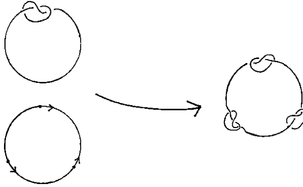
Fig. 9. The trefoil knot spun about the manifold M consisting of three disjoint points in S^1 . Note that the framing at each point (indicated by an arrow that depicts the orientation of the framing) determines how to attach the knot.
