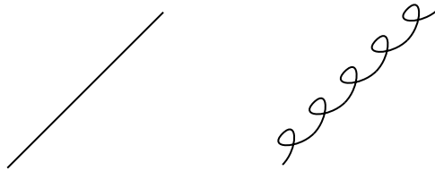
Fig. 11. Using the Lagrangian projection to approximate topological arcs.
