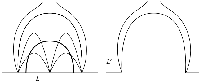
Fig. 22. Characteristic foliation associated to a boundary parallel dividing curve (left). The destabilization L' of L (right).
