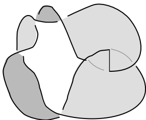
Fig. 5. A clasp surface in \mathbb{R}^3 .
