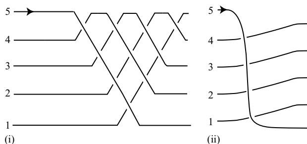
Fig. 24. (i) The 5-braid \Delta_5 . (ii) The 5-braid \delta_5 .
