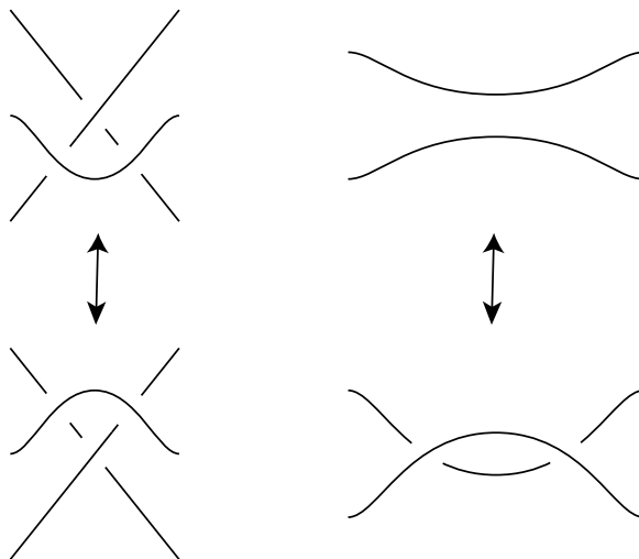
Fig. 12. Legendrian Reidemeister moves in the Lagrangian projection. (Also need the corresponding figures rotated 180^\circ about all three coordinate axes.)
