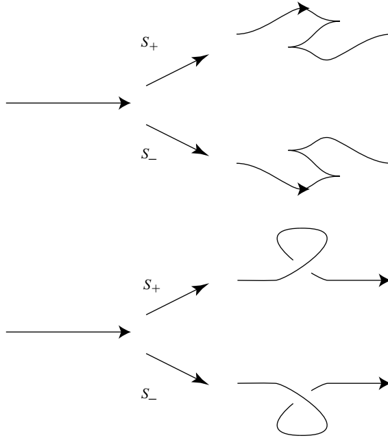
Fig. 19. Stabilizations in the front projection (top) and the Lagrangian projection (bottom).
