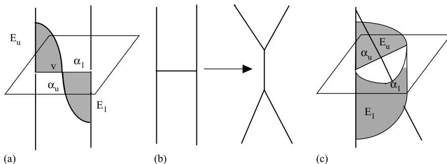
Fig. 12. A level cycle in the graph appears.
