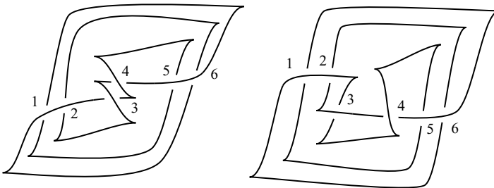
Fig. 41. Legendrian projections of the two “Chekanov knots” from Figure 29. L is on the left and L' is on the right.
