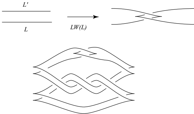
Fig. 57. The change to L \cup L' used to make LW(L) . Legendrian Whitehead double of the trefoil (bottom).
