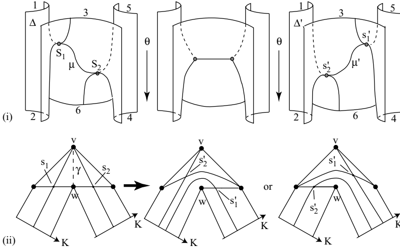
Fig. 18. Sketch (i) shows an isotopy of \mathcal{D} that induces a change in foliation. Sketch (ii) shows the effect of the change on two ab -tiles.
