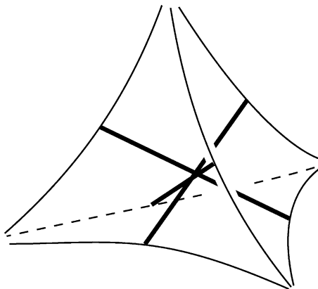
Fig. 12. Every ideal tetrahedron has three mutually perpendicular symmetry axes. To construct a symmetry axis, pick a pair of opposite edges and find the shortest geodesic \gamma connecting them. Because \gamma is the shortest path between those two edges, it must meet both the edges at right angles. A half-turn about \gamma therefore preserves each edge setwise while interchanging its endpoints-at-infinity. In other words, a half-turn about \gamma permutes the tetrahedron's ideal vertices and thus defines a symmetry of the tetrahedron. Elementary symmetry considerations then imply that the three symmetry axes – corresponding to the tetrahedron's three pairs of opposite edges – must meet orthogonally at the tetrahedron's center.
