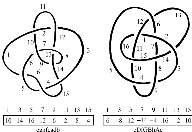
Fig. 3. DT sequences for knot diagrams.
