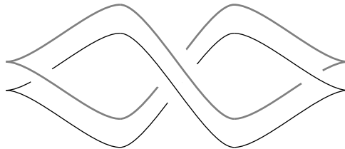
Fig. 16. Knots L (black) and L' (grey) used to compute tb(L) .
