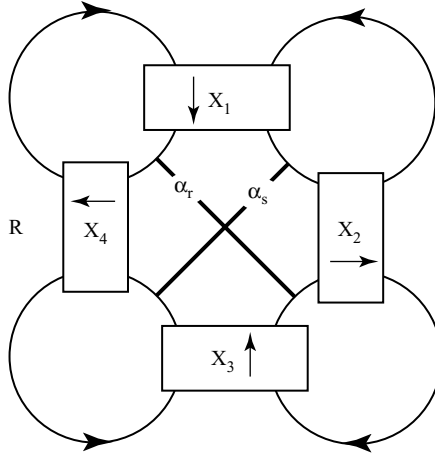
Fig. 10. The case where two reducing arcs at a peak intersect once.
