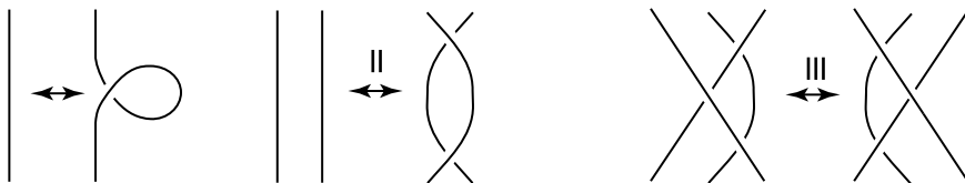
Fig. 6. The three Reidemeister moves. The 1, 2 or 3 strands in the left sketch of each have arbitrary orientations, also we give only one of the possible choices for the signs of the crossings, for each move.
