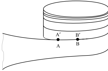
Fig. 6. Physical realization of a cut-open cusp whose edges are identified with a shift (Figure 5 bottom). The strip wraps around like a cylinder, approaching a limiting circle.
