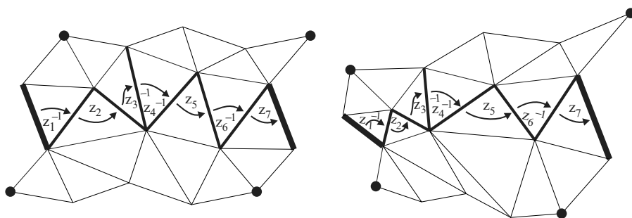
Fig. 17. The cross section of each cusp is a torus whose fundamental domain – viewed in the universal cover – is combinatorially a quadrilateral. In the special case that the quadrilateral is effectively a parallelogram (left) the covering transformations are pure translations. In the general case, by contrast, the quadrilateral is arbitrary (right) and the covering transformations are similarities, not isometries, of the Euclidean plane. Algebraically, the rotational–dilatational part of a covering transformation may be computed as a product of complex dihedral angles; the product will be exactly 1 if and only if the covering transformation is a pure translation.
