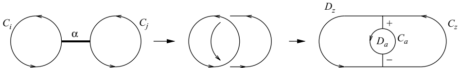
Fig. 5. The local picture of a reducing move.
