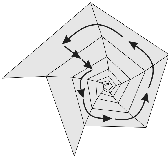
Fig. 22. View the solid cylinder of Figure 21 from above and note the path of a meridian encircling the missing central geodesic. That meridian defines the Dehn filling curve, so expressing it relative to the original (meridian, longitude) coordinates of the knot or link complement immediately gives the Dehn filling coefficients, in this case (2, 5) .
