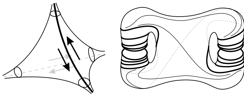
Fig. 7. For each 0-sphere (pair of points) in an n -component 2-dimensional link, shear along an edge connecting the two cusps belonging to that 0-sphere. Locally the result is as in Figure 6. Globally the result is a closed hyperbolic surface of genus n with n geodesic circles missing.
