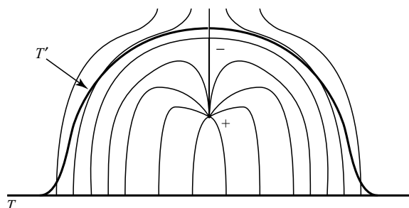
Fig. 21. Using the characteristic foliation to recognize a destabilization.
