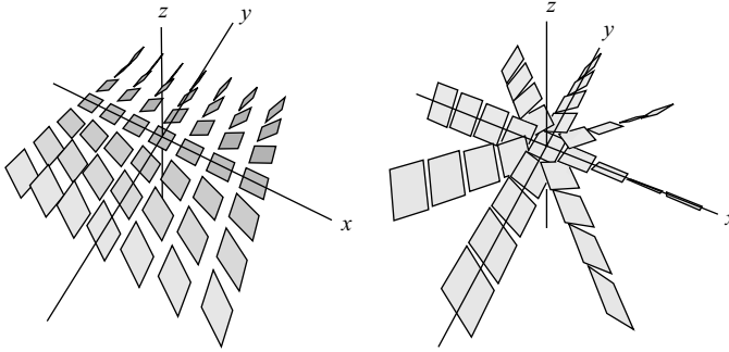
Fig. 1. The contact structure \xi_{\text{std}} (left) and \xi_{\text{sym}} (right) on \mathbb{R}^3 . (Figures courtesy of S. Schönenberger.)
