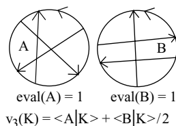
Fig. 31. Oriented chord diagrams for v_3 .
