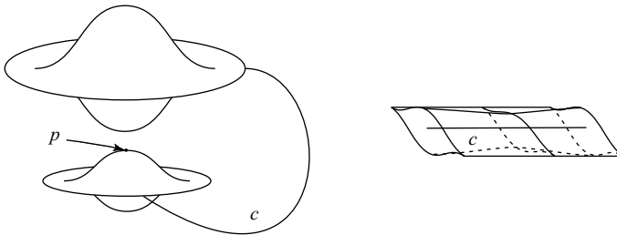
Fig. 54. The Legendrian knot L (left). To form L_k a neighborhood of the arc c should be replaced with the tube shown on the right.
