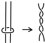
Fig. 5. Twisting by surgery.
