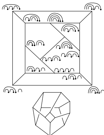
Fig. 52. The Stasheff polyhedron.
