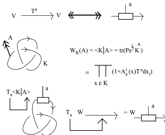
Fig. 26. Wilson loop insertion.
