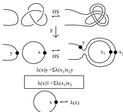
Fig. 47. Handle sliding and right integral.
