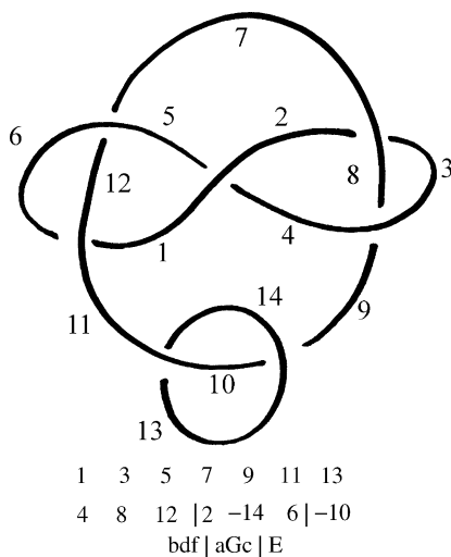
Fig. 4. A DT sequence for a link diagram.
