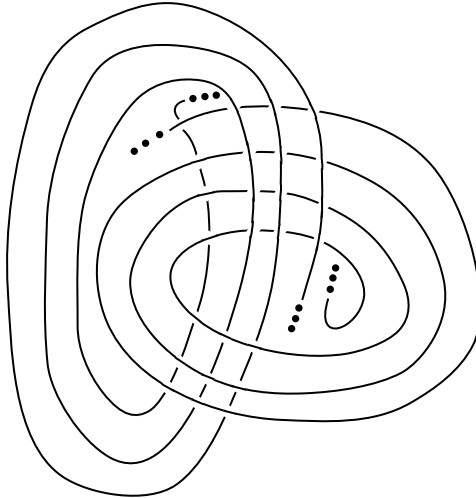
Fig. 8. These knots have meridian length approaching 4 from below.
