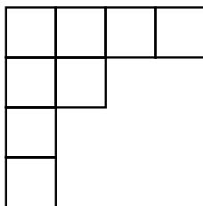
Fig. 22. The Young diagram corresponding to the partition 4 + 2 + 1 + 1 .
