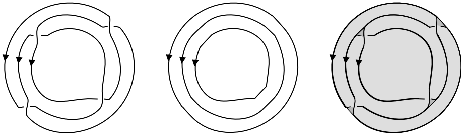
Fig. 12. Seifert's construction applied to a nested diagram.
