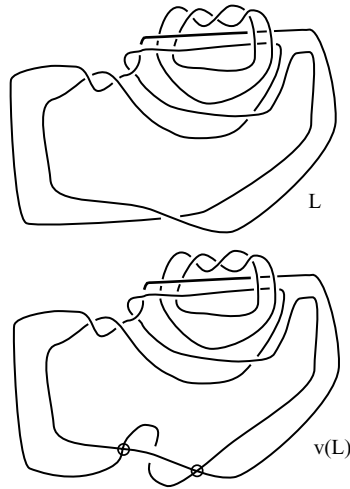
Fig. 71. The virtual link v(L) .
