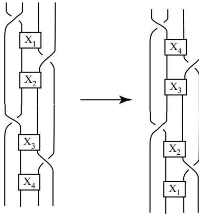
Fig. 12. Two braids whose respective closures are the result of performing the two pairs of reducing moves r, p and s, u indicated in Figure 11.
