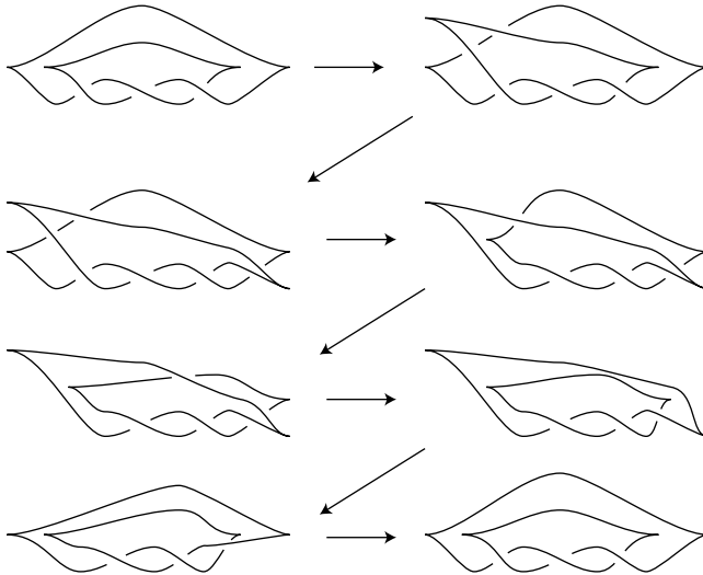
Fig. 50. A loop of Legendrian trefoils.
