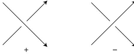
Fig. 17. Right handed crossing (on left) and a left handed crossing (on right). Note this figure is to indicate that right (left) crossings contribute + ( - ) to the writhe of a knot. The picture on the right cannot occur in a front projection, but non the less left handed crossings can.
