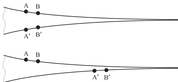
Fig. 5. A sliced open cusp. Glue the edges straight across (top) and the cusp is complete. Glue the edges with a shift (bottom) and the result is incomplete.
