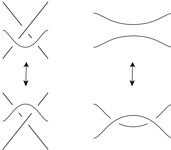
Fig. 14. Transverse Reidemeister moves. Add arrows in all ways that do not violate the conditions in Figure 13. (Also need the corresponding figures rotated 180^\circ about all three coordinate axes.)
