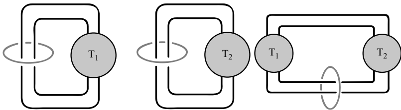
Fig. 4. The belted sum of two links.
