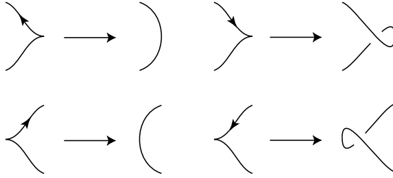
Fig. 24. Positive transverse push-off in the front projection.
