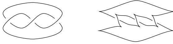
Fig. 5. Converting a knot diagram (left) into a Legendrian front (right).
