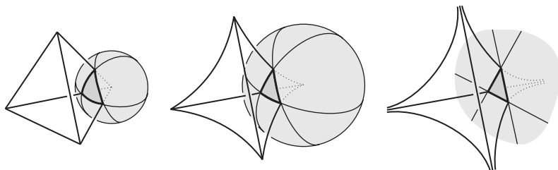
Fig. 13. In an ordinary tetrahedron (left) the cross section near a vertex – defined to be the intersection of the tetrahedron with a sphere centered at the vertex itself – is a spherical triangle. If we move the vertices outward (center), while keeping the cross section close to the tetrahedron's center, then the radius of the sphere must increase, making the cross section flatter. In the limit as the vertices go to infinity (right) the cross section becomes completely flat. Such a limiting sphere is called a horosphere and is in fact a 2-dimensional Euclidean plane sitting in 3-dimensional hyperbolic space. Even though it is intrinsically flat, the horosphere remains extrinsically convex to compensate for the ambient negative curvature of hyperbolic 3-space.
