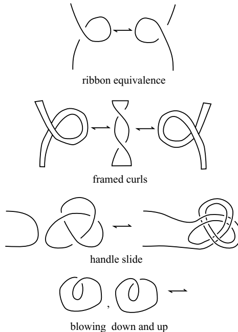
Fig. 42. Framing and Kirby calculus.
