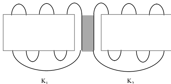
Fig. 4. Adding knots and bridge numbers.
