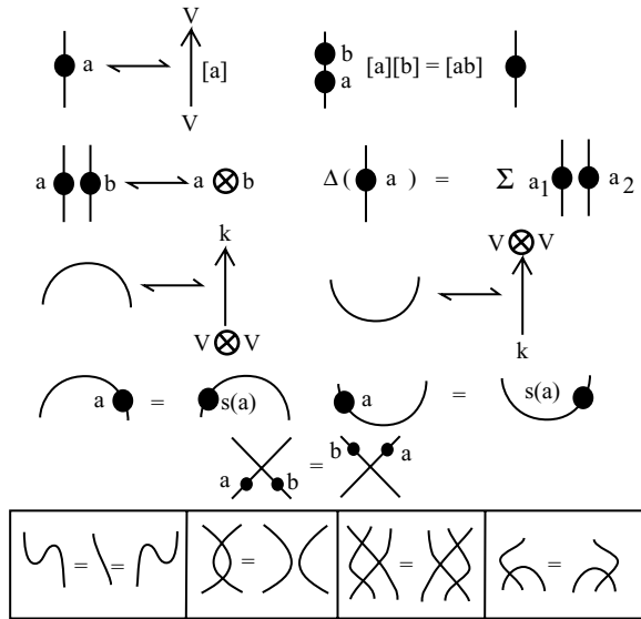
Fig. 44. Morphisms in \text{Cat}(A) .
