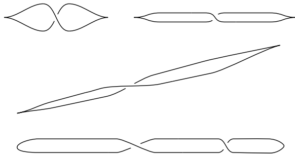
Fig. 34. Top left: the front projection of a Legendrian unknot. Top right: the stretched projection. Middle: the tilted projection that is easy to convert into the Lagrangian projection (bottom).
