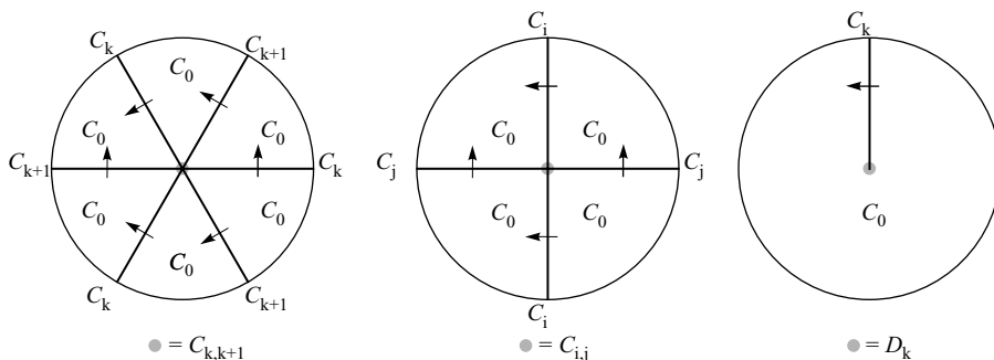
Fig. 14. The transverse structure of MP_n/\equiv_{\mathbb{R}} along its codimension-2 cells.
