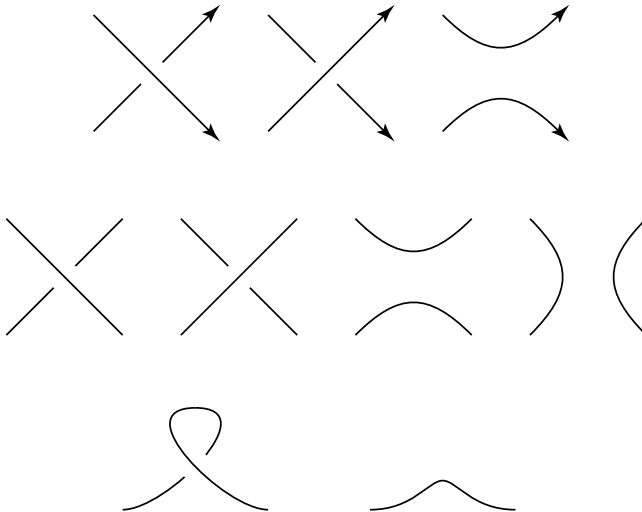
Fig. 25. The relation between K_+, K_-, K_0 (top), K_+, K_-, K_0 K_\infty (middle) and K_r, K (bottom).
