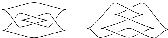
Fig. 10. Two fronts of the same Legendrian figure eight knot.
