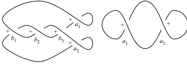
Fig. 28. The Lagrangian projection of a Legendrian trefoil and unknot. One corner of each crossings has been labeled with a + to help determine the signs of all the quadrants near the crossing.
