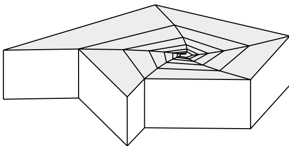
Fig. 21. Slice the cusp of Figure 20 into pieces along the illustrated cross sections and then re-glue the resulting pieces according to the identifications on their left, right, front and back sides. The result resembles a solid cylinder, with ever smaller pieces spiraling in towards the center.
