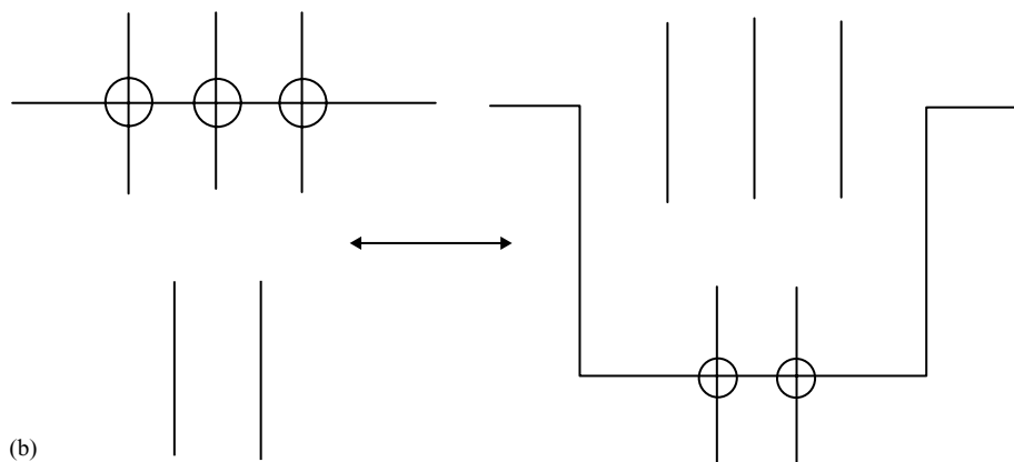
Fig. 53. (a) Generalized Reidemeister moves for virtuals. (b) Detour move.
