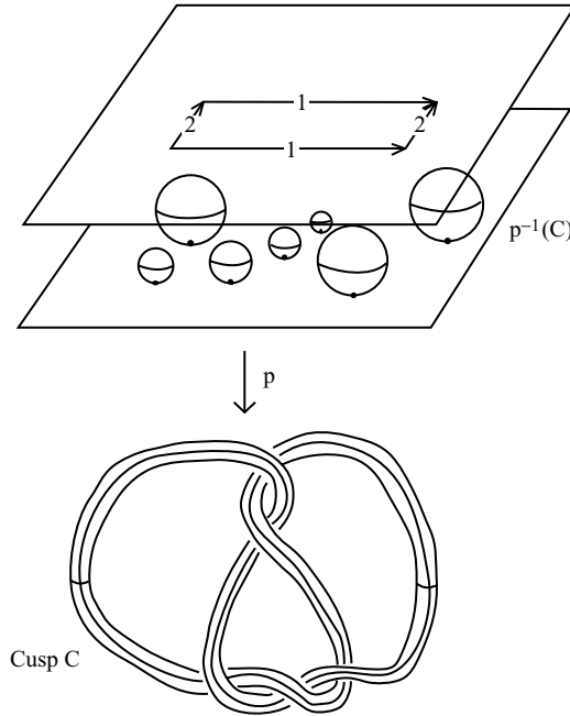
Fig. 7. The cusp of a knot.
