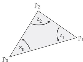
Fig. 15. Any one of the three complex dihedral angles z_0 , z_1 and z_2 determines the other two. Proof: Position the cusp cross section arbitrarily in the complex plane and let its vertices be the complex numbers p_0 , p_1 and p_2 . The definition of the complex dihedral angle (recall Figure 14) implies z_0 = (p_2 - p_0)/(p_1 - p_0) , z_1 = (p_0 - p_1)/(p_2 - p_1) = 1/(1 - z_0) and z_2 = (p_1 - p_2)/(p_0 - p_2) = 1/(1 - z_1) = 1 - (1/z_0) .
