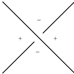
Fig. 27. Quadrants near a crossing in \pi(L) .
