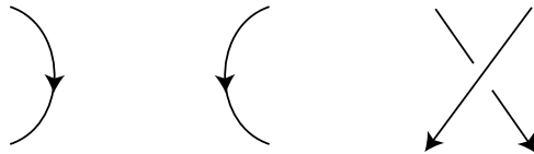
Fig. 13. Segments excluded from projections of transverse knots.
