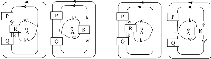
The two flype templates
