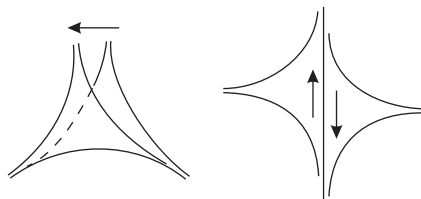
Fig. 4. Ideal triangles are rigid; any two are congruent. Proof: Given any two ideal triangles, move one so that one of its edges coincides with the corresponding edge of the other, and then slide it along until the third vertex coincides as well (left panel). The gluing between ideal triangles is flexible – two neighboring triangles may slide along each other like the two sides of the San Andreas fault (right panel).
