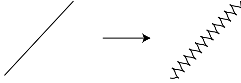
Fig. 7. C^0 approximating an arc by a Legendrian arc.
