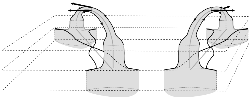
Fig. 10. Attaching \eta_x(h^{(1)}) to \cup_{o \in o_{D(L)}} o (left, positive; right, negative).
