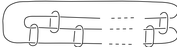
Fig. 6. Two-bridge knots come from surgery on these links.
