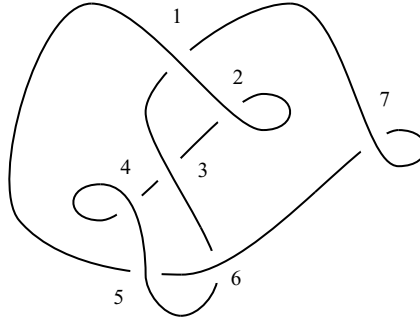
Fig. 32. The Legendrian knots L .
