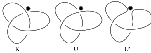
Fig. 60. Trefoil and two relatives.
