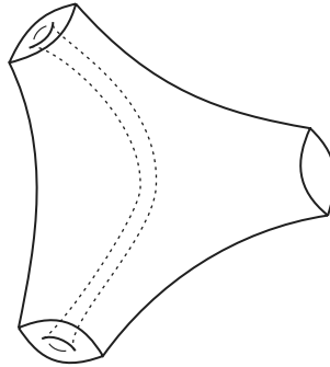
Fig. 11. A triangular pillow with a pre-drilled tube running through it provides a tunnel joining two of its truncated vertices.
