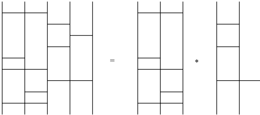
Fig. 17. An example of deplumbing.
