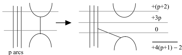
Fig. 10. A useful slide that, sadly, raises width.
