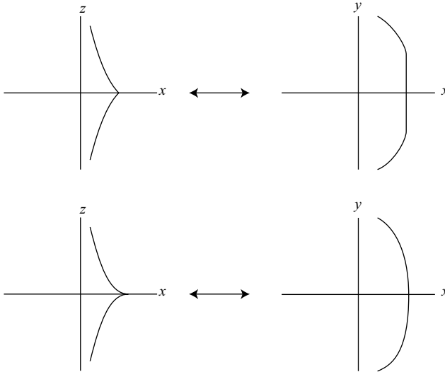
Fig. 3. Top row shows two projections of a Legendrian arc with x'(\theta) = 0 on an open interval. Bottom row shows a near by Legendrian arc with x'(\theta) = 0 only at one point.
