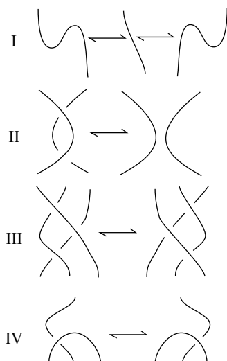
Fig. 36. Regular isotopy with respect to a vertical direction.
