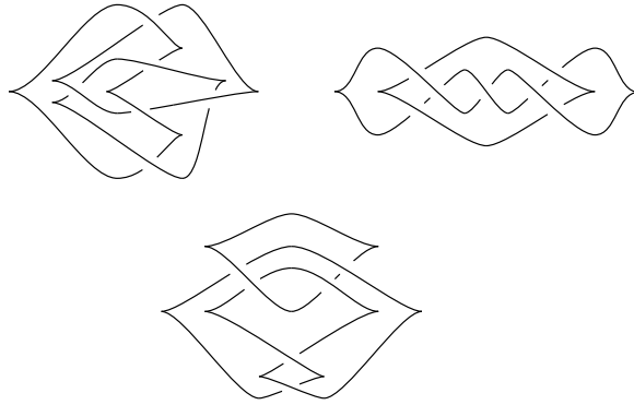
Fig. 48. Legendrian Borromean rings with tb = -4 (top left), Legendrian Whitehead link with tb = -5 (top right) and Legendrian Whitehead mirror realized by two tb = -1 unknots (bottom).
