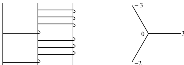
Fig. 25. Two representations of a quasipositive Lover's Knot.
