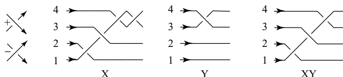
Fig. 1. Examples of 4-braids X , Y and their product XY .
