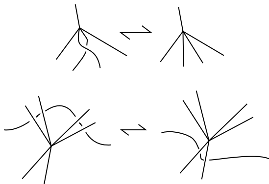
Fig. 13. Extra moves for topological isotopy of graphs.
