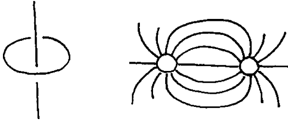
Fig. 3. The decomposition of S^3 (thought of as \mathbb{R}^3 plus a “point at infinity”) into two solid tori S^1 \times B^2 and B^2 \times S^1 . The left-hand picture shows the circular cores of the tori (the vertical line becomes a circle as it wraps through the point at infinity). The right-hand picture shows a slice along the y - z plane: the two disks are a slice of one solid torus (cut a donut in half and then view it on end), while the arcs represent slices of the meridional disks of the other solid torus.
