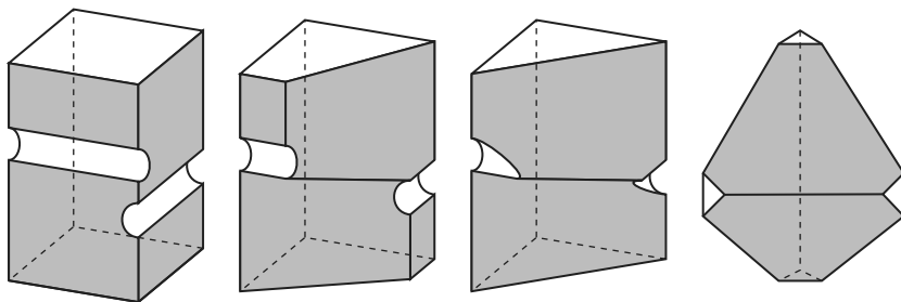
Fig. 10. The pieces in the decomposition of Figure 9 are all identical. Each has a square truncated vertex touching the upper surface of S^2 \times I , another square truncated vertex touching the lower surface of S^2 \times I , and two hemi-cylindrical truncated vertices running along the boundary of the (excised) tubular neighborhood of the link (far left panel). In addition, each piece has six regular faces: two squares and four hexagons. Deforming the two square faces to become narrow rectangles does not change the topology (center left panel). Collapsing those two narrow rectangles to become lines (center right panel) yields a polyhedron that is combinatorially a truncated tetrahedron (far right panel), with four truncated vertices (all triangles) and six faces (all hexagons).
