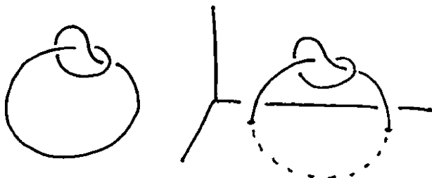
Fig. 6. Turning a knotted circle into a knotted arc in the upper half-space in order to spin it about the plane.
