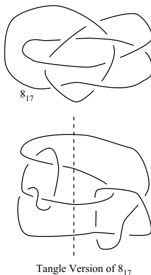
Fig. 32. Tangle decomposition of 8_{17} .
