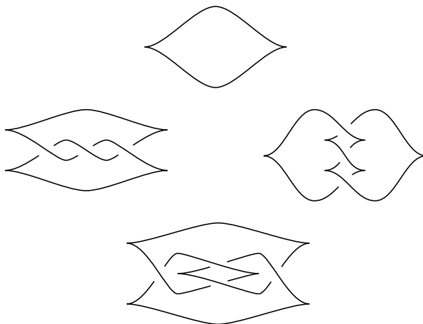
Fig. 4. Legendrian knots realizing the unknot, right and left trefoil knots and the figure eight knot.
