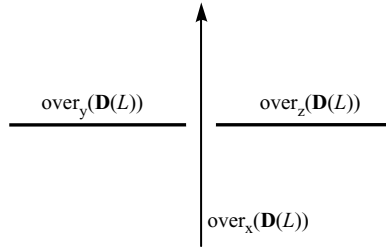
Fig. 8. Labeled over-arcs (the unlabelled crossing need not be \mathbf{x} ).
