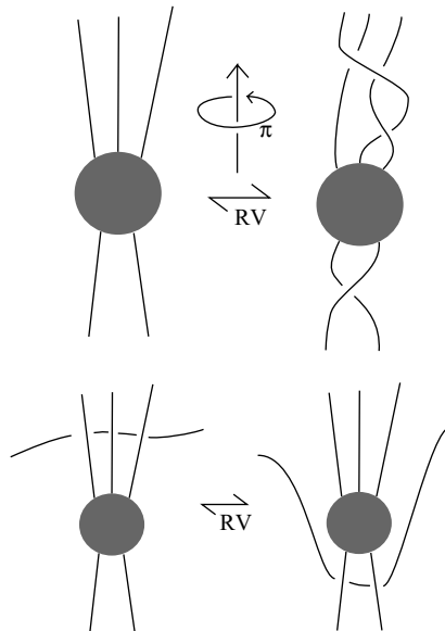
Fig. 15. Diagrammatic rigid vertex isotopy.
