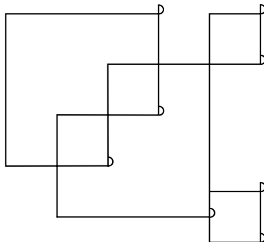
Fig. 22. A fence diagram for the plumbed Seifert surface of \mathcal{D}(O\{2,3\}; 0; +) .
