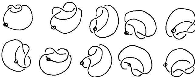
Fig. 13. Rolling the trefoil. The small circle in these figures represents B_- . Rather than moving B_- , it is more illustrative to hold it fixed and roll the knot around it! In fact, this roll of the trefoil is twisted with respect to the unlinked longitude. Furthermore, due to the symmetries of a torus knot, the rolling part of the deformation has no effect, only the twisting. Can you see why? Nonetheless, this diagram illustrates the idea of the procedure.
