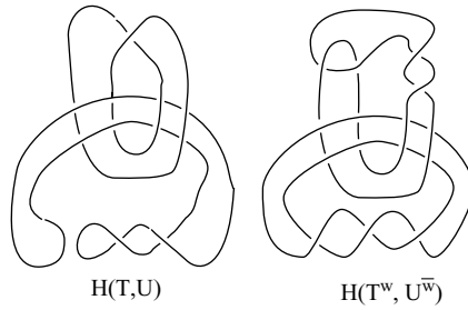
Fig. 67. Applying omega operations to an unlink.
