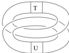
Fig. 65. Hopf link satellite H(T, U) .
