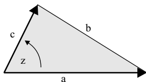
Fig. 14. Consider more carefully the horospherical cross section (defined in Figure 13) of the cusp of an ideal tetrahedron. The cross section is a Euclidean triangle whose three angles are simply the (real) dihedral angles of the tetrahedron. It turns out to be more convenient to replace each real dihedral angle \theta with a complex dihedral angle z whose argument \arg z is the real dihedral angle \theta and whose modulus |z| is the ratio of the lengths of the adjacent sides (in the example shown, |z| = c/a ). In other words, z is the complex number that rotates one side of the triangle counterclockwise to an adjacent side, as viewed from the cusp.
