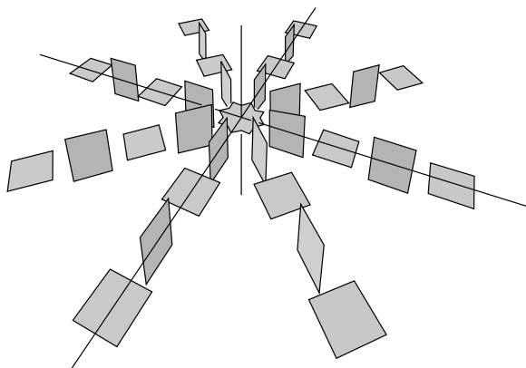
Fig. 2. The contact structure \xi_{\text{ot}} on \mathbb{R}^3 . (Figures courtesy of S. Schönenberger.)
