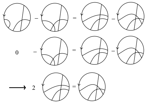
Fig. 19. Four-term relation for type three invariant.
