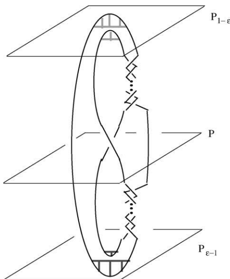
Fig. 1. Level planes for a 2-bridge knot.
