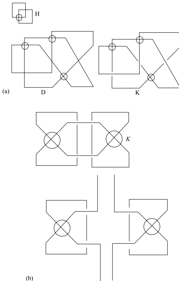
Fig. 54. (a) Flats H and D , and the knot K . (b) Kishino and parts.
