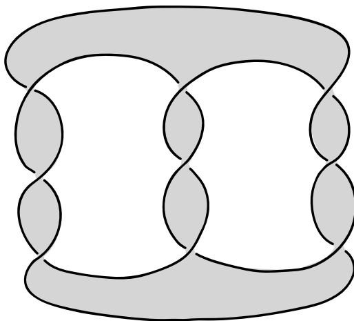
Fig. 9. A (3,3,3) -pretzel knot has a totally geodesic Seifert surface.
