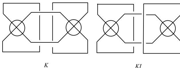
Fig. 58. The knot K and the Kishino diagram KI .
