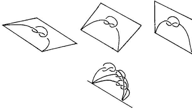
Fig. 7. A schematic of knot spinning.
