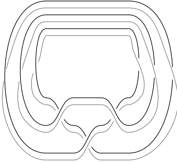
Fig. 18. The braid T in black and its push-off by v in grey.
