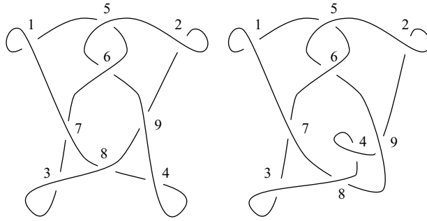
Fig. 29. The knot L (left) and L' (right).
