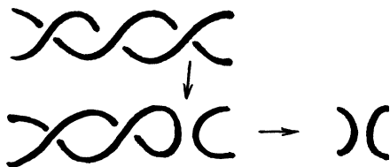
Fig. 6. Smoothing and reducing.
