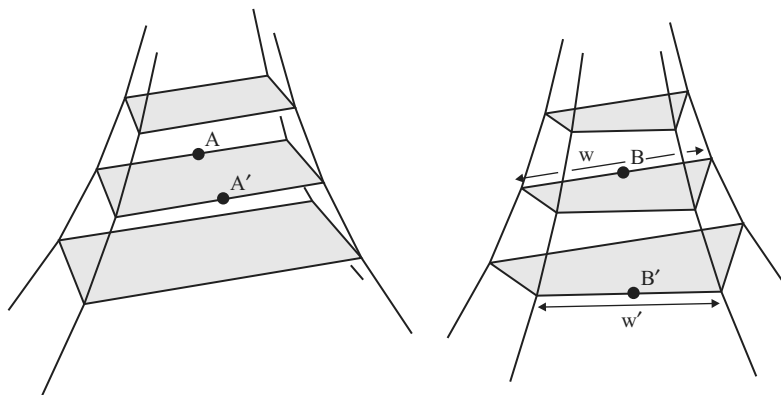
Fig. 19. A cut-open 3-dimensional cusp looks like an infinitely tall Eiffel tower. The cross sections are all quadrilaterals, which are similar to one another and whose size shrinks exponentially fast as you travel upward, in strong analogy to the cut-open 2-dimensional cusps of Fig. 5 whose cross sections are line segments shrinking exponentially fast. The cusp on the left has a parallelogram cross section (cf. Figure 17 left), while the cusp on right has a generic cross section (cf. Figure 17 right).
