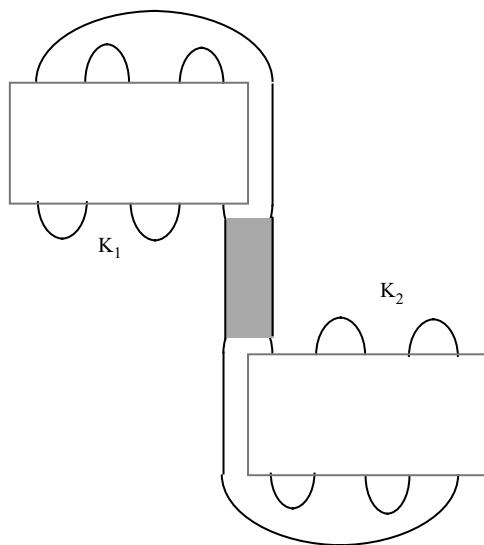
Fig. 5. Adding knots and knot width.
