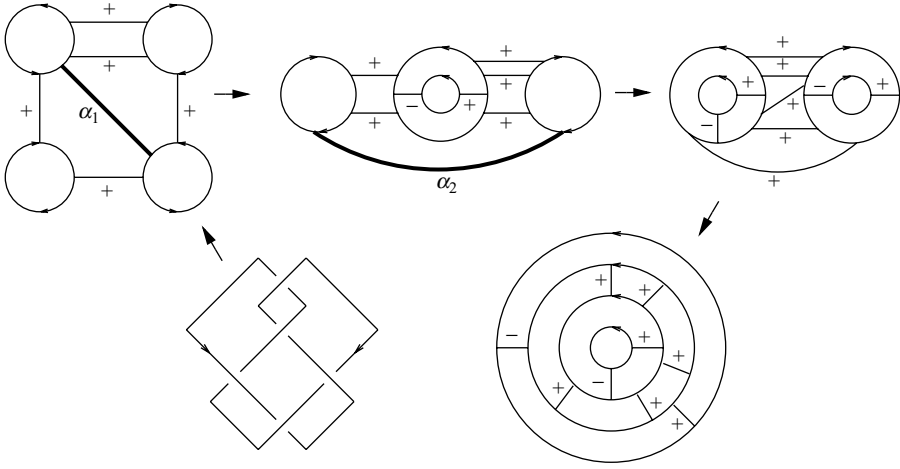
Fig. 4. The Yamada–Vogel algorithm performed on the knot 5_2 .
