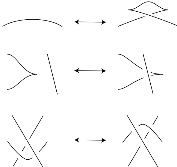
Fig. 8. Legendrian Reidemeister moves. (Also need the corresponding figures rotated 180^\circ about all three coordinate axes.)
