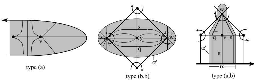
Fig. 17. A vertex v of type (a) , (a, b) and (b, b) .
