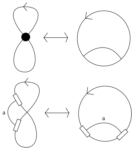
Fig. 24. Weight system and Casimir insertion.
