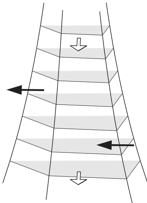
Fig. 20. In this example a traveller going to the left and returning from the right (black arrow) drops down two levels, while a traveller going towards the front and returning from the back (white arrow) goes up five levels. Because the offsets are rational multiples of each other ( 5/2 or 2/5 ) the cross-sectional quadrilaterals piece together to form a consistent surface. If the offsets were not rational multiples of each other, no such consistent set of equally spaced cross sections would be possible.
