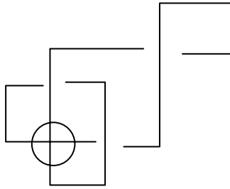
Fig. 59. A counterexample to the Poincaré conjecture for virtual three-manifolds.
