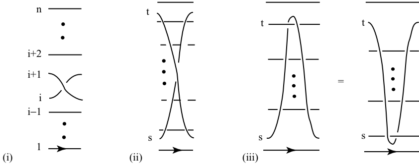
Fig. 2. (i) The elementary braid \sigma_i . (ii) The elementary braid \sigma_{s,t} . (iii) The pure braid A_{s,t} = A_{t,s} = \sigma_{s,t}^2 .
