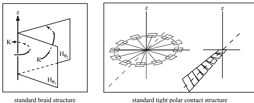
Fig. 21. The standard braid structure and tight contact structure on \mathbb{R}^3 .
