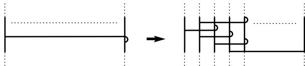
Fig. 19. “Trefoil insertion” on a fence diagram preserves the Seifert form while eliminating a negative band.
