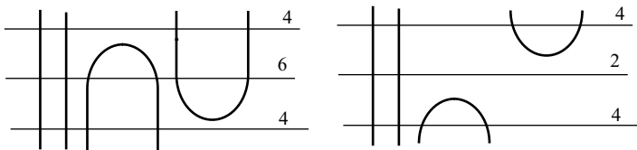
Fig. 3. Maximum and minimum exchanging places.
