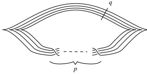
Fig. 43. Positive (p, q) -torus knot.
