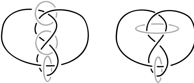
Fig. 3. Two augmented alternating links from the figure-eight knot.
