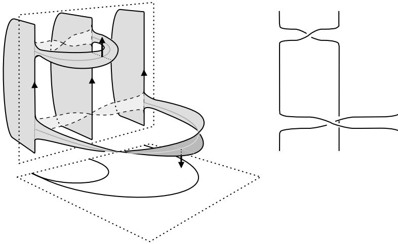
Fig. 15. Left: a surface \Sigma(b) ; \varepsilon(b(l)) = - , \varepsilon(b(l)) = + . Right: a braid diagram for \beta(b) .
