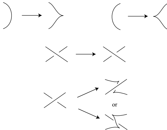
Fig. 6. Realizing a knot type as a Legendrian knot.
