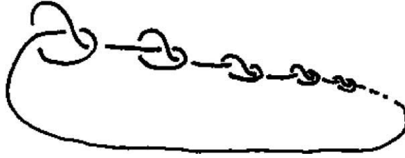
Fig. 2. A “wild” knot that is not locally flat at the point of infinite “knottedness”.
