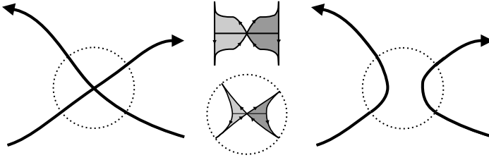
Fig. 3. Local smoothing, using a bowtie.
