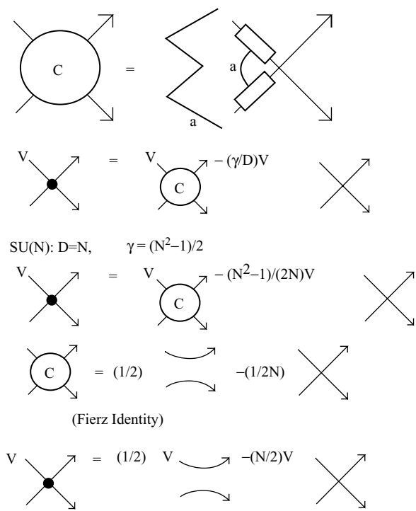
Fig. 25. Modified recursion formula.
