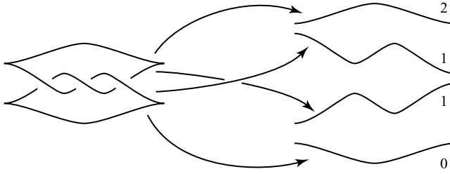
Fig. 38. The four strands associated (right) associated with the front (left). The numbers are a Maslov potential.
