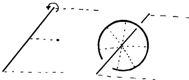
Fig. 5. Spinning a point in the half-plane around the axis.
