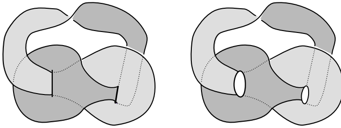
Fig. 6. A ribbon surface in \mathbb{R}^3 and its smoothing.
