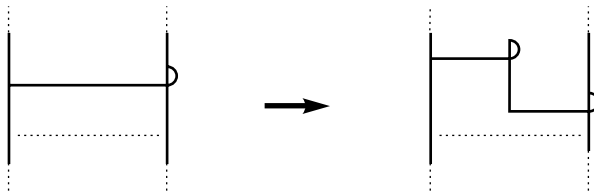
Fig. 21. “Twist reduction” on a fence diagram.
