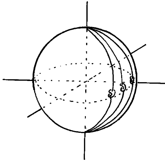
Fig. 8. A second schematic of knot spinning.
