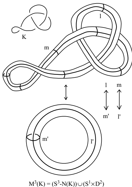
Fig. 43. Surgery on a blackboard framed link.
