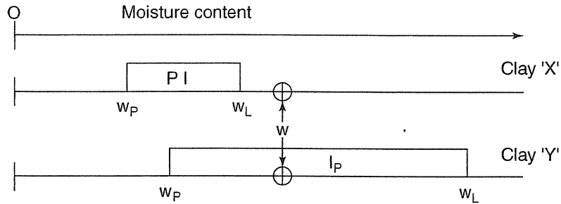
Figure 2.3 Consistencies of two clays
