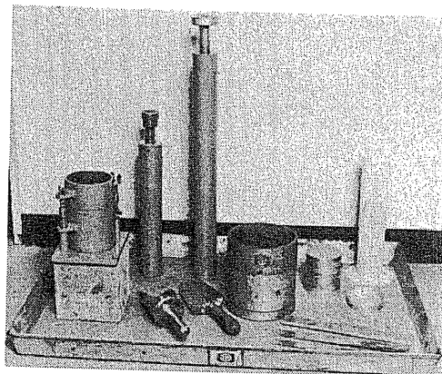
Figure 6.10 Equipment for compaction tests
