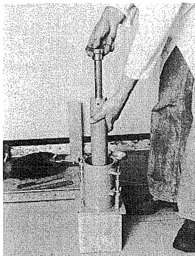
Figure 6.11 Compacting soil into mould
