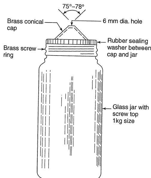
Figure 3.16 Pyknometer
