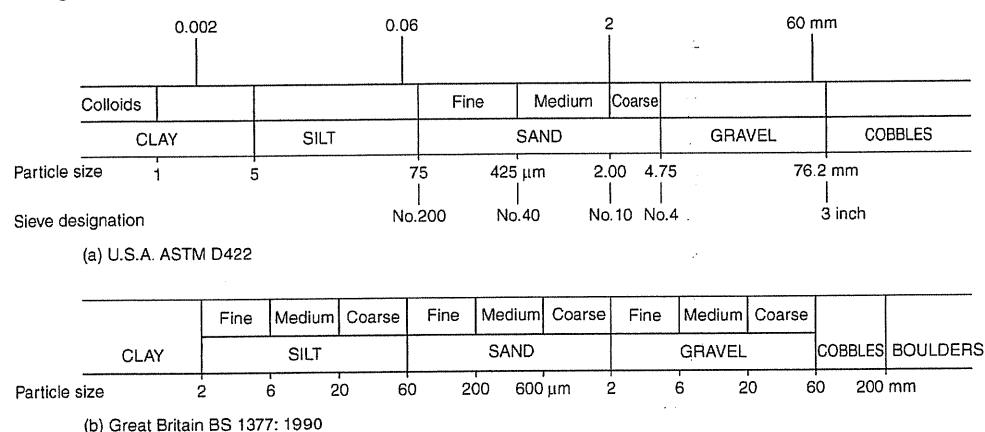
Figure 4.2 Comparison of systems for classifying particle size ranges of soils
