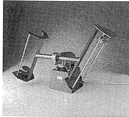
Figure 3.15 End-over-end gas jar shaker (photograph courtesy of ELE International)
