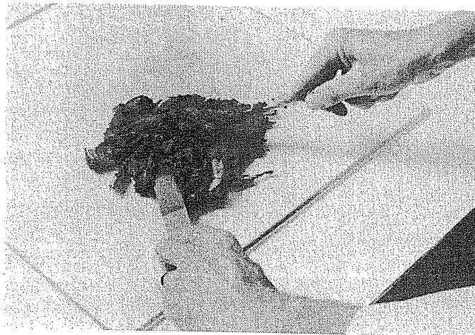
Figure 2.9 Mixing water into soil for liquid limit test
