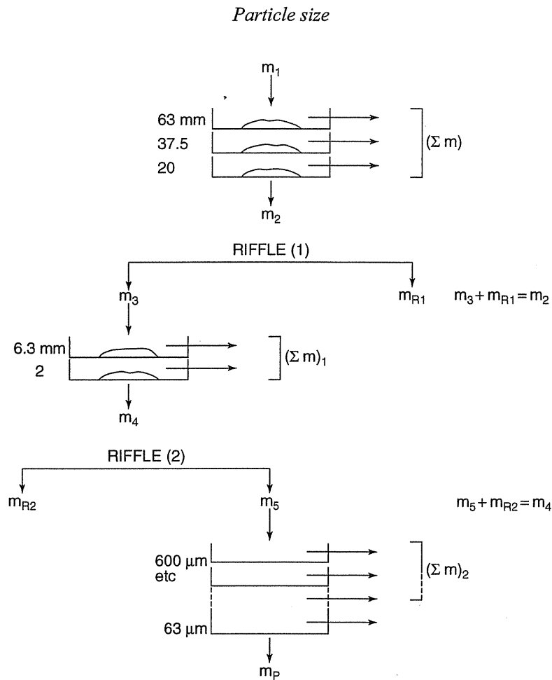
Figure 4.12 Sequence diagram, composite sieving
