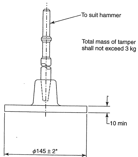
Figure 6.23 Tamper for vibrating hammer (courtesy of BSI, London)
