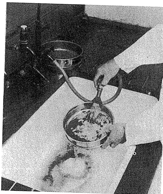
Figure 4.15 Washing soil on 63 \mu\text{m} sieve
