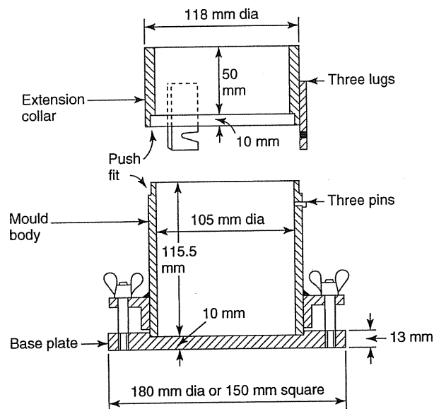
Figure 6.8 British Standard one-litre compaction mould
