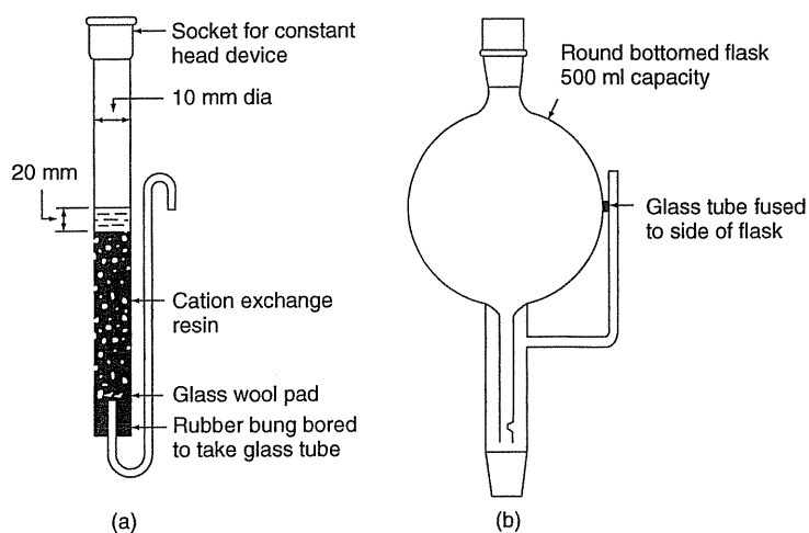
Figure 5.8 Ion-exchange column and constant-head apparatus
