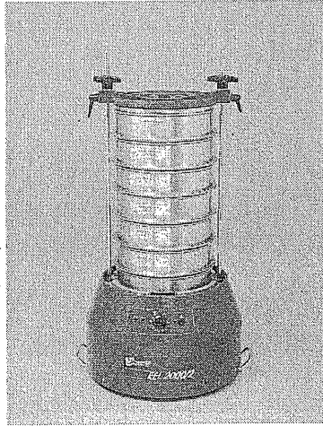
Figure 1.21 Sieve shaker (photograph courtesy of ELE International)
