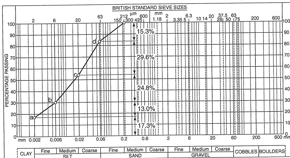
Figure 4.27 Particle size curve from pipette analysis
