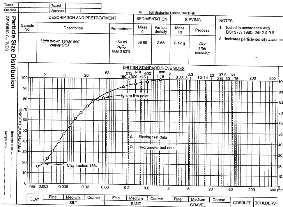
Figure 4.31 Particle size curve from hydrometer test and related sieving
