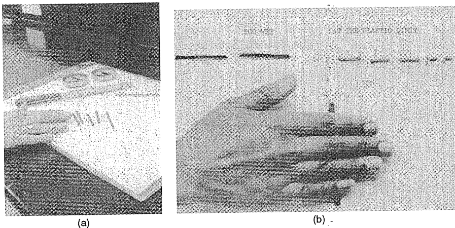
Figure 2.22 Plastic limit test: (a) apparatus, (b) soil thread before and after rolling (photograph courtesy of Geolabs)
