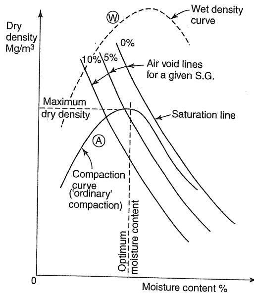
Figure 6.2 Dry density–moisture content relationship for soils
