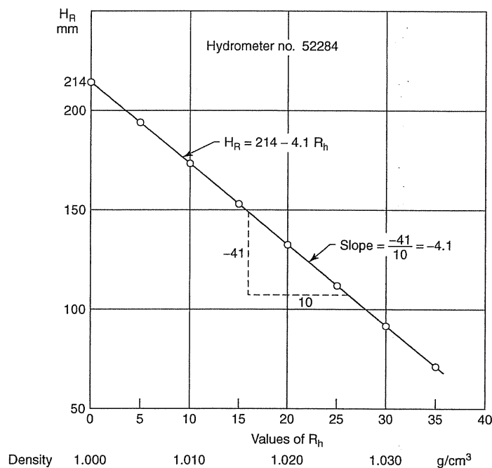
Figure 4.33 Hydrometer calibration curve
