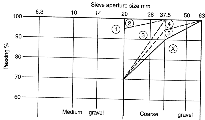
Figure 6.7 Summary of soil grading zones
