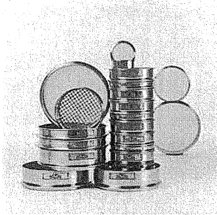
Figure 4.8 Test sieves (photograph courtesy of Impact Test Equipment)
