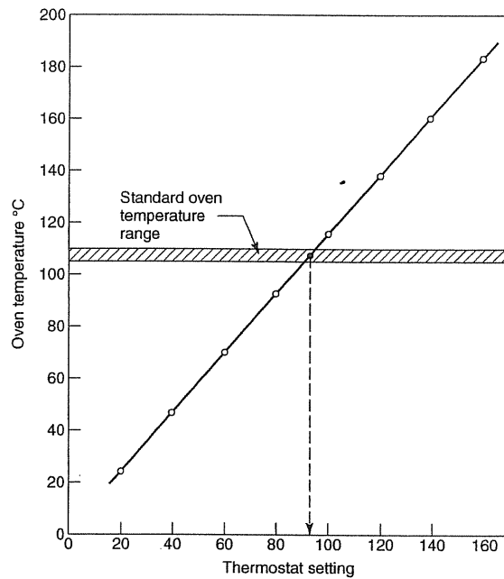
Figure 1.8 Typical calibration of a drying oven
