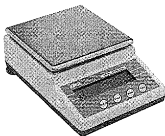
Figure 1.3 Electronic coarse top-pan balance, with a capacity of 30 kg and a resolution of 1 g (photograph courtesy of ELE International)
