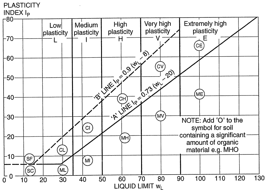
Figure 2.6 Plasticity chart
