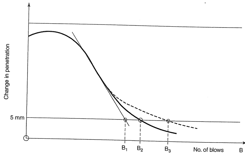
Figure 6.31 English and Scottish methods of interpretation of penetration curve from MCV test
