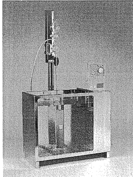
Figure 1.14 Constant-temperature bath with heater/thermostat/stirrer unit (photograph courtesy of ELE International)
