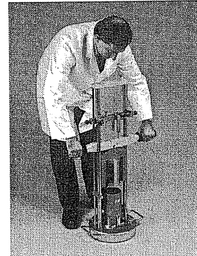
Figure 6.27 Apparatus for moisture condition test (photograph courtesy of ELE International)
