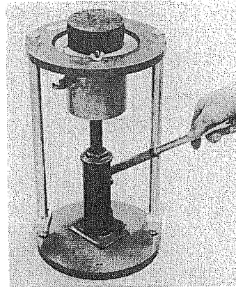
Figure 6.14 Jacking soil out of mould
