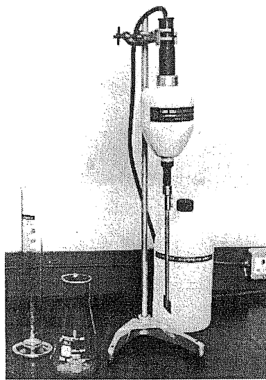
Figure 4.24 Vibro-stirrer
