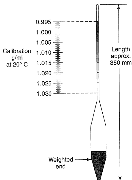
Figure 4.28 Soil hydrometer
