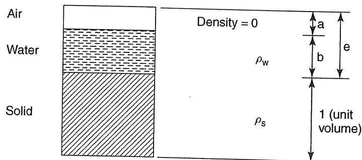
Figure 6.4 Representation of soil with air voids
