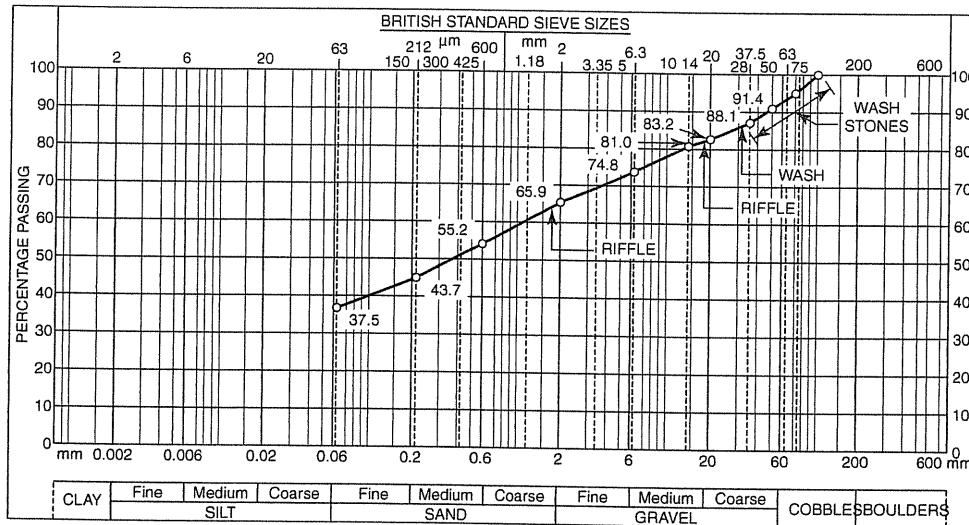
Figure 4.21 Grading curve from sieving test on 'boulder clay'.
