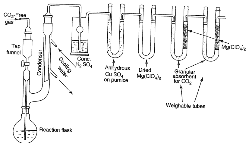
Figure 5.9 Arrangement of carbon dioxide absorption apparatus
