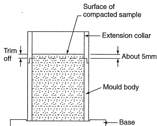
Figure 3.19 Soil in mould after compaction
