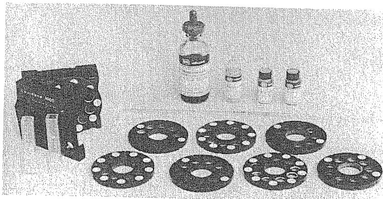
Figure 5.6 Lovibond Comparator for pH measurement
