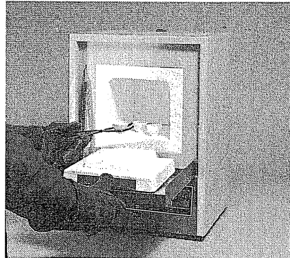
Figure 1.26 Muffle furnace (photograph courtesy of ELE International)
