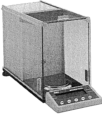
Figure 1.5 Analytical balance, with a capacity of 210 g and a resolution of 0.1 mg (photograph courtesy of ELE International)
