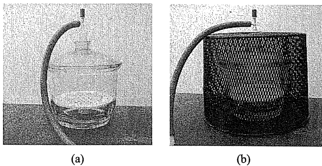
Figure 1.12 (a) Vacuum desiccator and (b) with protective cage (photograph courtesy of Cranfield University)
