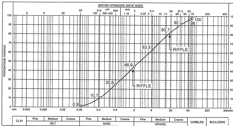
Figure 4.13 Grading curve, composite sieving
