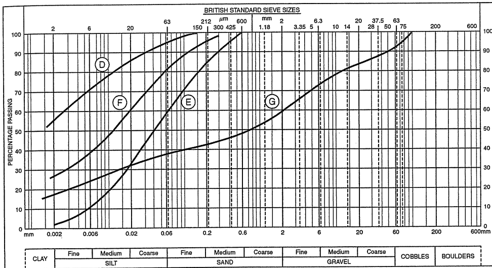
Figure 4.6 Particle size curves: silts and clays
