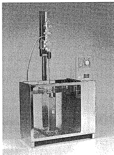
Figure 4.26 Apparatus for pipette sampling (photograph courtesy of ELE International)
