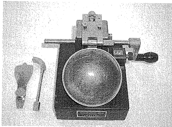
Figure 2.15 Casagrande liquid limit apparatus and tools (photograph courtesy of Cranfield University)
