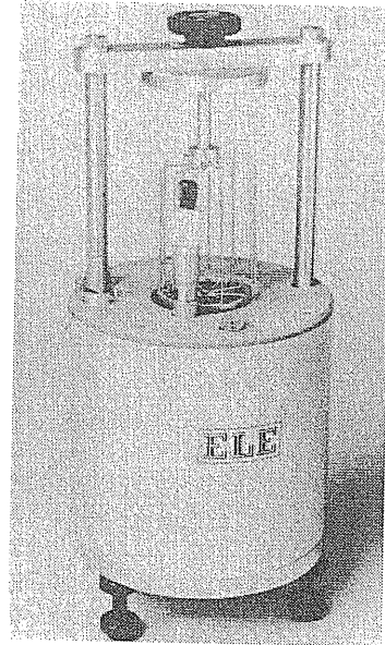
Figure 2.23 Shrinkage limit test — TRL apparatus
