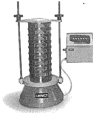
Figure 1.22 Sieve shaker, high frequency vibratory type (photograph courtesy of Impact Test Equipment)
