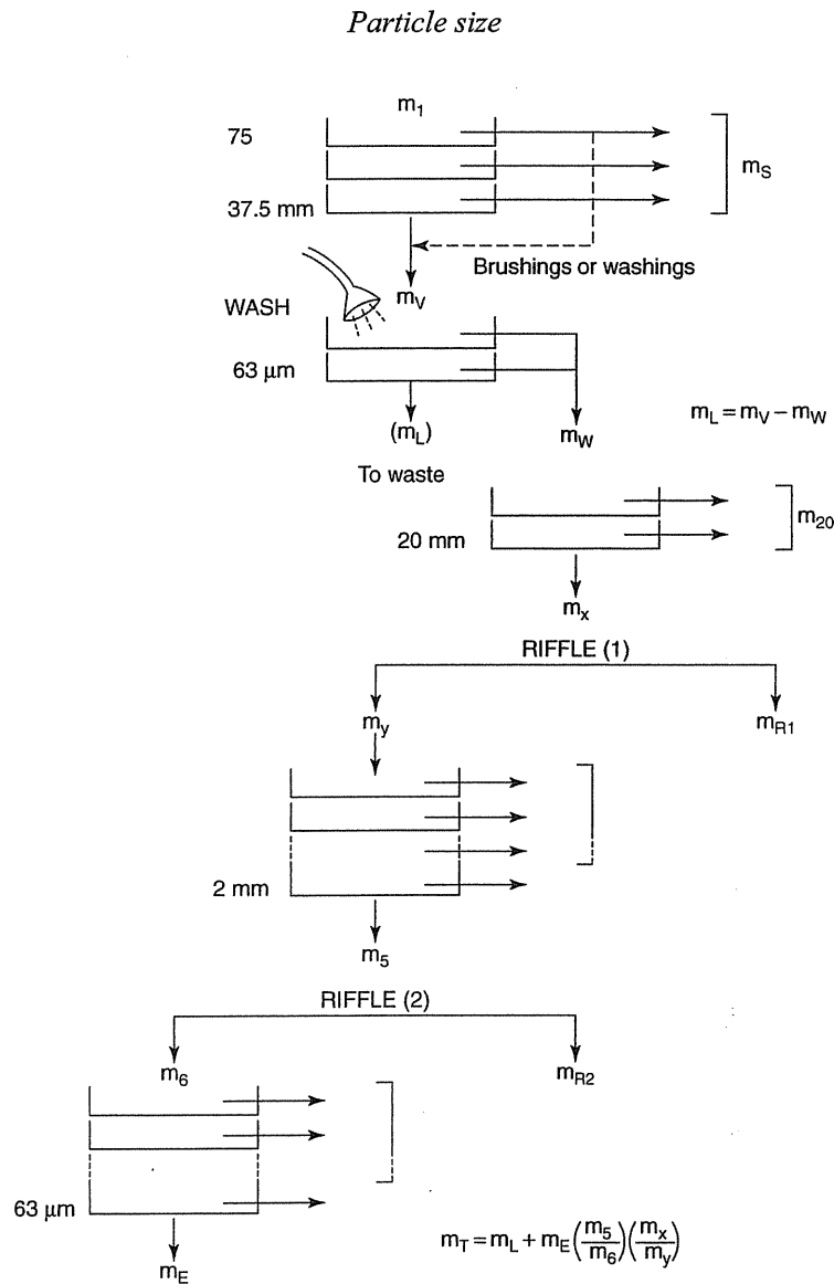
Figure 4.20 Sequence diagram for sieving cohesive soils with gravel ('boulder clay' type)
