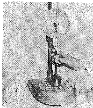
Figure 2.12 Cone penetrometer test immediately after penetration
