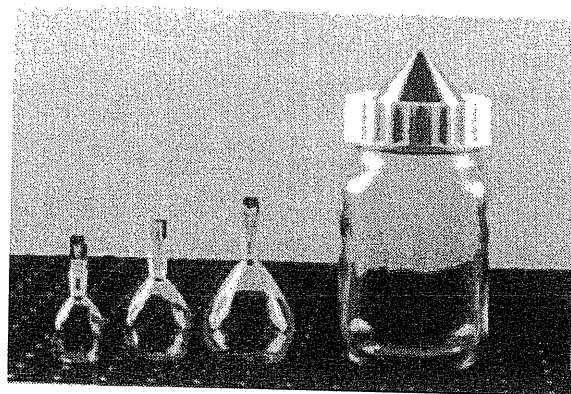
Figure 3.14 Density bottles and large pyknometer
