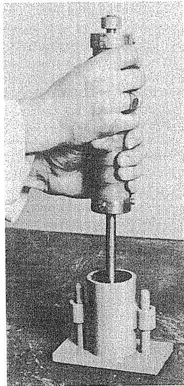
Figure 6.24 Harvard compaction apparatus (photograph courtesy of ELE International)
