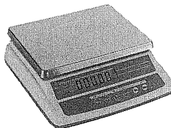
Figure 1.4 Electronic medium top-pan balance, with a capacity of 2100 g and a resolution of 0.01 g (photograph courtesy of ELE International)
