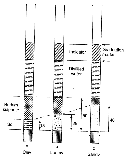
Figure 5.4 Glass tubes for pH test (colorimetric method)
