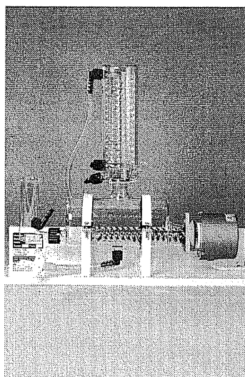
Figure 1.17 Electric water still (photograph courtesy of ELE International)
