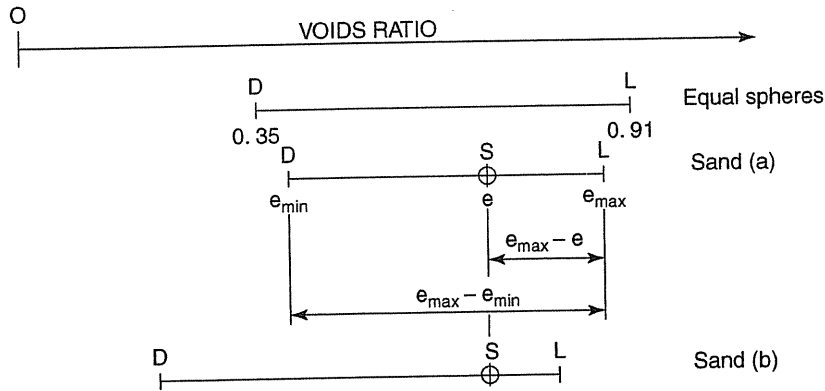
Figure 3.7 Density index of two sands
