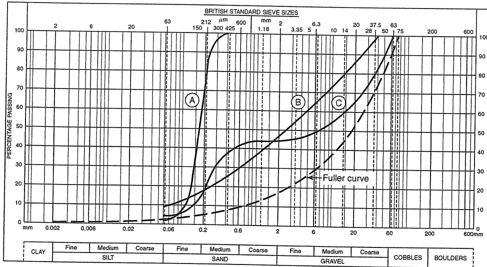
Figure 4.5 Particle size curves: sands and gravels
