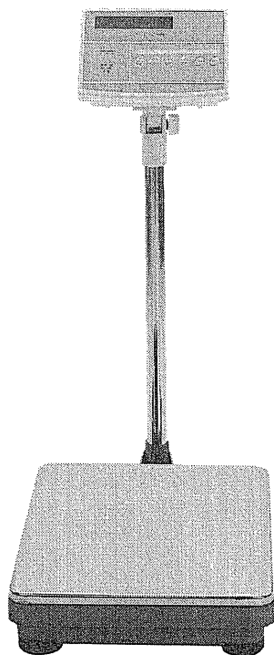
Figure 1.2 Electronic platform scales, with a capacity of 60 kg and a resolution of 10 g (photograph courtesy of ELE International)
