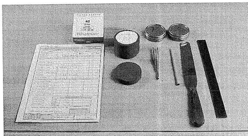
Figure 2.28 Equipment for soil suction test (photograph courtesy of Soil Property Testing Ltd.)
