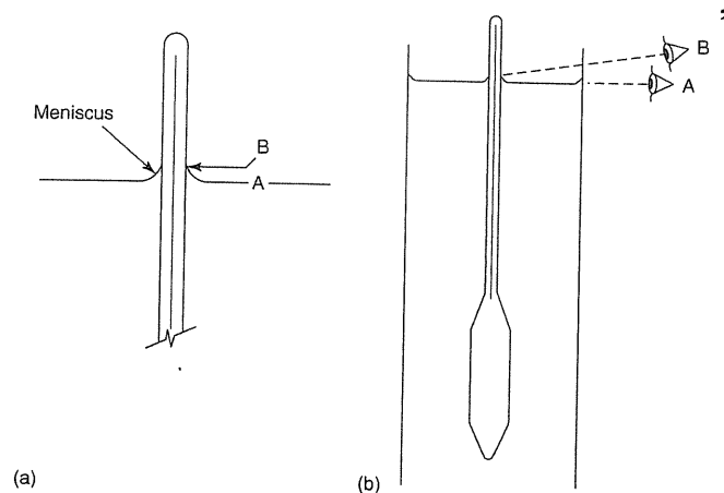
Figure 4.30 Reading a hydrometer
