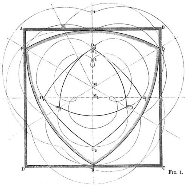
Figure 21: A Reuleaux triangle moving in a square (from Reuleaux, 1876/1963, p. 136)
