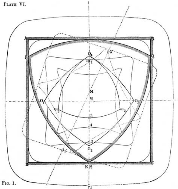
Figure 22: A square moving around a Reuleaux triangle (from Reuleaux, 1876/1963, p. 137)
