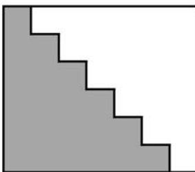
Figure 7: A visual proof of the formula for the sum from 1 to n
