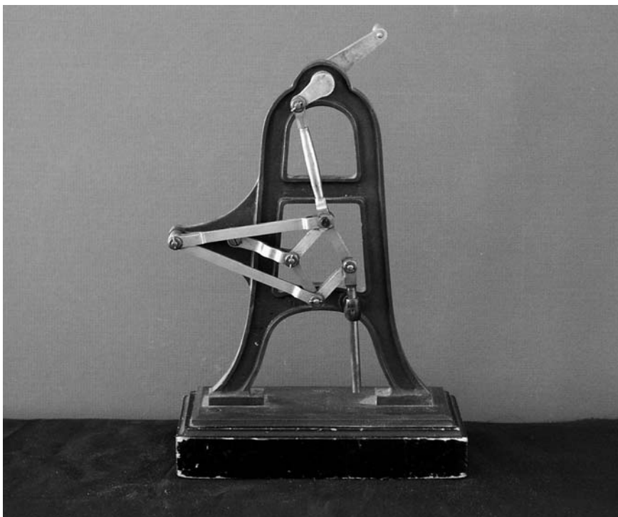
Figure 17a: The Peaucellier linkage (photographed by Francis C. Moon)
