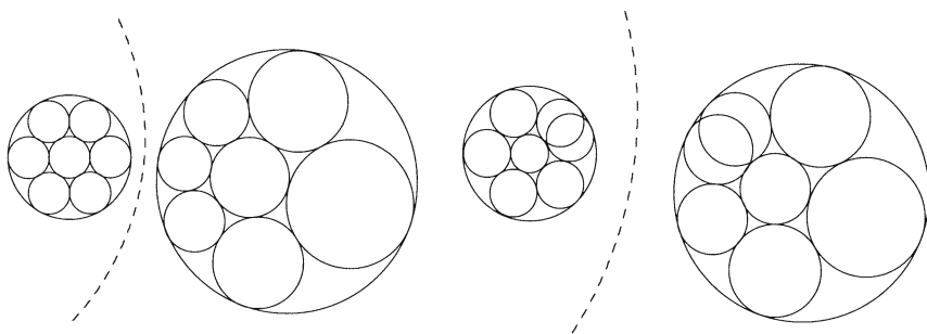
Figure 9: Inversion provides a solution to Steiner's circle problem
