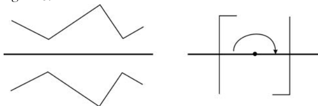
Figure 3: ‘Straight’ as meaning “symmetric”
