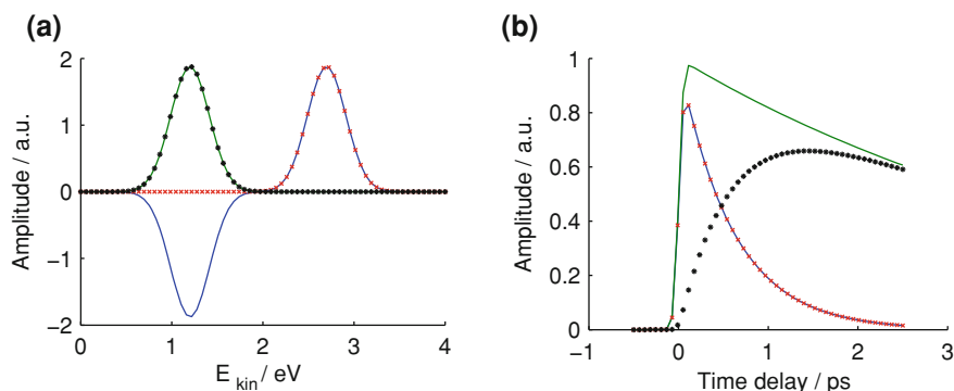
Fig. 3.6 Representation of the global fit of the time-resolved photoelectron spectrum shown in Fig. 3.5. a DAs A_1 (blue) and A_2 (green). Also shown are the photoelectron spectra \epsilon_1 (red) and \epsilon_2 (black). b basis functions B_1 (blue) and B_2 (green). Also shown are the time-dependent populations of the \alpha (red) and \beta (black) states, convolved with the Gaussian cross correlation of the pump and probe pulse
