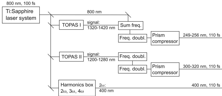
Fig. 6.3 Schematic overview of the laser setup in Ottawa. Indicated are the wavelength ranges and outputs used in the experiments conducted in this project. Pulse durations are fwhm values
