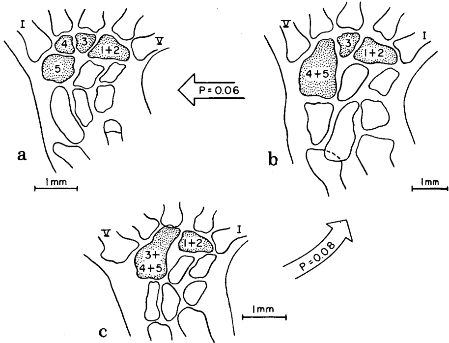
Figure 4.26. Patterns of variation in distal tarsal arrangements (stippled) in Bolitoglossa , a tropical genus of salamanders. Intraspecific variation can be extrapolated to interspecific variation. (From Alberch 1980, with permission.)
