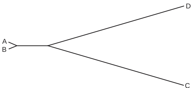
Figure 2.13. The case in four-taxon analyses where sister taxa are unusually long-branched.
