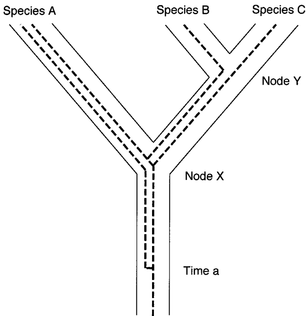
Figure 3.5. Relationships between gene histories and population divergence. Nodes refer to population splits, resulting in species formation. At time a , a gene lineage splits into two. At node X , both gene lineages survive in separated species A , but only one survives in the right-hand lineage. At the time of population splitting at node X , another gene lineage arises and survives to node Y and in species B but disappears in the population leading to species C .
