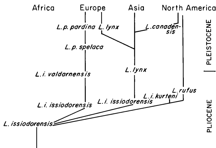
Figure 6.20. The phylogeny of the genus Lynx . Note the transitional subspecies and species in the evolution of L. pardina . (After Werdelin 1981.)
