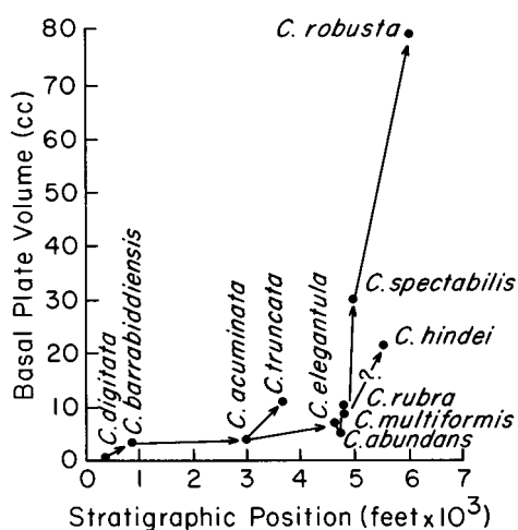
Figure 6.11. Increase of size of the principal "species" of Calceolispongia , as a function of stratigraphic position. (After Teichert 1949.)
