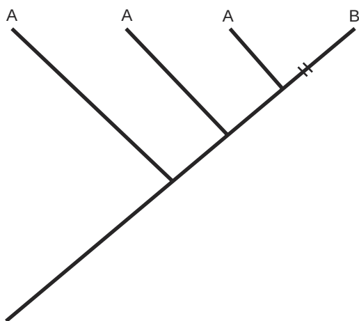
Figure 3.1. A cladogram showing population B, which is reproductively isolated from the three A populations. If the three A populations are reproductively compatible, then conflicts exist between the biological species concept and the phylogenetic species concept.
