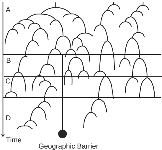
Figure 3.6. A complex history of allelic births and deaths is interrupted by a geographic separation at the end of period A . During periods B and C , the lineages in incipient species 2 are polyphyletic, but by period D , the complex ancestry is erased by extinctions and new alleles, producing monophyletic lineages of genes for each new species. (After Avise and Ball 1990.)
