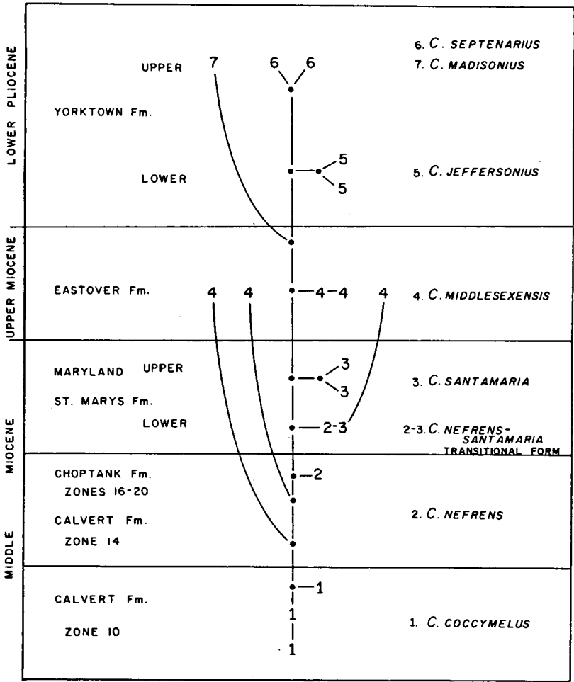
Figure 2.19. Cladogram for the Miocene-Pliocene Atlantic coastal plain scallop Chesapeecten , superposed on the stratigraphic sequence. (From Miyazaki and Mickevich 1982, with permission.)
