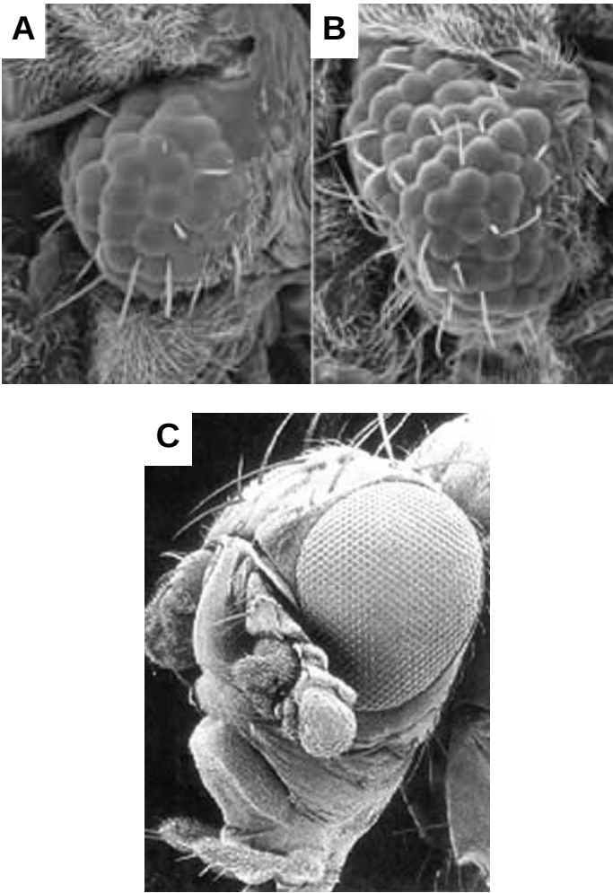
Figure 4.9. (A and B) Ectopic eyes induced by application onto fruit flies of mRNAs; (C) products of the Pax-6 gene from the squid Loligo opalescens . (From Tomarev et al. 1997 with permission; © 1997, National Academy of Sciences USA.)
