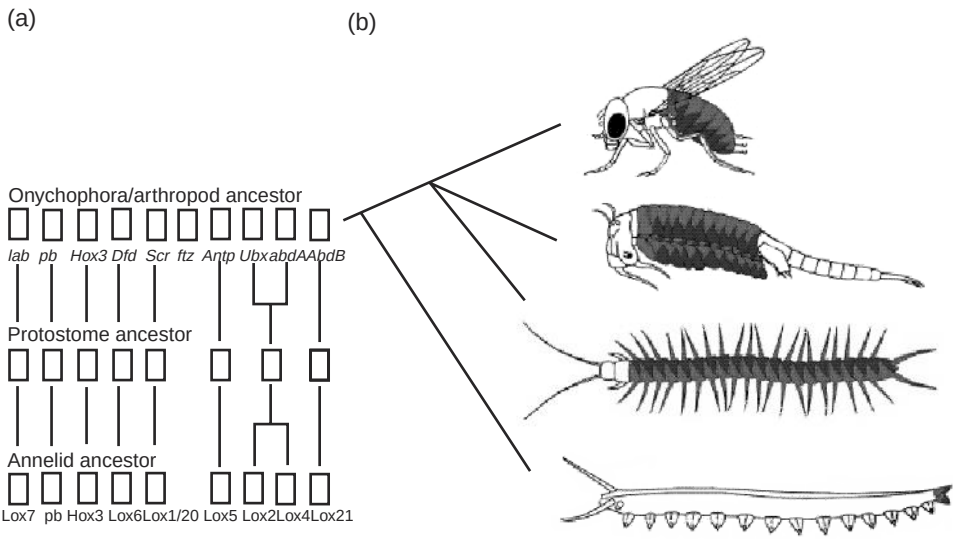
Figure 4.11. Hox gene evolution in arthropods and relatives. Drosophila , Artemia , a centipede, and an onychophoran all share the same Hox genes, casting suspicion on the idea that Hox genes alone are sufficient for segment specification. Annelids and arthropods have evolved a pair of Hox genes by means of duplication. The expression patterns of Ultrabithorax (black) and abdominal-A (shaded) are shown at right.
