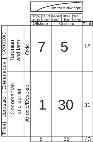
Figure 7.12. The time and environment of first occurrences of orders of marine macroinvertebrates. The larger numbers form a contingency table whose contents are nonrandom. (After Jacobs and Lindberg 1998.)
