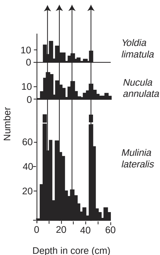
Figure 7.1. Diagrammatic representation of actual abundance over time in Long Island Sound of the opportunistic bivalve Mulinia lateralis and the bivalve Nucula annulata , which lives in more environmentally constant conditions. Right, preservation in the fossil record, as recorded in cores.
