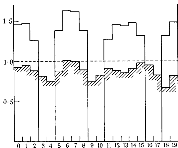
Figure 4.20. Development of spatial inhomogeneity (clear bars) following a local perturbation in concentration of a diffusible substance (hatched bars). (Details of model in Turing 1952.)
