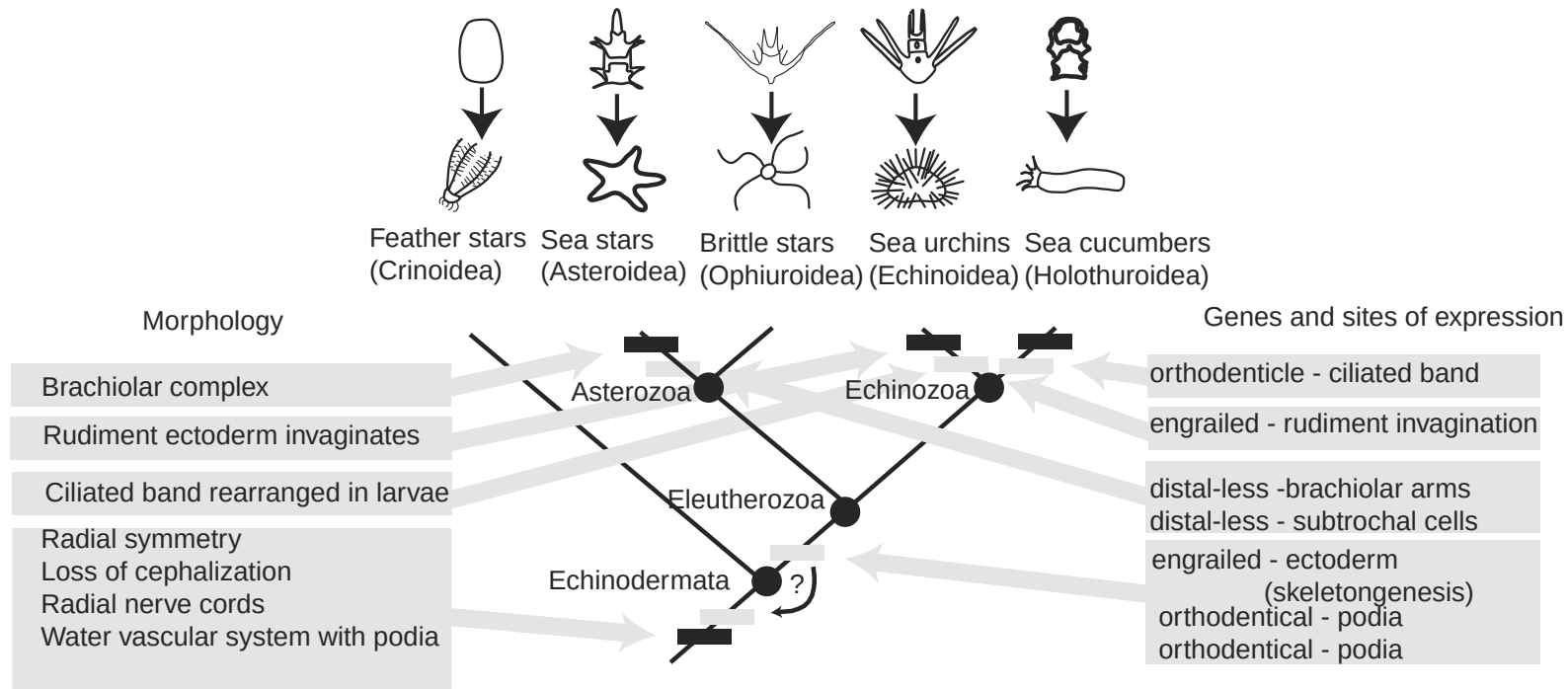
Figure 4.14. Evolutionary history and recruitment of function of developmental roles within the phylum Echinodermata. Reconstructed changes in morphology on left and expression of developmental genes on right. (From Lowe and Wray 1997; reprinted with permission from Nature , © 1997, Macmillan Magazines, Ltd.).
