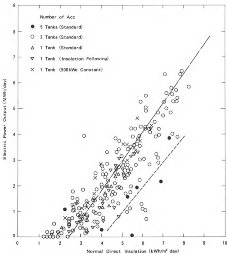
Fig. 10 Relation between Generated Electricity and Insolation
