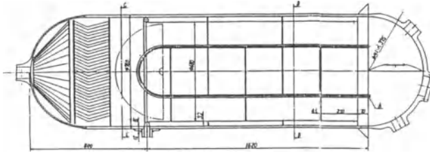
Fig.4.1 Steam generator
