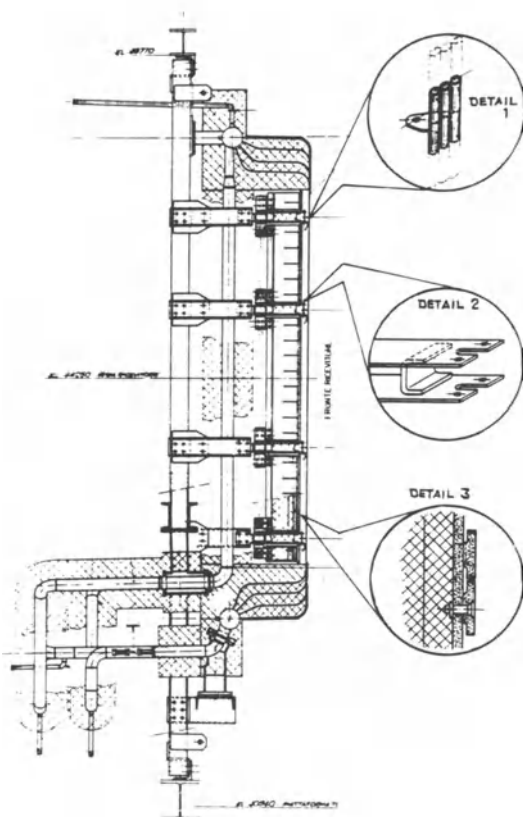
FIG. 2 - Absorber back-structure details
