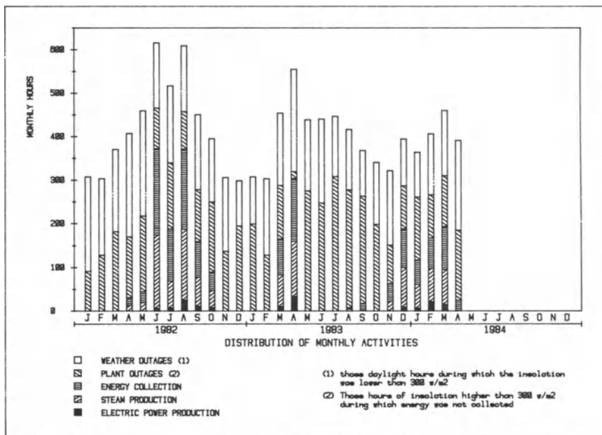
Fig. 1 SSPS-CRS Operation Statistic 1982-4/1984
