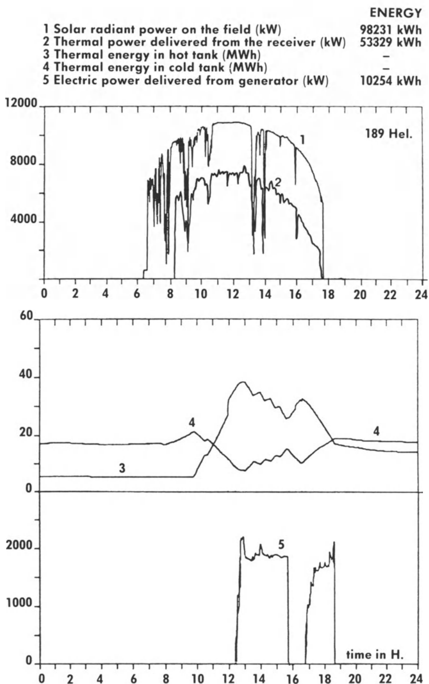
Figure 7 Daily operation: output and energy april 6, 1984
