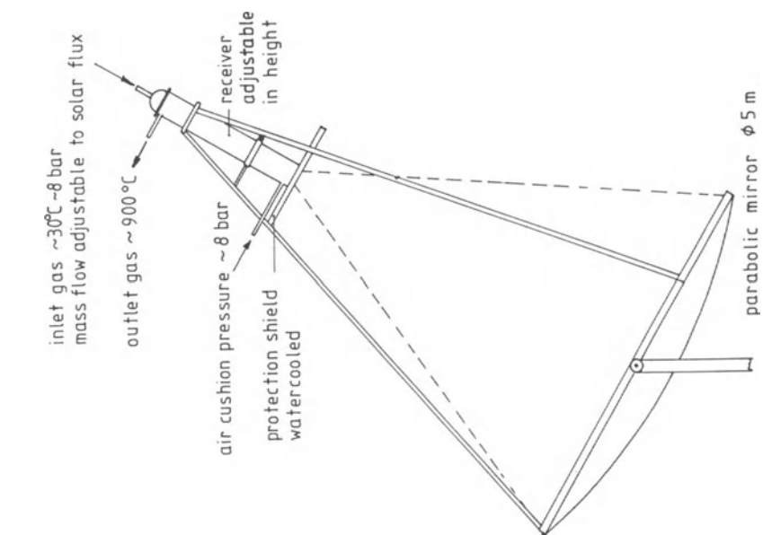
fig. 6: Receiver test facility
