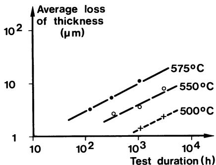
Figure 4- Evolution of the average loss of thickness of 316L SS between 500 and 575°C versus time at various temperatures.
