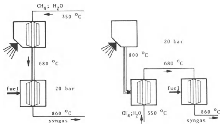
Fig. 4 Alternative Concepts for Solar Steam Reforming
