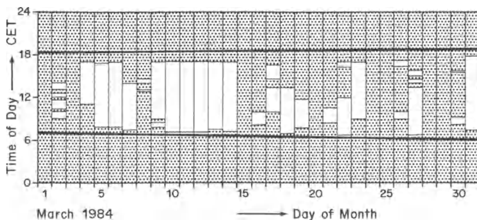
Fig. 4: Monthly sunshine duration chart. Clear spaces represent sunshine, the dotted area sunless periods. The lower solid line represents the astronomical sunrise, the upper one the astronomical sunset.
