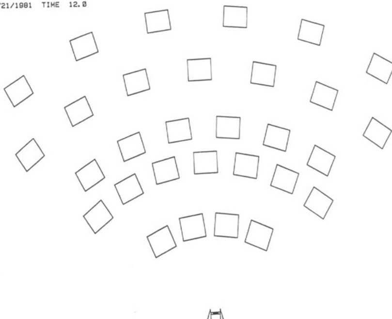
Figure 4. Heliostat Layout For ARCO 'Fairfield Lease' Project
