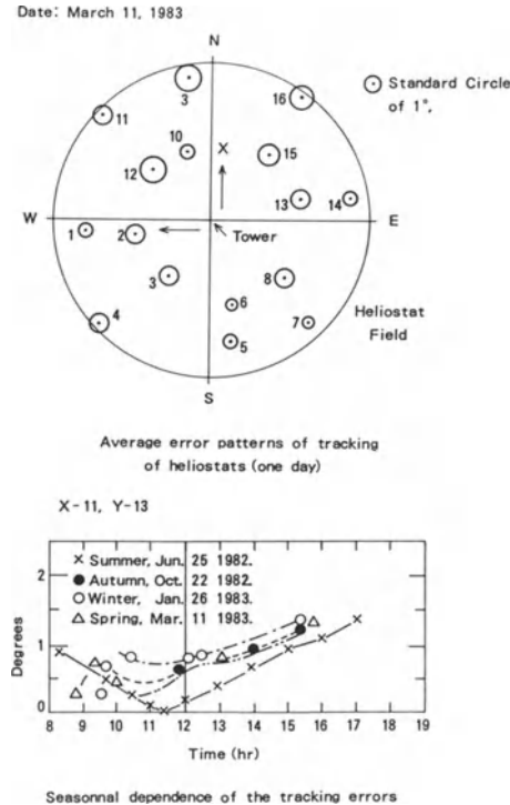
Fig. 4 Tracking Characteristics
