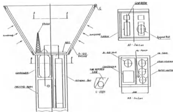
Fig.4.2 An typical arrangement at the top area
