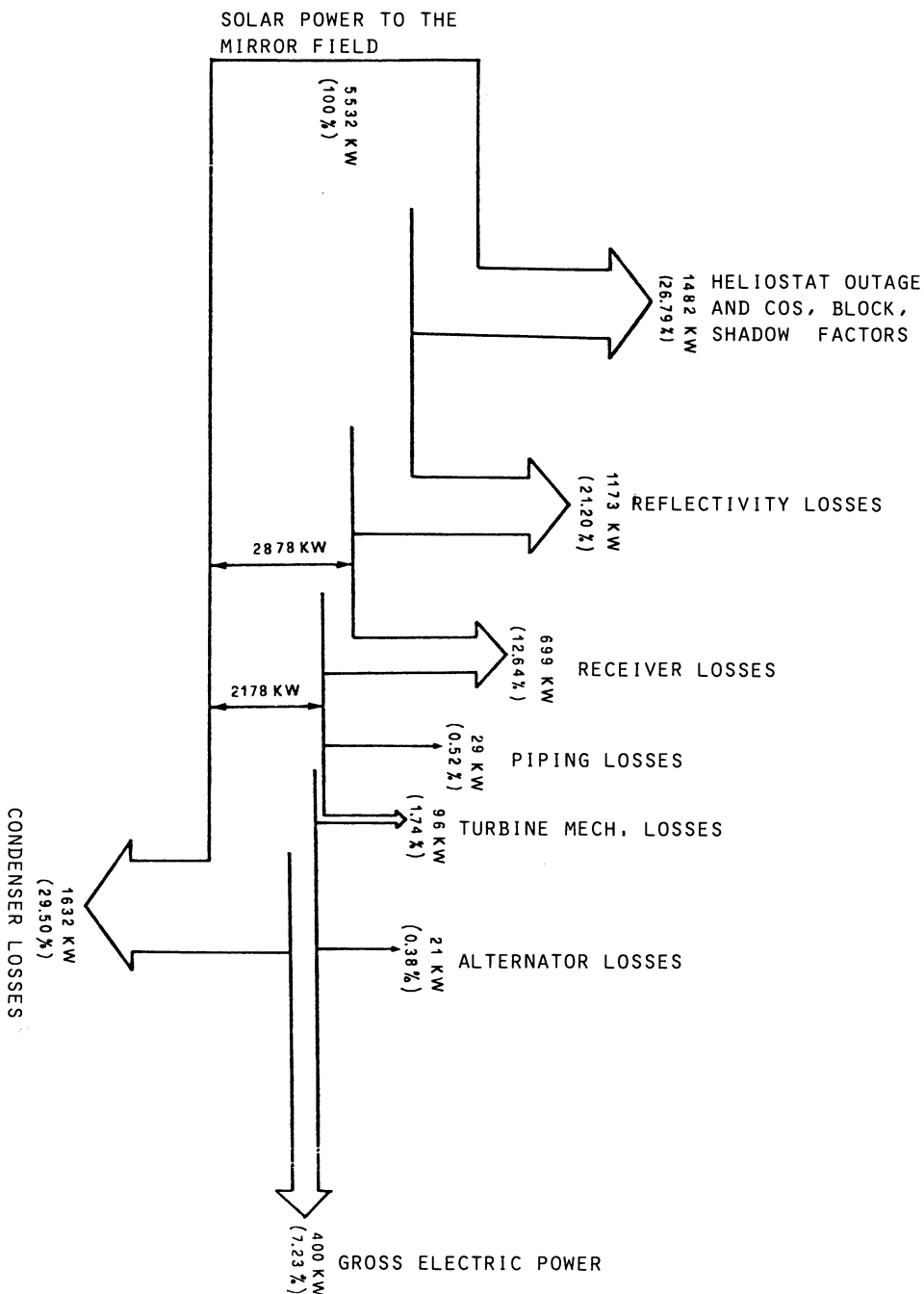
FIG. 1 - PLANT THERMAL BALANCE (DIRECT INSOLATION 890 \text{ W/M}^2 )
