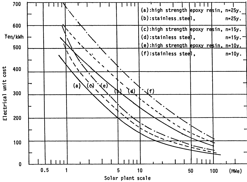
Fig.5 ESTIMATED ELECTRICAL UNIT COST
