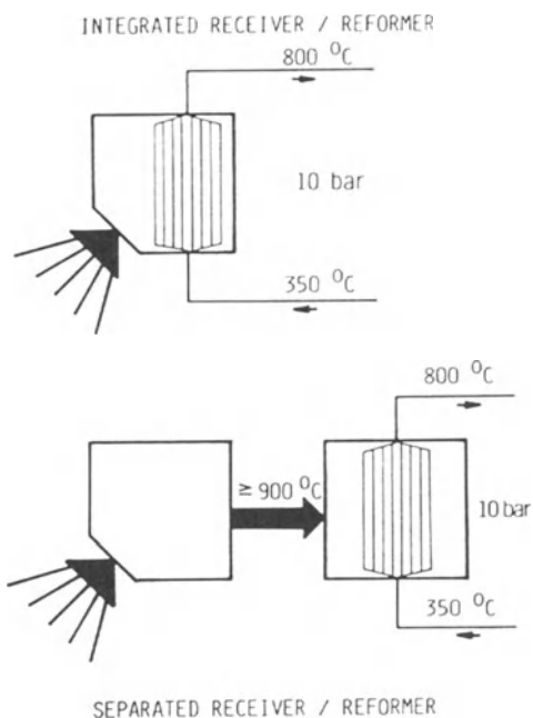
Fig. 3 Receiver/Reformer Arrangements
