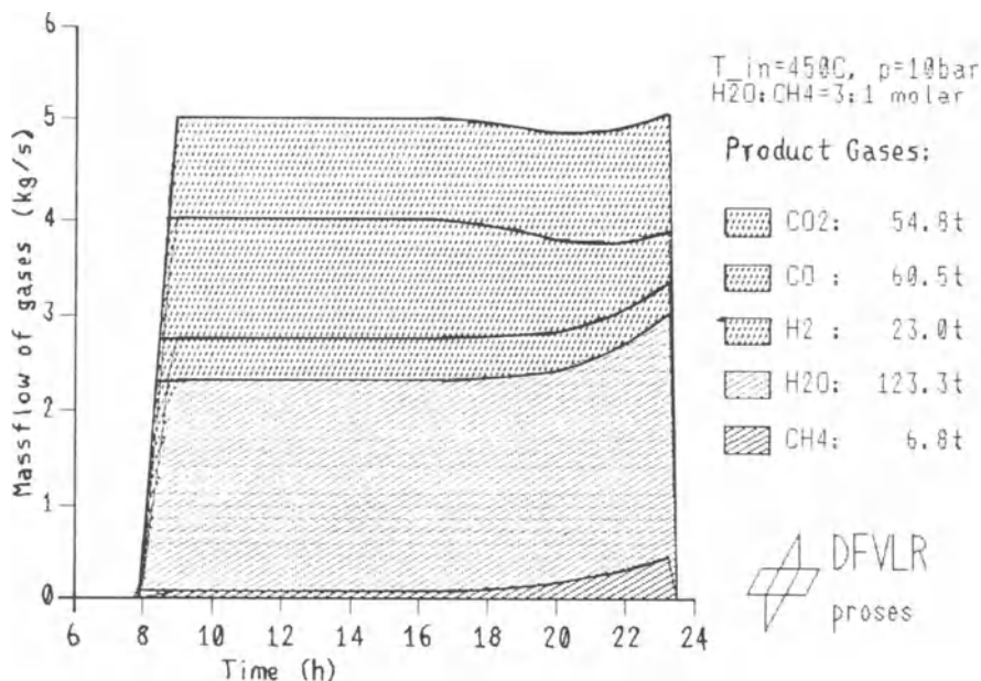
Figure 4: Output of methane/steam reformer on December 21. The temperature dependance of the process has been computed with the programs "GLEICH" and "END" of KFA Jülich, NFE project.
