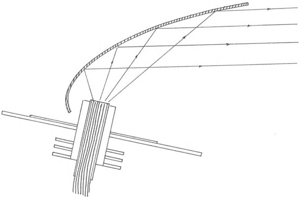
Fig.4 Proposed Connection of fiber and channel
