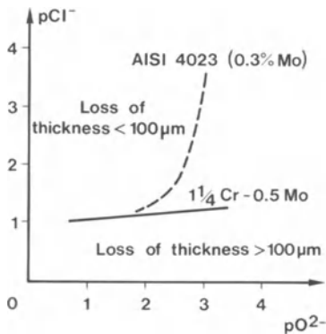
Figure 7 - Effect of oxoacidity and chloride content on corrosion of two ferritic steels (1345h at 500°C).
