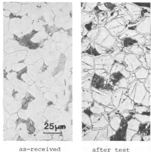
Figure 8 - Nitridation of the AISI 4023 (0.3 % Mo) steel specimen during test in salt without sodium hydroxide addition (100 h, 500°C).
