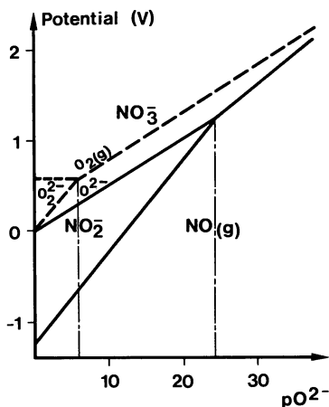
Figure 1- Potential-oxoacidity diagram of nitrate-nitrite mixture at 227°C.
