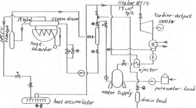
Fig.3.4 Reference system ( Nio plant )
