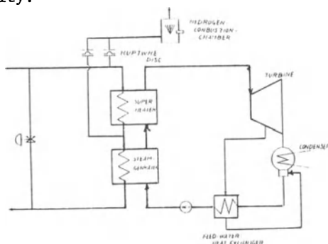
Fig.2.1 Safety System Diagram of Na System Reaction
