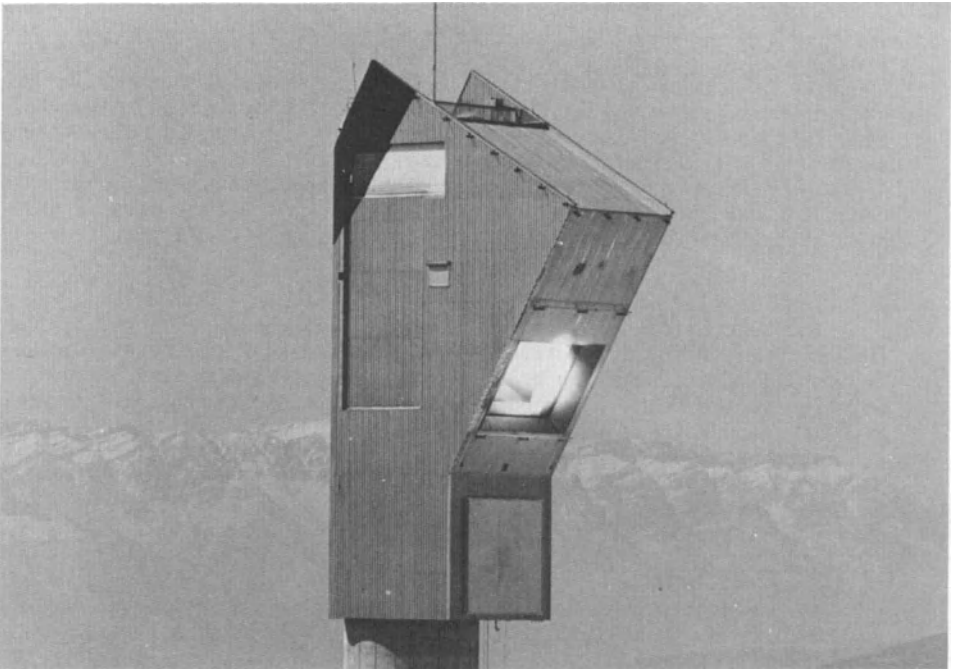
Figure 4 Solar receiver
