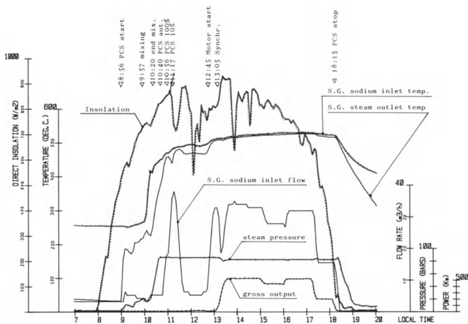
Fig. 15 DAILY OPERATION CHARACTERISTICS 21-FEBRUARY-1984
