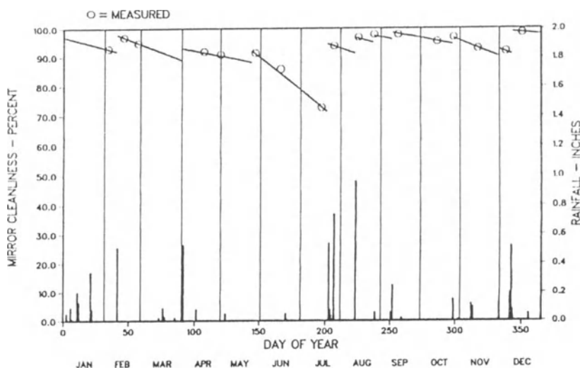
Figure 10. Solar One Mirror Cleanliness and Rainfall: 1982
