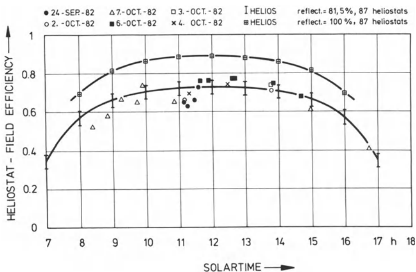
Fig. 5 SSPS-helioStatfield efficiency with respect to solar time in comparison with HELIOS computations
