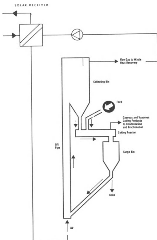
Fig. 6 Adaptation of Heat Exchanger to Test Bed Loop and Lurgi Reactor
