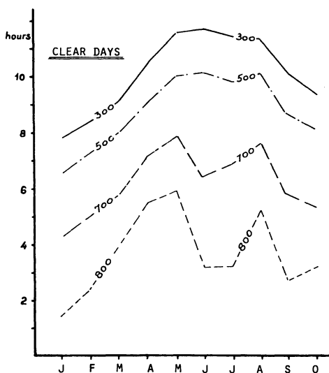
Fig. 6 Sunshine Hours (Jan. - Oct. 1983) Clear Days
