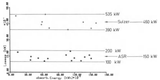
FIGURE 4 Losses during Operation versus absorbed Energy
