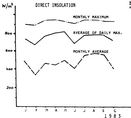
Fig. 7 Direct Insolation Data (Jan. - Oct. 1983)
