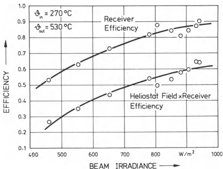
Fig. 6 Receiver and thermal efficiency measurements in dependance of the beam irradiance
