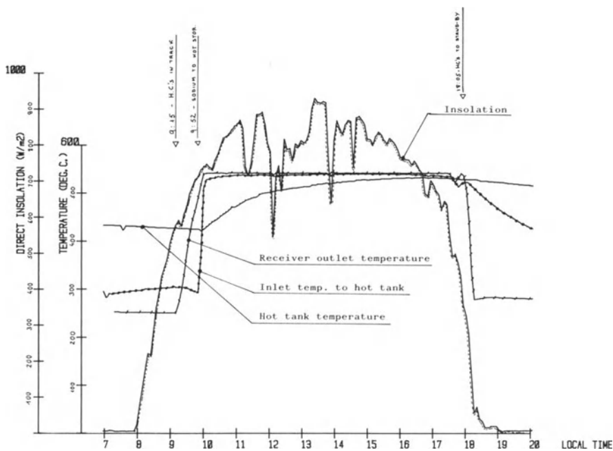
Fig. 14 DAILY OPERATION CHARACTERISTICS 21-FEBRUARY-1984
