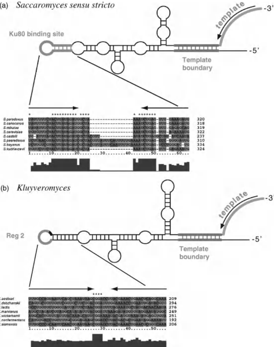
FIGURE 2.5 The 5' arm of Saccharomyces and Kluyveromyces telomerase RNAs. Schemes illustrate the 5' arm, template, and template boundary of Saccharomyces sensu stricto (a) and Kluyveromyces (b) TERs. Blue lines indicate sequence conservation. Sequence alignments showing the conservation of the Ku80-binding site (48 nt stem-loop) in Saccharomyces and a CGGA sequence motif in the Kluyveromyces Reg 2 element were made by the computer program ChustaIX (Chenna et al., 2003). (See the color version of this figure in Color Plates section.)
