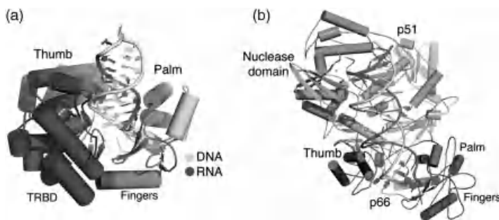
FIGURE 3.4 (a) Same as Figure 3.3a. (b) The structure of the HIV-1 RT bound to an RNA–DNA heteroduplex (PDB ID: 1RTD). (See the color version of this figure in Color Plates section.)
