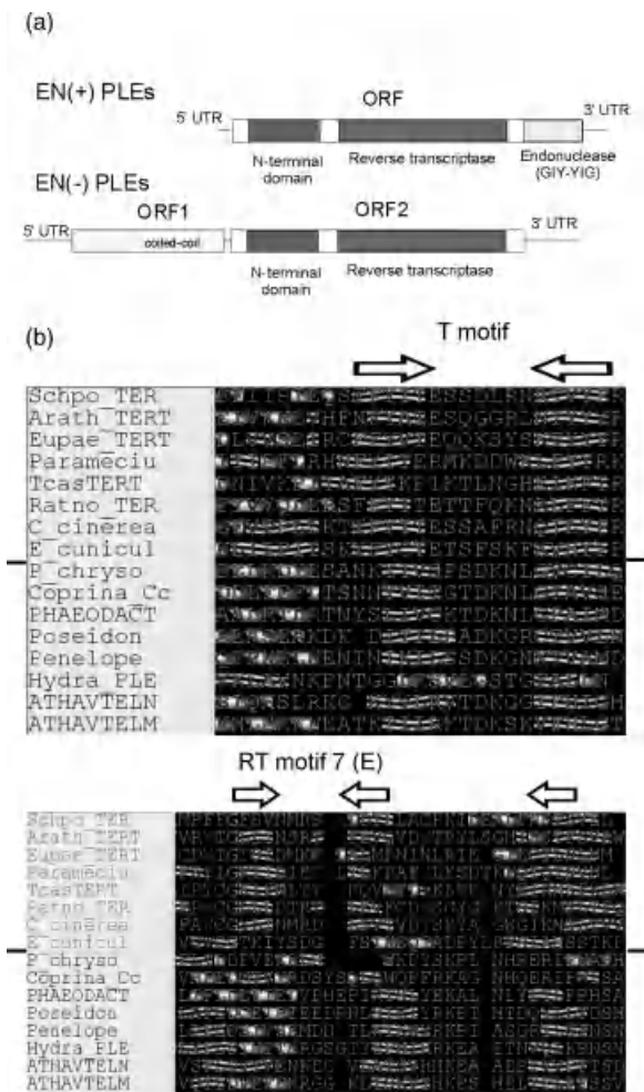
FIGURE 11.6 Structural organization of Penelope -like elements (a) and their similarity to telomerases (b). The EN(–) (endonuclease-deficient) PLEs exhibit specificity for telomerases in diverse eukaryotes. In panel (b), secondary structure predictions for representative TERT (top 8) and PLE (bottom 8) sequences are compared in selected portions of the RT amino acid alignment, showing the N-terminal T-motif region and the C-terminal motif 7 of the core RT domain. Arrows designate characteristic beta-hairpins in the secondary structure. Sequences were viewed with the aid of a structure-based sequence alignment program (STRAP) ( http://www.bioinformatics.org/strap/ ). (See the color version of this figure in Color Plates section.)
