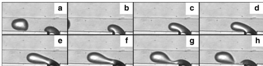
Fig. 1.4 The droplet generation in the dripping regime (a to h) with Ca = 0.036 and Q = 1.2 , where Ca is defined as (1.15) and Q is the flow rate ratio ( Q_d/Q_c )
