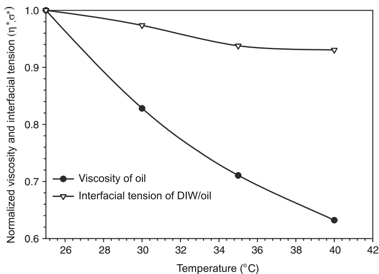
Fig. 3.2 Characteristic temperature dependency of viscosity of a mineral oil and of the interfacial tension between this oil and water
