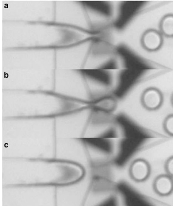
Fig. 3.8 Squeezing regime A encountered at a temperature of 35°C
