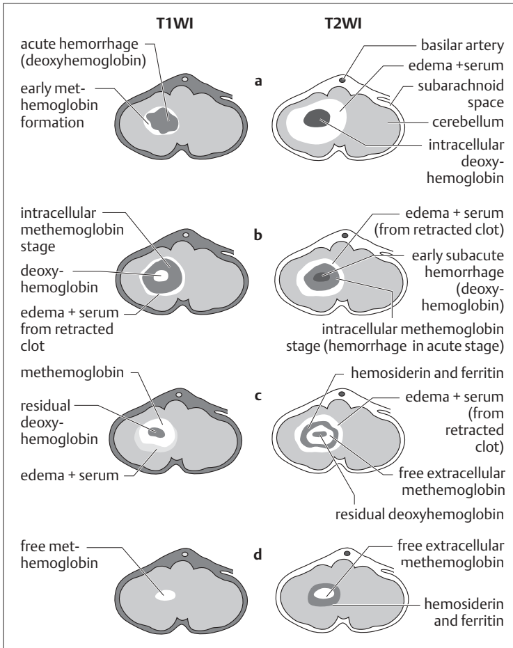
Fig. 4 Stages and estimation of age of hemorrhage on MRI. MRI scenarios of posterior fossa (right cerebellar) hemorrhage during: a the acute stage, i.e., within 48 hours of ictus. On the T1WI hemorrhage appears slightly hypodense to cerebellar parenchyma, due to the T2 effect of deoxyhemoglobin. There is a small amount of peripheral high density due to early intracellular methemoglobin formation. The T2WI demonstrates marked hypointensity caused by intracellular deoxyhemoglobin in intact red blood cells. b Early subacute stage, i.e., within 3 to 7 days from ictus, during the time in which there is oxidation of the deoxyhemoglobin to methemoglobin inside the red blood cells at the periphery of the clot. On the T1WI the central hemorrhage shows a high signal due to intracellular deoxyhemoglobin, whereas on the T2WI
