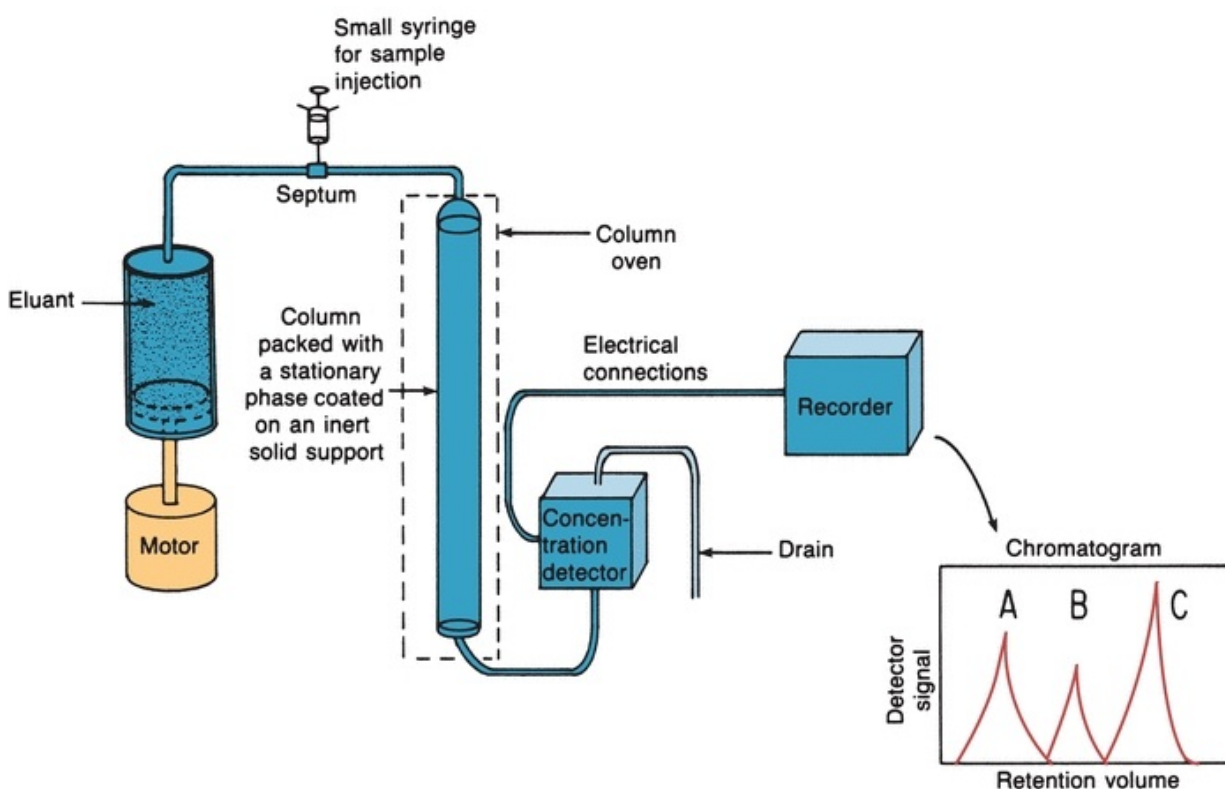
FIGURE 6.4 High-performance liquid chromatography basic components. (Adapted from Bender GT. Chemical Instrumentation: A Laboratory Manual Based on Clinical Chemistry. Philadelphia, PA: WB Saunders; 1972.)
