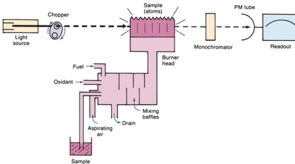
FIGURE 5.11 Single-beam atomic absorption spectrophotometer—basic components.
