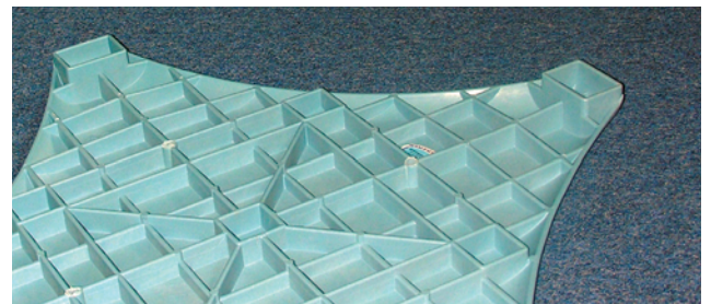
DIAMOND ARMATURE of an injection-molded plastic table is visible against the light. Design: IKEA.
