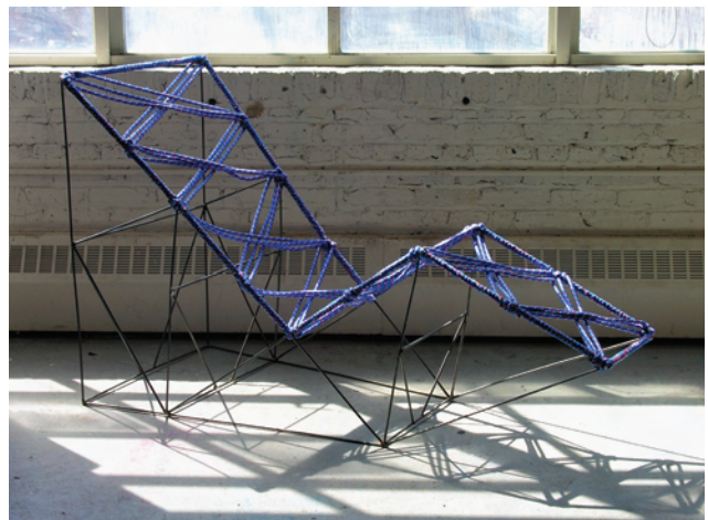
ROPE AND METAL CHAIR. We resolved the issue of the rope slipping along the metal frame by wrapping rope around the metal rod to create spacers between the knots. Design: Lily Worledge, MICA.
