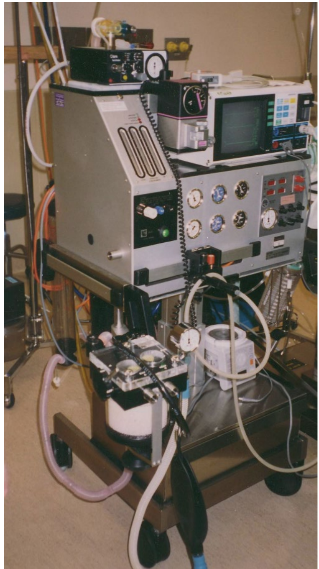
Figure 2.5 Ergonomic anesthetic machine with Claire ventilator and monitor on top.
