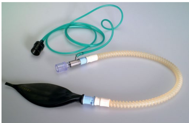
Figure 2.7 Jackson Rees T piece modification with his prolonged intubation tube attached.
