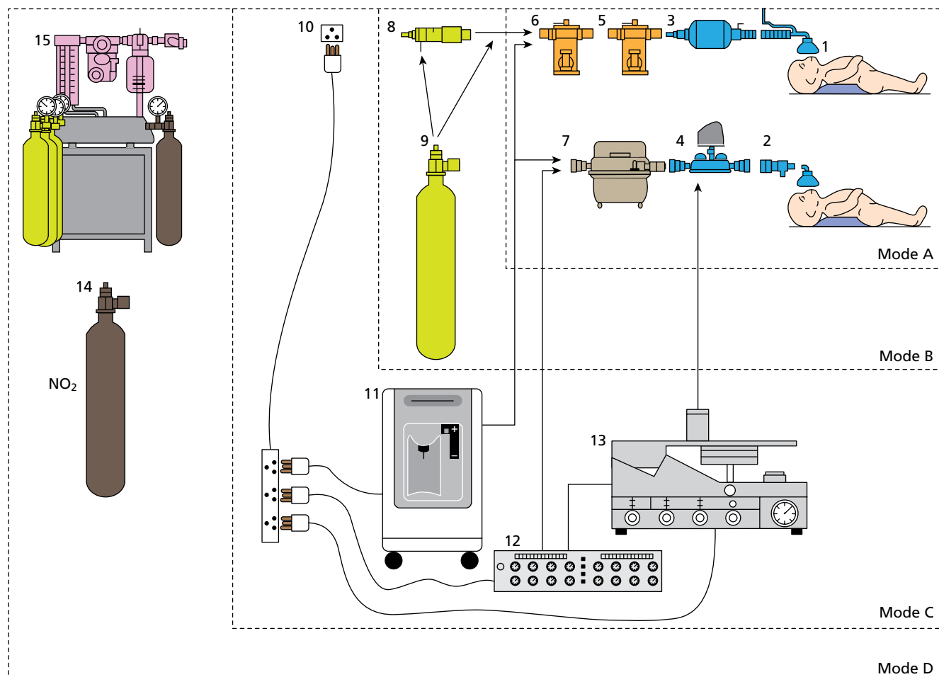
Figure 44.5 A schematic diagram of anesthetic systems that could be used, depending on available resources. Mode A provides basic inhalation anesthesia with air, spontaneous ventilation, or self-inflating bags. Draw-over vaporizers are required. Mode B provides oxygen enrichment but requires the availability of oxygen cylinders. Plenum vaporizers can be used. Mode C requires electricity to power the oxygen concentrator, air compressor, and/or ventilator. A mechanical ventilator (e.g. Manley) does not require electrical power. Mode D requires a Boyle's machine and nitrous oxide cylinders. 1, T-piece with reservoir tube and facemask; 2, Ambu paed valve; 3, self-inflating bag (Ambu); 4, Oxford inflating bellows; 5, Oxford miniature vaporizer (OMV) with halothane; 6, OMV with trichloroethylene; 7, EMO (Epstein Macintosh Oxford) vaporizer with ether. These circuits and manual ventilators are interchangeable and ether, halothane, and trichloroethylene can be used on their own or in series. 8, Farman's entrainer with an oxygen cylinder (9) can be used to supplement oxygen, or an electrical power source (10) is available with an oxygen concentrator (11), air compressor (12), or Manley ventilator (13). Nitrous oxide (14) and Boyle's apparatus (15) allow anesthesia practice equivalent to that of developed countries.
