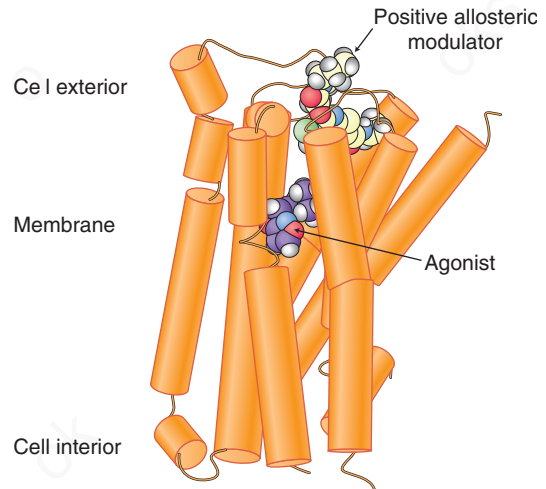
Fig 3.7 Structure of the M_2 muscarinic receptor. High-resolution image showing the conformation of the M_2 muscarinic receptor bound with both an agonist (orthosteric) and a positive allosteric modulator. The brown cylinders represent the transmembrane domains. The full extent of the N- and C-terminal domains and the third intracellular loop are not shown. (Courtesy A. Christopoulos.)
