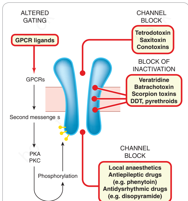
Fig. 3.21 Drug-binding domains of voltage-gated sodium channels (see Ch. 44). The multiplicity of different binding sites and effects appears to be typical of many ion channels. DDT , Dichlorodiphenyltrichloroethane (dicophane, a well-known insecticide); GPCR , G protein-coupled receptor; PKA , protein kinase A; PKC , protein kinase C.
