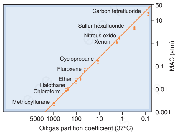
Fig. 42.1 Correlation of anaesthetic potency with oil:gas partition coefficient. Anaesthetic potency in humans is expressed as minimum alveolar partial pressure (MAC) required to produce surgical anaesthesia. There is a close correlation with lipid solubility, expressed as the oil:gas partition coefficient. (From Halsey, M.J., 1989. Physicochemical properties of inhalation anaesthetics . In: Nunn, J.F., Utting, J.E., Brown, B.R. (Eds), General Anaesthesia , Butterworth, London.)
