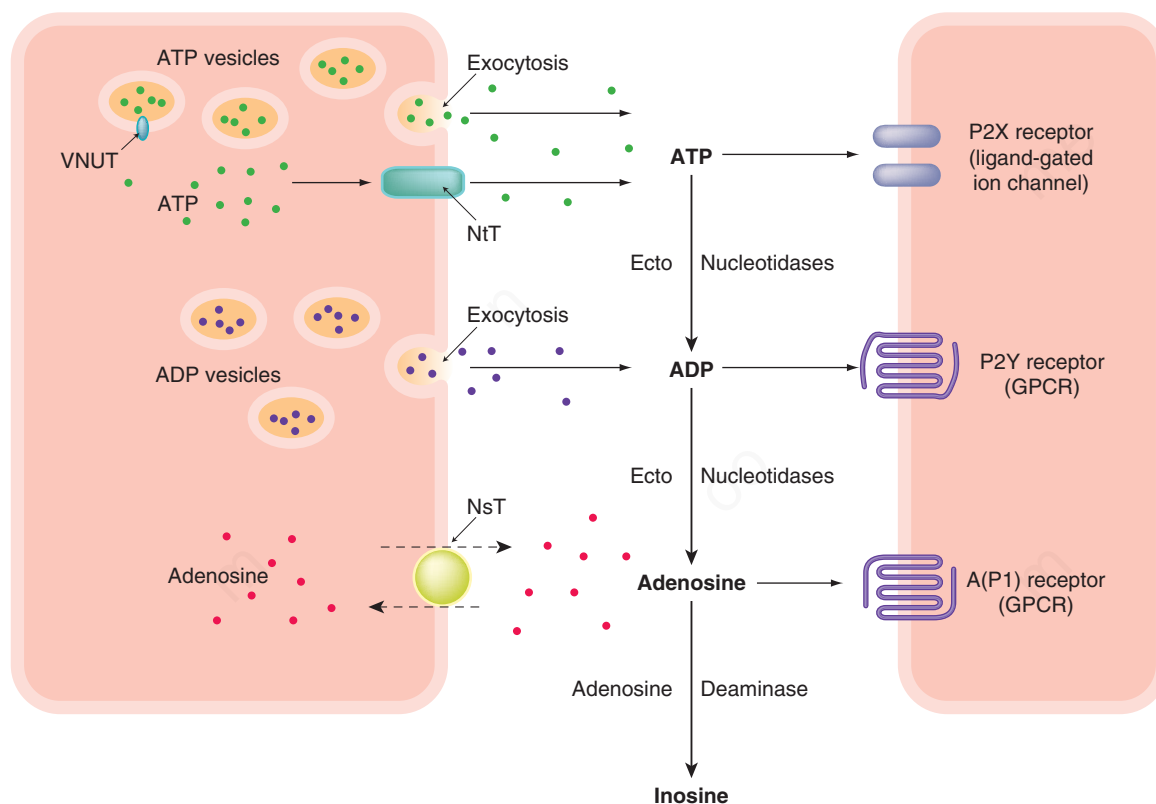
Fig. 17.1 Purines as mediators. ATP (and in platelets, ADP) is present in the cytosol of cells (and released following cellular damage) or concentrated into vesicles by the vesicular nucleotide transporter (VNUT). Nucleotides may be released by exocytosis or through membrane channels such as pannexins (Pnx) or transporters (NtT). Once released, ATP can be converted to ADP and to adenosine by the action of ectonucleotidases. Adenosine is present in the cytosol of all cells and is released and taken up via a specific membrane transporter(s) (NsT), which is blocked by dipyridamole. Adenosine itself can be hydrolysed to inosine by the enzyme adenosine deaminase. ATP acts directly upon the P2X receptors (ligand-gated ion channels) but also upon P2Y receptors (GPCRs; G protein coupled receptors), the principal target for ADP. Adenosine itself acts on A receptors (also called P1 receptors), which are also GPCRs. Ch. 4 contains more details of exocytotic and other secretory mechanisms.
