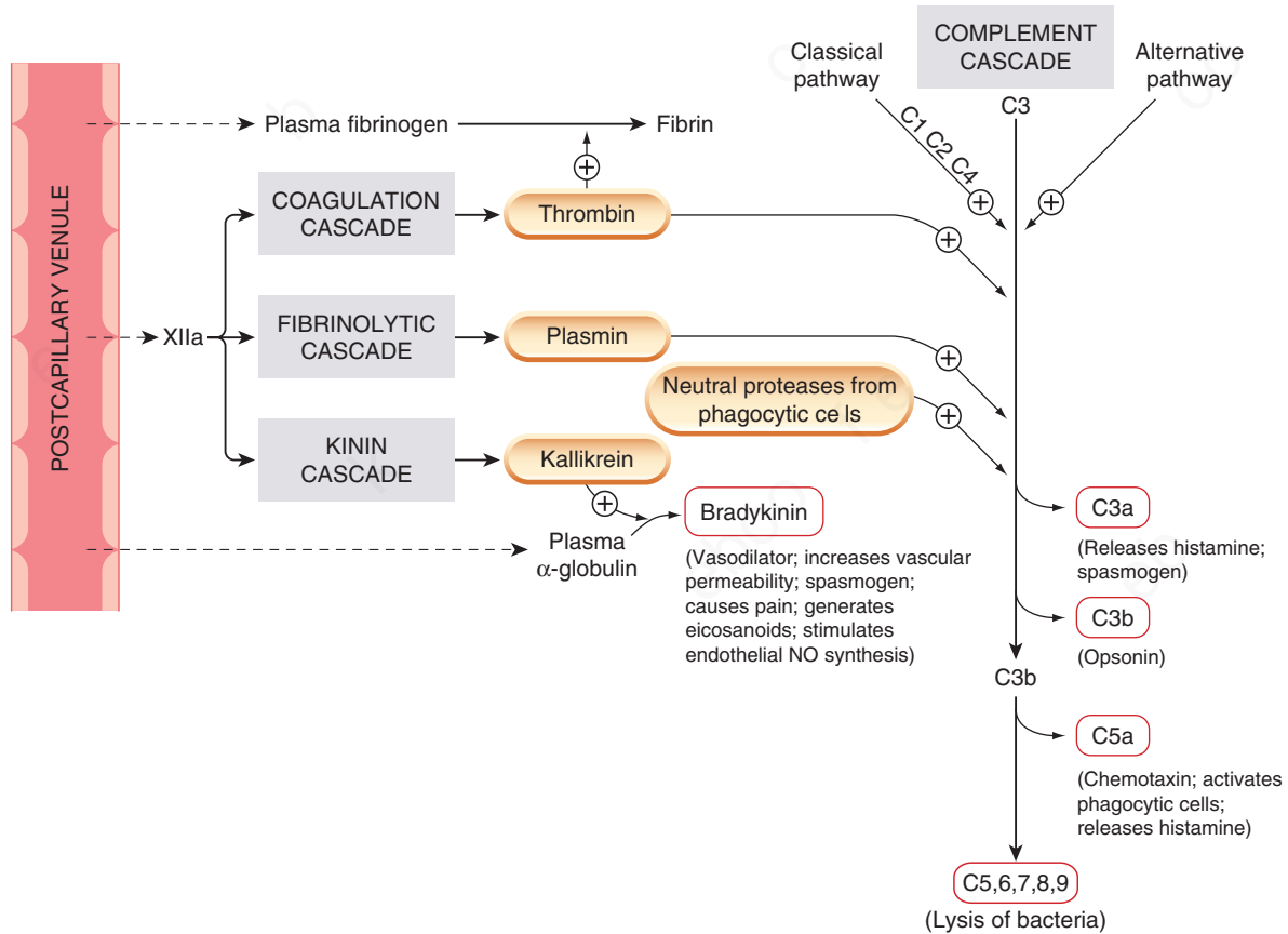
Fig. 7.1 Four enzyme cascades are activated when plasma leaks out into the tissues as a result of the increased vascular permeability of inflammation. Factors causing exudation are depicted in Fig. 7.2. Mediators generated are shown in red-bordered boxes. Complement components are indicated by C1, C2, etc. When plasmin is formed, it tends to increase kinin formation and decrease the coagulation cascade. XIIa, Factor XIIa, see text. (Adapted from Dale, M.M., Foreman, J.C., Fan, T-P. (eds), 1994. Textbook of Immunopharmacology. 3rd ed. Blackwell Scientific, Oxford.)
