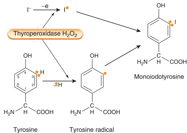
Fig. 35.2 Iodination of tyrosyl residues by the thyroperoxidase- \text{H}_2\text{O}_2 complex. This probably involves two sites on the enzyme, one of which removes an electron from iodide to give the free radical \text{I}^\bullet ; another removes an electron from tyrosine to give the tyrosyl radical (shown by orange dot). Monoiodotyrosine results from the addition of the two radicals.
