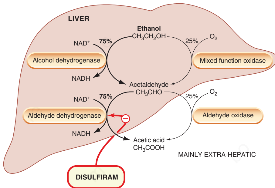
Fig. 49.5 Metabolism of ethanol. NAD, nicotinamide adenine dinucleotide.
