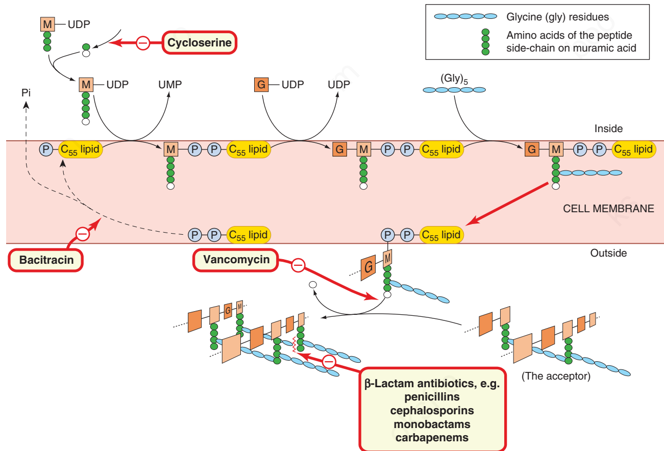
Fig. 51.3 Schematic diagram of the biosynthesis of peptidoglycan in a bacterial cell (e.g. Staphylococcus aureus ), with the sites of action of various antibiotics. The hydrophilic disaccharide–pentapeptide is transferred across the lipid cell membrane attached to a large lipid (C 55 lipid) by a pyrophosphate bridge (–P–P–). On the outside it is enzymically attached to the ‘acceptor’ (the growing peptidoglycan layer). The final reaction is a transpeptidation, in which the loose end of the (Gly) 5 chain is attached to a peptide side-chain of an M in the acceptor and during which the terminal amino acid (alanine) is lost. The lipid is regenerated by loss of a phosphate group (Pi) before functioning again as a carrier. G, N-acetylglucosamine; M, N-acetylmuramic acid; UDP, uridine diphosphate; UMP, uridine monophosphate.
