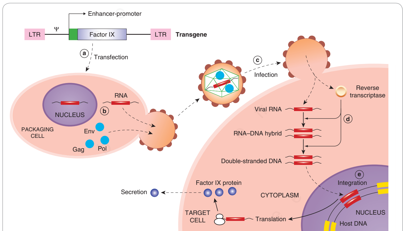
Fig. 5.3 Strategy for making retroviral vectors. The transgene (the example shows the gene for factor IX) in a vector backbone is introduced (a) into a packaging cell, where it is integrated into a chromosome in the nucleus, and (b) transcribed to make vector mRNA, which is packaged into the retroviral vector and shed from the packaging cell. It then infects the target cell (c). Virally encoded reverse transcriptase (d) converts vector RNA into an RNA–DNA hybrid, and then into double-stranded DNA, which is integrated (e) into the genome of the target cell. It can then be transcribed and translated to make (in this case) factor IX protein. 'Env', 'Gag' and 'Pol' represent components of the retroviral vector. LTR , long terminal repeat. (Redrawn from Verma & Somia, 1997.)
