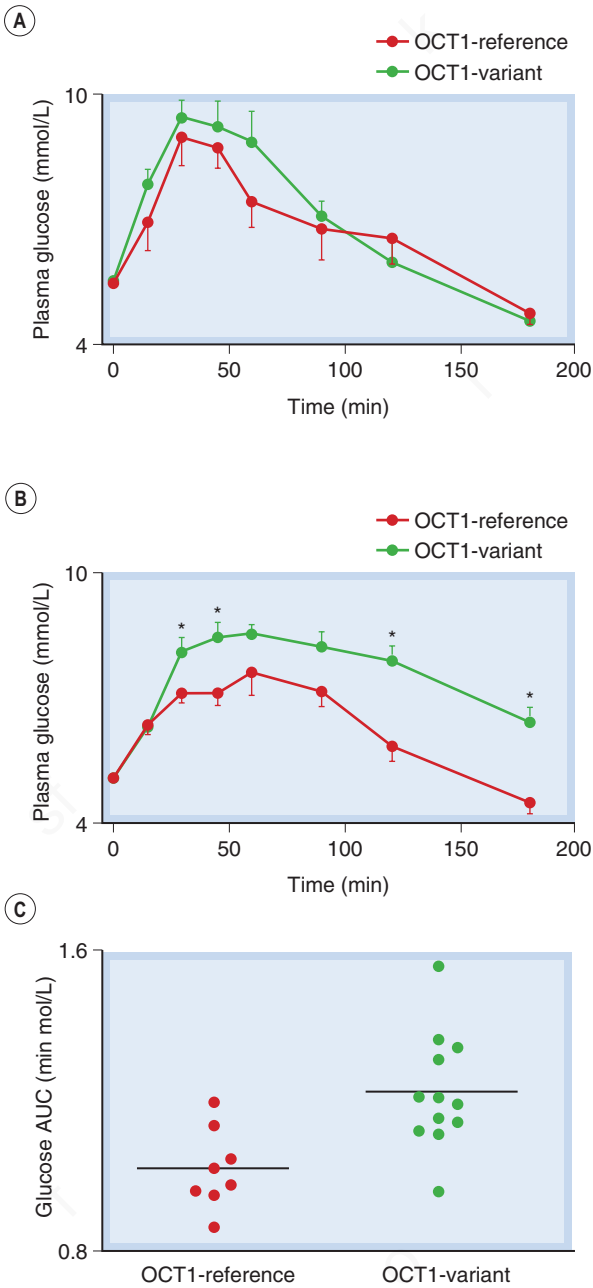
Fig. 9.6 Genetic variants of organic cation transporter 1 (OCT1) are associated with different responses to metformin in healthy humans. (A) An oral glucose tolerance test (OGTT) gave similar plasma glucose responses in control subjects with only reference OCT1 alleles versus subjects with at least one reduced function OCT1 allele. (B) In contrast, after metformin treatment, the OGTT response was less in the same reference subjects than in those with reduced function OCT1 alleles – i.e. the effect of metformin was blunted in the variant-allele group. (C) Glucose exposure estimated by area under the glucose time curves (AUC) was significantly lower in subjects with only reference OCT1 alleles, p = 0.004 . (Data redrawn from Yan Shu, et al., 2007. J. Clin. Invest. 117, 1422–1431)
