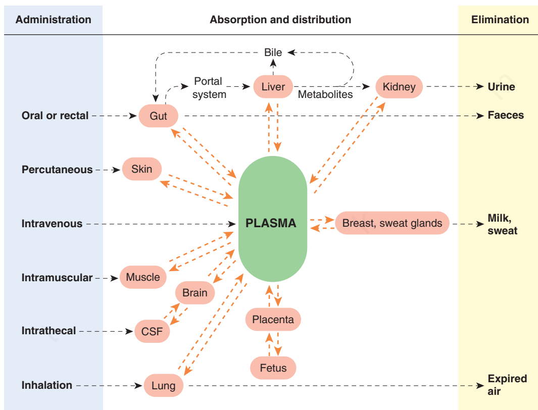
Fig. 9.8 The main routes of drug administration and elimination. CSF, cerebrospinal fluid.
