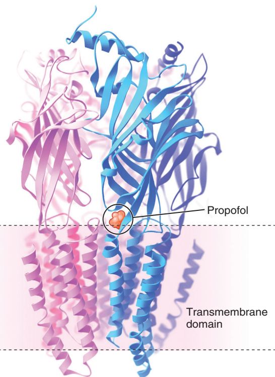
Fig. 42.2 Putative propofol binding site on the \beta subunit of the GABA A receptor. A molecular model showing the approximate binding position of propofol at the interface between the transmembrane domain and the extracellular domain of the \beta subunit. (Based on the original report by Yip et al., 2013. Nat. Chem. Biol. 9, 715–720.)
