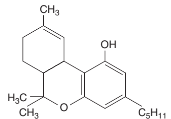
\Delta^9 -Tetrahydrocannabinol (THC)
