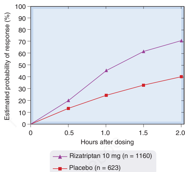
Fig. 16.2 The triptan, rizatriptan, relieves the pain associated with attacks of migraine. The graph is a Kaplan-Meier plot showing the probability of experiencing relief from the pain of the attack after treatment with placebo or with 10 mg rizatriptan. (Modified from Dahlof et al., 1999).
