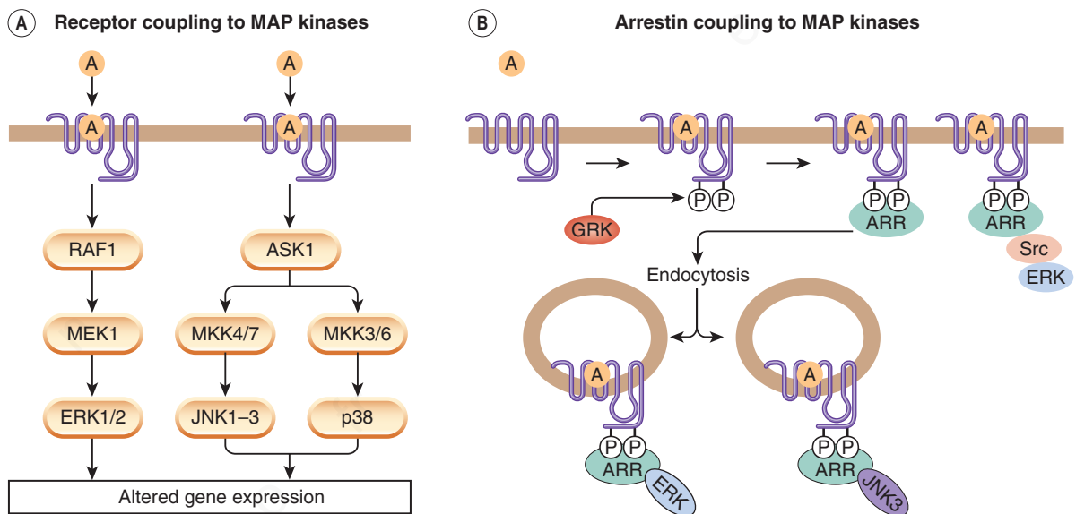
Fig. 3.15 G protein-coupled receptor (GPCR) activation of mitogen-activated protein (MAP) kinase cascade (A) Sequential activation of the multiple components of the MAP kinase cascade. GPCR activation of MAP kinases can involve G\alpha and G\beta\gamma subunits (not shown). (B) Activation of ERK and JNK3 through interaction with arrestins ( \beta ARR). Activation of ERK can occur either at the plasma membrane involving Src, or by direct activation after internalisation of the receptor/arrestin complex. ARR, arrestin; GRK, G protein-coupled receptor kinase.
