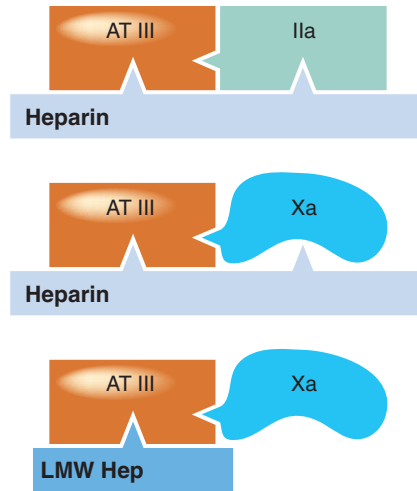
Fig 25.6 Action of heparins. The schematic shows interactions of heparins, antithrombin III (AT III) and clotting factors. To increase the inactivation of thrombin (IIa) by AT III, heparin needs to interact with both substances ( top ), but to speed up its effect on factor Xa it need only interact with AT III ( middle ). Low molecular-weight heparins (LMW Hep) increase the action of AT III on factor Xa ( bottom ), but cannot increase the action of AT III on thrombin because they cannot bind both simultaneously.
