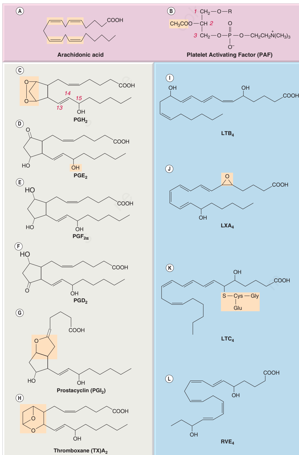
Fig 18.2 Some key lipid mediators involved in the host defence response. (A) Arachidonic acid, an important precursor of prostanoids, leukotrienes and (some) lipoxins and resolvins. Note the conjugated double bonds ( in shaded box ). (B) Platelet-activating factor (PAF); the location of the acetyl group at C2 is shown in the shaded box . R is a 6- or 8-carbon saturated fatty acid attached by an ether linkage to the carbon backbone. (C) Prostaglandin (PG) \text{H}_2 , one of the labile intermediates in the synthesis of prostaglandins; note unstable ring structure ( in shaded box ) which can spontaneously hydrolyse in biological fluids if not enzymatically changed. (D) \text{PGE}_2 , the 15-hydroxyl group ( in shaded box ) is crucial for the biological activity of prostaglandins and its removal is the first step in their inactivation. (E) and (F) \text{PGF}_{2\alpha} and \text{PGD}_2 . (G) Prostacyclin ( \text{PGI}_2 ); note unstable ring structure ( in shaded box ). (H) Thromboxane ( \text{TX})\text{A}_2 ; note unstable oxane structure ( in shaded box ). (I) Leukotriene ( \text{LT})\text{B}_4 . (J) Lipoxin ( \text{LX})\text{A}_4 ; note unstable and highly reactive oxygen bridge structure ( in shaded box ). (K) Leukotriene ( \text{LT})\text{C}_4 ; note conjugated glutathione moiety ( in shaded box ). (L) Resolvin ( \text{Rv})\text{E}_4 .
