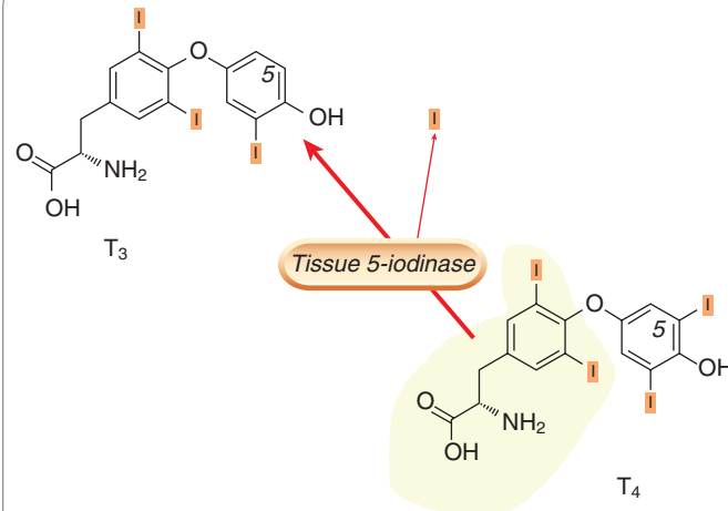
Fig. 35.3 The structures of thyroxine T_3 and T_4 . The position of the iodine residues are indicated in orange. T_4 is converted, in a tissue-specific manner, to the more active species T_3 by mono de-iodination at position 5 of the ring. The basic tyrosine unit is shaded in yellow.
