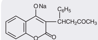
Warfarin (vitamin K antagonist)
