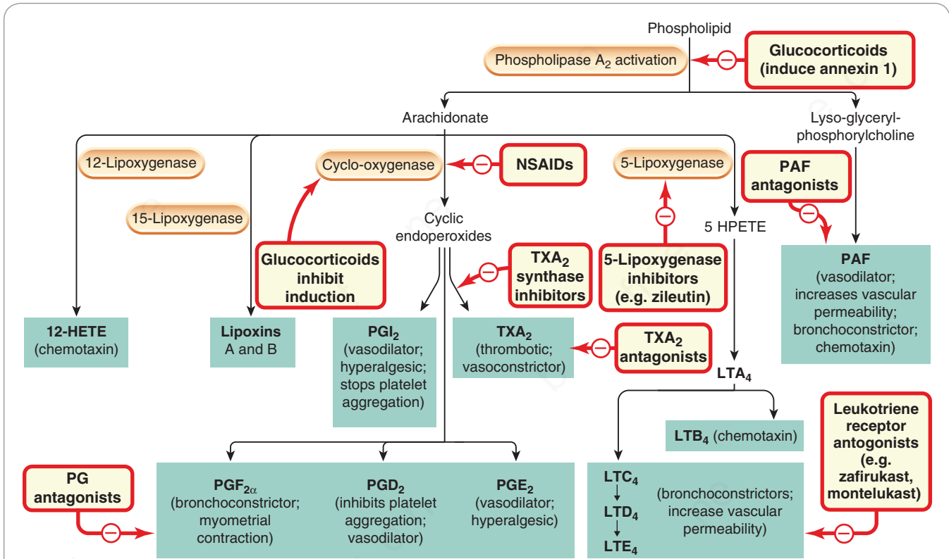
Fig. 18.3 Summary diagram of the inflammatory mediators derived from phospholipids, with an outline of their actions and the sites of action of anti-inflammatory drugs. Arachidonate metabolites are known as eicosanoids. The glucocorticoids inhibit transcription of the gene for cyclo-oxygenase (COX)-2, which is induced in cells by inflammatory mediators and induce and release Annexin A1 which down-regulates phospholipase A 2 activity thereby limiting arachidonate release. The effects of prostaglandin (PG) E2 depend on which of the four receptors it activates. HETE, hydroxyeicosatetraenoic acid; HPETE, hydroperoxyeicosatetraenoic acid; LT, leukotriene; NSAID, non-steroidal anti-inflammatory drug; PAF, platelet-activating factor; PGI 2 , prostacyclin; TX, thromboxane.
