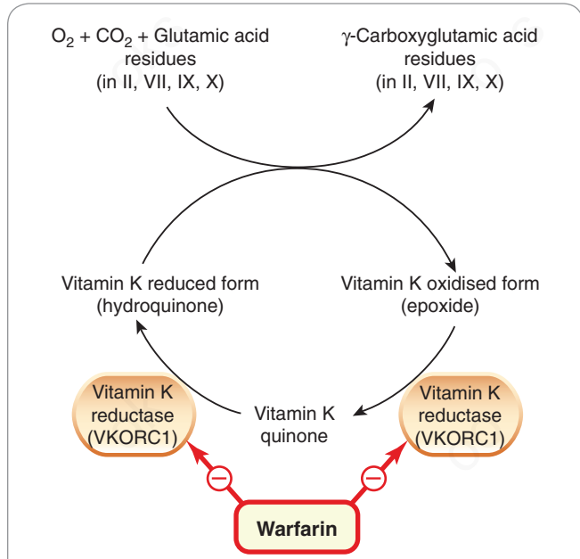
Fig. 25.5 Mechanism of vitamin K and of warfarin. After the peptide chains in clotting factors II, VII, IX and X have been synthesised, reduced vitamin K (the hydroquinone) acts as a co-factor in the conversion of glutamic acid to \gamma -carboxyglutamic acid. During this reaction, the reduced form of vitamin K is converted to the epoxide, which in turn is reduced to the quinone and then the hydroquinone by vitamin K epoxide reductase component 1 (VKORC1), the site of action of warfarin.
