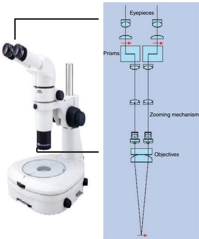
Figure 23.11 Components and optical principles of stereomicroscopes (CMO). Figure reproduced with permission from Nikon Instruments UK.
