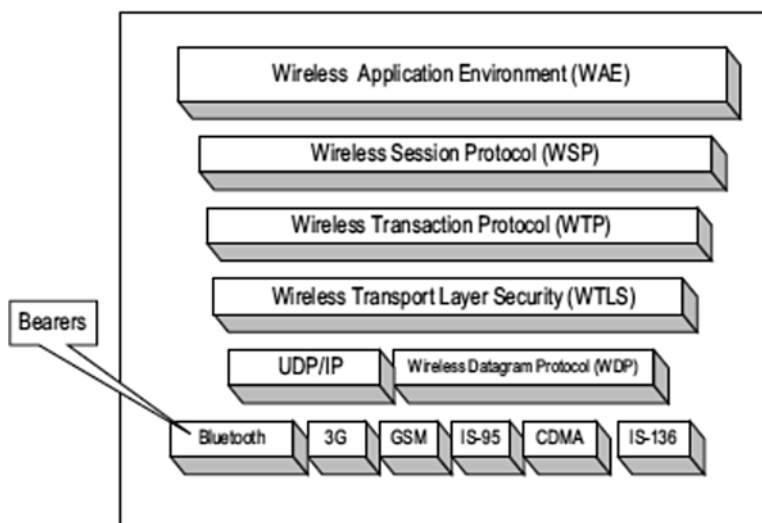
Fig. 18.7 The WAP protocol stack
