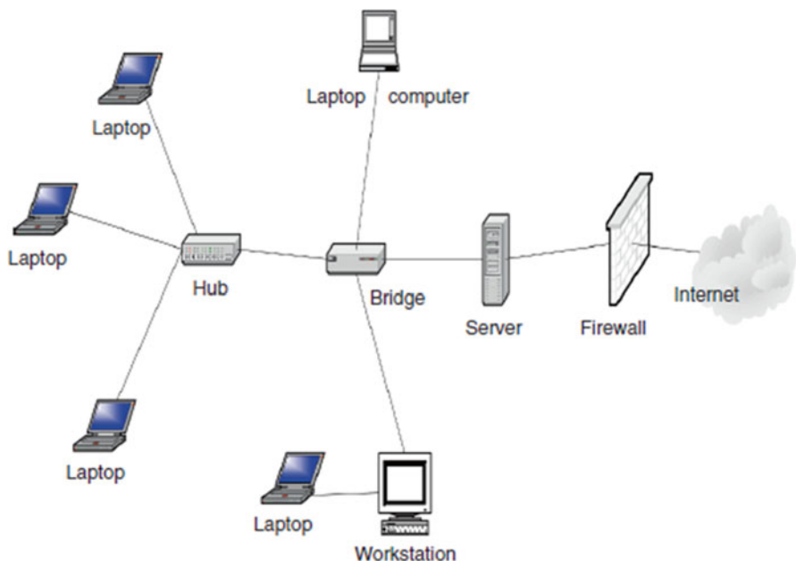
Fig. 1.27 Multi-ported bridge
