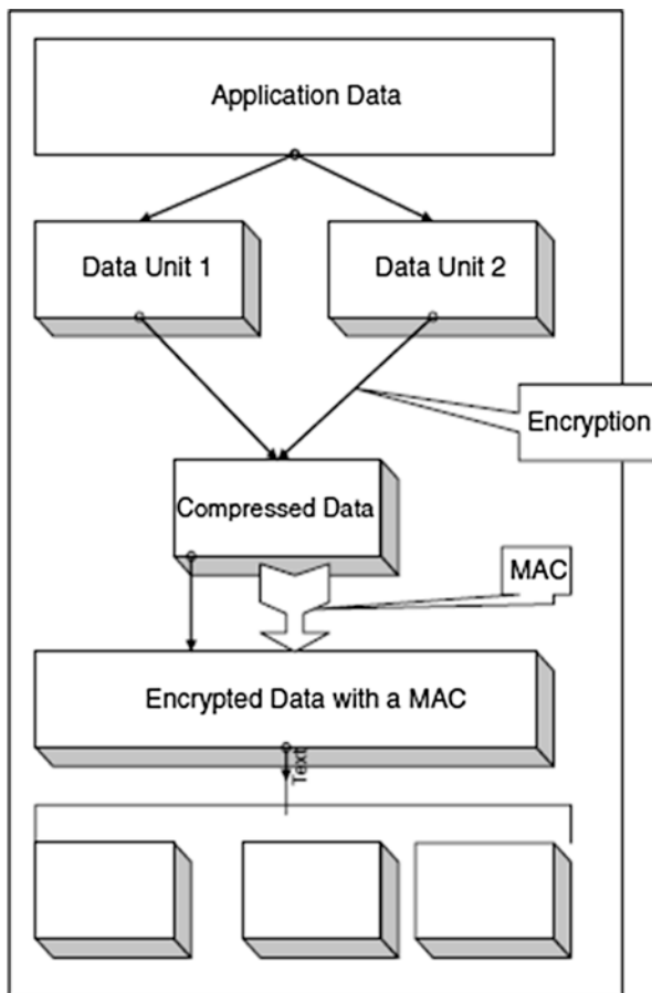
Fig. 17.5 SSL record protocol operation process
