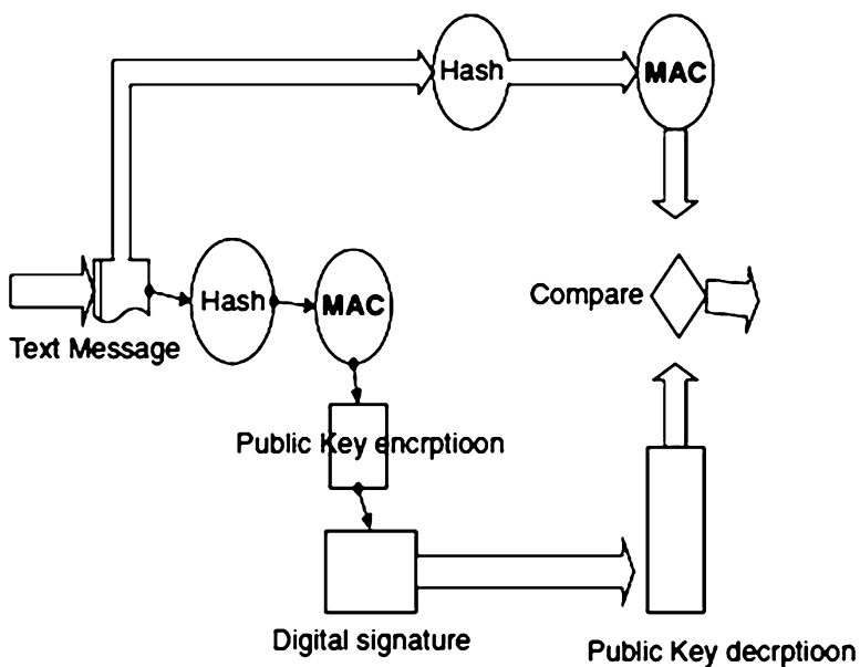
Fig. 11.9 Verifying a digital signature in message authentication
