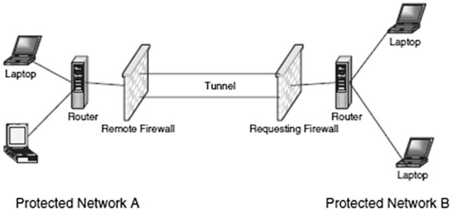
Fig. 17.13 Establishing a VPN using IPSec and IKE
