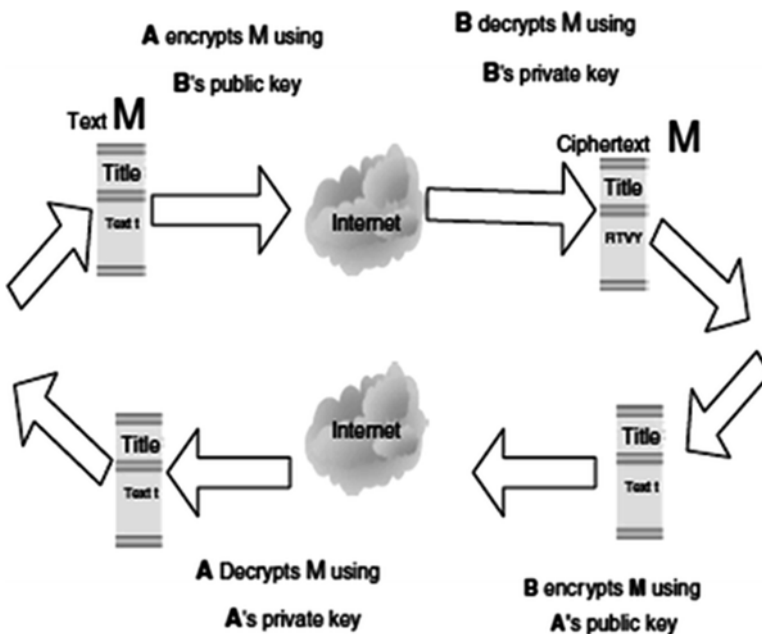
Fig. 11.4 Public-key encryption with data integrity and confidentiality
