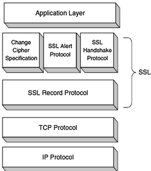
Fig. 17.4 The SSL protocol stack
