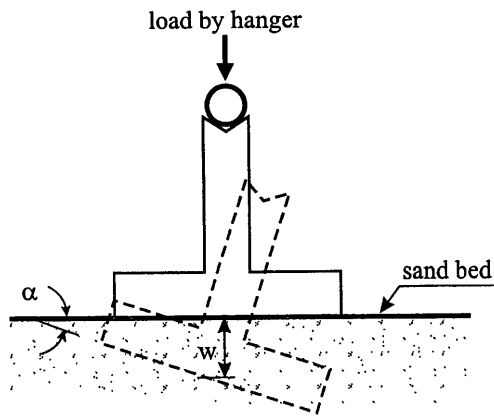
Fig. 7. Set up of the experiments by Edmonds (1993)
