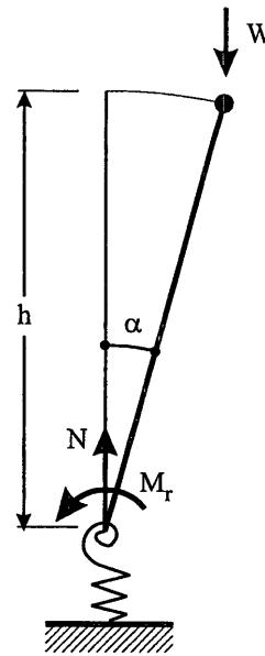
Fig. 13. The inverted pendulum
