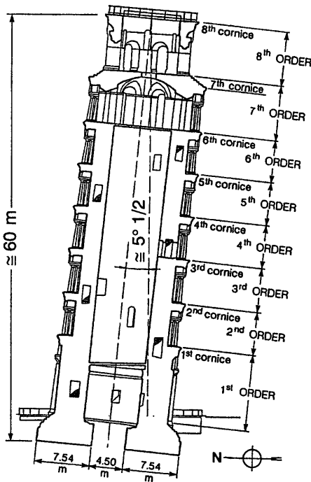
Fig. 1. Cross section of the Leaning Tower of Pisa
