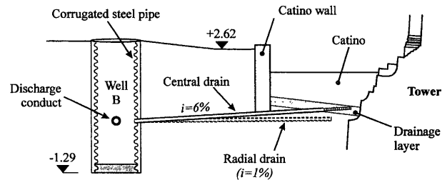
Fig. 42. Control of water table on north side—cross-section
