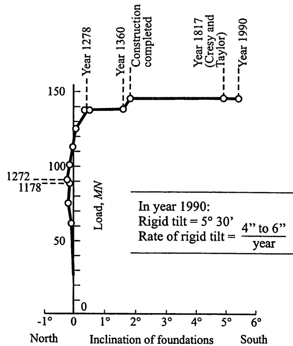
Fig. 6. History of inclination
