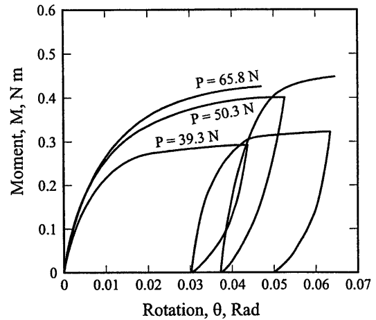
Fig. 18. Centrifuge experiments by Cheney et al. (1991)
