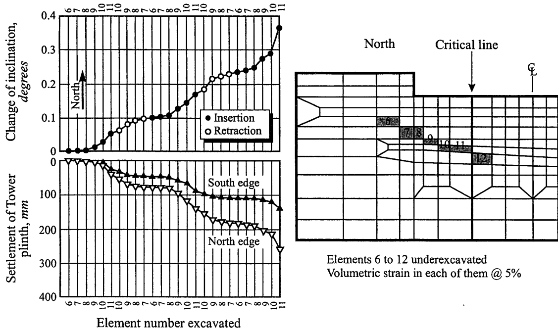
Fig. 23. Finite element simulation of the underexcavation, performed after the history of inclination up to 5% has been simulated
