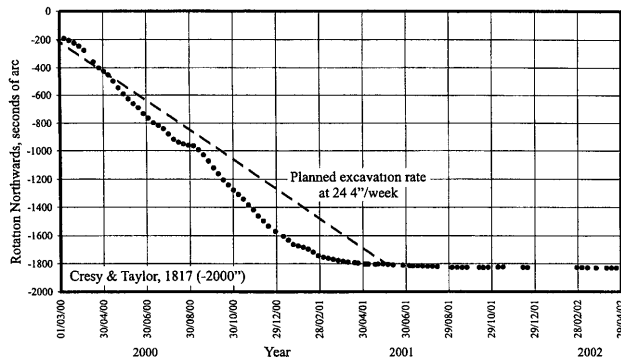
Fig. 38. Results of full underexcavation (2000-2001)
