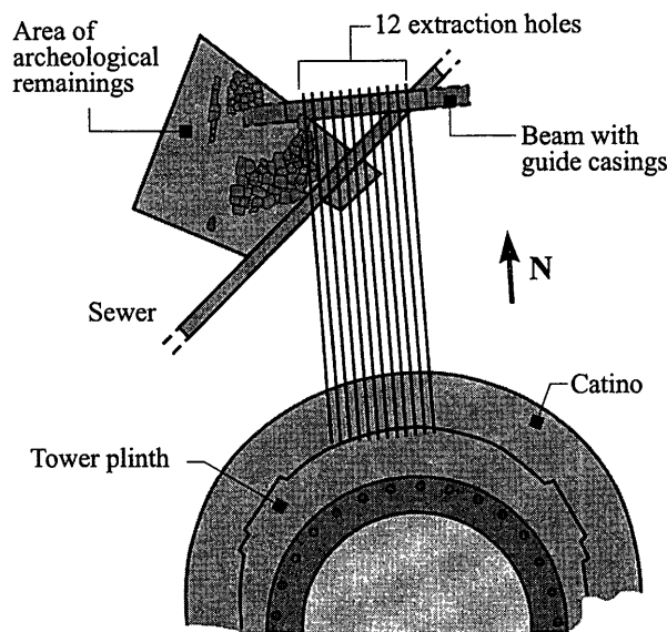
Fig. 29. Holes for the preliminary ground extraction
