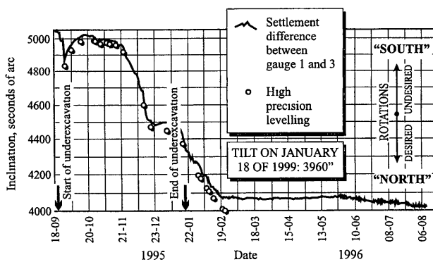
Fig. 28. Result of large scale underexcavation experiment
