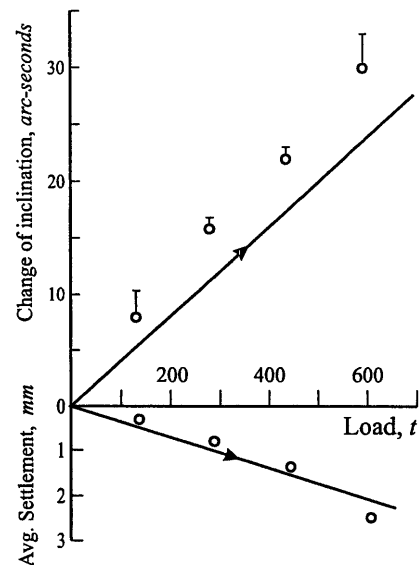
Fig. 20. Comparison between prediction and measurements of changes in inclination and average settlement of the Tower during the application of lead ingots
