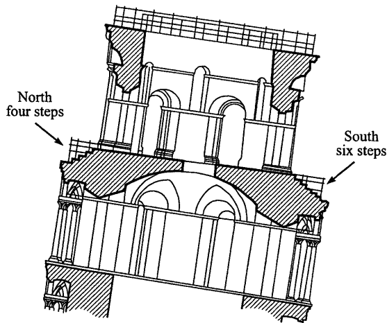
Fig. 4. Detail of the bell chamber
