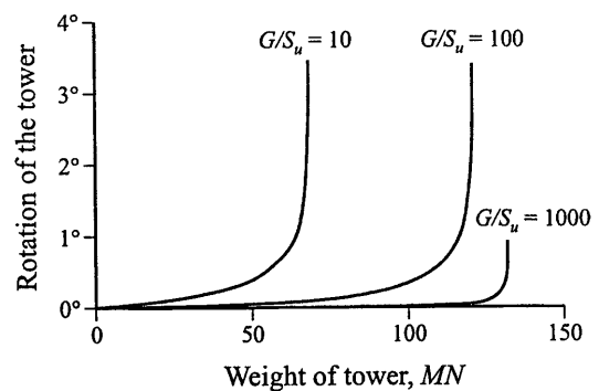
Fig. 10. Load-settlement response of the tower on soft and stiff clay
