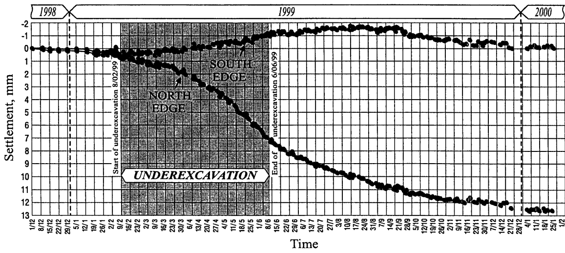
Fig. 32. Results of the preliminary underexcavation
