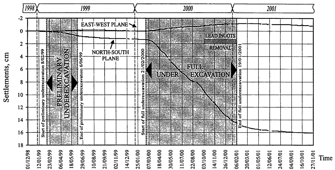
Fig. 37. Results of full underexcavation
