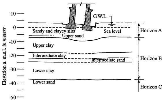
Fig. 2. Subsoil profile
