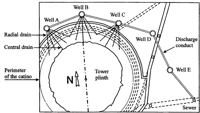
Fig. 41. Control of water table on north side—plane view
