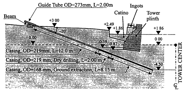
Fig. 36. A hole for full ground extraction
