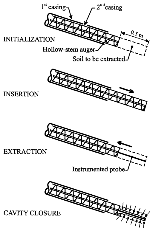
Fig. 26. Drilling technique adopted to remove the soil
