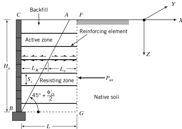
FIGURE 15.30 MSE wall using Rankine's method.
