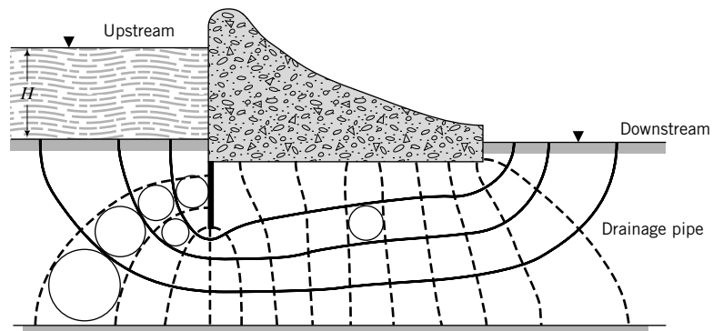
FIGURE 14.4 Flownet under a dam with a cutoff curtain (sheet pile) on the upstream end.
