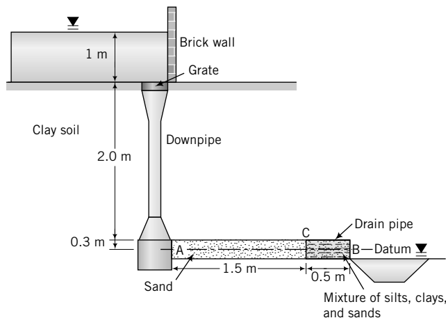
FIGURE E6.3a Illustration of blocked drainage pipe.
