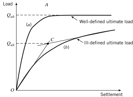
FIGURE 13.12 Load–settlement curves.
