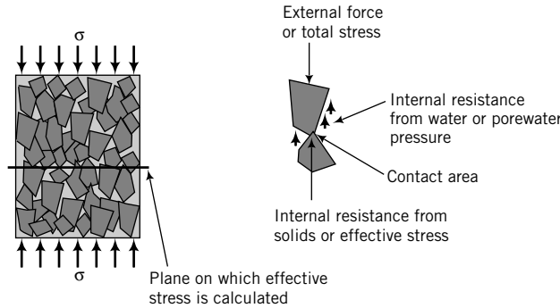
FIGURE 7.14 Effective stress.
