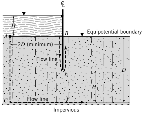
FIGURE 14.8 A sheet pile wall.
