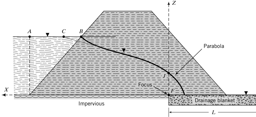
FIGURE 14.11 A horizontal drainage blanket at the toe of an earth dam.
