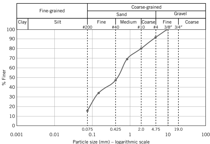
FIGURE E2.1 Grading curve.
