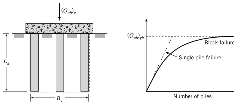
FIGURE 13.18 Block failure mode.
