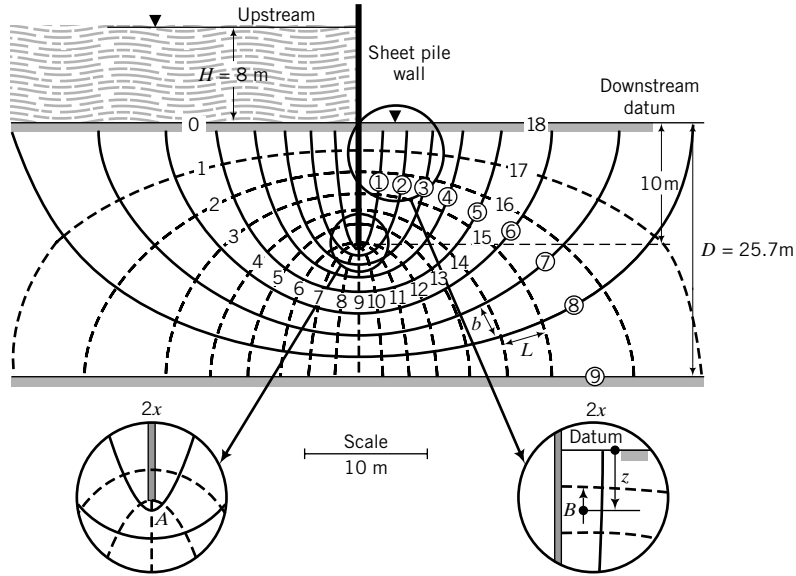
FIGURE 14.3 Flownet for a sheet pile.
