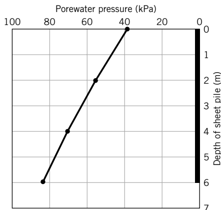
FIGURE E14.3c Porewater pressure distribution.
