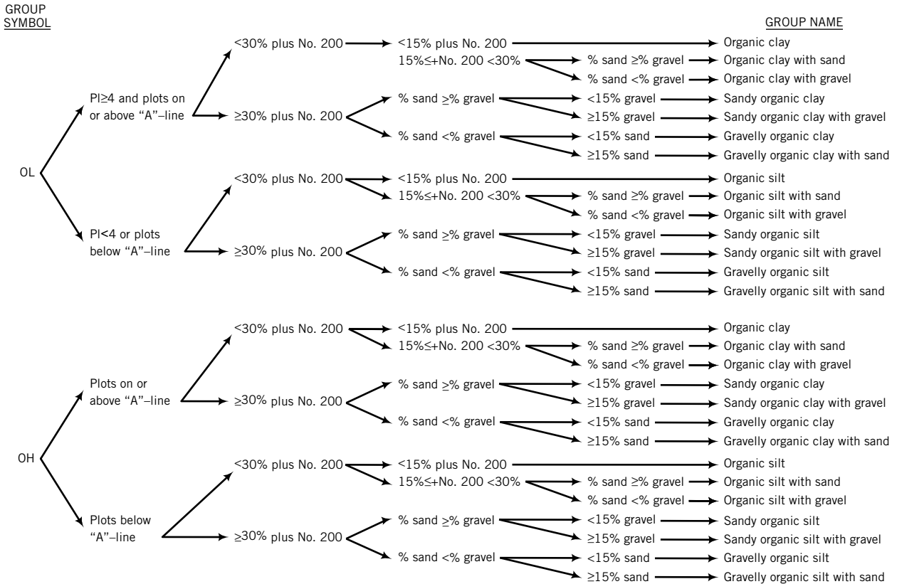
FIGURE 4.10c Flowchart for classifying organic fine-grained soils (50% or more fines). (Source: Reprinted with permission from ASTM D 2487-10 Standard Practice for Classification of Soils for Engineering Purposes, copyright ASTM International, 100 Barr Harbor Drive, West Conshohocken, PA 19428.)
