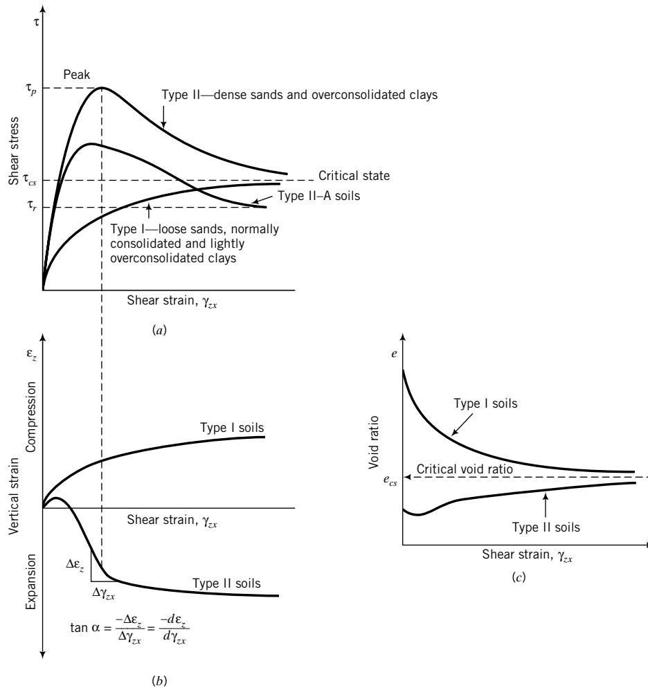
FIGURE 10.3 Response of soils to shearing.
