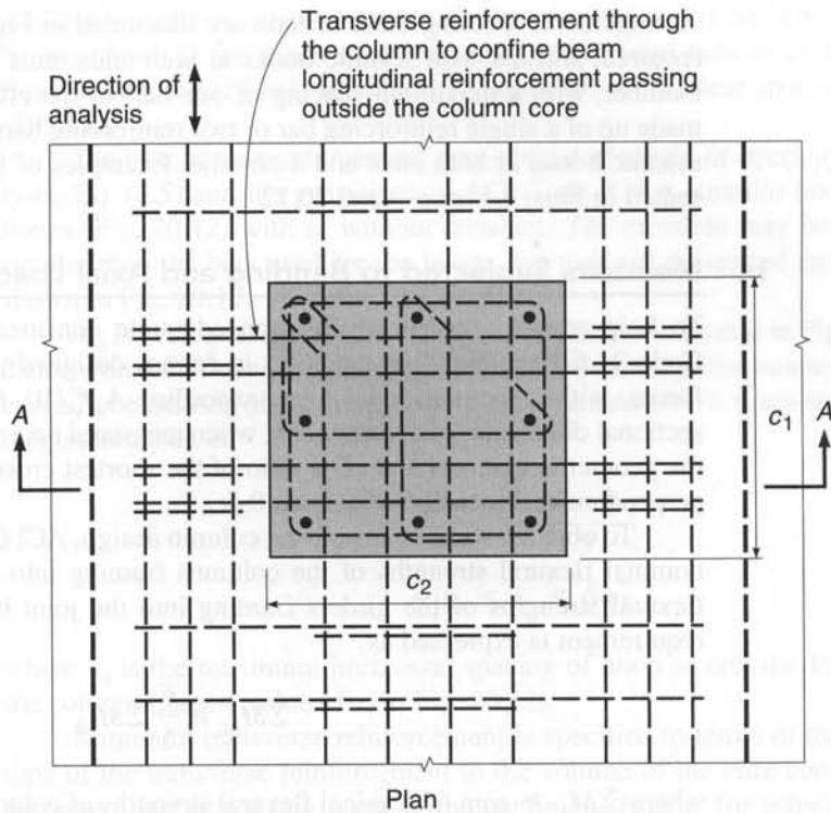
FIGURE 20.13 Maximum effective width of wide beam and required transverse reinforcement. (Adapted from Ref. 20.9.)
