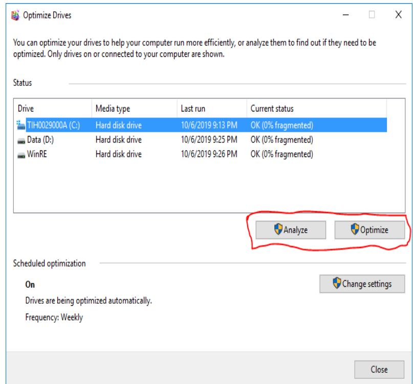
Fig. 1.4 Optimize Drive
