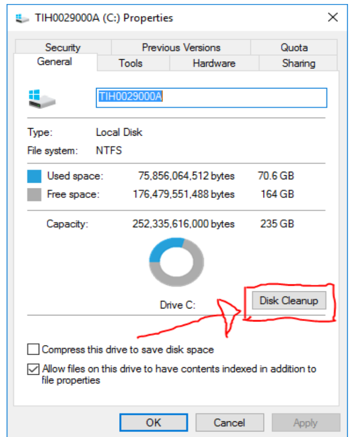
Fig. 1.3 Disk Cleanup
