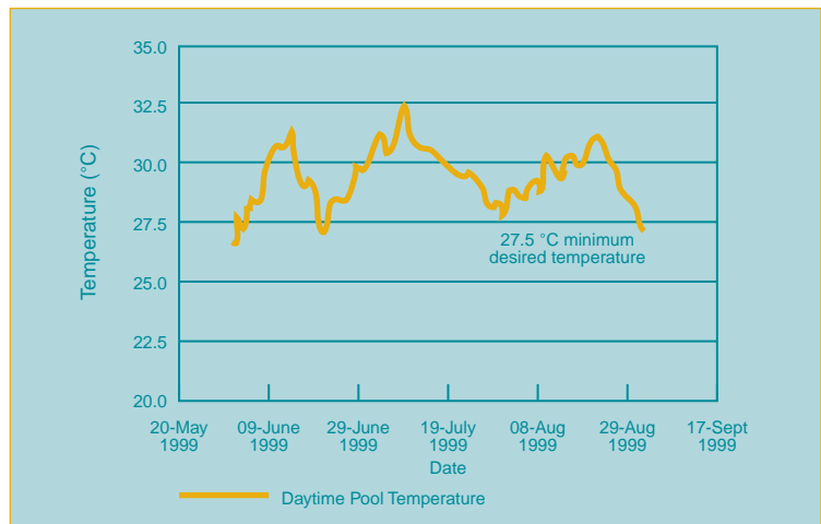
▲ Figure 2. Typical temperature profile for a solar heated pool in Ontario.
