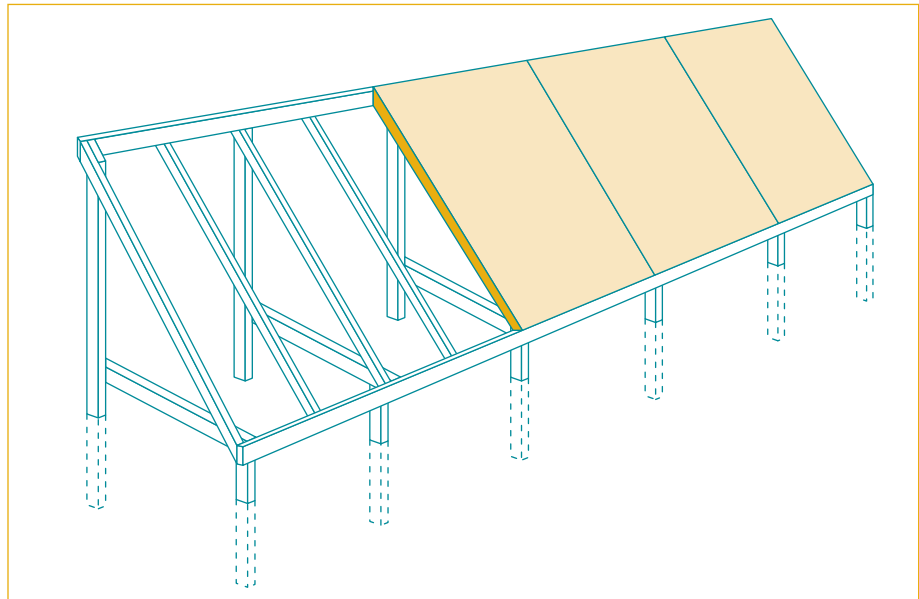
▲ Figure 10. Ground-mounted rack.
