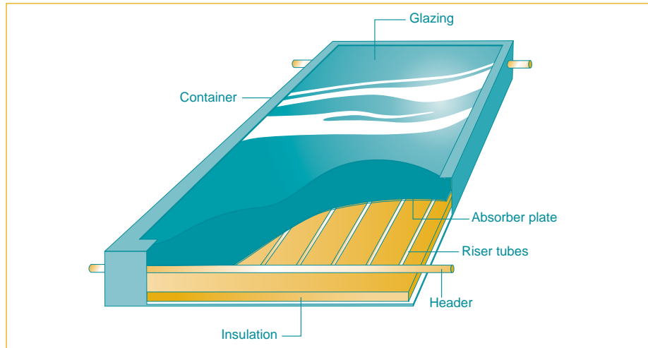
▲ Figure 7. Schematic of a glazed collector.
