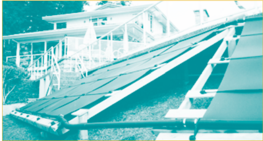
▲ White Rock, British Columbia. Eight 4-m 2 (4-ft. x 10-ft.) solar collectors on a wooden ground rack. Photo courtesy of Taylor Munro Energy Systems.
