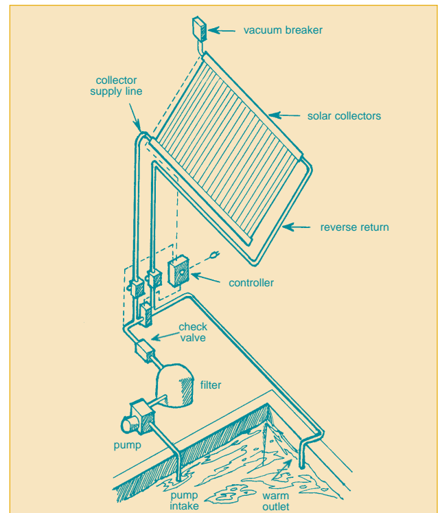
▲ Figure 1. Components of a solar pool heater.
