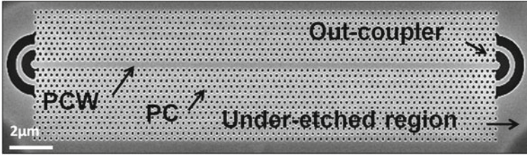
Fig. 3.1 SEM image of a 20 \mu\text{m} W1 PCW end-terminated with out-couplers fabricated from a 130 nm GaAs slab. The lattice constant a = 254 nm and hole radius r = 71 nm
