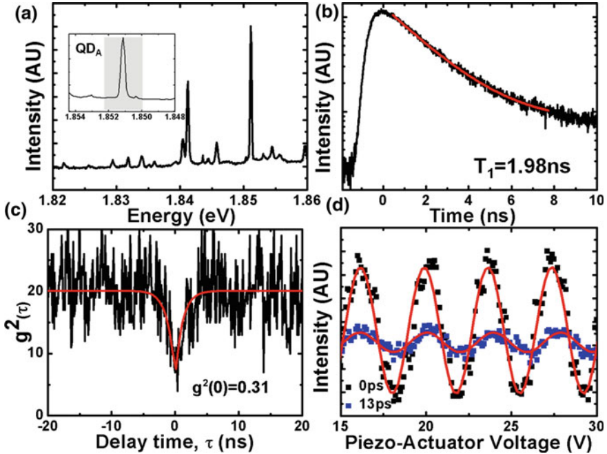
Fig. 6.4 a \mu PL spectra recorded from a typical L3 PC cavity showing InP QD emission. The inset shows a QD line at 1.851 eV (670 nm) used in the following experiments, QD_A , with the grey shaded area showing the spectral window used for interferometry. b Decay transient recorded for QD_A , red line is a monexponential fit to the data with a decay time T_1 = 1.98 ns. c HBT autocorrelation measurement from QD_A with a fitted g^2(0) = 0.31 . d Interference fringe contrast measured as a function of piezo-actuator voltage for path delay 0 ps ( black ) and 13 ps ( blue ) and their respective fits ( red )
