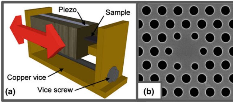
Fig. 7.14 a Schematic diagram of the experimental set-up used to apply a uniaxial strain to the sample. b Scanning electron microscope image of an H1 PC cavity with the optimised parameters for hole size and position employed for the experimental studies
