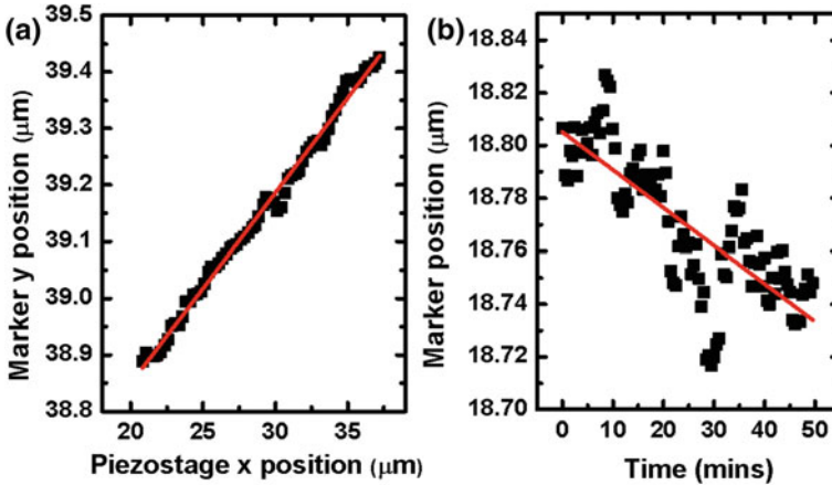
Fig. 7.4 a Linear fit, y = 0.03364x + 38.17 , to the marker position data extracted from the laser reflection map in Fig. 7.3. b The position of a marker relative to the piezostage as a function of time. A linear fit, y = -0.00144x + 18.805 , estimates the drift of the set up to be approximately 1.4 nm/min
