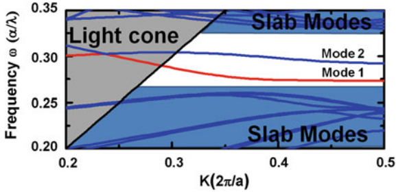
Fig. 3.2 A band diagram calculated using MPB for a W1 GaAs PCW with r/a = 0.28 . The mode 1 (red) indicates the first guided mode studied in this chapter. The light line, w = ck and light cone are shaded grey whilst other modes not localised to the PCW or outside the photonic bandgap are labelled slab modes and shaded blue
