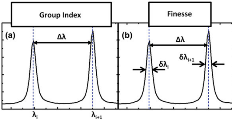
Fig. 3.5 Example of how the properties of the FP fringes are used to calculate a the group index of the guided mode and b finesse of the FP cavity
