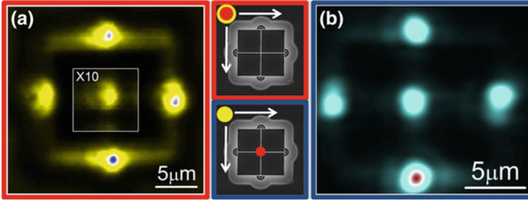
Fig. 4.7 PL intensity maps, integrated over the QD distribution, recorded from the crossed waveguide device, by a scanning the collection fiber and excitation laser together across the structure as shown schematically in the inset ( red border ) and b scanning the collection fiber with the excitation laser fixed at the intersection as shown in the inset ( blue border )
