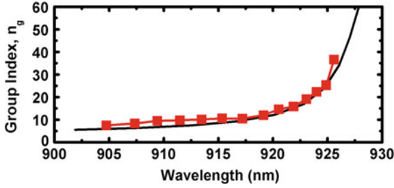
Fig. 3.6 Comparison of group index extracted from analysis of FP resonances shown in Sect. 3.8 (red) and extracted from MPB simulations (black)
