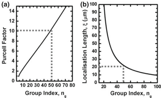
Fig. 3.13 a Calculated Purcell factors as a function of group index for the W1 PCW. For a Purcell factor of 10 it is shown that a group index of 50 is required, which is shown to restrict the localisation length to 20 \mu\text{m} , by the dashed grey line . b Localisation length, \xi extrapolated from the value of \alpha extracted on Fig. 3.12 where \xi = \frac{\ln(1/e)}{\alpha}
