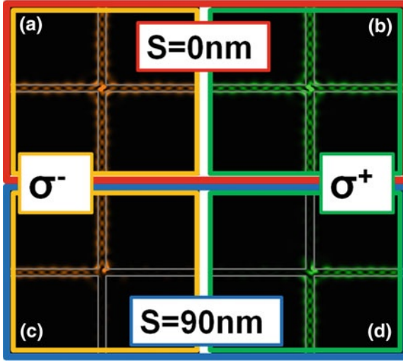
Fig. 5.8 Electric field intensity, |E|^2 at the centre of the waveguides for different source locations and polarisations 0.65 ps after the CW source begins to emit. a \sigma^- polarised source located at centre. b \sigma^+ polarised source located at centre. c \sigma^- polarised source located off-centre at s = 90 nm. d \sigma^+ polarised source located off-centre at s = 90 nm
