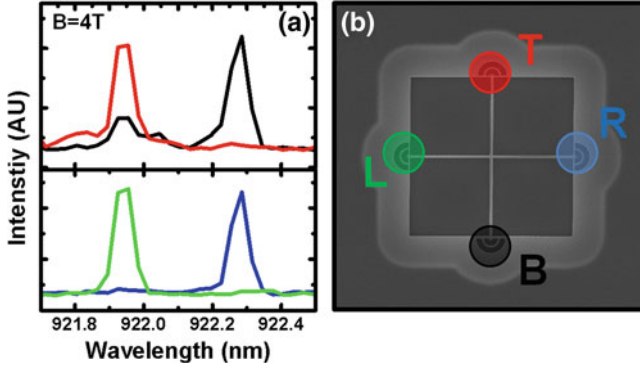
Fig. 5.1 a PL spectra of a Zeeman split QD doublet ( B = 3T ) recorded from the colour coded out-couplers on a crossed waveguide structure schematically represented in b
