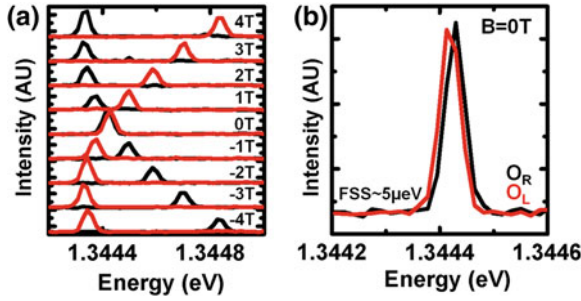
Fig. 5.2 a B-field dependent spectra recorded from outcouplers O_R (black) and O_L (red), in the range B = -4T to B = 4T . At B = 0T the spectra is displayed again in b . The two transitions have a fine structure splitting of \sim 5 \mu\text{eV}
