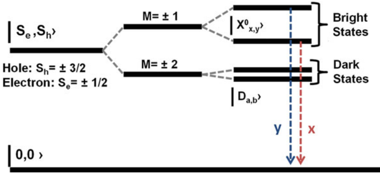
Fig. 1.5 Energy level scheme of the eigenstate splitting for a neutral exciton. With spins, S , and total angular momentum projection for the states, M , bright and dark manifolds |X^0_{x,y}\rangle , |D_{a,b}\rangle and the orthogonally linearly polarised emission Y , X are labelled
