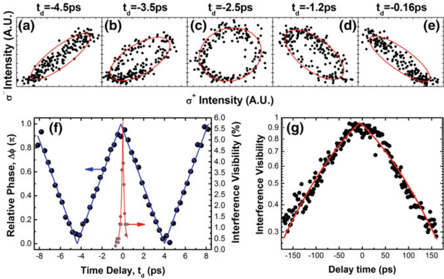
Fig. 4.4 a–e Intensity plots of right and left circularly polarised states interfered simultaneously on two detectors. f Plot of relative phase between the two transitions as the path delay in one arm of the MZI is varied. The line shows a triangular waveform fit to the data. g Coherence measurement of the \sigma^+ transition using Fourier transform spectroscopy, a linewidth of 12.8 \mu\text{eV} ( \sim 150 ps) is extracted
