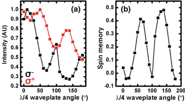
Fig. 5.12 a Intensity of the \sigma^+ (red), \sigma^- (black) Zeeman split ( B = 3T ) QD transitions studied in Device-B as the polarisation of the 850nm excitation laser is modified by the rotation of a \lambda/4 waveplate in the excitation path. The PL from the QD transitions is collected from the same position as the excitation at the centre of the waveguide intersection. b The Spin memory S = (I_{\sigma^+} - I_{\sigma^-}) / (I_{\sigma^+} + I_{\sigma^-}) of the \sigma^+ , \sigma^- transitions as a function of the waveplate angle
