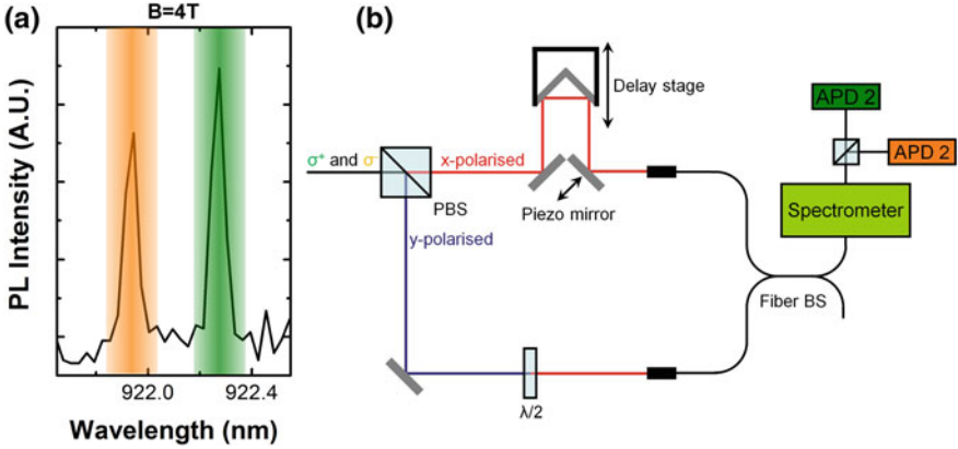
Fig. 4.2 a \mu PL spectrum showing the Zeeman split transitions of a single QD with an applied magnetic field, B = 4T . The shaded regions, orange and green indicate the spectral window collected on the two colour coded APDs, orange ( \sigma^- ) and green ( \sigma^+ ). b Experimental set-up used to demonstrate polarisation to which path interface using bulk optics
