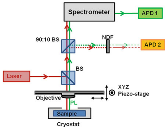
Fig. 7.2 Schematic diagram of the experimental set-up used to register QDs
