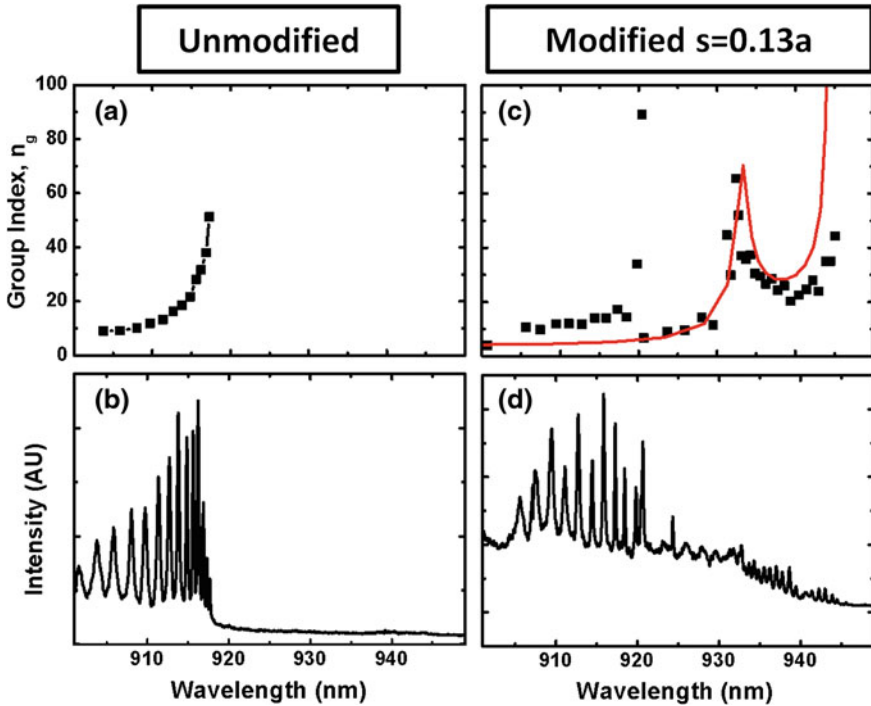
Fig. 3.17 Displays the comparison between the PL, (b), and group index, (a), extracted from an unmodified PCW and the PL (d) and group index (c) from an engineered PCW with transverse hole shifts of 0.13a . The solid red line in (c) is the expected group index extracted from simulation. Deviations from the simulation below 920 nm are due to the second guided mode crossing the guide mode of interest which is not included in the simulations
