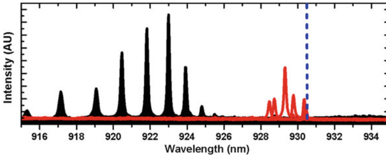
Fig. 3.8 \mu PL spectra recorded from a 20 \mu m PCW when the laser excitation spot is positioned at the centre of the PCW and the PL is collected from an out-coupler ( solid black trace ) and when the \mu PL spectra is recorded for a number of positions above the PCW as the excitation and collection spots are scanned simultaneously along the PCW ( red ). A number of distinctive features appear at localised positions. The waveguide band edge extracted from the simulations is superimposed for reference ( blue dash )
