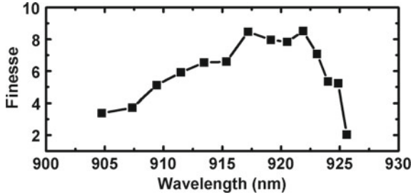
Fig. 3.7 Finesse of the Fabry-Perot (FP) resonances observed from an out-coupler as shown in Fig. 3.8, where F = \Delta\lambda_i/\delta\lambda_i as defined in Fig. 3.5
