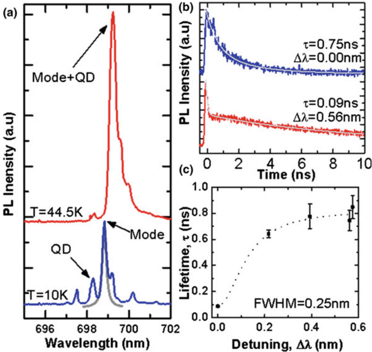
Fig. 6.3 a Photoluminescence spectra of a weakly coupled QD-cavity system recorded at 10 and 44.5 K. Light gray line shows a Lorentzian fit to the cavity mode resonance at 10 K, with Q = 3,300 and \text{FWHM} = 0.21 nm. b Decay transients recorded from the QD at 10 K ( \Delta\lambda = 0.56 nm) and 44.5 K ( \Delta\lambda = 0 nm). c Measured QD lifetime as a function of QD-cavity mode detuning. Dashed line shows Lorentzian fit, with \text{FWHM} = 0.25 nm
