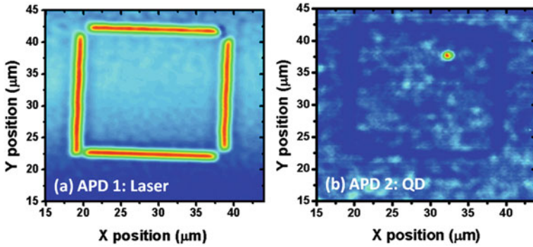
Fig. 7.3 a Intensity map of the 633 nm laser reflections from of a marker set with 120 \times 120 data points. b PL intensity map of QD emission from the same marker set with 120 \times 120 data points
