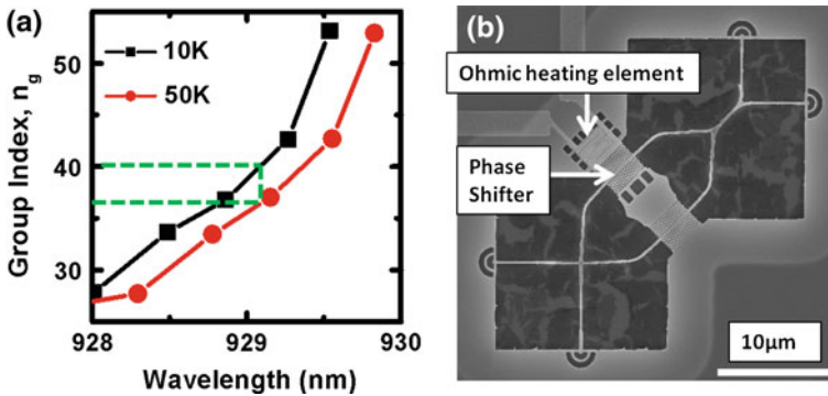
Fig. 3.16 a Close up of the temperature dependant group index at 929 nm from 10 K (black) to 50 K (red), displaying a change in group index of 4 at this wavelength (green dash). b SEM image of a prototype quantum optical circuit that incorporates an on-chip PCW phase shifter
