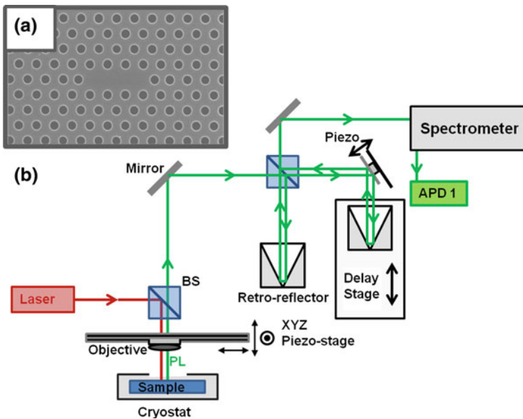
Fig. 6.1 a SEM image of an L3 type photonic crystal cavity used in these experiments. b Experimental set-up of the \mu\text{PL} and Michelson interferometer system
