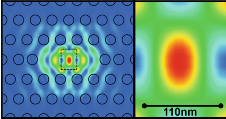
Fig. 7.1 The electric field profile for the fundamental mode of an L3 type cavity with a lattice period a = 187 nm, hole radius r = 0.3a and end hole shift s = 0.18 calculated with finite difference time domain (FDTD) analysis. A Blue-Red scale is used such that red colours represent areas of high electric field or antinodes, and the blue colours are of low field, nodes. The central antinode can be seen as the red dot with an approximate spatial diameter of 50 nm
