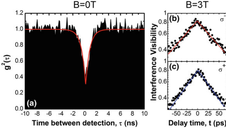
Fig. 4.9 a Photon correlation histogram of the QD transition at B = 0T using a Hanbury-Brown and Twiss set-up. The red-line shows a fit to the data of the function g^{(2)}(\tau) = (1 - (1 - M)e^{(-|\tau|/\tau_d)}) , where M = 0.28 is the multi-photon emission probability and \tau_d = 0.76 ns is the lifetime of the QD. Coherence time measurements of the \sigma^- (b), and \sigma^+ (c), transitions respectively. The solid red and blue lines show fits to the data following Ref. [23]
