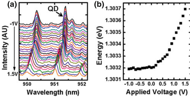
Fig. 7.10 a QD PL emission as a function of applied voltage. b Energy of the PL emission labelled QD in figure (a) as the externally applied voltage across a P-I-N diode is varied between -1 and 1.5 V. A maximum Stark shift of 0.5 meV is observed
