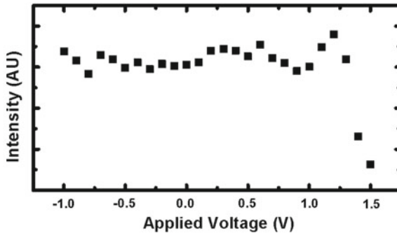
Fig. 7.12 Intensity of the emission line labelled QD in Fig. 7.10a as the applied voltage is varied between -1 and 1.5 V. There is little change in the emission intensity of around 2,000 counts for voltages below 1 V before the electrical turn on of the diode is reached at which point the intensity rapidly decreases
