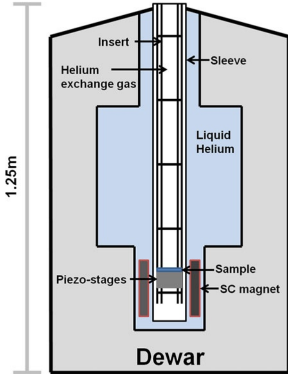
Fig. 2.5 Schematic diagram of a helium bath cryostat
