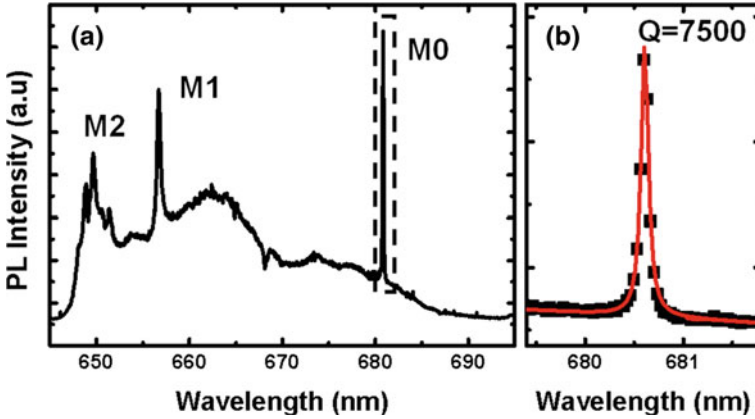
Fig. 6.2 a \mu PL spectra recorded from a typical GaInP L3 PC, showing emission from InP QD ensemble (650–685 nm) and cavity modes. b Fundamental mode emission of cavity with quality factor of \sim 7,500
