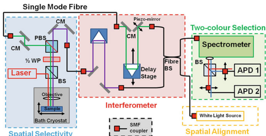
Fig. 2.8 Schematic diagram of the experimental set-up used to provide two-colour, spatially selective collection and interference measurements. The four subsections of the functionality required in the measurement are highlighted with coloured boxes for visual reference and to emphasise that the subsections can be individually incorporated into other experimental set-ups as required
