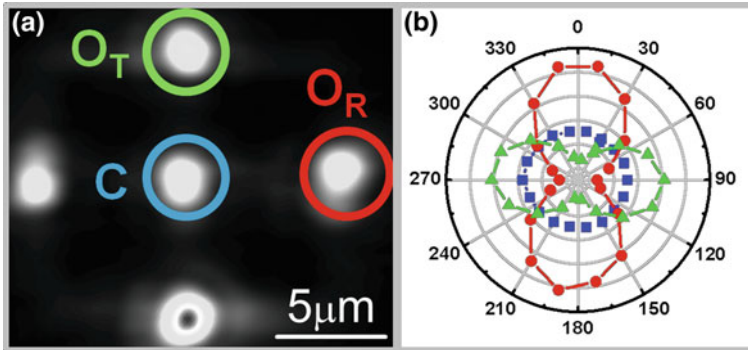
Fig. 4.8 a The PL map from Fig. 4.7b is used here to mark the three areas of strong emission: the crossed waveguide intersection ( C (blue)) and two orthogonal out-couplers ( O T (green) and O R (red)), from which polarisation dependent collection measurements are taken. b The two out couplers are strongly linearly polarised, orthogonal to one another, whilst PL from intersection is unpolarised
