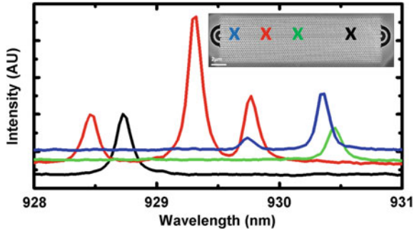
Fig. 3.9 PL spectra of Anderson modes observed at four colour coded positions marked on the SEM image of the PCW inset
