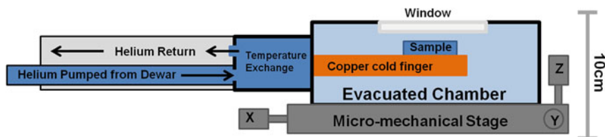
Fig. 2.4 Schematic diagram of a cold finger continuous flow helium cryostat
