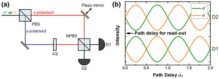
Fig. 4.1 Shows the principle of operation of the polarisation to which path interface. a Mach-Zehnder Interferometer comprised of one polarising beam splitter (PBS), one non-polarising beam splitter (NPBS), half wave plate ( \lambda/2 ) and two detectors (D1 and D2). b Interference fringes recorded on D1 and D2 as the path delay in one arm of the MZI is modulated using a piezo controlled mirror
