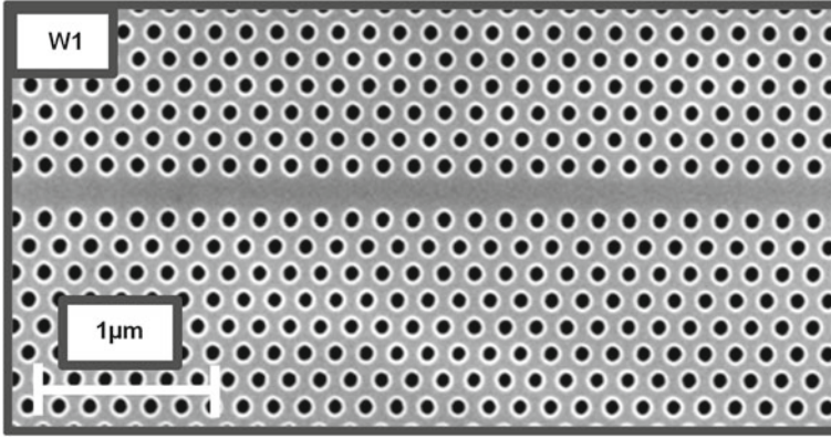
Fig. 1.3 SEM image of an W1 type photonic crystal waveguide. With the etched air holes and the waveguide formed by the omission of a single row of air holes
