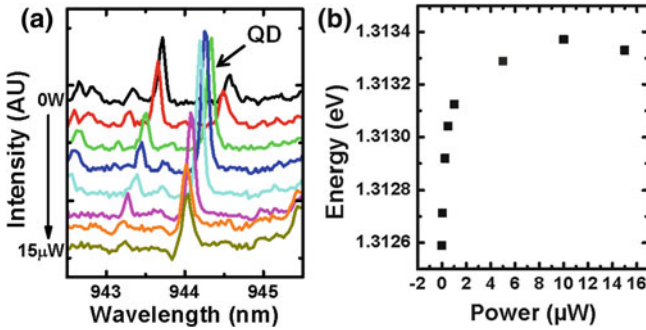
Fig. 7.11 a PL emission from a photonic crystal P-I-N diode structure under resonant and above bandgap excitation. As the power of the above bandgap excitation increases charged photogenerated carriers screen the internal field and induce a Stark Shift. b Energy of quantum dot emission labelled QD in figure (a) as a function of the incident HeNe laser power a Stark Shift of 0.8 meV is observed
