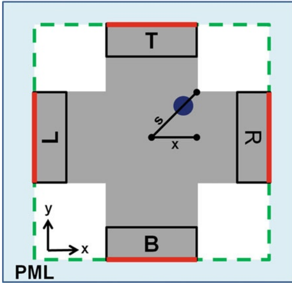
Fig. 5.5 Schematic diagram of the computational area of the waveguide intersection used in the FDTD simulations. The source is indicated by a blue dot and is located within the waveguide intersection at a position along a direction, s , diagonal from the centre or x , orthogonal to the y direction waveguide. The planes over which the Poynting vector is integrated to determine the power coupled into the waveguides are coloured red . The green dashed line represented the planes around the computational cell on the boundary with the perfectly matched layer (PML) over which the Poynting vector is integrated to determine the total power output of the source
