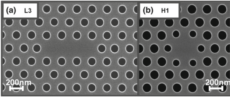
Fig. 1.2 SEM images of (a) L3 and (b) H1 type photonic crystal cavities. With the etched air holes and the cavity formed by the omission of three and one air holes respectively
