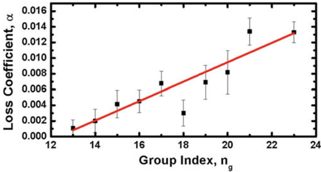
Fig. 3.12 Loss coefficient, \alpha , taken from the data of reflectivity rounded to nearest group index fitted with R = R'e^{-\alpha l} for each value of group index. A linear function, An_g + B , is fitted and parameters A = 12(\pm 2) \times 10^{-4} \text{ nm}^{-1} and B = -15(\pm 3) \times 10^{-3} \text{ nm}^{-1} extracted
