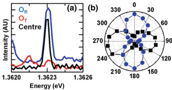
Fig. 4.11 a \mu PL spectra recorded from the crossed waveguide intersection, Centre (black), and two orthogonal out-couplers O_T (red) and O_R (blue). b Intensity of the QD transition shown in a with polarisation dependent detection from the Centre and O_R . The transition is cross polarised between the Centre and O_R whilst not being visible from O_T . This is consistent with a QD coupled to only one waveguide when located off centre and not in the intersection
