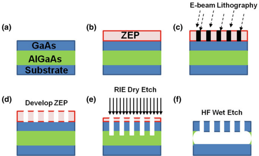
Fig. 2.2 Schematic of the fabrication process used to create air-bridged photonic crystal cavities and similar under-etched structures. a A sample containing an AlGaAs sacrificial layer, b ZEP 520 A positive resist is spun onto the sample. c The pattern is written into the resist by exposure using E-beam lithography. d The pattern is developed using a Xylene developer. e The pattern is transferred to the sample by etching down to the sacrificial layer using an RIE. f Sacrificial AlGaAs is selectively wet etched with HF, leaving the under-etched photonic crystal structure
