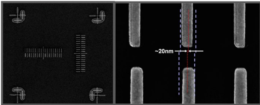
Fig. 7.7 SEM image of the alignment test markers to determine the accuracy of the electron beam lithography. Alignment guides and approximate offset is labelled. The shadowing is caused by a double evaporation process
