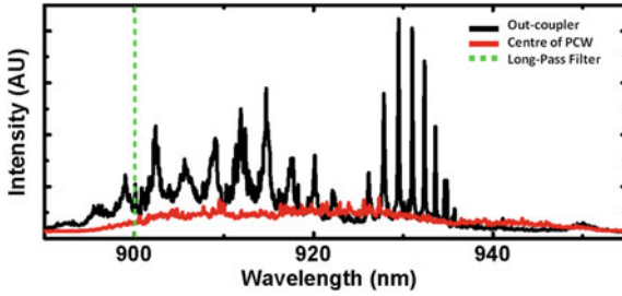
Fig. 3.4 \mu PL spectra recorded from a 20 \mu m PCW when laser excitation spot is positioned at the centre of the PCW and the light is collected from an out-coupler ( solid black trace ) and the point of excitation ( red ). The 900 nm long-pass filter edge is superimposed for reference ( green dash ). FP type resonances are observed from the outcoupler but not from the centre of the waveguide, where only emission from the QD ensemble is collected
