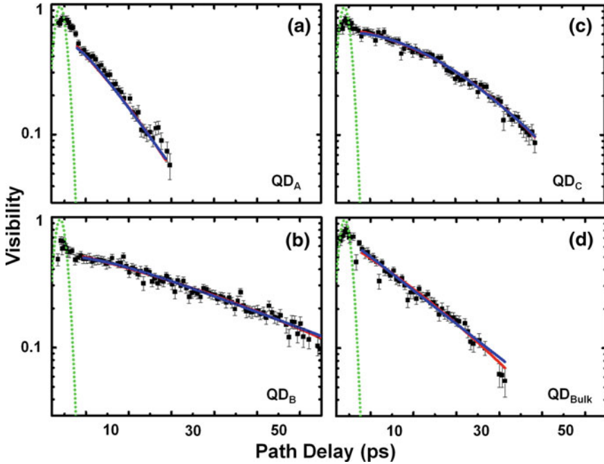
Fig. 6.5 Semi-log interference visibility traces for three QD transitions a QD_A b QD_B and c QD_C located in a photonic crystal cavity and a QD transition taken from an unpatterned area of the sample, d QD_{Bulk} . The data sets have been fitted with function C_1(t) (Blue) and C_2(t) (Red). The dashed green line represents the system response function for incoherent light obtained from white light illumination
