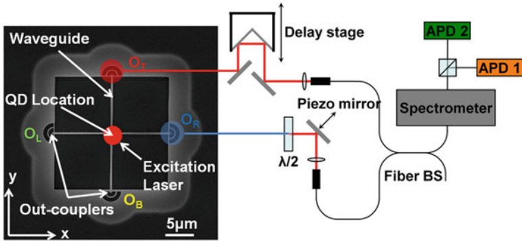
Fig. 4.6 Schematic diagram of the optical set-up used for the self interference of the two Zeeman split QD transitions. Spatially selective collection spots positioned in the sample plane collect PL from orthogonal out-couplers O_T and O_R . PL is excited by a laser at the positioned at the intersection. The two optical collection paths are recombined by a single mode fiber beam-splitter, ensuring good spatial overlap of the modes. Interference fringes are recorded for each QD transition on separate APDs having been isolated in energy by the spectrometer. The path length is modulated by a piezo-actuated mirror and motorised delay stage
