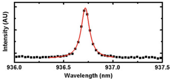
Fig. 3.10 PL spectra of an Anderson mode with a spectrometer resolution limited Q-factor of 9,300
