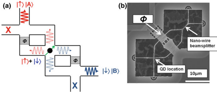
Fig. 8.1 A schematic diagram of an on-chip spin-photon entangler for photons to be used as inputs into a linear optical circuit. In the case of where the QD is located as in Device-B, the O_T , O_L and O_B , O_R waveguide arms may be combined using a standard Mach-Zehnder type device, where the \Phi box represents a tunable phase shift. The output may be tuned such that the photon component is emitted out of one arm only. What results is two photon paths that may be fed into a typical linear-optical circuit. (b) SEM image of a prototype quantum optical circuit that shares similar geometry to the schematic in (a) with the incorporation of an on-chip PCW phase shifter and beamsplitter into the O_B , O_R output arms of a crossed waveguide device
