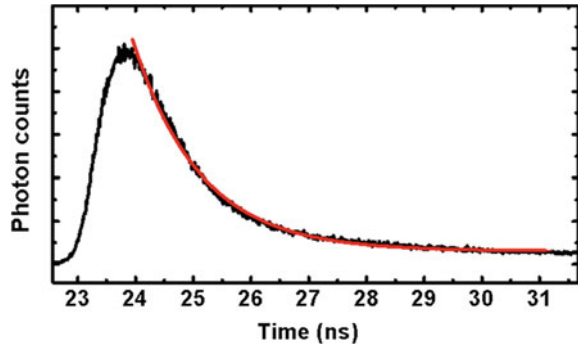
Fig. 2.6 Decay transient of detection events recorded on an APD as a function of time for a single InAs QD excited with a pulsed laser. The decay curve is fitted with a single exponential decay that reveals the lifetime of the QD to be 1.2 ns
