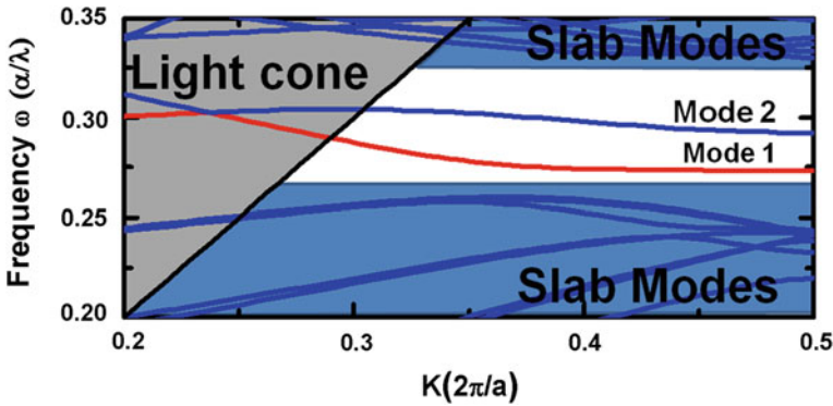
Fig. 1.4 A band diagram calculated using MPB for a W1 GaAs PCW with r/a = 0.28 . The mode 1 ( red ) indicates the first guided mode studied in this chapter. The light line \omega = ck and light cone are shaded grey whilst other modes not localised to the PCW or outside the bandgap are labelled slab modes and shaded blue
