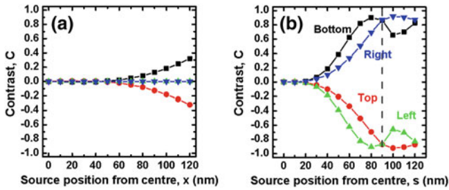
Fig. 5.7 Calculated contrast, ( C_\alpha = (I_+ - I_-)/(I_+ + I_-) , where \alpha = T, B, R, L ) between coupling of \sigma^+ and \sigma^- polarised light to the four waveguides as the position of the source is moved a horizontally along x and b diagonally along s . The dotted line at s = 90 nm indicates the inferred position of the QD in device-B
