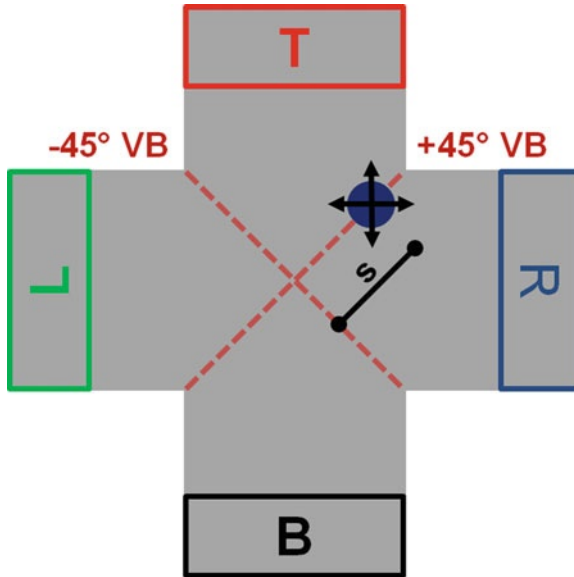
Fig. 5.9 The quantum dot is positioned a distance s from the centre along the diagonal. The intersection acts like a superposition of two 50:50 beam-splitters along the \pm 45^\circ directions
