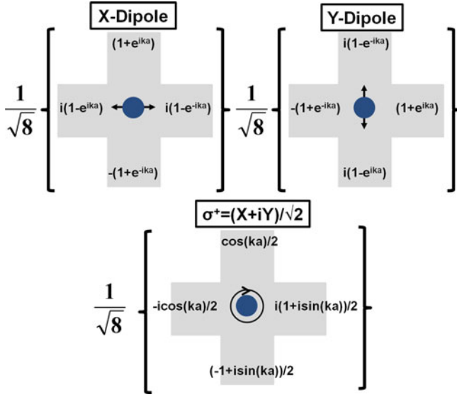
Fig. 5.11 ( x -, y -Dipoles) These diagrams give the amplitudes of the output ports for the QD with \hat{x} - and \hat{y} - polarised optical dipoles respectively. The diagrams are mapped by a reflection about the +45^\circ axis. Note that in the case where the dot is at the centre, ka = 0 , the x -polarised emission exits by the top and bottom waveguides only, as observed for Device-A. ( \sigma^+ ) This gives the amplitudes of the output ports in the case of a \sigma^+ polarised optical dipole. This is found from an interference of an x and iy -polarised dipole. In the case where ka = \pi/2 the light exits from the right and bottom ports only, as observed for Device-B
