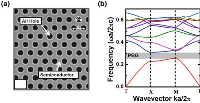
Fig. 1.1 a Scanning electron microscope (SEM) image of a photonic crystal slab where air holes of radius, r , have been etched through semiconductor in a periodic triangular lattice with lattice constant, a . b A band diagram calculated using the MIT photonic bands software package (MPB) for a photonic crystal with r/a = 0.28 . A photonic bandgap, highlighted in grey , forms between band 1 ( red ) and band 2 ( blue )
