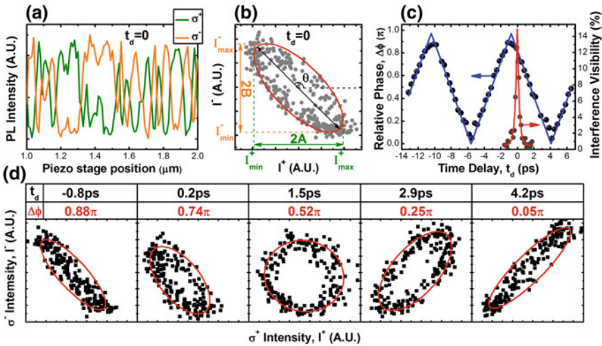
Fig. 4.12 a Interference fringes for \sigma^+ (green) and \sigma^- (orange) polarised light detected from O_T and O_R , recorded as the piezo mirror position is varied at t_d = 0 . b Intensity plot of the interference data presented in a showing that the \sigma^+ and \sigma^- transitions are \sim\pi out of phase at t_d = 0 . The red line is the elliptical fit to the data which is used to extract the relative phase between the \sigma^+ and \sigma^- transitions. c The left hand axis shows a plot of \Delta\phi as a function of the time delay. The blue line is a triangular waveform fit to the data. The right hand axis plots the visibility of the incoherent light interference of the QD and the fitting function (red) used to determine t_d = 0 . d Intensity plots of the interference fringes recorded simultaneously from the \sigma^+ and \sigma^- transitions at different delay times of the interferometer. The red lines are the elliptical fits to the data
