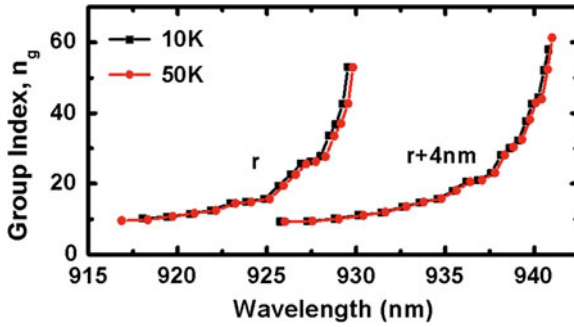
Fig. 3.15 Group Index for two PCWs recorded at temperatures of 10 K (black) and 50 K (red)
