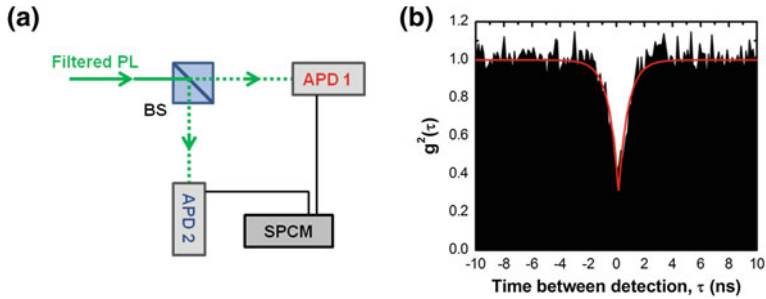
Fig. 2.7 a Schematic diagram of a Hanbury-Brown and Twiss experimental set-up. Spectrally filtered PL is incident on a beam-splitter (BS) and directed to two avalanche photo diodes (APD) that record incident photons and pass a signal to the single photon counting module (SPCM). The SPCM is responsible for recording a count conditioned on a detection of a previous photon detection signal. b An example of the coincident count histogram of detection events recorded by the SPCM for a single InAs QD transition. The function g^{(2)}(\tau) = (1 - (1 - M)e^{-|\tau|/\tau_d}) is fitted (red line) revealing a multi photon probability, M = 0.28 and lifetime of the QD \tau_d = 0.76 ns
