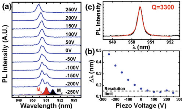
Fig. 7.15 a \mu PL spectra recorded from an H1 PC cavity as a function of piezo voltage from -250 to 250 V. b Cavity mode splitting as function of piezo voltage. c Unpolarised fundamental mode emission at a bias of 250 V, with a Q-factor of 3,300
