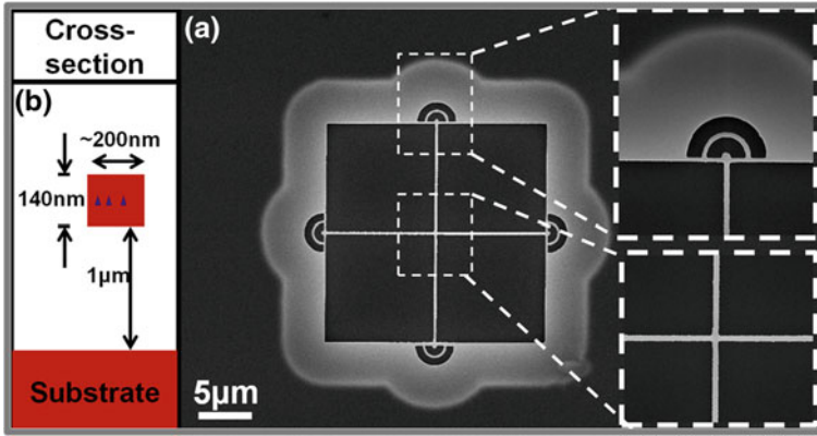
Fig. 4.5 a SEM image of a fabricated device. The crossed waveguides are terminated by four out-couplers. Inset, selected zoomed sections to highlight fabrication quality. b Schematic cross section of the prototype device. Free standing waveguides (nanowires) 200 nm wide and 140 nm deep contain a single layer of InAs QDs
