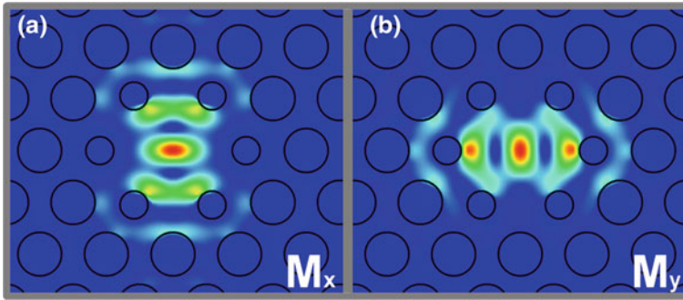
Fig. 7.13 Calculated electric field distributions for the a x-polarised and b y-polarised fundamental modes of the H1 PC cavity
