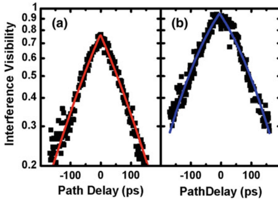
Fig. 5.4 Coherence time measurements of the a \sigma^+ and b \sigma^- transitions, respectively. The solid red and blue lines show fits to the data following Ref. [2]. Coherence times of 103 ps and 104 ps are found for the \sigma^+ and \sigma^- transitions, respectively
