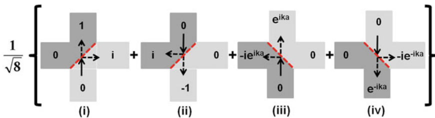
Fig. 5.10 The \hat{x} -polarised QD-dipole inputs light of wavevector \pm k\hat{y} . (i, ii) In the case of the +45^\circ beam-splitter, because the QD lies on the beam-splitter axis, these wave-vector components have identical input phase. (iii, iv) In the case of the -45^\circ beam-splitter, the QD lies above the beam-splitter axis and the different wave-vector components acquire a phase factor of e^{\pm ika} , where a = s/\sqrt{2} . The output is a superposition of the for possible input and beam-splitter configurations
