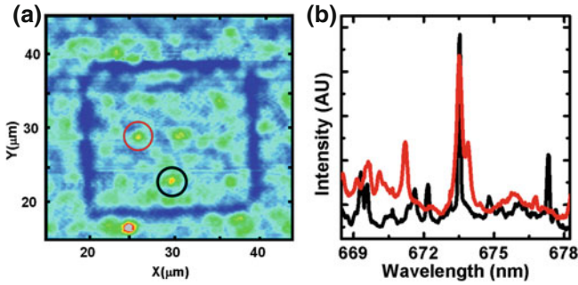
Fig. 7.8 a A PL map of one set of markers with the spectral window set at \sim 973.5 nm. Two spectra taken at the locations circled in (a) are colour coded and displayed in (b), b QD emission lines with wavelengths of 973.522 and 973.518 nm are observed
