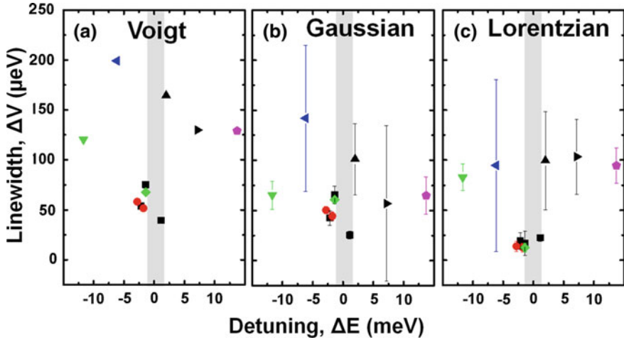
Fig. 6.6 Plots of the a Voigt b Gaussian c Lorentzian contribution to QD linewidths, \Delta V , extracted from C_2(t) as a function of detuning from the nearest photonic crystal mode, \Delta E . The grey region represents a typical FWHM for the photonic crystal modes studied with Q \sim 700 . Each individual QD transition is represented by one of eight unique shapes. Where a single shape is repeated, data has been recorded for the same QD transition on separate occasions when the relative QD to mode detuning has been tuned through nitrogen condensation. The data points are also colour coded ( pink, red, green, black, blue ) to group QD transitions that were observed in the same photonic crystal cavity from the five cavities studied
