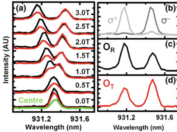
Fig. 4.10 a \mu PL spectra of a single quantum dot transition recorded from the crossed waveguide intersection, Centre (green), and two orthogonal out-couplers O_T (red) and O_R (black). Spectra are also displayed of the Zeeman split QD transition observed from O_T and O_R as a magnetic field is applied normal to the plane of the sample. b Spectra of the Zeeman split QD transition at B = 3T observed from the centre with polarisation sensitive detection of \sigma^+ (light grey) and \sigma^- (dark grey). c and d are the spectra of the Zeeman split QD transition at B = 3T recorded from O_R and O_T respectively
