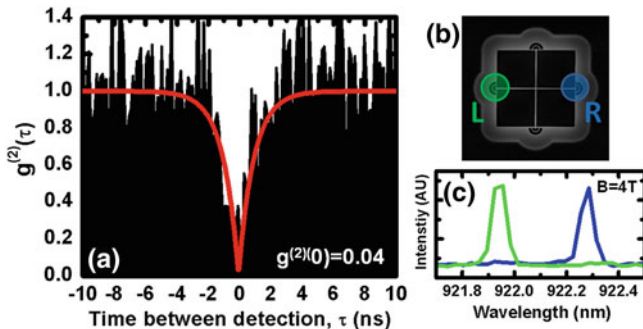
Fig. 5.3 Cross-correlation histogram recorded for the transitions in c on Device-B from O_R and O_L as depicted schematically in b . The red-line shows a fit to the data of the function g^{(2)}(\tau) = (1 - (1 - M)e^{-|\tau|/\tau_d}) , with M = 0.04 and \tau_d = 1.01 \text{ ns} . c The spectra of the QD transitions observed for the out-couplers O_R (blue) and O_L (green)
