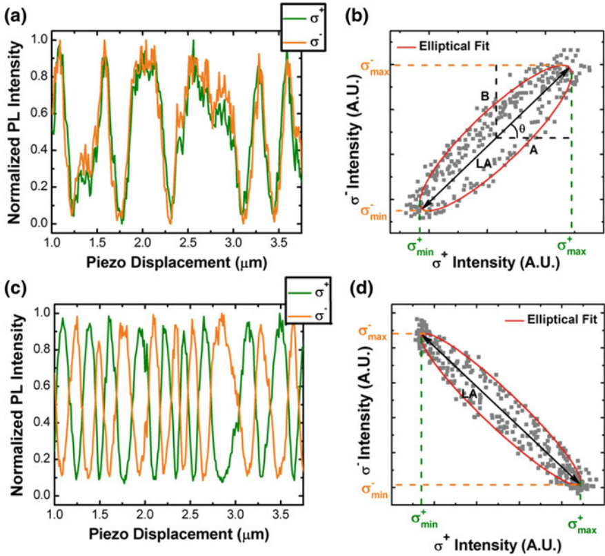
Fig. 4.3 a Interference fringes recorded when \Delta\phi = 0 and the \sigma^+ and \sigma^- polarised transitions are in phase, as the path delay in one arm of the interferometer is varied using the piezo-actuated mirror. b Scatter plot showing intensity of \sigma^- transition plotted against intensity of \sigma^+ transition for data in a . The red line shows an elliptical fit to the data, and the values LA, B, A and \theta are defined for use in extracting \Delta\phi . c , d Display the corresponding plots to a , b for the case where \Delta\phi = \pi and the \sigma^+ and \sigma^- polarised transitions are out of phase
