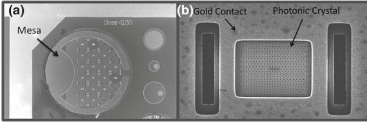
Fig. 7.9 SEM images of the photonic crystal P-I-N diodes. a A complete diode mesa. b A photonic crystal situated on the mesa labelled in (a) shown with the gold contact aperture around the photonic crystal
