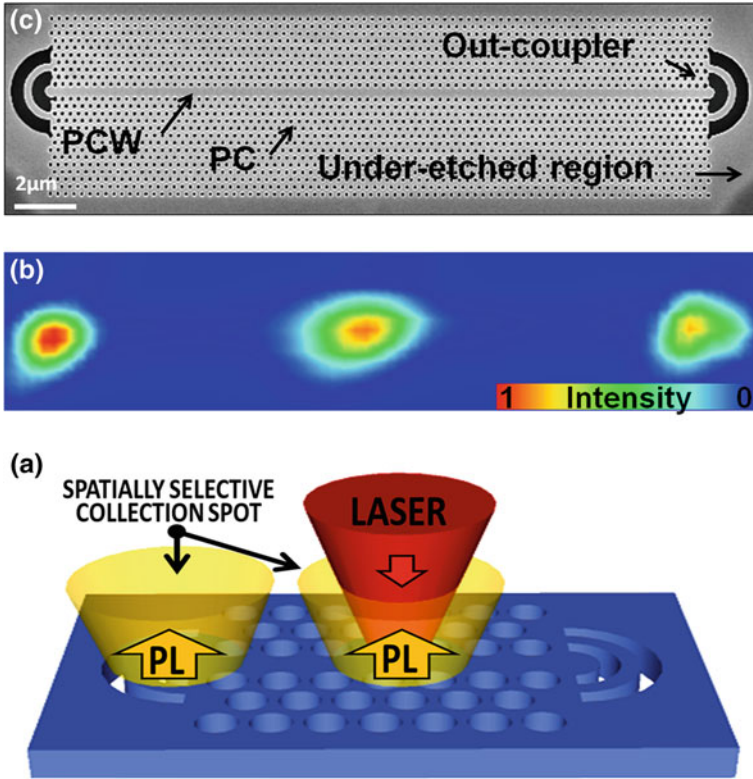
Fig. 3.3 a 3D diagram of the experimental set-up with laser excitation spot ( red cone ) and spatially selective PL collection ( yellow cones ) both of which can be independently positioned on the sample ( blue ). b PL intensity map of the PCW shown in the SEM diagram, c produced by scanning the spatially selective collection spot whilst the centre of the PCW was excited by a 850 nm laser. Three areas of bright PL are observed; at the location of excitation and from the the two outcouplers that terminate the PCW. This demonstrates that PL excited at the centre propagates along the PCW and is scattered vertically by the outcouplers
