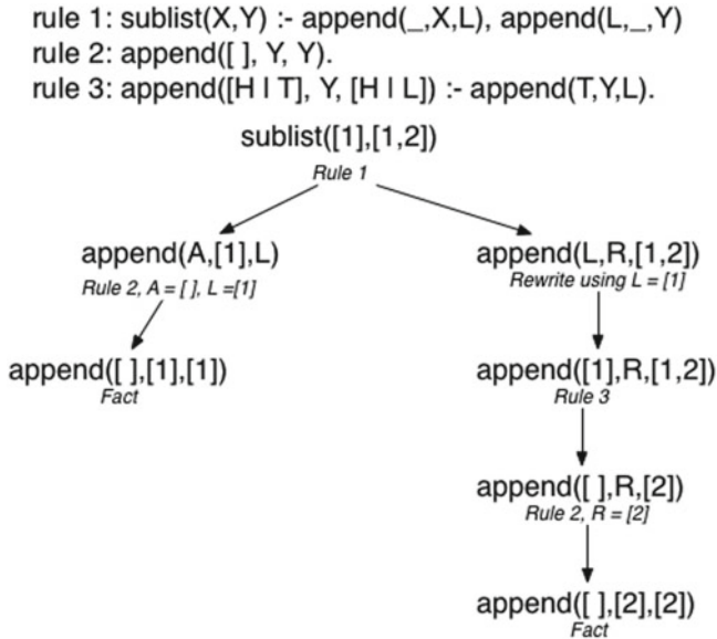
Fig. 7.3 A unification tree
