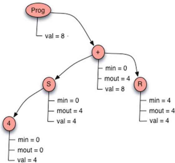
Fig. 7.11 Annotated AST for + S 4 R
