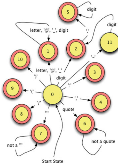
Fig. 4.29 The JCoCo scanner FSM
