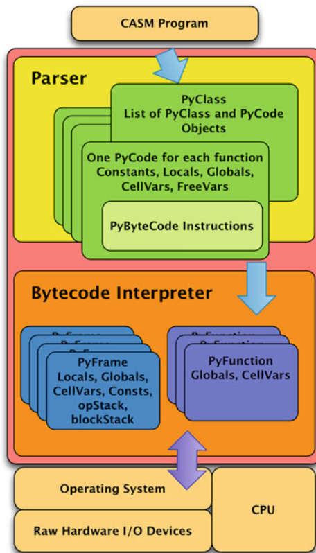
Fig. 4.2 The JCoCo virtual machine
