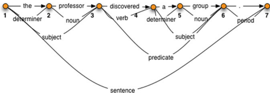
Fig. 7.8 An upside down parse tree
