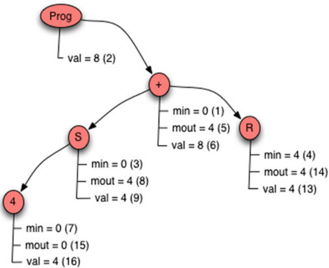
Fig. 7.14 Decorated tree for the prefix expression + S 4 R
