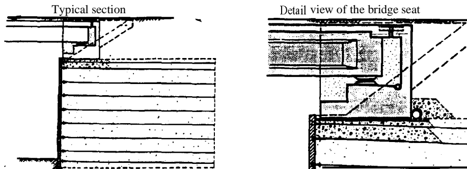
Fig 6.6.1-Abutment types
