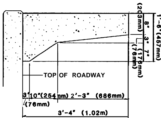
Fig. 2.2.1.5-Parapet curb and railing section
