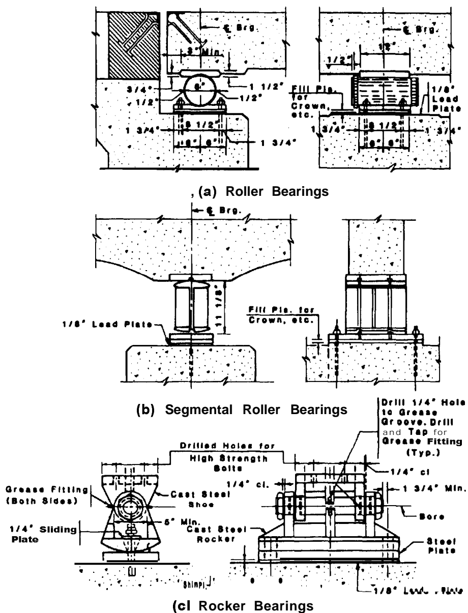
Fig. 11.2.2.4-Steel bearings
