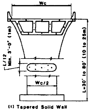
Fig. 11.6.2(e) and (f)-Multicolumn piers and tapered solid wall piers
