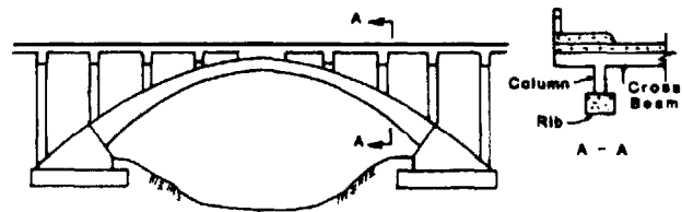
Fig. 2.5.5.2-Single span open spandrel or ribbed arch bridge
