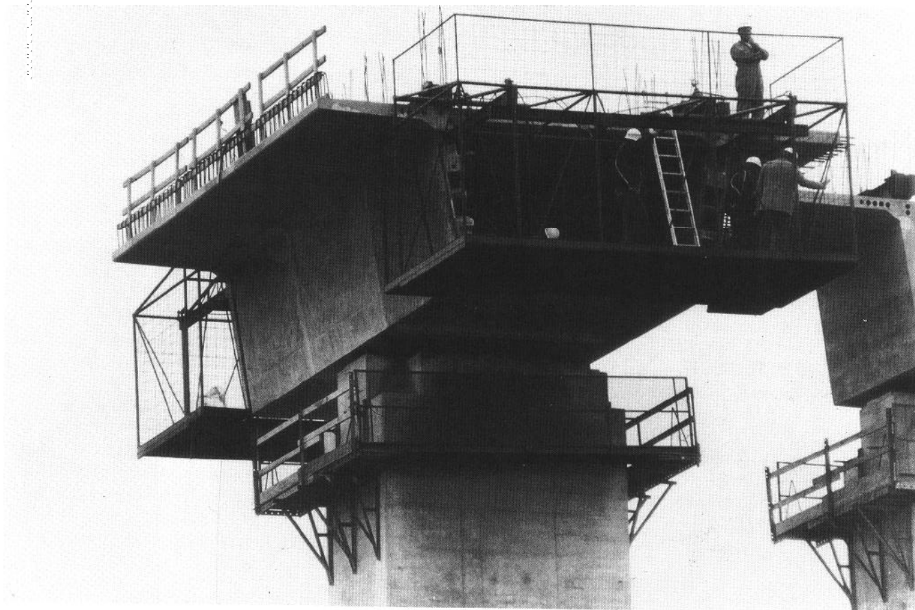
Construction of precast concrete box girder bridge (photo courtesy of Texas Highway Department)
