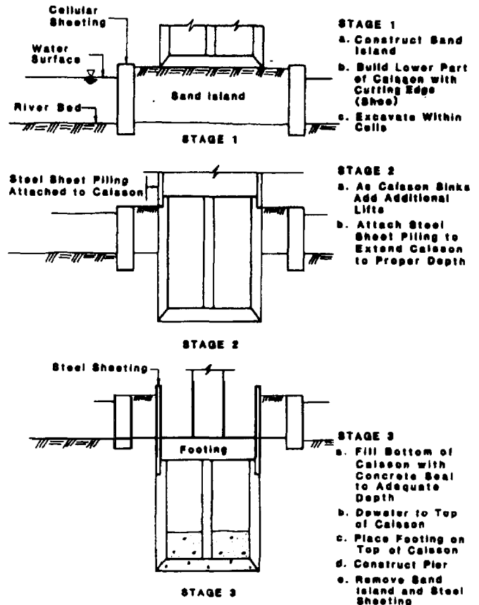
Fig. 11.3.6.1--Open-dredged caisson using sand island
