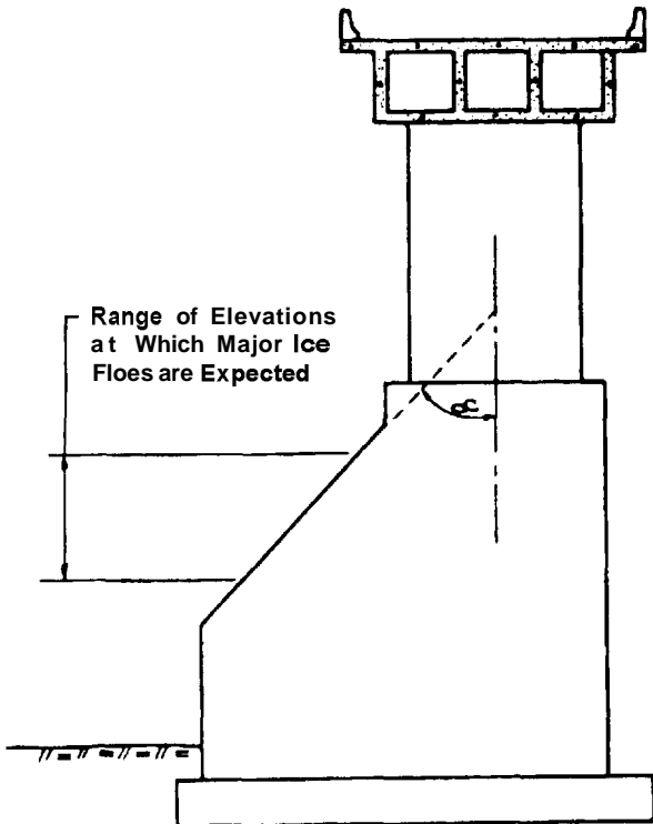
Fig. 11.6.2(j)-Piers with ice breaker
