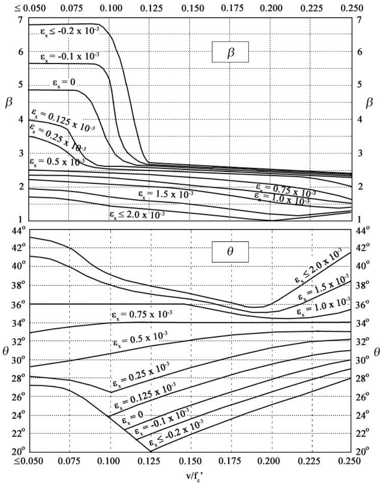
Figure 4-3: Values of \theta and \beta for Sections with Transverse Reinforcement
