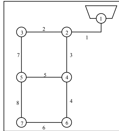
Figure 1. Layout of two loop pipe network
