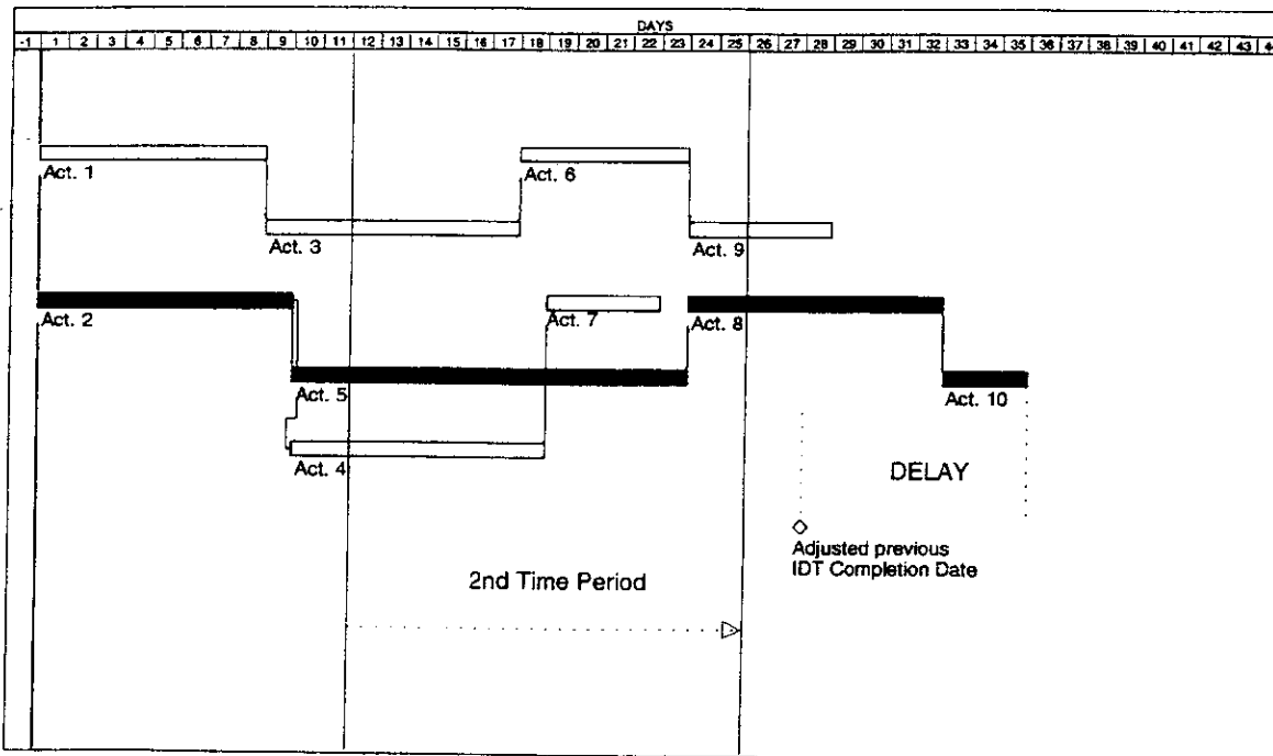
Figure 18 Second IDT analysis (from the contractor's point of view)
