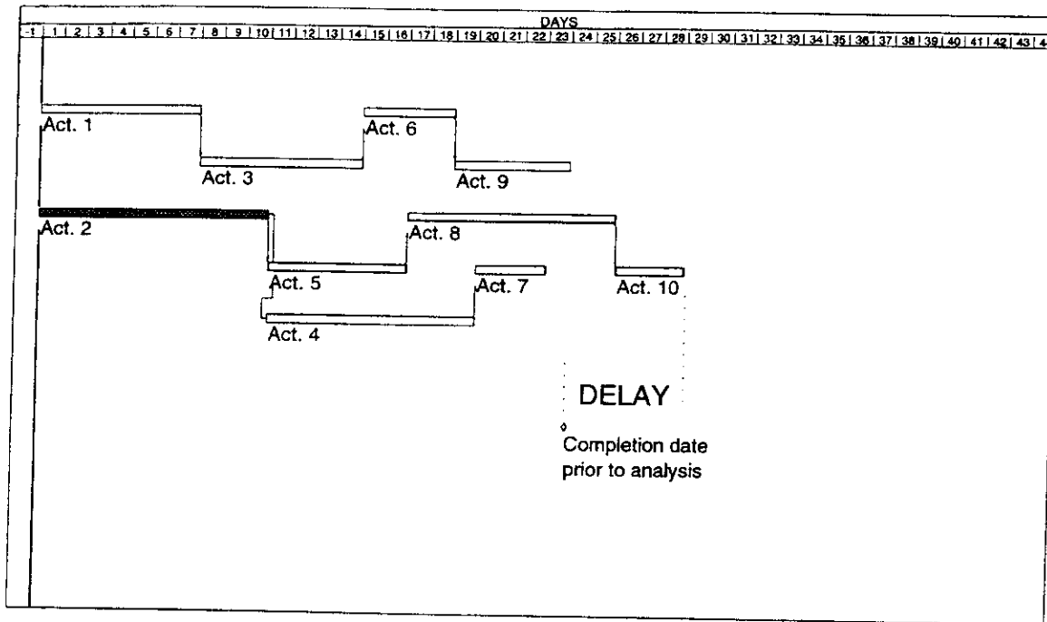
Figure 12 Time impact technique - activity 2
