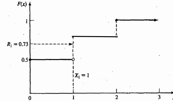
Figure 8.6 Cdf of number of shipments, X .
