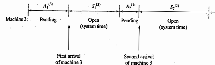
Figure 6.2 Arrival process for a finite-population model.
