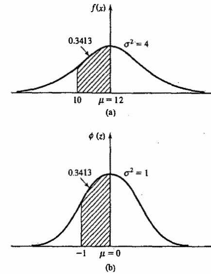
Figure 5.16 Transformation to standard normal for vessel-loading problem.
