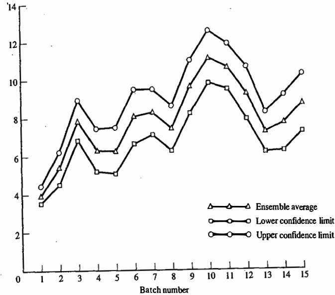
Figure 11.6 Ensemble averages \bar{Y}_j for M/G/1 queue with 95% confidence intervals.
