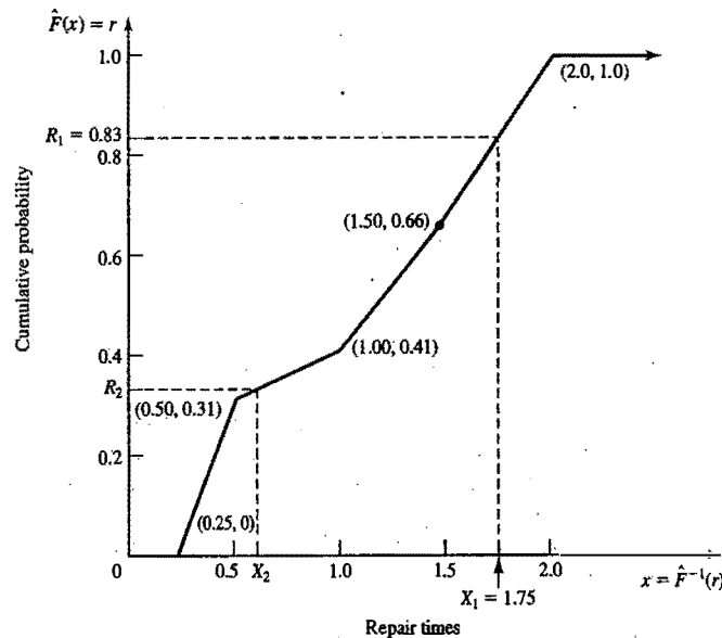
Figure 8.5 Generating variates from the empirical distribution function for repair-time data ( X \geq 0.25 ).
