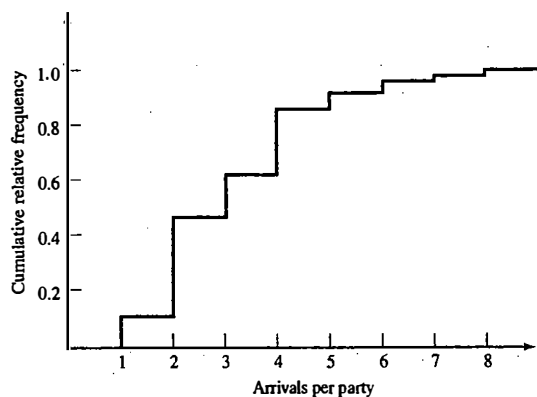
Figure 5.28 Empirical cdf of party size.
