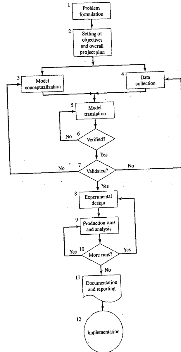
Figure 1.3 Steps in a simulation study.
