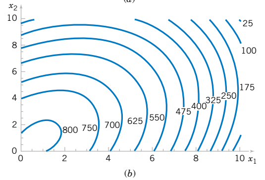
Figure 12-3 (a) Three-dimensional plot of the regression model E(Y) = 800 + 10x_1 + 7x_2 - 8.5x_1^2 - 5x_2^2 + 4x_1x_2 . (b) The contour plot.
