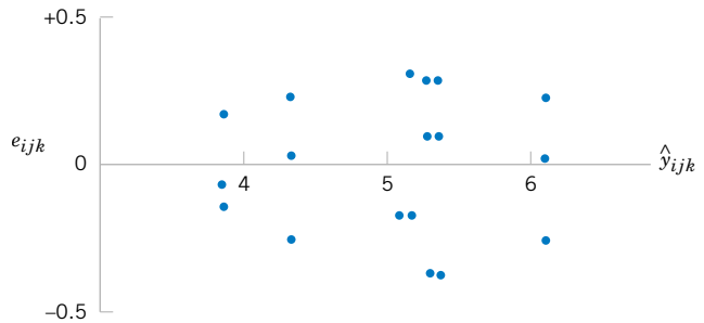
Figure 14-14 Plot of residuals versus predicted values \hat{y}_{ijk} .
