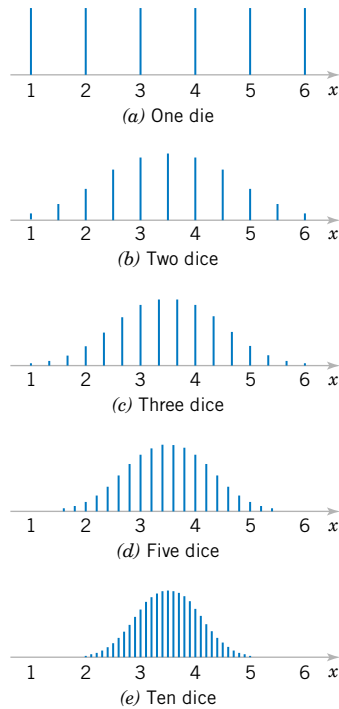
Figure 7-1 Distributions of average scores from throwing dice. [Adapted with permission from Box, Hunter, and Hunter (1978).]
