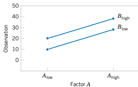
Figure 14-3 Factorial experiment, no interaction.
