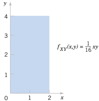
Figure 5-16 Random variables with zero covariance from Example 5-22.
