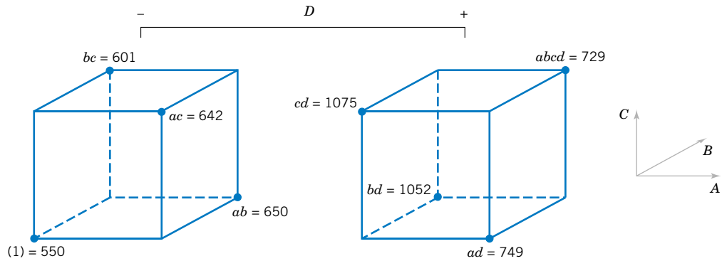
Figure 14-33 The 2^{4-1} design for the experiment of Example 14-8.
