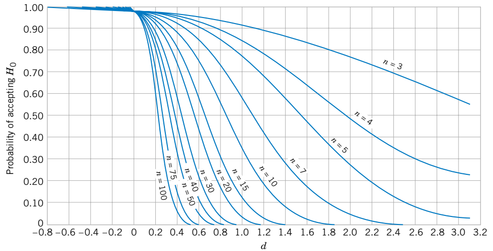
(h) O.C. curves for different values of n for the one-sided t -test for a level of significance \alpha = 0.01 .
