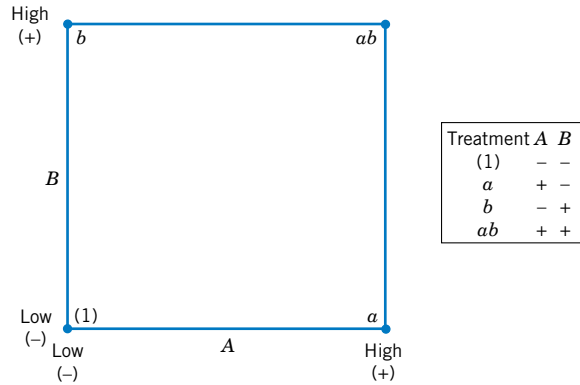
Figure 14-15 The 2^2 factorial design.
