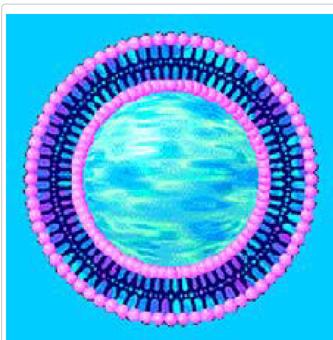
Figure 4: Structure of Liposomes.
