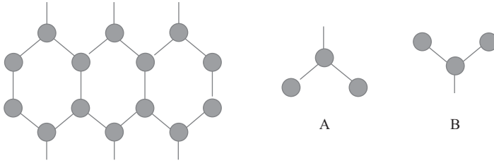
Figure 2.8 Interpenetrating sublattices
