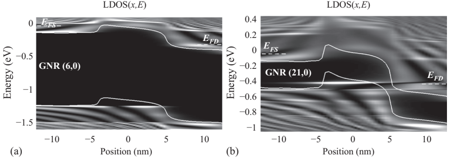
Figure 4.5 Local DOS of GNRFET with the channel of (a) GNR (6,0) and (b) GNR (21,0). Note that the gate voltage V_G = 0.5\text{ V} and drain voltages of GNR (6,0) and GNR (21,0) are V_D = 0.3 and 0.4\text{ V} , respectively. The oxide thickness t_{ox} and the physical gate length L_G are 1 and 5 nm, respectively. The dielectric layer is assumed to be aluminum nitride (AlN) with the relative dielectric permittivity k = 9
