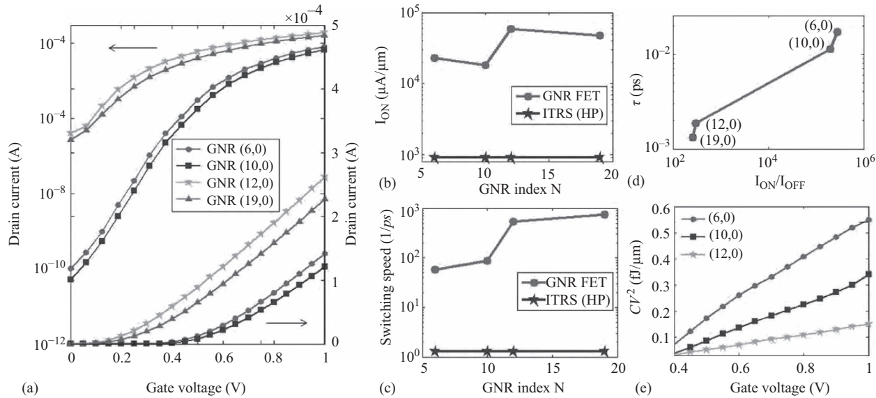
Figure 4.11 Transfer characteristics of GNR FET for different graphene nanoribbons, (b) on-current density versus GNR index, (c) switching speed versus GNR index and ITRS projection, (d) intrinsic gate-delay versus I_{ON}/I_{OFF} ratio, (e) dynamic power versus gate voltage for GNR (6,0), GNR (10,0), and GNR (12,0)
