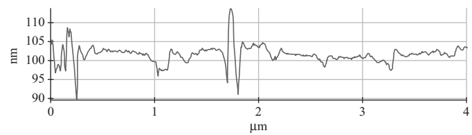
Figure 2.10 HR-AFM of domained GaSb/AlSb/Si surface
