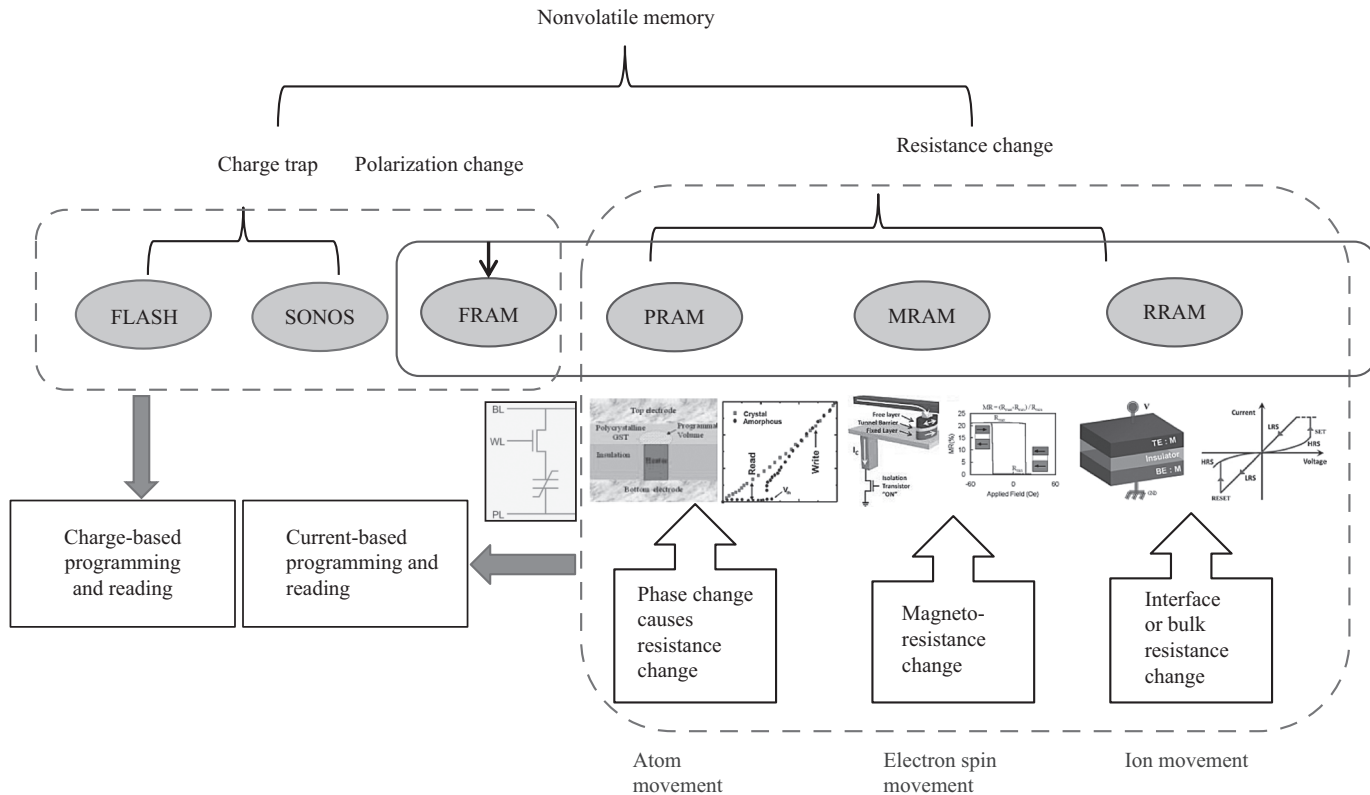
Figure 12.1 Various nonvolatile memory technologies classified in terms of the switching mechanisms involved in their operation Source: Yole Development; Leti, 2012
