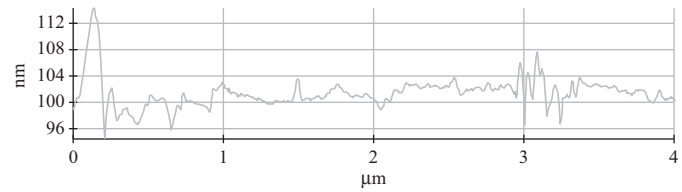
Line profile: Blue
