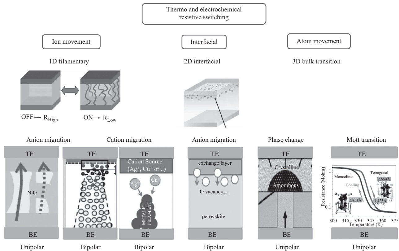
Figure 12.4 Fundamental characteristics of different two terminal thermo- and electrochemical switching devices
