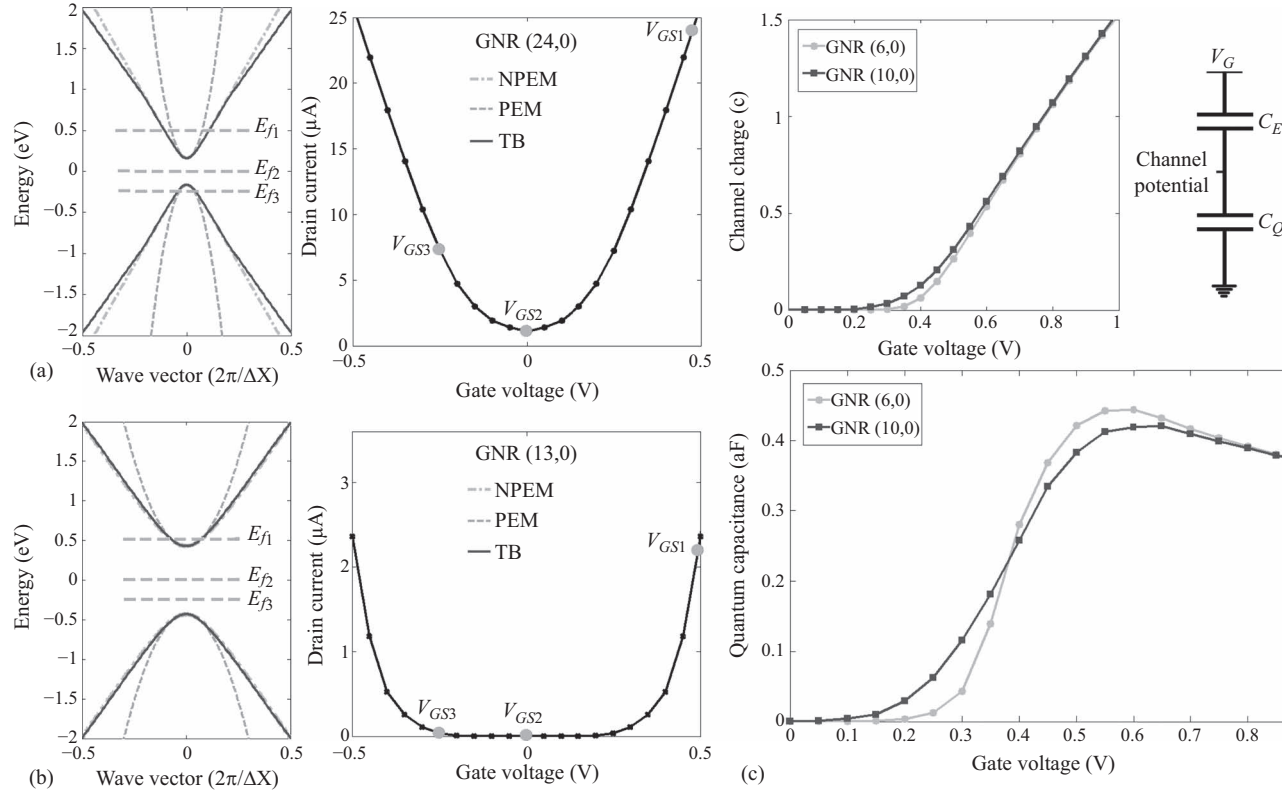
Figure 4.7 First conduction and valence bands of (a) GNR (24,0) and (b) GNR (13,0) and corresponding drain current-gate voltage characteristics. Note that three Fermi levels and the corresponding gate voltages are also shown. (c) Channel charge and corresponding quantum capacitance versus gate voltage for GNR (6,0) and GNR (10,0). Note that the series configuration of electrostatic capacitance and quantum capacitance is also shown
