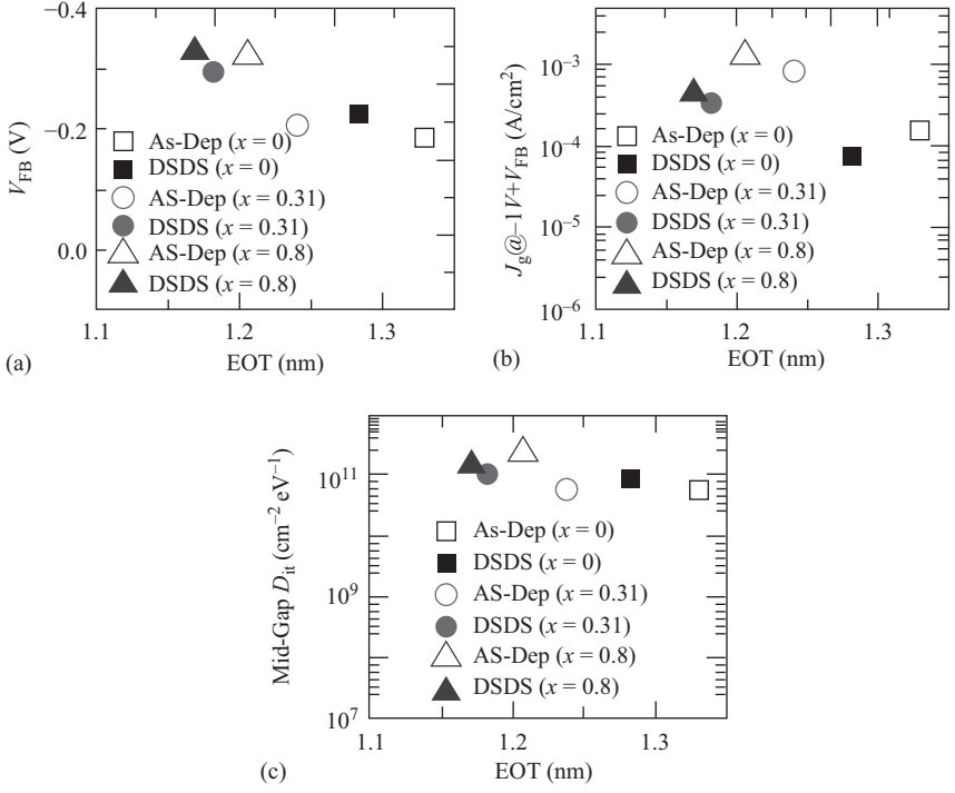
Figure 1.5 (a) Flat-band voltage as a function of EOT for DSDS and As-Dep Hf_{1-x}Zr_xO_2 with x = 0, 0.31 , and 0.8 , (b) comparison of gate leakage current density sensed at -1V + V_{FB} , and (c) comparison of the mid-gap level D_{it} as a function of EOT for different dielectrics
