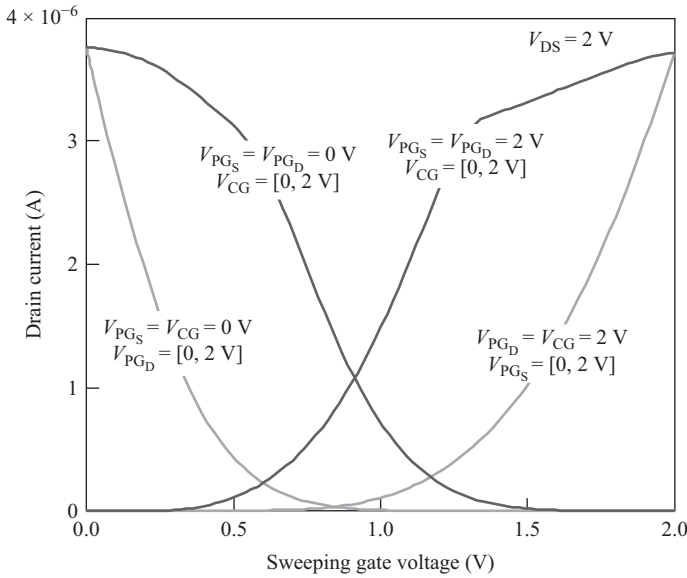
Figure 8.6 Simulation dual- V_T characteristics of an optimized TIG SiNWFET
