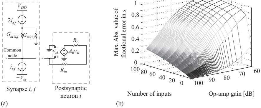
Figure 12.7 (a) Simplified model of the synapse connected to the input of a postsynaptic neuron. (b) Number of neuron inputs and op-amp gain versus the maximum absolute value of the fractional error between the total synaptic output current and the ideal total synaptic output current
