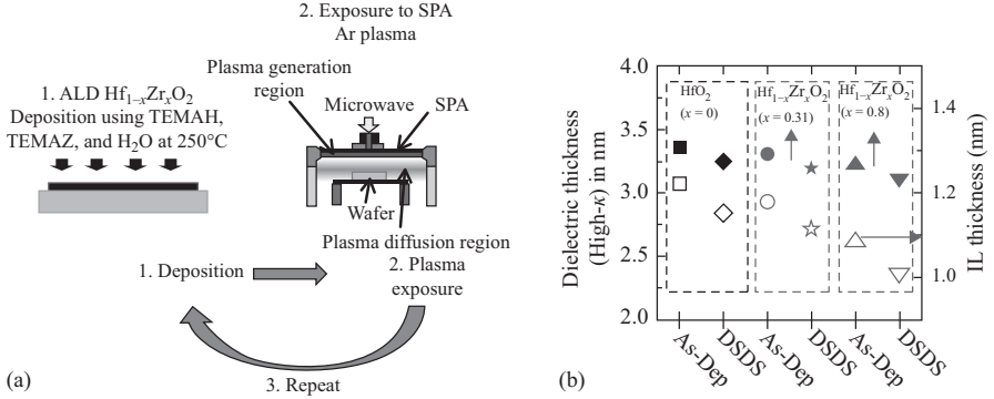
Figure 1.4 (a) Schematic representation of DSDS process using an SPA plasma in a cluster tool system. (b) Dielectric thickness (filled symbols on left scale) and IL thickness (open symbols on right scale) for MOSCAPs with DSDS and As-Dep \text{HfO}_2 ( x=0 ), \text{Hf}_{1-x}\text{Zr}_x\text{O}_2 ( x=0.31 ), and \text{Hf}_{1-x}\text{Zr}_x\text{O}_2 ( x=0.8 ). Abbreviations: MOSCAP, metal oxide semiconductor capacitor; DT, direct tunneling; RF, radio frequency; RLSA, radial line slot antenna; TEMAZ, tetrakis (ethylmethylamido) zirconium; ESC, electrostatic chuck; F–N, Fowler–Nordheim; P–F, Poole–Frenkel
