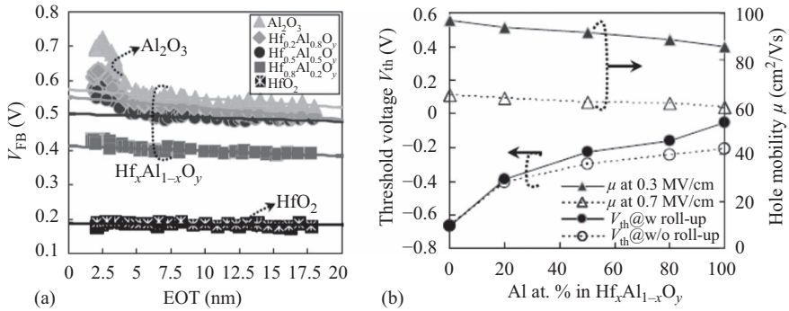
Figure 1.10 (a) V_{FB} – EOT plots for NiSi/Hf_xAl_{1-x}O_y /terraced SiO_2/n - Si p-MOSFETs. All samples were subjected to PDA at 800^\circ C and post-Si deposition annealing at 1000^\circ C . (b) Dependencies of V_{th} and hole mobility at both 0.3 and 0.7 MV/cm on Al content in Hf_xAl_{1-x}O_y for NiSi/Hf_xAl_{1-x}O_y/SiO_2 (1 nm)/Si p-MOSFETs. The closed circles stand for experimental V_{th} that takes V_{FB} roll-up effects into consideration, and the open circles stand for estimated V_{th} that excludes V_{FB} roll-up effects, which have been calculated qualitatively by comparing measured data with fitted linear V_{FB} – EOT relationship in (a) Source: © 2009 AIP Publishing LLC. Reprinted, with permission, from W. Wang, K. Akiyama, W. Mizubayashi, T. Nabatame, H. Ota, and A. Toriumi, “Effect of Al-diffusion-induced positive flatband voltage shift on the electrical characteristics of Al-incorporated high-k metal-oxide-semiconductor field-effective transistor,” J. Appl. Phys. 2009, vol. 105(6), pp. 064108-1–6
