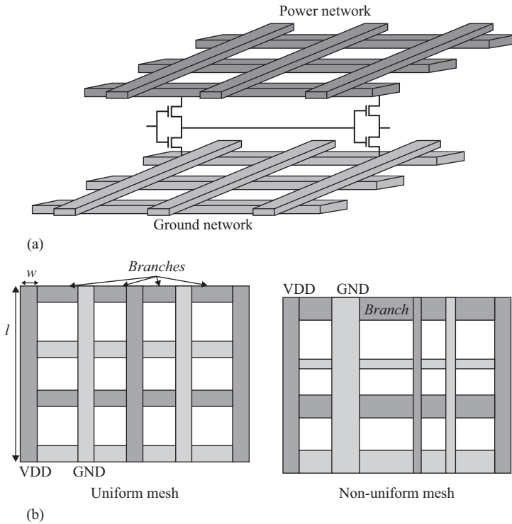
Figure 9.2 (a) Illustration of global power delivery network for a single tier and (b) description of uniform and non-uniform power delivery networks. The meshes have the same area and regular structure but some tracks have different widths, thus varying the branch lengths
