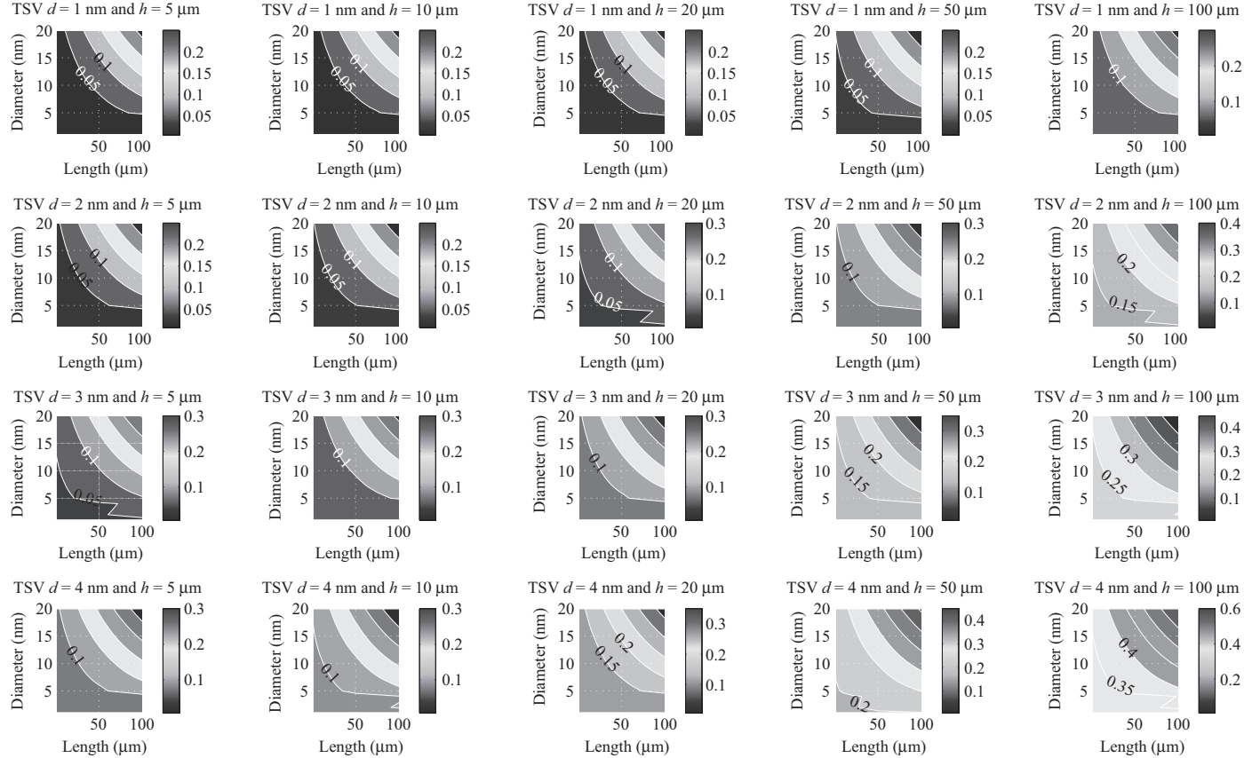
Figure 9.16 Total voltage drop on 3D power delivery network considering the voltage drop on Tier 1, TSVs and Tier 2. Each figure shows the total voltage drop as a function of branch CNT length and diameters (both Tier 1 and Tier 1 branches are uniform) and also as dimensions of TSV diameter and height
