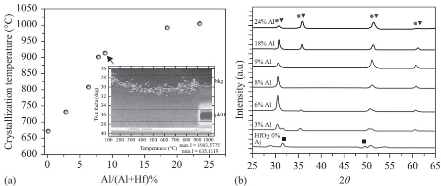
Figure 1.8 (a) Crystallization temperature of \text{Hf}_{1-x}\text{Al}_x\text{O}_y as a function of \text{Al}/(\text{Al} + \text{Hf})\% in the dielectrics. Inset shows XRD plot at the onset of crystallization for \text{Hf}_{1-x}\text{Al}_x\text{O}_y with x = 0.09 . (b) Synchronous grazing in plane XRD pattern for ALD \text{Hf}_{1-x}\text{Al}_x\text{O}_y as a function of \text{Al}/(\text{Al} + \text{Hf})\%
