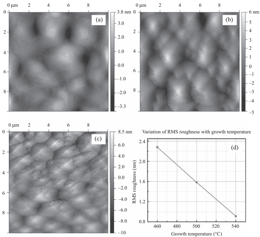
Figure 2.1 AFM images of 2 \mu\text{m} thick IMF-grown GaSb epilayers on GaAs at different growth temperatures. (a) 540^\circ\text{C} , (b) 500^\circ\text{C} , (c) 460^\circ\text{C} , (d) graph showing the variation of surface roughness with growth temperature, \text{RMS}_{\text{sq}} = 2.28 \text{ nm} at 460^\circ\text{C} , 1.582 \text{ nm} at 500^\circ\text{C} , and 0.912 \text{ nm} at 540^\circ\text{C}
