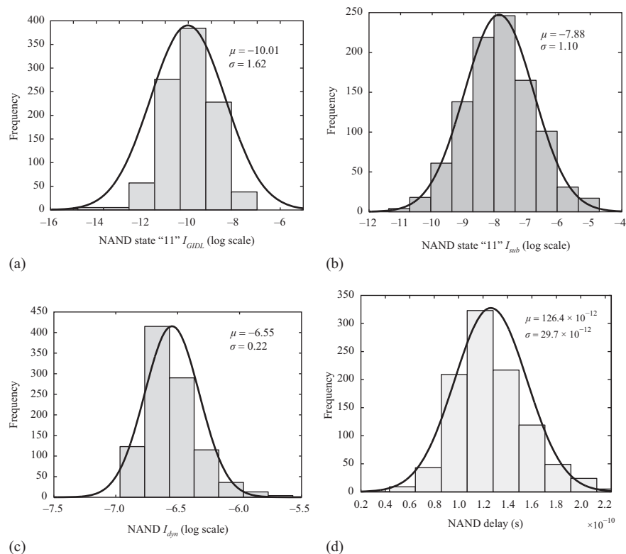
Figure 6.13 Distributions of GIDL current ( \hat{I}_{GIDL} ) and sub-threshold current ( \hat{I}_{sub} ) for input 11, and dynamic current ( \hat{I}_{dyn} ) and propagation delay for HKMG-based two-input NAND gate. (a) State 11: GIDL, (b) State 11: sub-threshold, (c) average: I_{dyn} , and (d) average: delay
