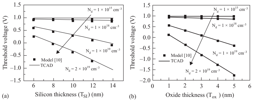
Figure 5.3 V_{th} fluctuation according to various (a) T_{SI} (b) T_{ox} in JL-DGFET as a parameter of doping concentration. V_{th} model data is taken from reference 10
