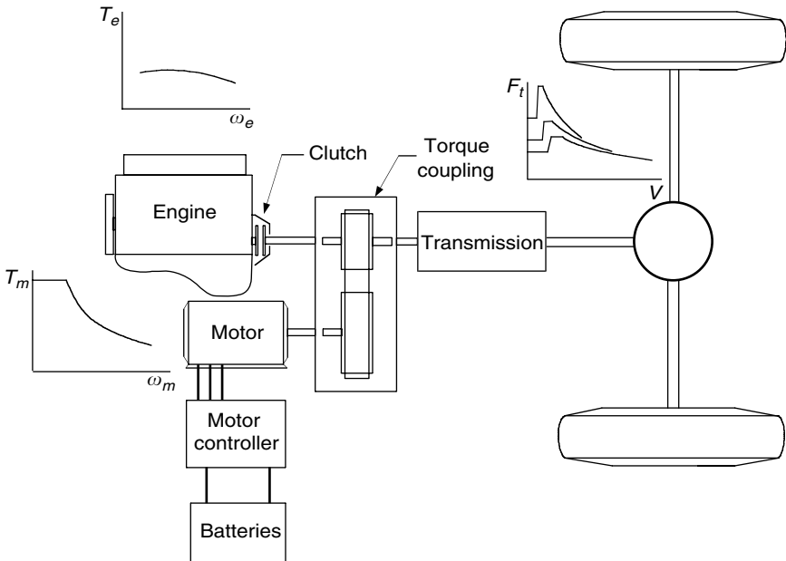
FIGURE 5.10 Two-shaft configuration
