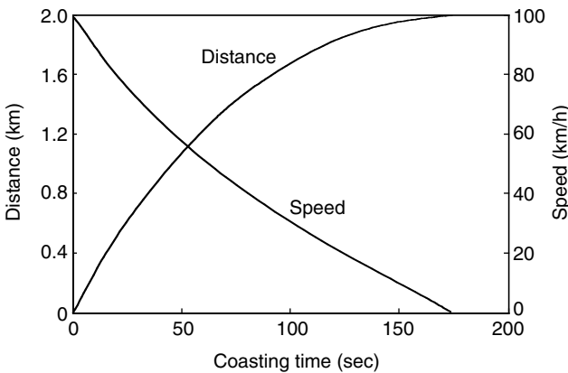
FIGURE 11.1 Coasting speed and distance
