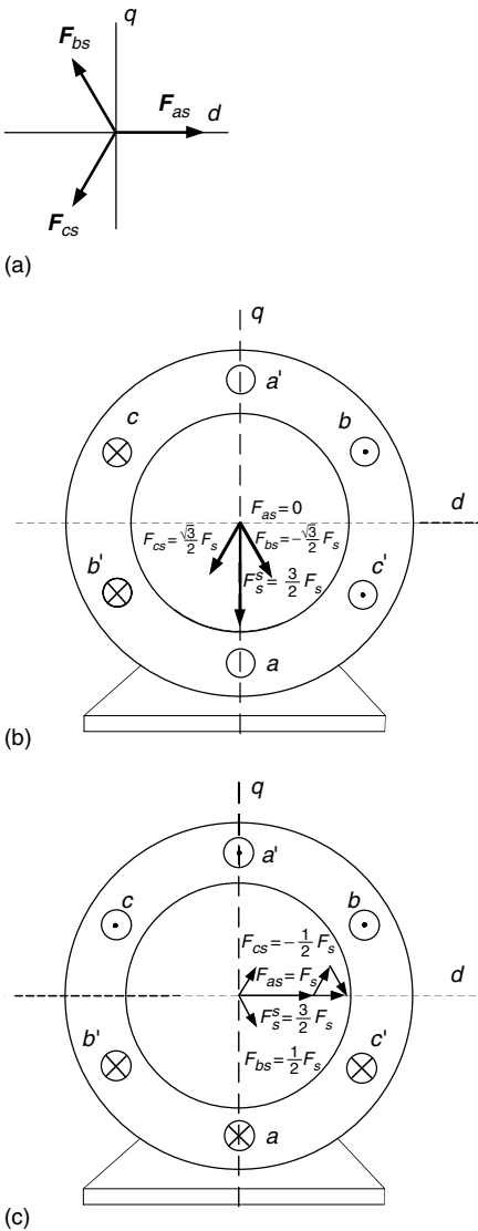
FIGURE 6.16 Stator mmf vectors: (a) positive direction of each phase (b) stator mmf vectors at \omega t = 0 and (c) stator mmf vectors at \omega t = 90^\circ
