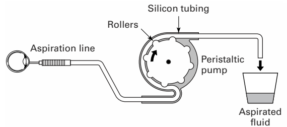
Figure 4.7 Peristaltic pump.
