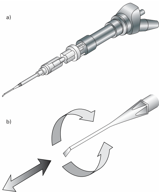
Figure 4.13 Neosonix (Alcon). (a) Hand piece: internal view. (b) Action: oscillatory motion in addition to conventional ultrasonic energy ( \pm 2^\circ at 100 Hz).
