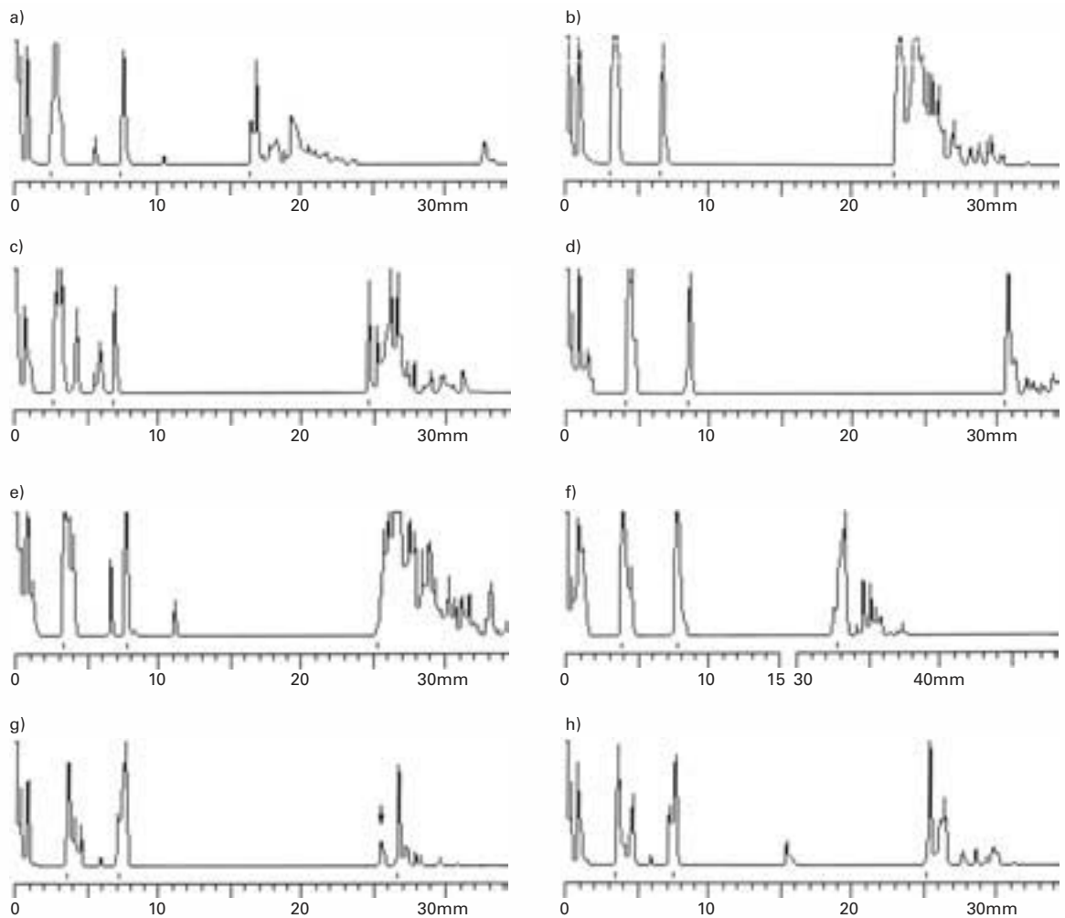
Figure 6.3 A-mode traces: cursors directly above horizontal axis indicate echoes accepted by machine in measurement. (a) Nanophthalmic eye (visual axis). (b) Average length eye (visual axis). (c) Dense cataract with multiple internal lens echoes (visual axis). (d) Highly myopic eye (visual axis). (e) Posterior staphyloma: note the gradual slope of vitreo-retinal interface (visual axis). (f) Highly myopic eye with posterior staphyloma: note the gradual slope of vitreo-retinal echo (visual axis). (g) Non-visual axis A-mode trace: system ignores vitreo-retinal interface echo (arrow) as amplitude too low and accepts echo from a more posterior structure; measurement 1.4 mm too long. (h) Same eye as (g) but with visual axis alignment.
