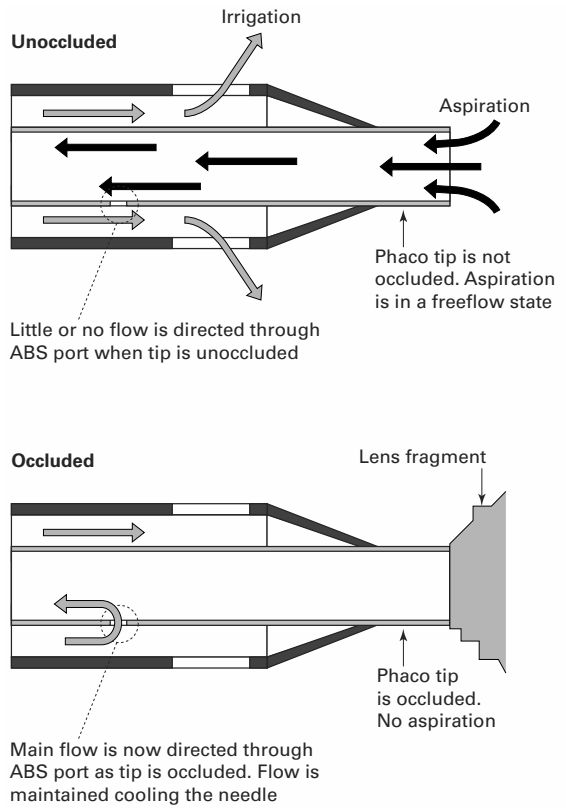
Figure 4.12 Aspiration bypass tips.
