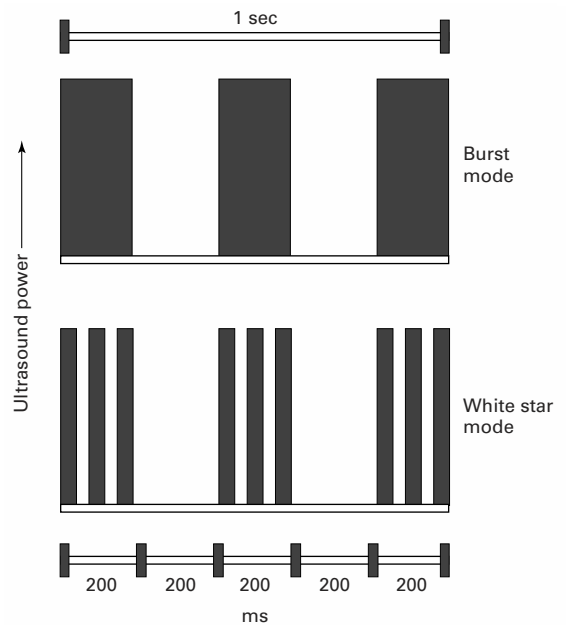
Figure 4.14 Burst mode versus Whitestar (Allergan; 600 ms duty cycle/400 ms rest).
