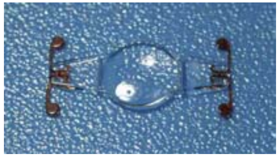
Figure 7.16 Accommodative silicone model AT-45 hinged plate intraocular lens (C&C Vision).
