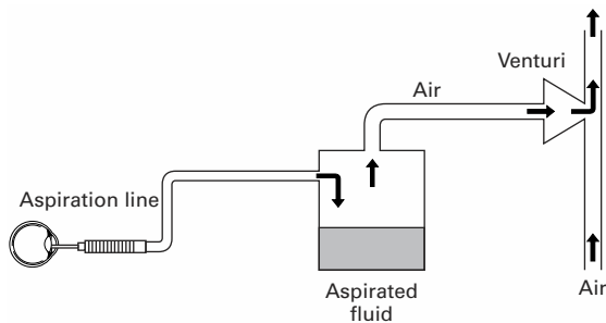
Figure 4.8 Venturi pump.
