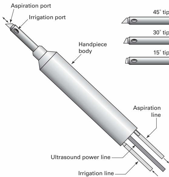
Figure 4.2 Hand piece with irrigation/aspiration channels and different tip angles.
