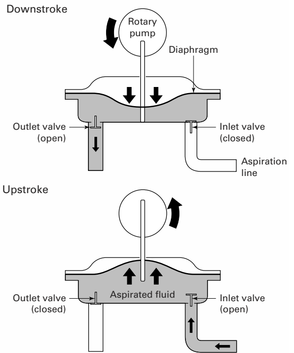
Figure 4.9 Diaphragm pump.
