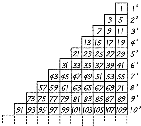
FIG 1. THE ARITHMETIC TRIANGLE OF FIBONACCI
