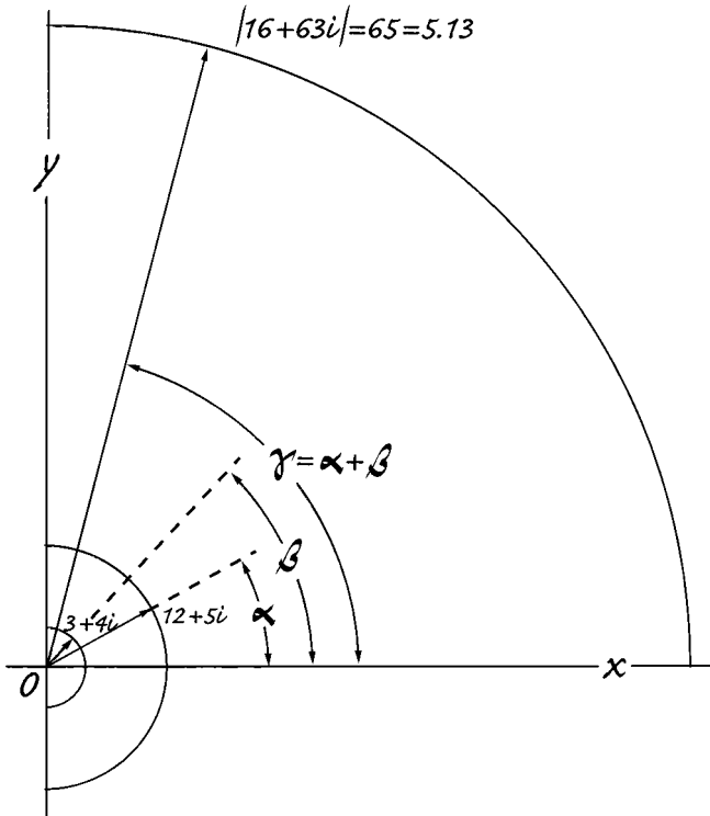
FIG. 3. COMPOUND TRIPLES AND COMPLEX INTEGERS
