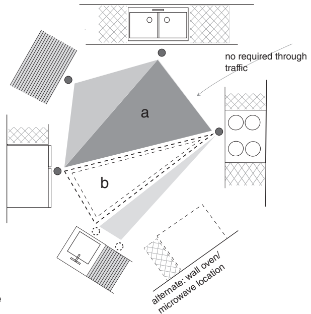
Figure 4-7b The two-cook kitchen can be designed based on doubled-double work triangles. It consists of two triangles (a and b) connecting the major centers (using two sinks) and two secondary triangles connecting preparation/work areas with the sink and refrigerator (the primary prep area should be 36 inches [914 mm] wide).
