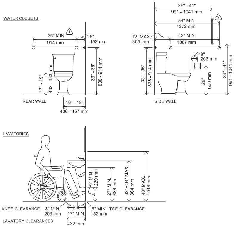
Figure 6-28a Wheelchair-accessible toilet and lavatory elevations. Note that lavatory height is listed as 34 inches (864 mm) maximum; however, the IDEA Center recommends 32 inches (813 mm) for residences. See also Figure 6-25.
