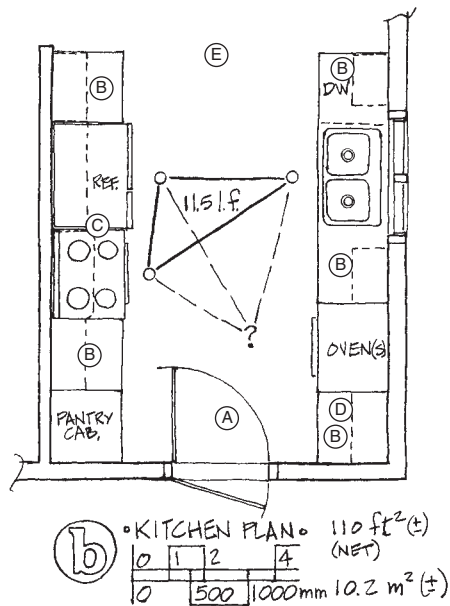
Figure 4-52 Negative example. Problematic kitchen plan.
