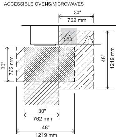
Figure 4-24b Wall oven/microwave clearances and clear counter space for wheelchair users.
