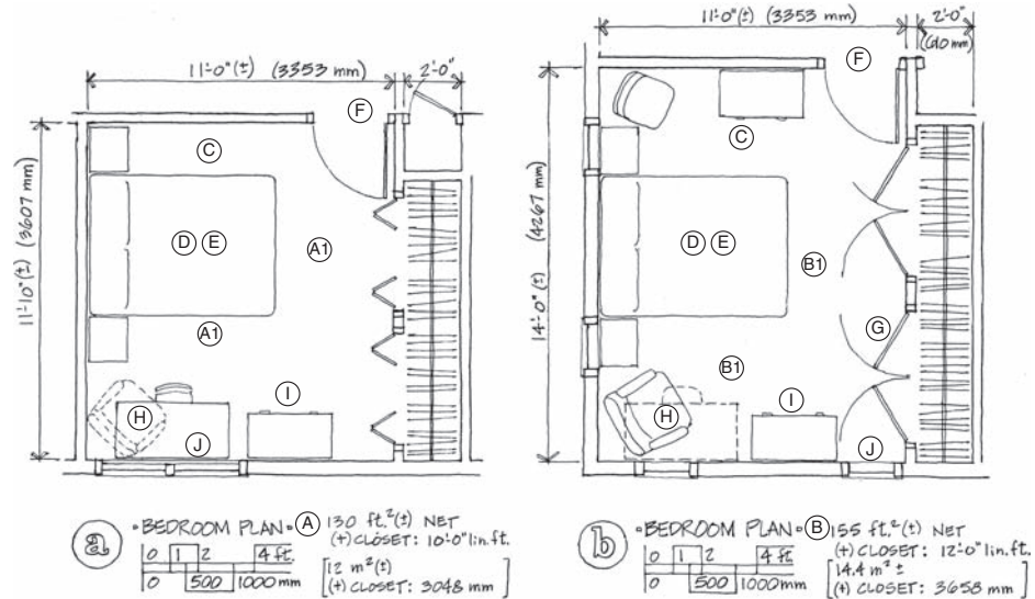
Figure 5-16 Room size, circulation, and furniture layout.
