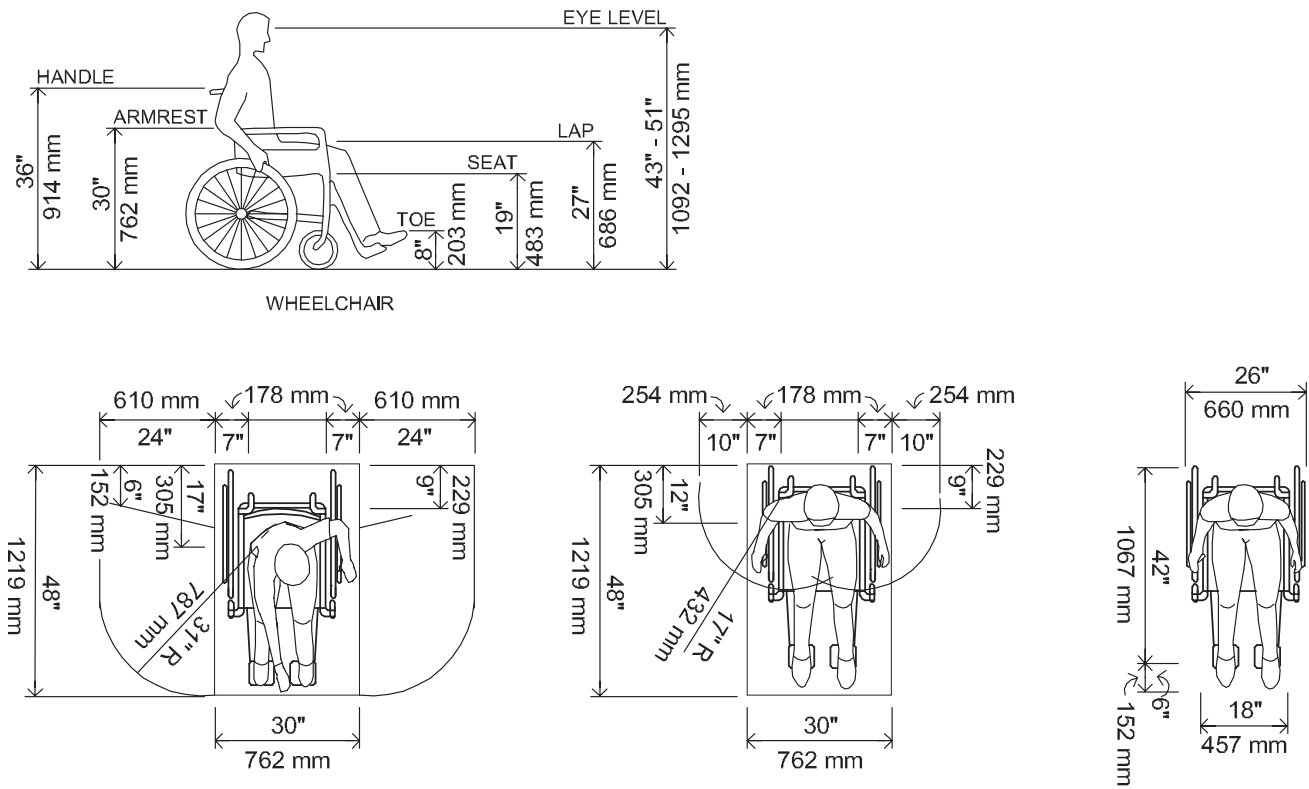
Figure C-1 Dimensional information for wheelchairs and users.
