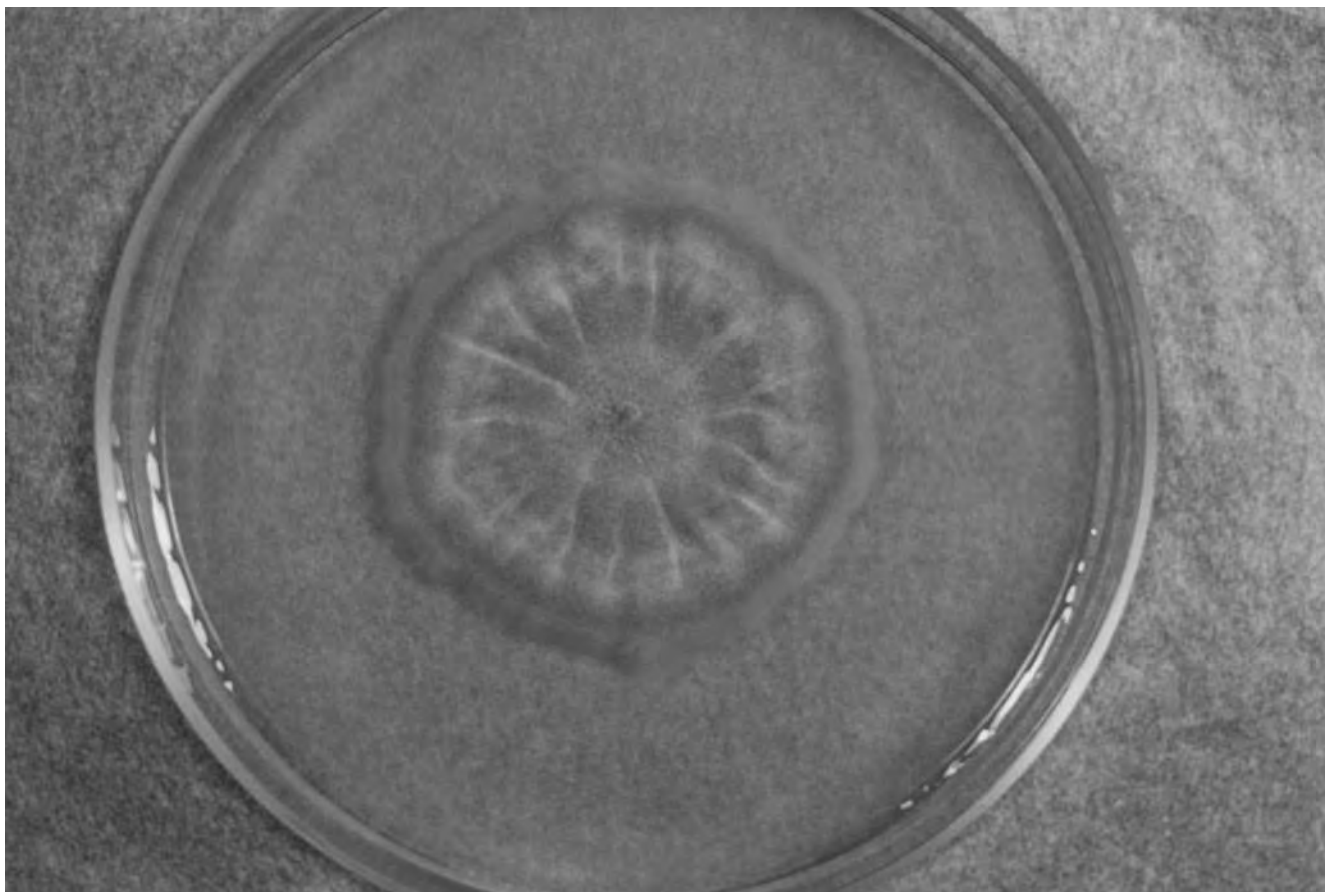
Fungus colony.
