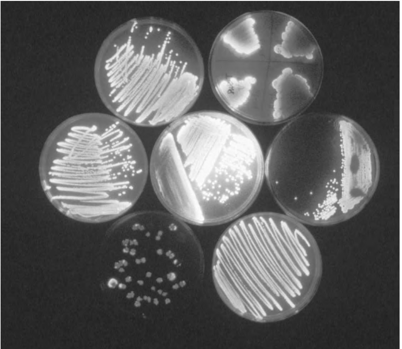
Bioluminescent bacteria.
