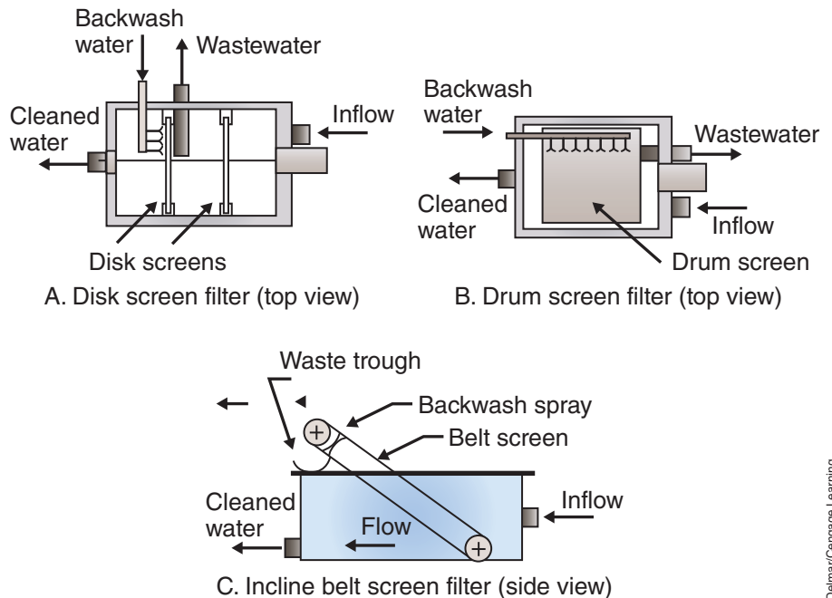
FIGURE 15-3 Examples of how three screen filters work to capture and remove suspended solids.
