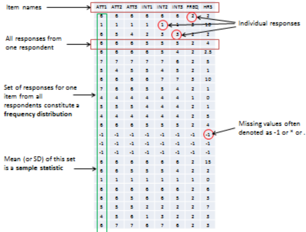
Figure 8.2. Sample Statistic
