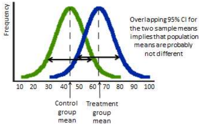
Figure 15.2. Student's t-test
