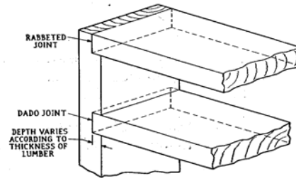
Fig. 13 Dado and Rabbet joints
