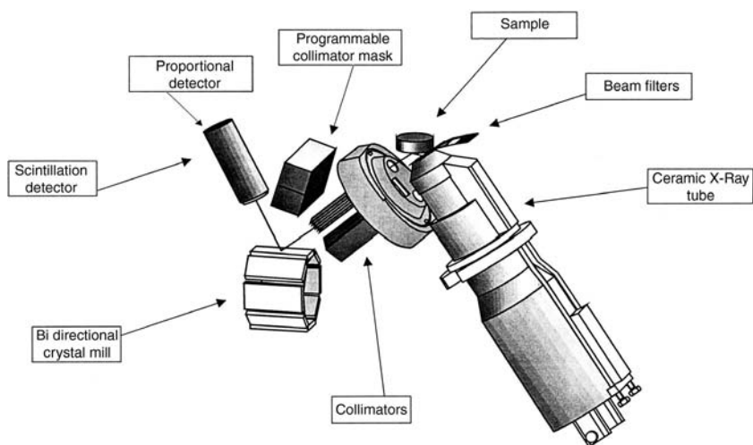
Figure 8.17 The schematic layout of a commercial sequential X-ray spectrometer, the MagiX, showing a series of selectable beam filters located between the X-ray tube and the sample. [Courtesy of PANalytical, Inc., The Netherlands ( www.panalytical.com ).]
