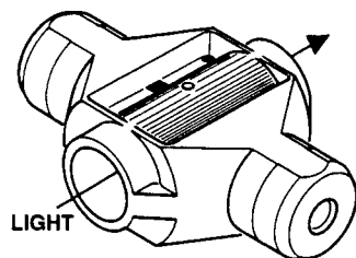
Figure 6.12 A graphite tube for a transversely heated furnace. [Courtesy of PerkinElmer Inc., Shelton, CT ( www.perkinelmer.com ).]
