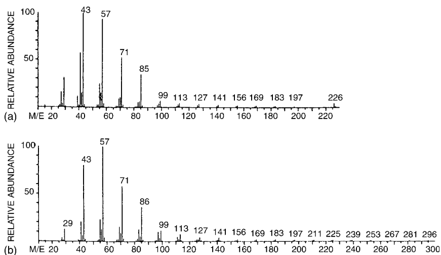
Figure 10.13 (a) Mass spectrum of n -hexadecane, \text{C}_{16}\text{H}_{34} and (b) n -tridecane, \text{C}_{30}\text{H}_{62} . The MW of n -hexadecane is 226 Da; the molecular ion is visible in spectrum (a) but small. The MW of n -tridecane is 422 Da; the spectrum does not extend far enough to see the molecular ion, but it would be very small as well. Both n -alkanes show a similar pattern of peaks separated by 14 Da, due to the loss of \text{CH}_2 groups and both show very similar patterns at the low m/z end of the spectrum.
